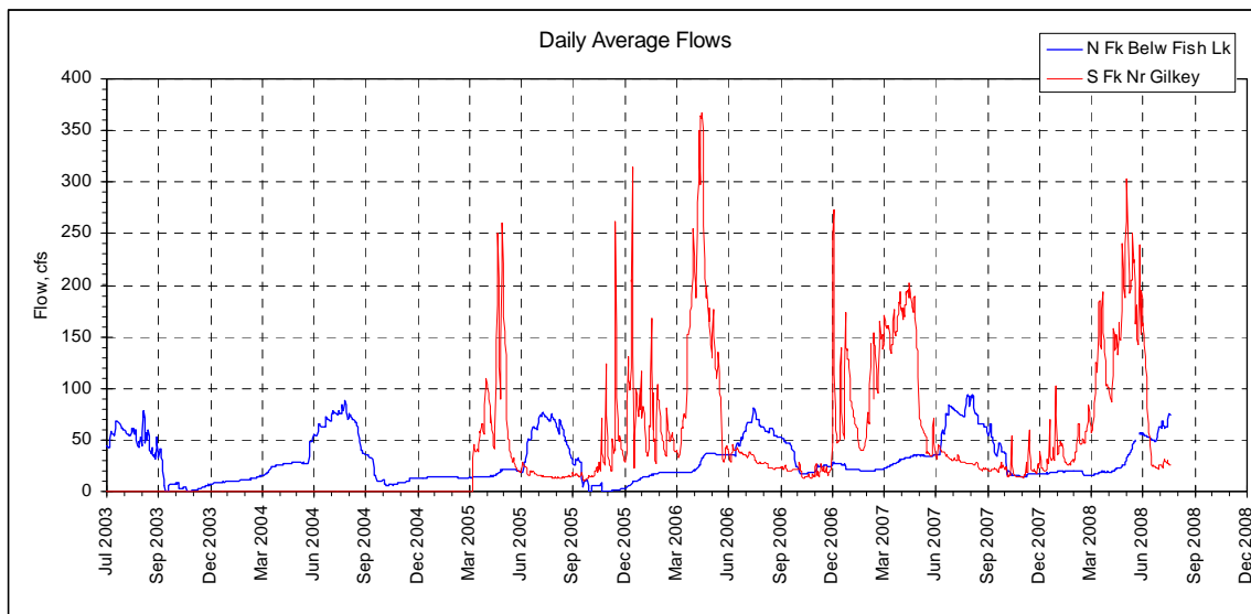
Figure 4-7 North Fork and South Fork Daily Flows.
