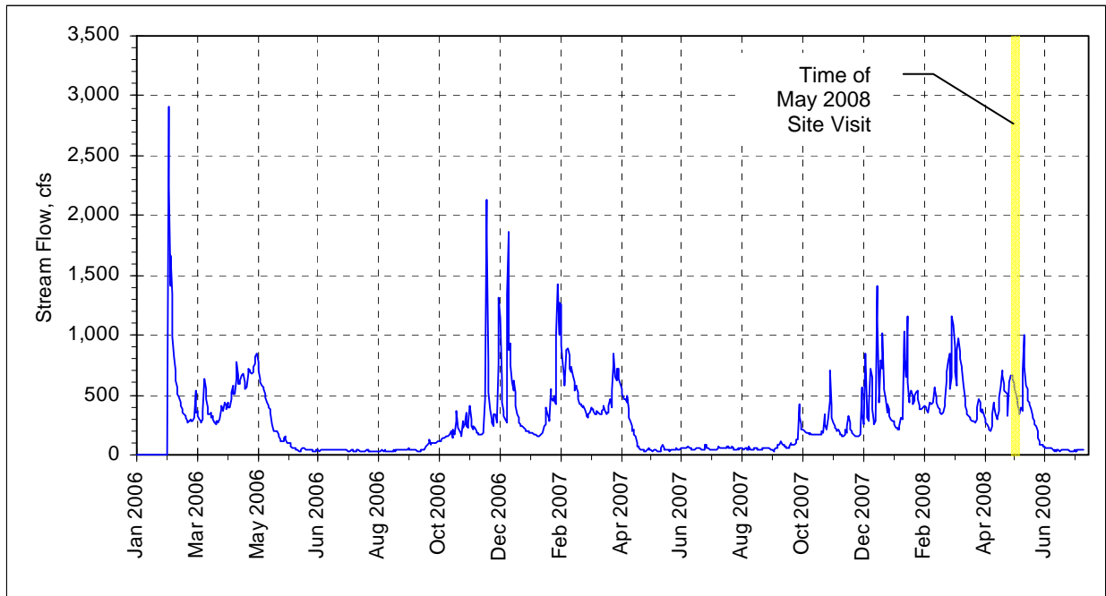
Figure 2-2 Recent Stream Flows of Little Butte Creek at Eagle Point. (USBR, 2008)
