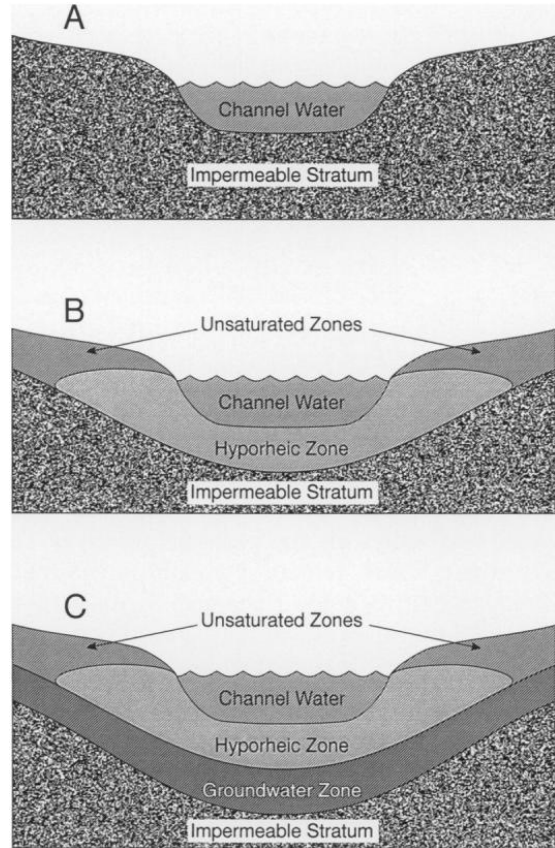
Figure 2-1 Conceptual Cross Sections Showing Surface Water-Groundwater Interaction Zones: A – No Hyporheic Zone, B – Hyporheic Zone Due Only To the Steam Flow, and C – a Hyporheic Zone Created by Both the Stream and Groundwater (White, 1993).
