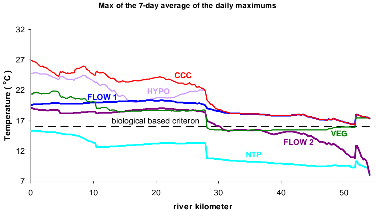
Figure 3-2 Comparison of Results for Various Temperature Scenario Simulations; Note Comparison of the Current Conditions (“CCC”) Shown as a Red Line Versus the Hyporheic Conditions (“Hypo”) Shown in Lavender. Other ODEQ Modeling Scenarios are Shown for Reference Only and Do Not Pertain Directly to the Hyporheic Flow Scenario.
