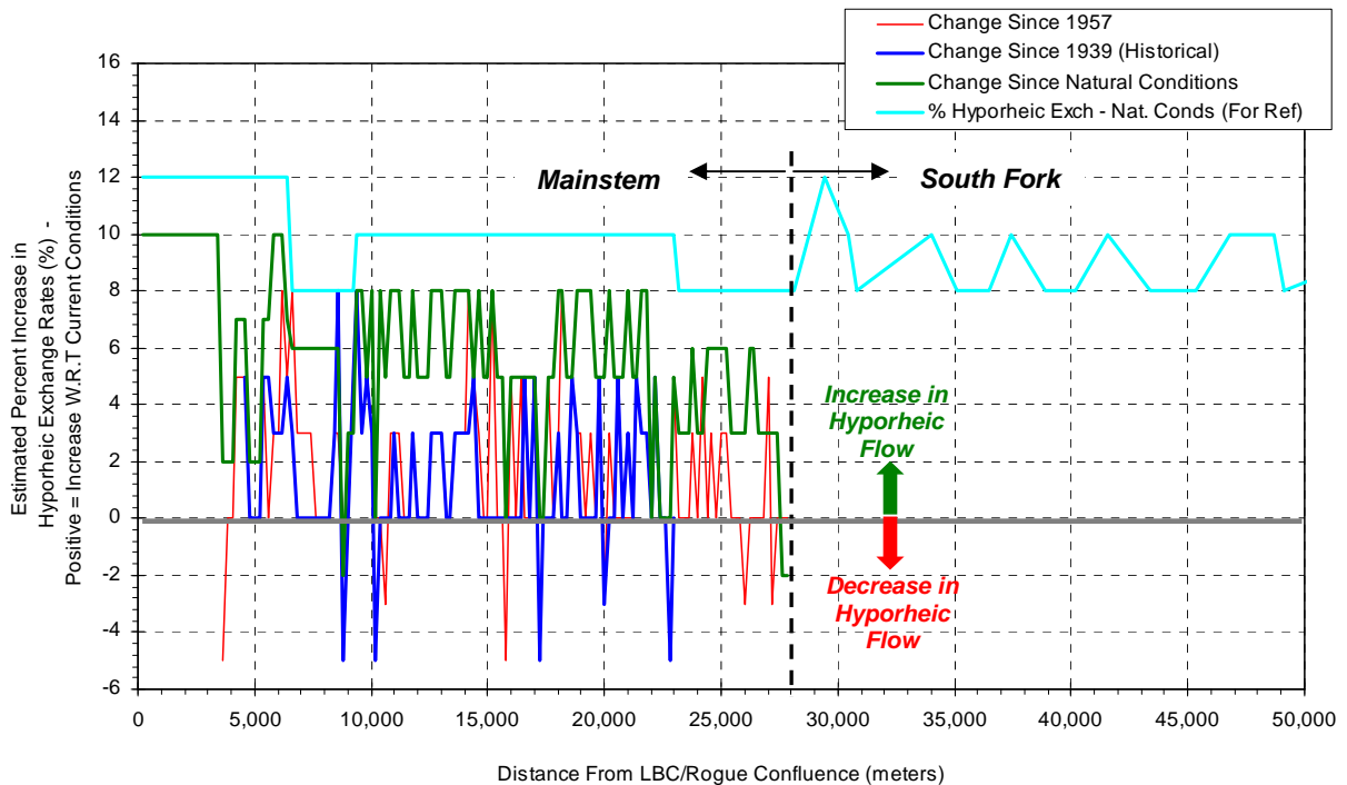
Figure 3-1 Estimated Percent Changes in Hyporheic Flow Exchange in Little Butte Creek (Mainstem and South Fork).
