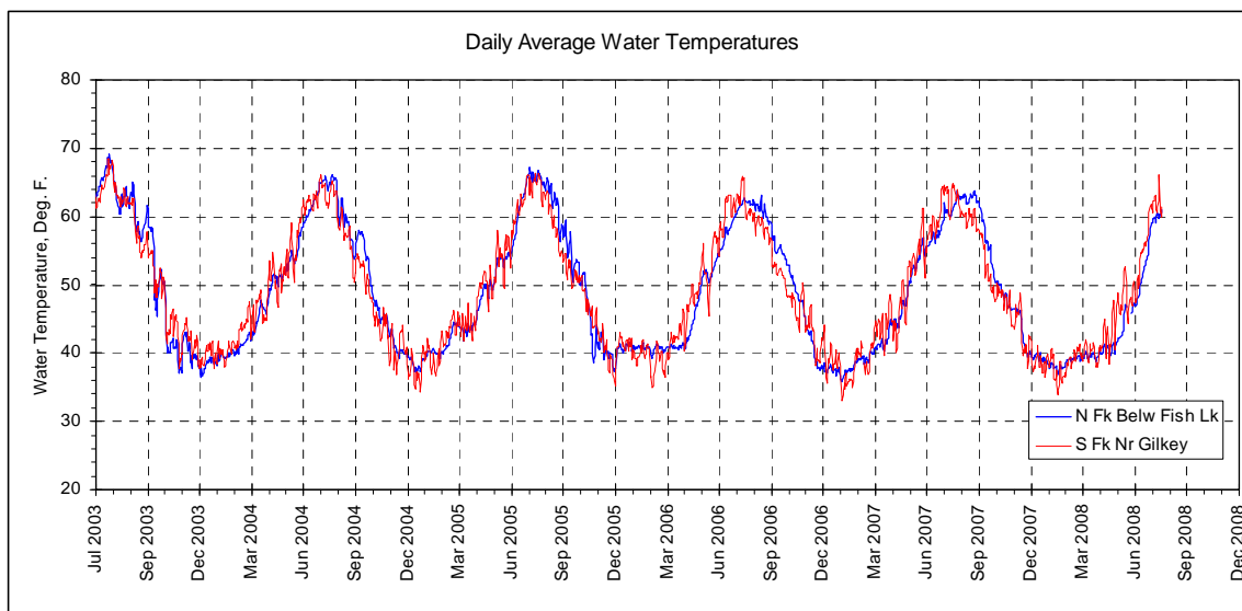
Figure 4-5 North Fork and South Fork Daily Average Water Temperatures.
