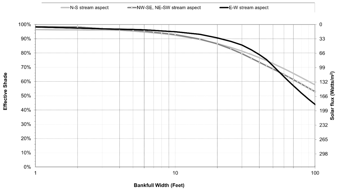
Figure 9-7: Generalized curve G with vegetation height 94 ft. and 85% density for head and shade. Heat loads represent summer daily average.
