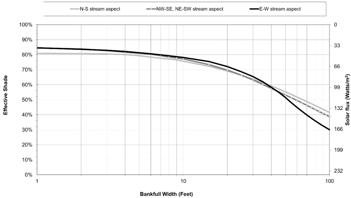
Figure 9-8: Generalized curve H with vegetation height 98 ft. and 53% density for head and shade. Heat loads represent summer daily average.
