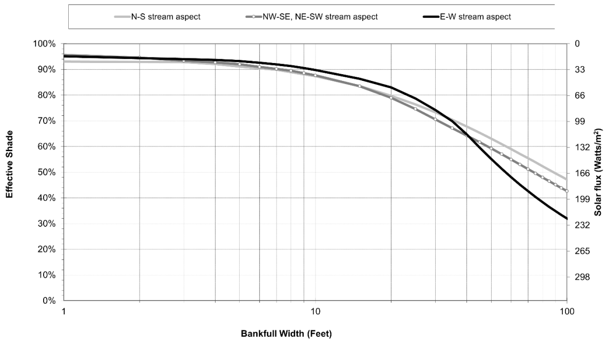
Figure 9-5: Generalized curve E with vegetation height 77 ft. and 80% density for head and shade. Heat loads represent summer daily average.
