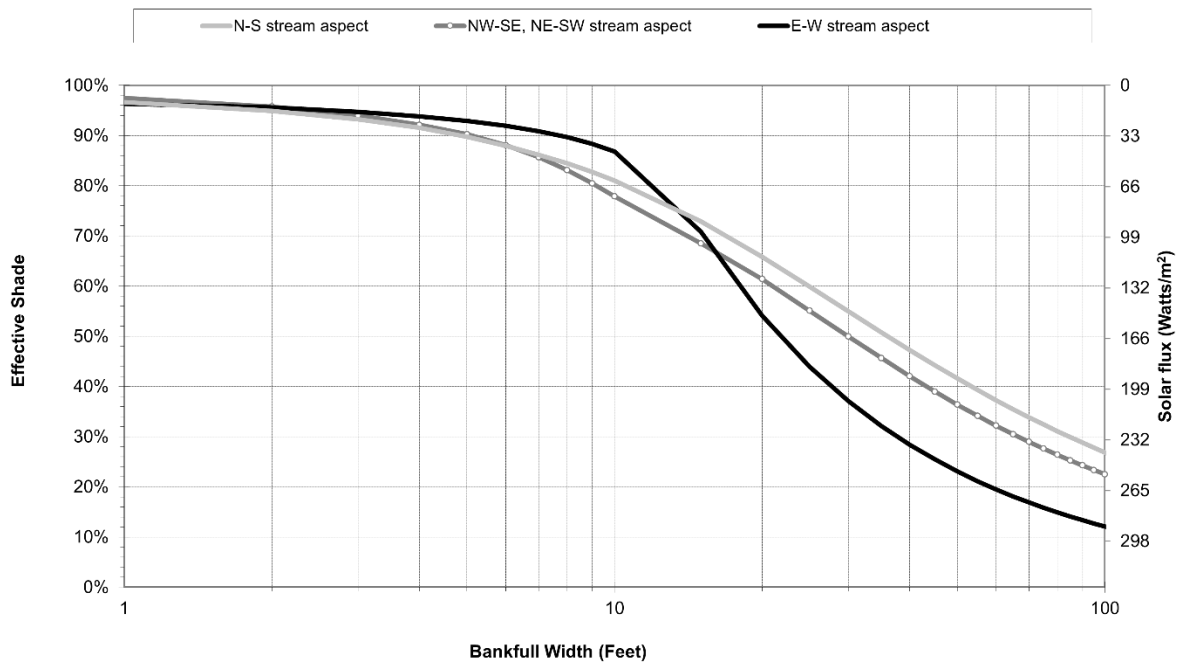
Figure 9-3: Generalized curve C with vegetation height 28 ft. and 90% density for head and shade. Heat loads represent summer daily average.
