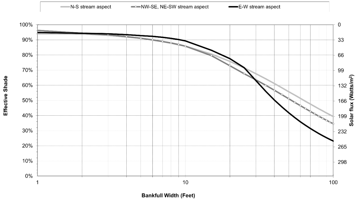
Figure 9-4: Generalized curve D with vegetation height 53 ft. and 85% density for head and shade. Heat loads represent summer daily average.
