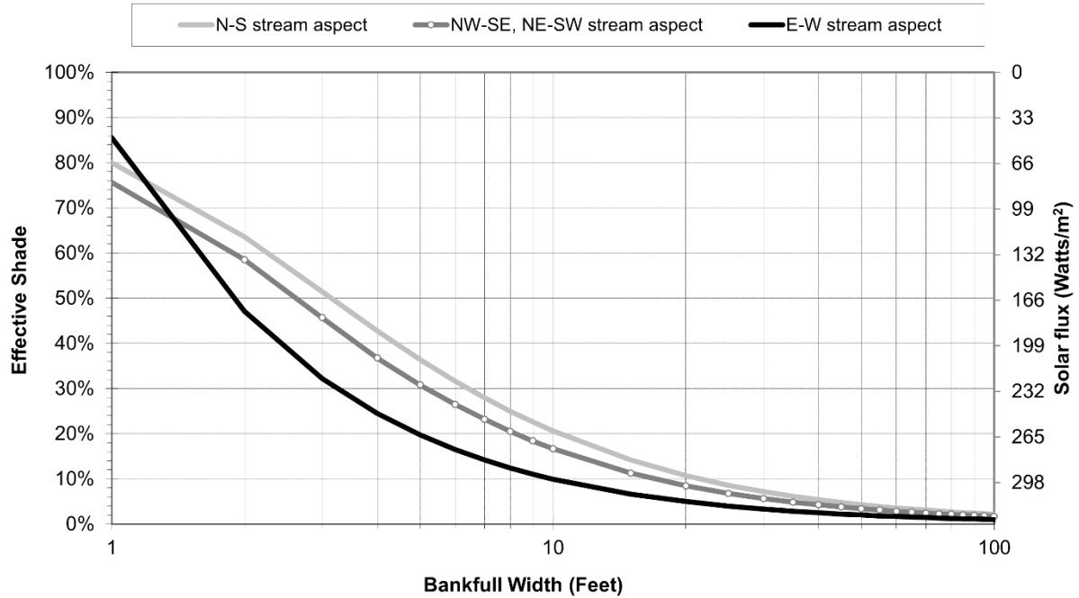
Figure 9-1: Generalized curve A with vegetation height 2 ft. and 90% density for heat and shade. Heat loads represent summer daily average.
