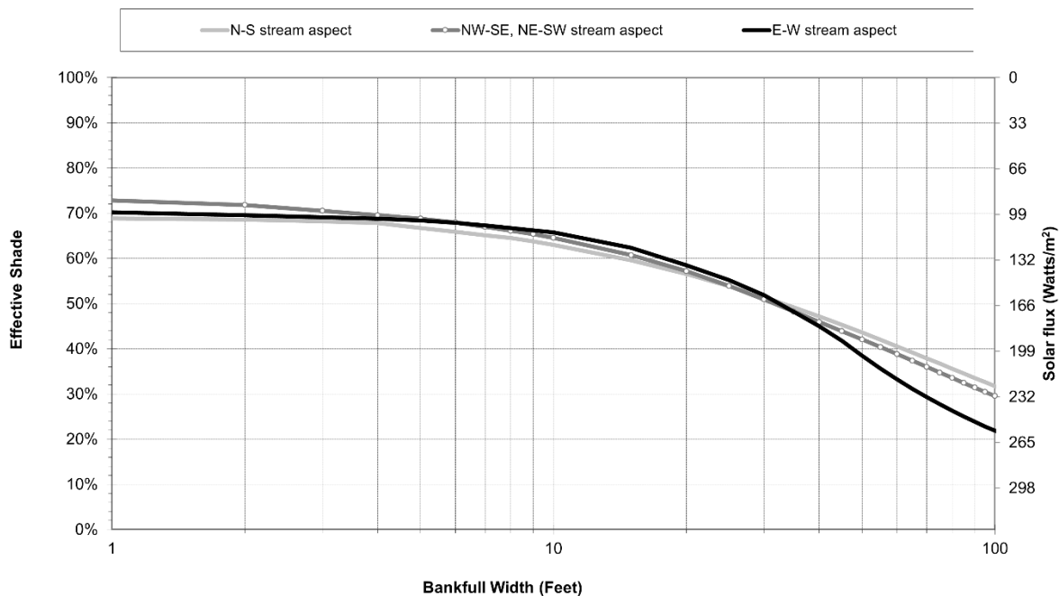
Figure 9-9: Generalized curve I with vegetation height 90 ft. and 43% density for head and shade. Heat loads represent summer daily average.
