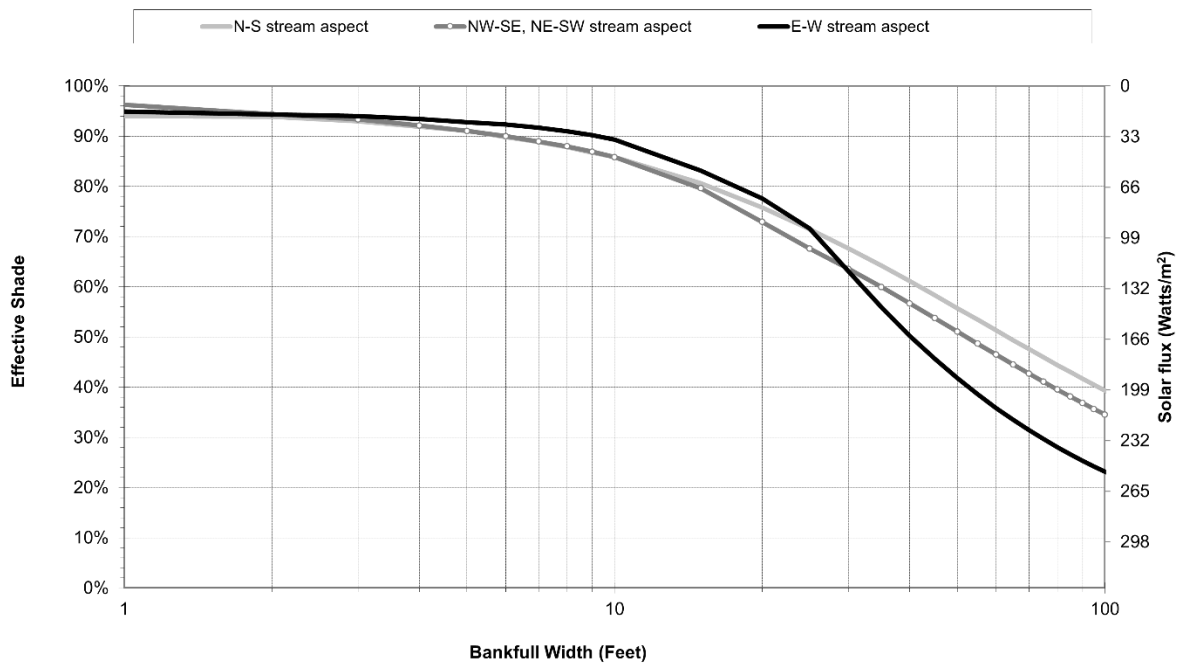
Figure 9-4: Generalized curve D with vegetation height 53 ft. and 85% density for head and shade. Heat loads represent summer daily average.
