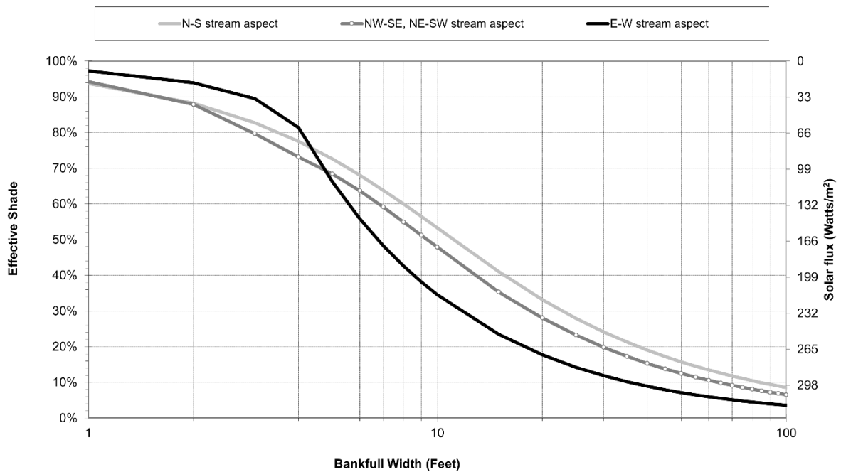
Figure 9-2: Generalized curve B with vegetation height 8 ft. and 85% density for head and shade. Heat loads represent summer daily average.
