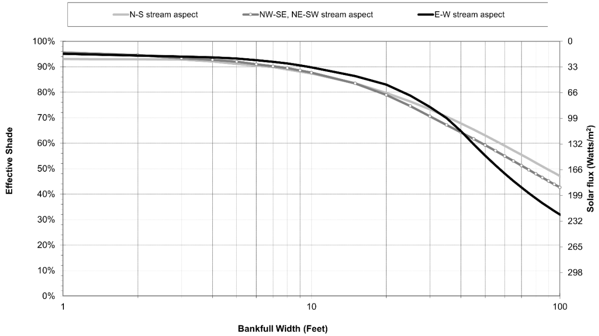
Figure 9-5: Generalized curve E with vegetation height 77 ft. and 80% density for head and shade. Heat loads represent summer daily average.
