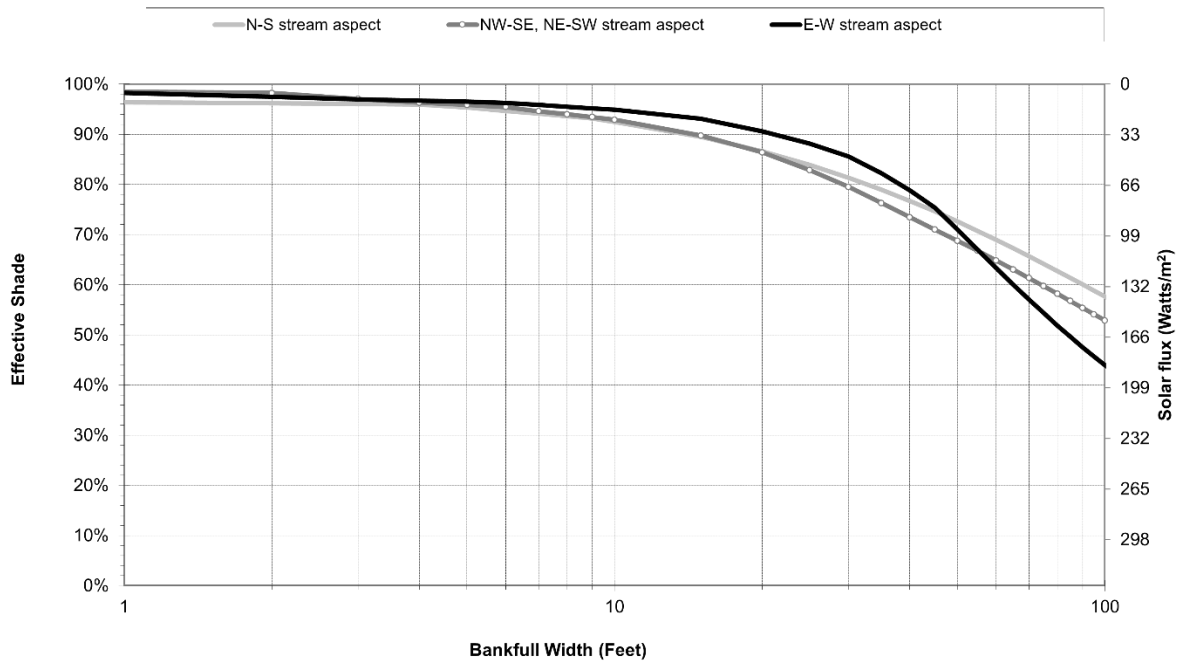
Figure 9-7: Generalized curve G with vegetation height 94 ft. and 85% density for head and shade. Heat loads represent summer daily average.
