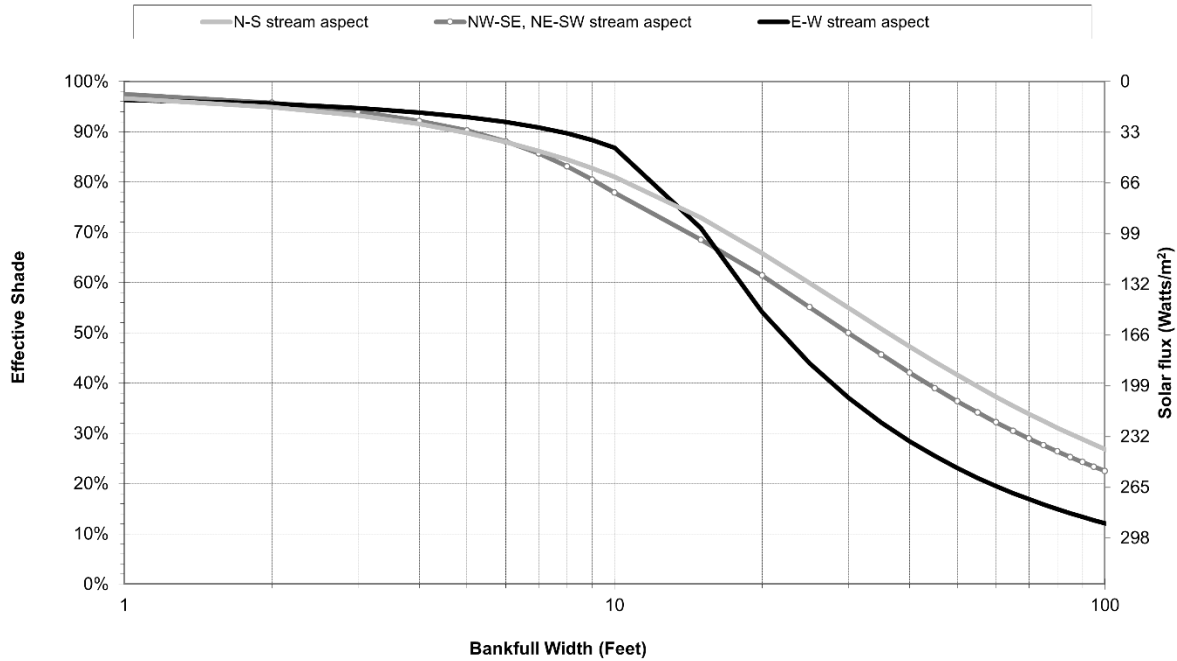
Figure 9-3: Generalized curve C with vegetation height 28 ft. and 90% density for head and shade. Heat loads represent summer daily average.
