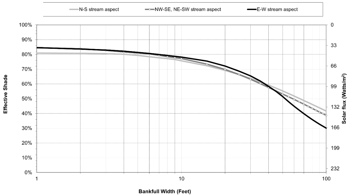
Figure 9-8: Generalized curve H with vegetation height 98 ft. and 53% density for head and shade. Heat loads represent summer daily average.
