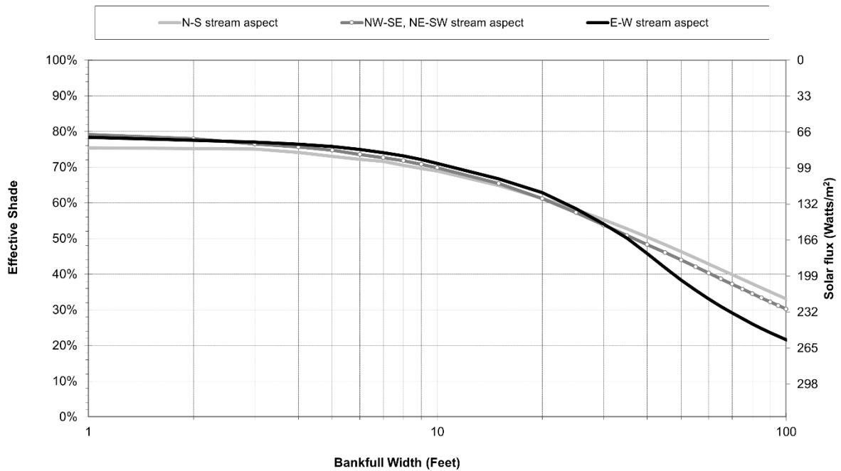
Figure 9-6: Generalized curve F with vegetation height 77 ft. and 53% density for head and shade. Heat loads represent summer daily average.
