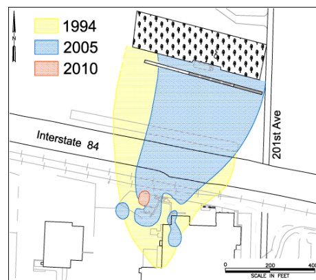
1996 to 2010 TGA Plume Shrinkage
