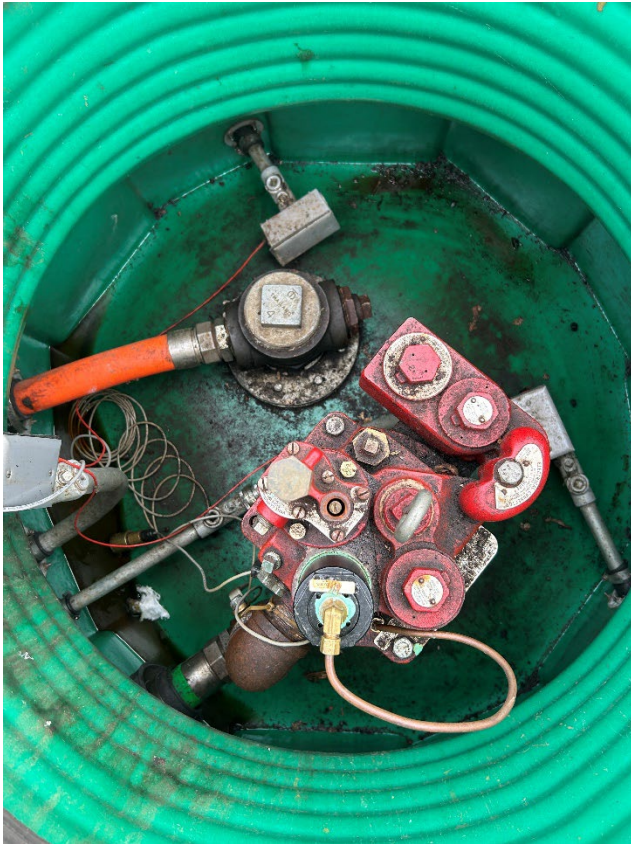
9: Diesel sump #1 with turbine
