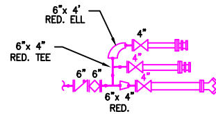
DETAIL 1 FOAM INJECTION ● PRODUCT MANIFOLD
