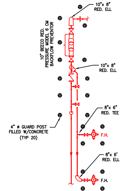
DETAIL 3 BACK-FLOW PREVENTOR
