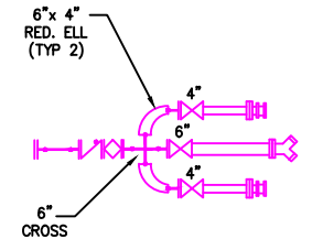
DETAIL 2 FOAM INJECTION ● PRODUCT MANIFOLD
