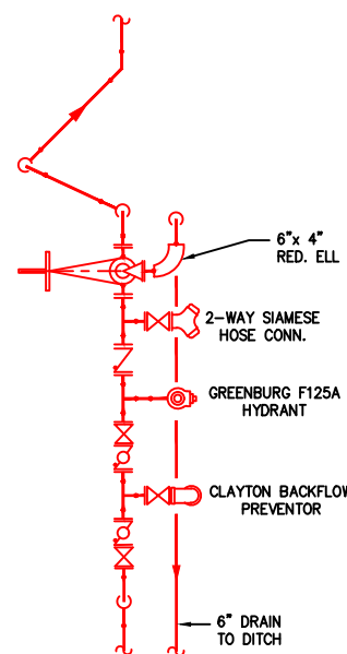
DETAIL 4 VALVE MANIFOLD
