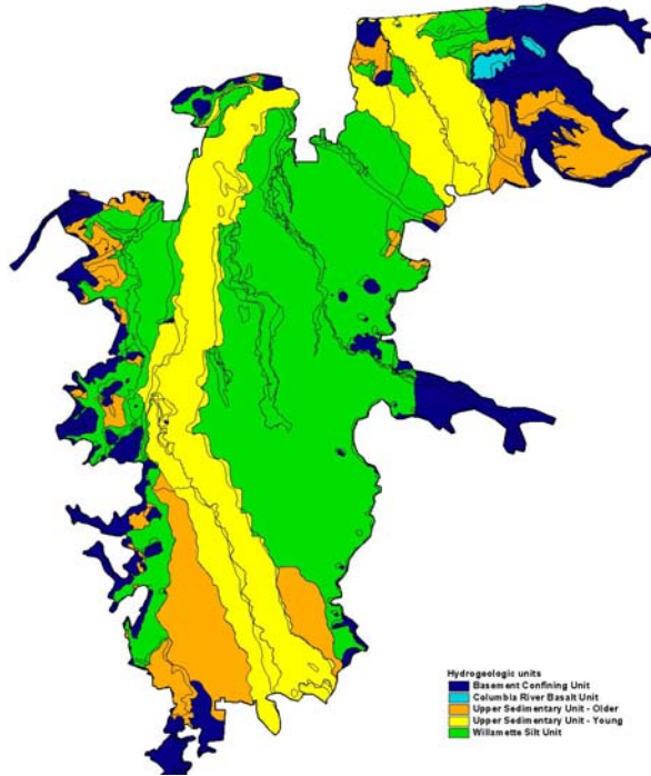
Figure 4: Hydrogeologic Units
