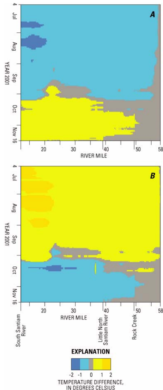
Figure 17. Difference in temperature between the base model and the model with dam release flows (A) increased by 20 percent and (B) decreased by 20 percent, using the 7-day moving average of daily maximum water temperature in degrees Celsius. The gray color zone includes all temperature differences within 0.05^{\circ}\text{C} of 0^{\circ}\text{C} .
