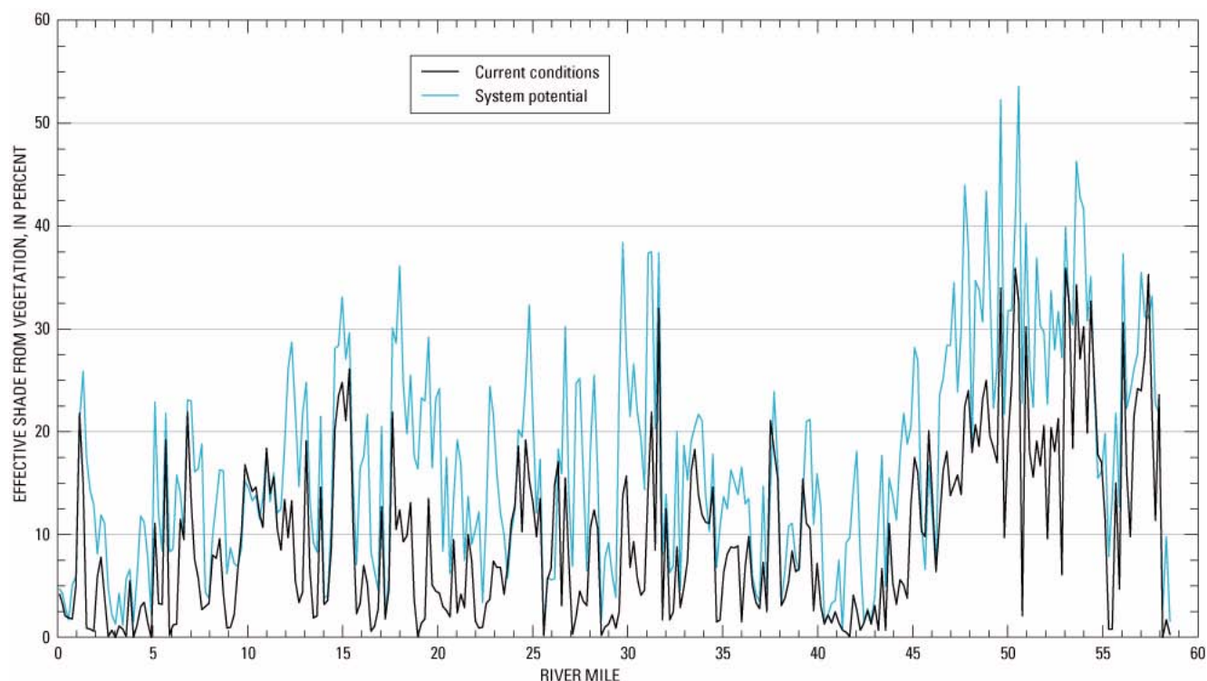
Figure 6. Vegetative shading for current conditions and system potential on August 1, 2001, for the North Santiam and Santiam Rivers. Shading is calculated as the percentage of the solar radiative flux that is blocked over the course of the entire day.
