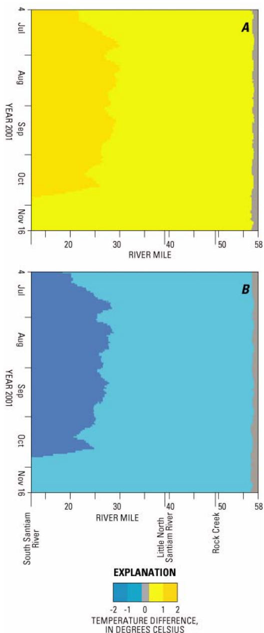
Figure 15. Difference in water temperature between the base model and the model with air temperature (A) increased by 5°C and (B) decreased by 5°C, using the 7-day moving average of daily maximum water temperature in degrees Celsius. The gray color zone includes all temperature differences within 0.05°C of 0°C.
