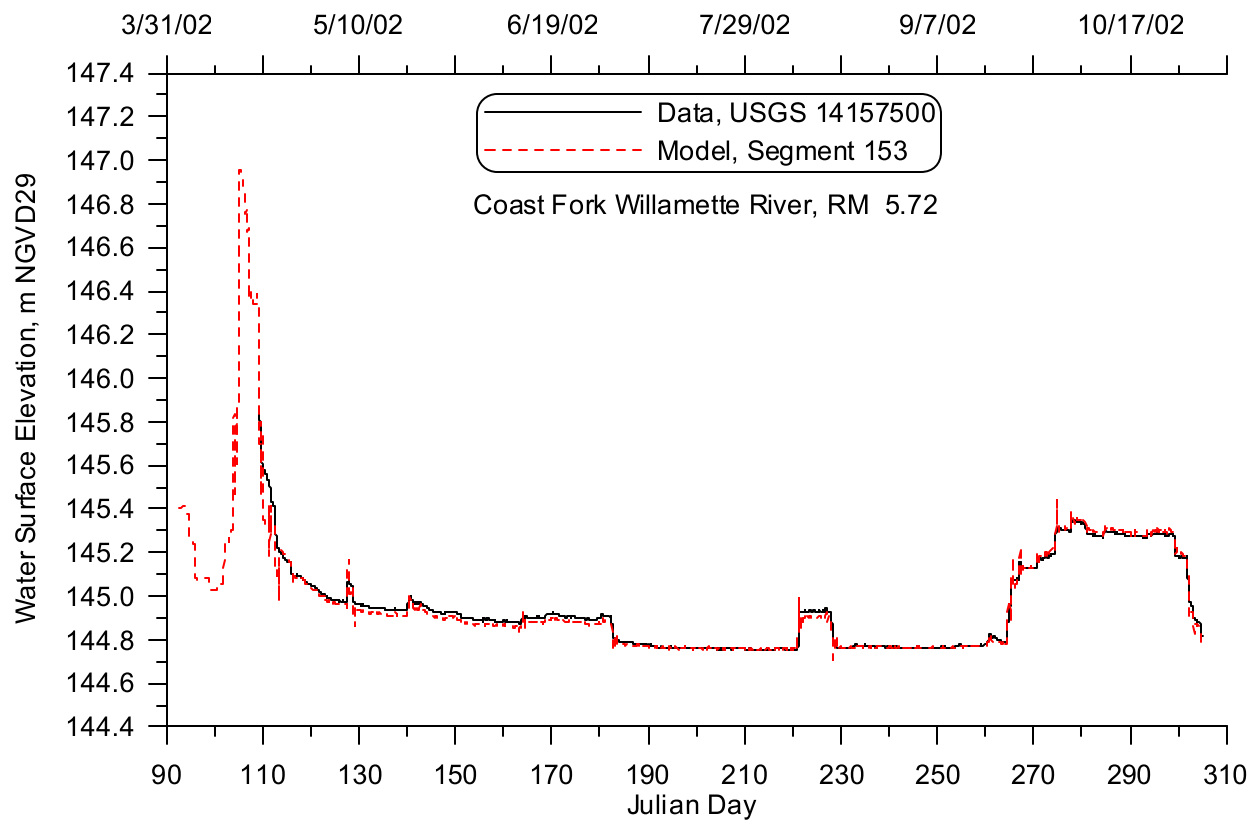
Figure 425: Coast Fork Willamette River near Goshen model-data water level comparison, 2002
