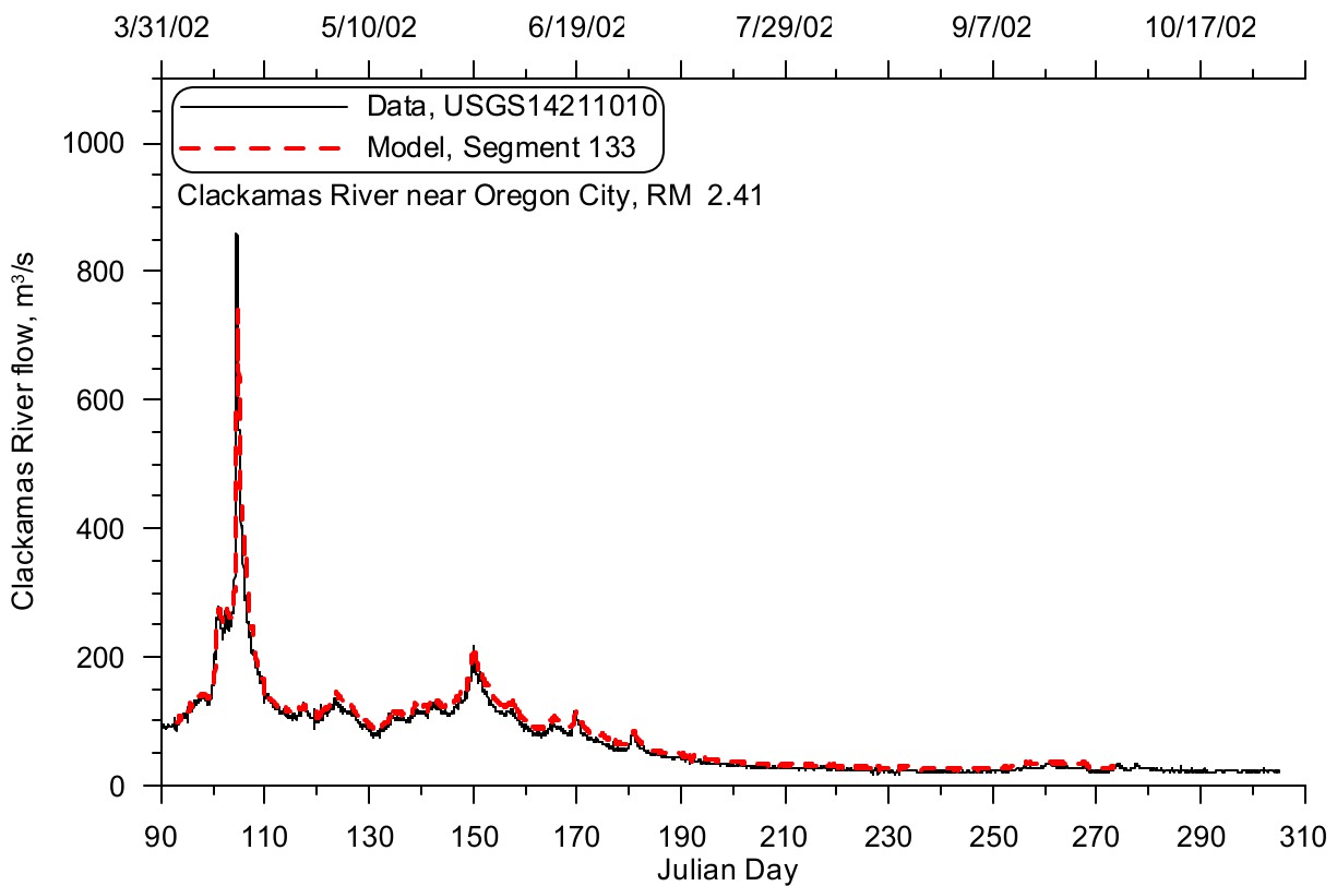
Figure 271: Clackamas River near Oregon City model-data flow comparison, 2002
