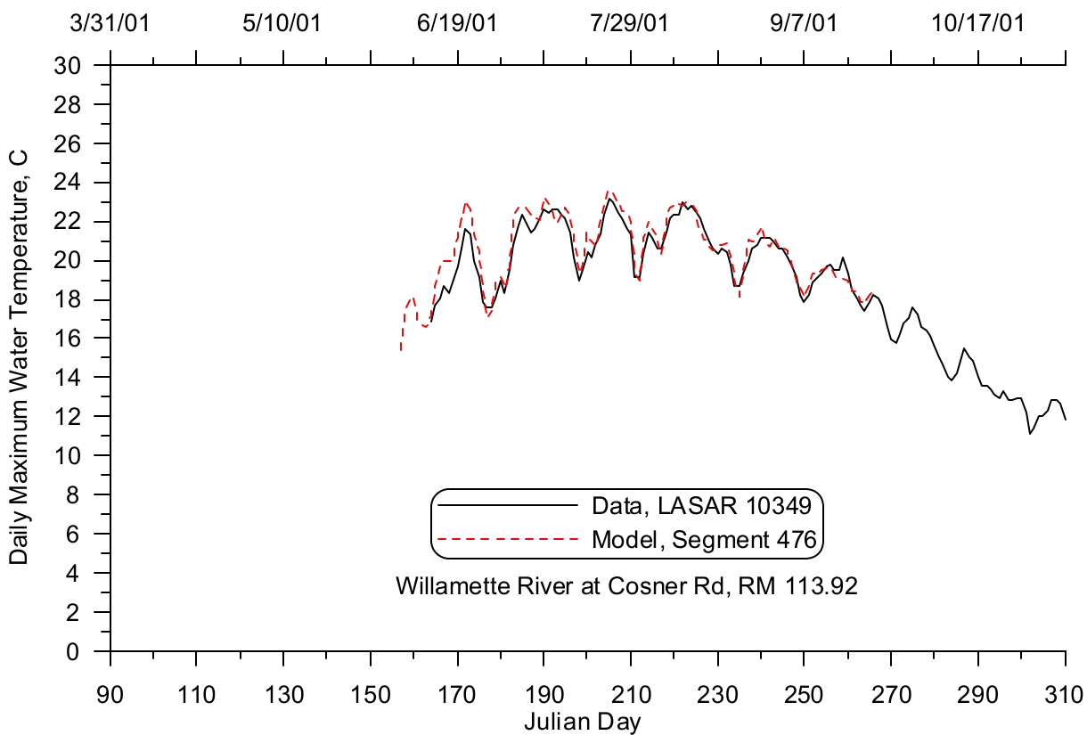
Figure 248: Upper Willamette River at Conser Rd model-data daily maximum temperature comparison, 2001
