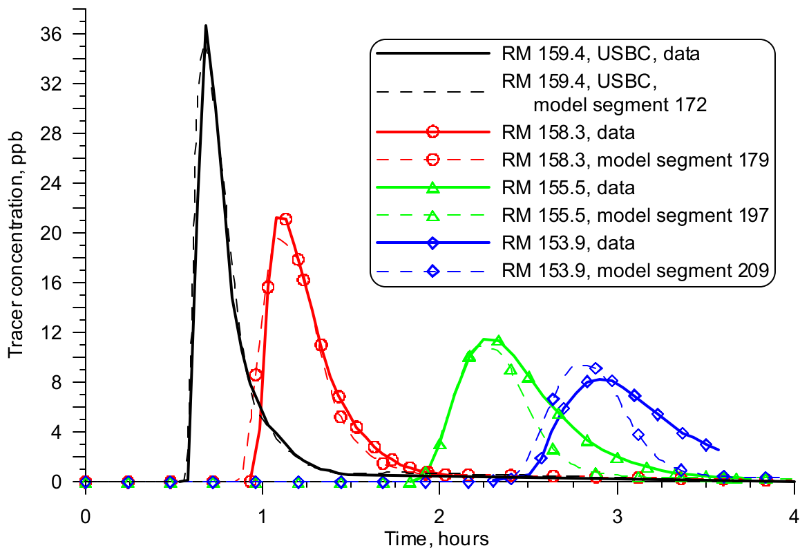
Figure 212: June 29, 1998 dye study model simulation
