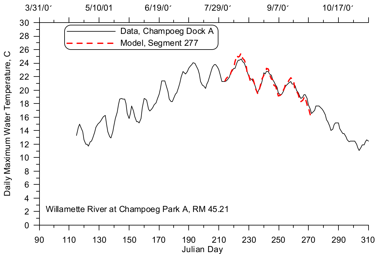
Figure 146: Willamette River at Champoege Park A model-data daily maximum temperature comparison, 2001
