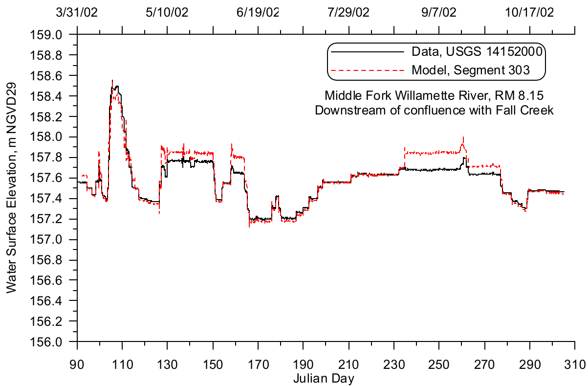
Figure 431: Middle Fork Willamette River at Jasper model-data water level comparison, 2002
