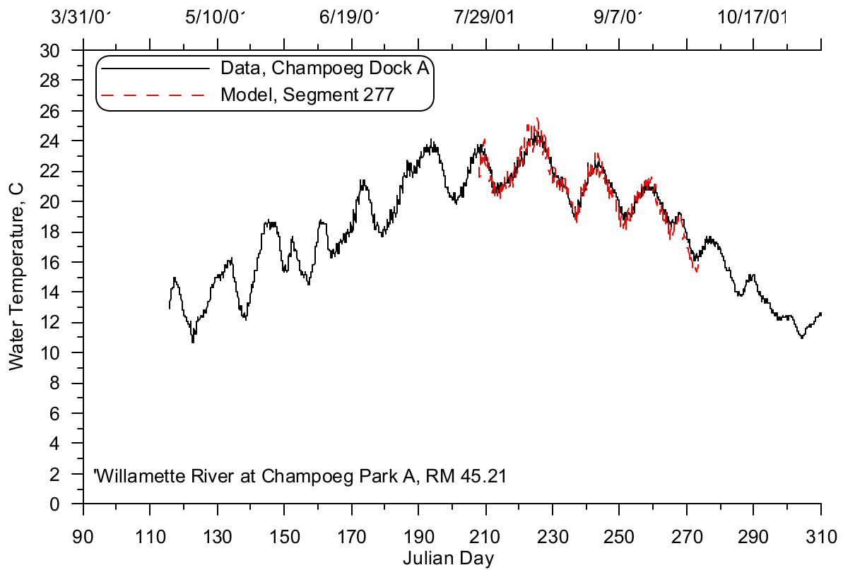
Figure 108: Willamette River at Champoege Park A model-data continuous temperature comparison, 2001
