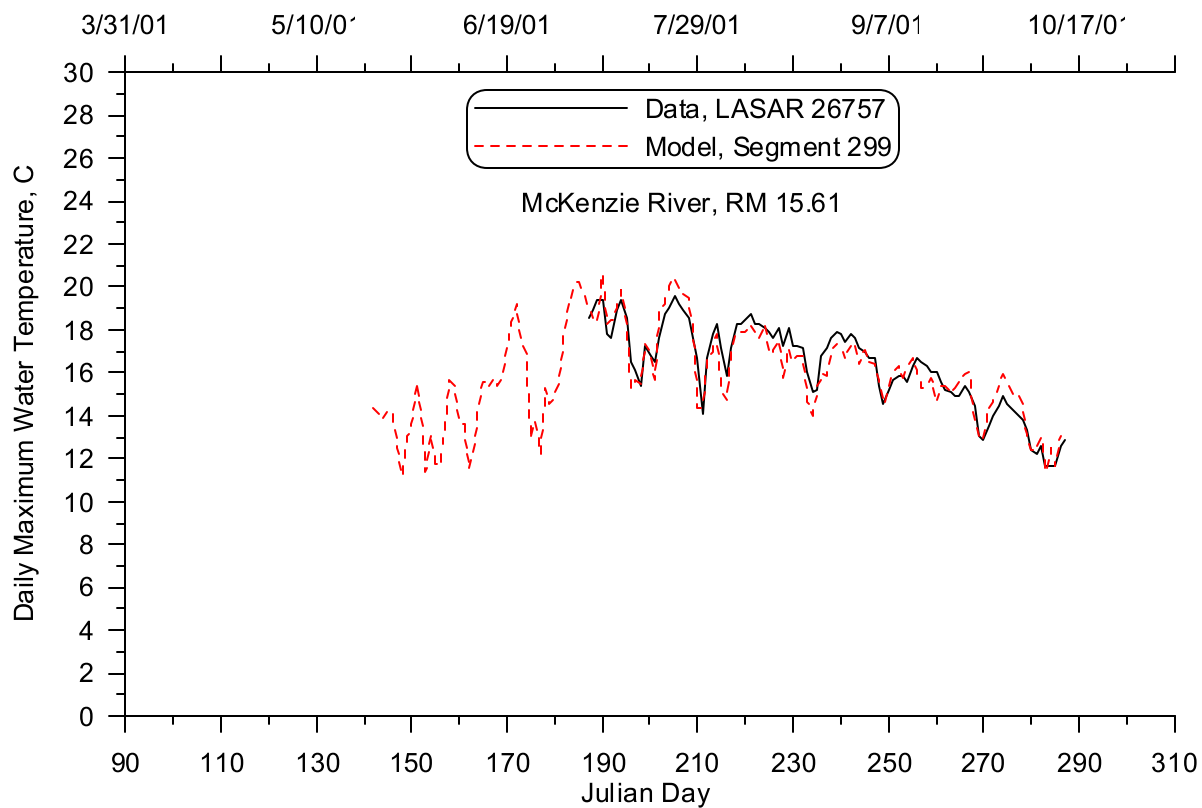
Figure 392: McKenzie River at Bellinger Landing model-data daily maximum temperature comparison, 2001
