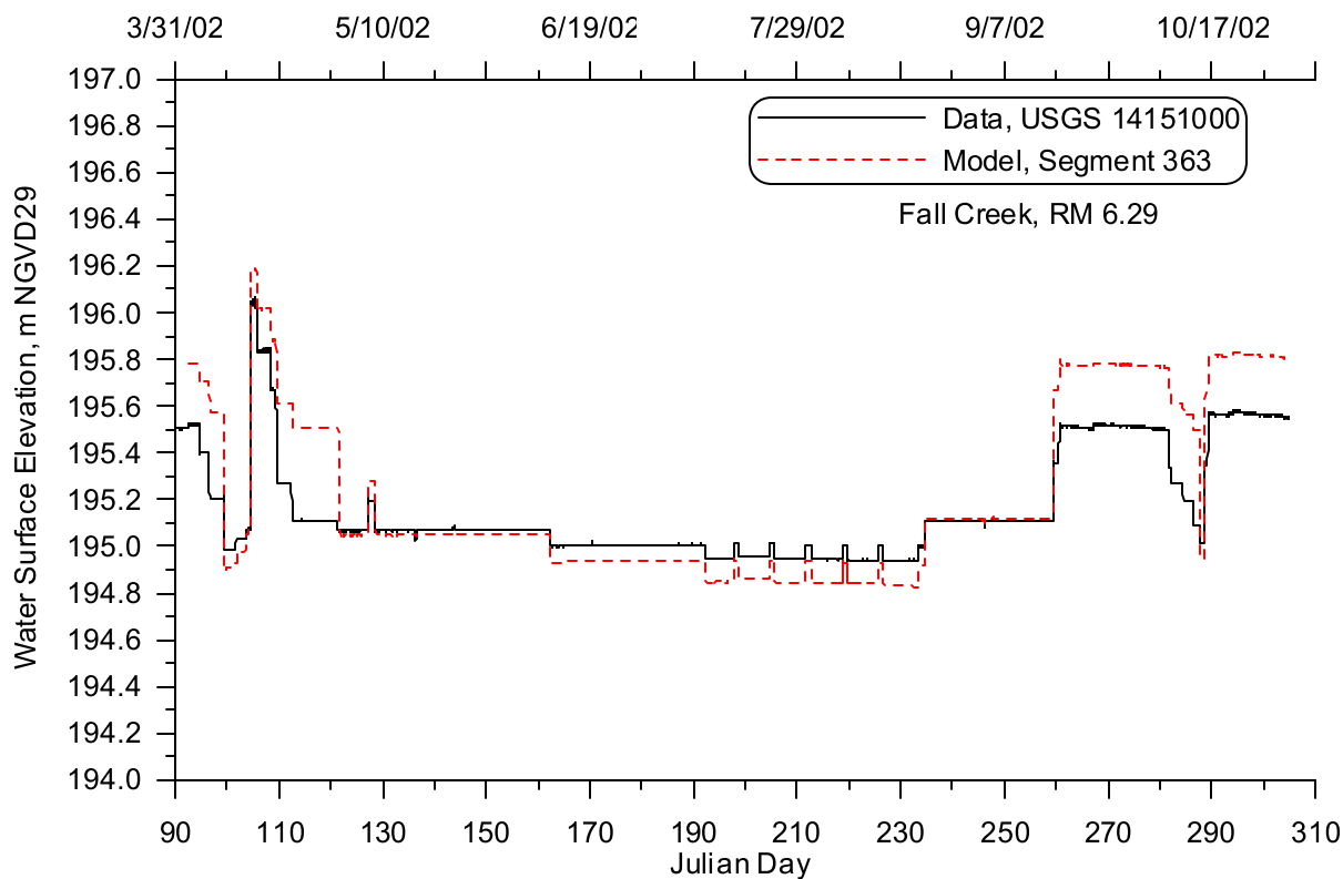
Figure 433: Fall Creek below Winberry Creek model-data water level comparison, 2002
