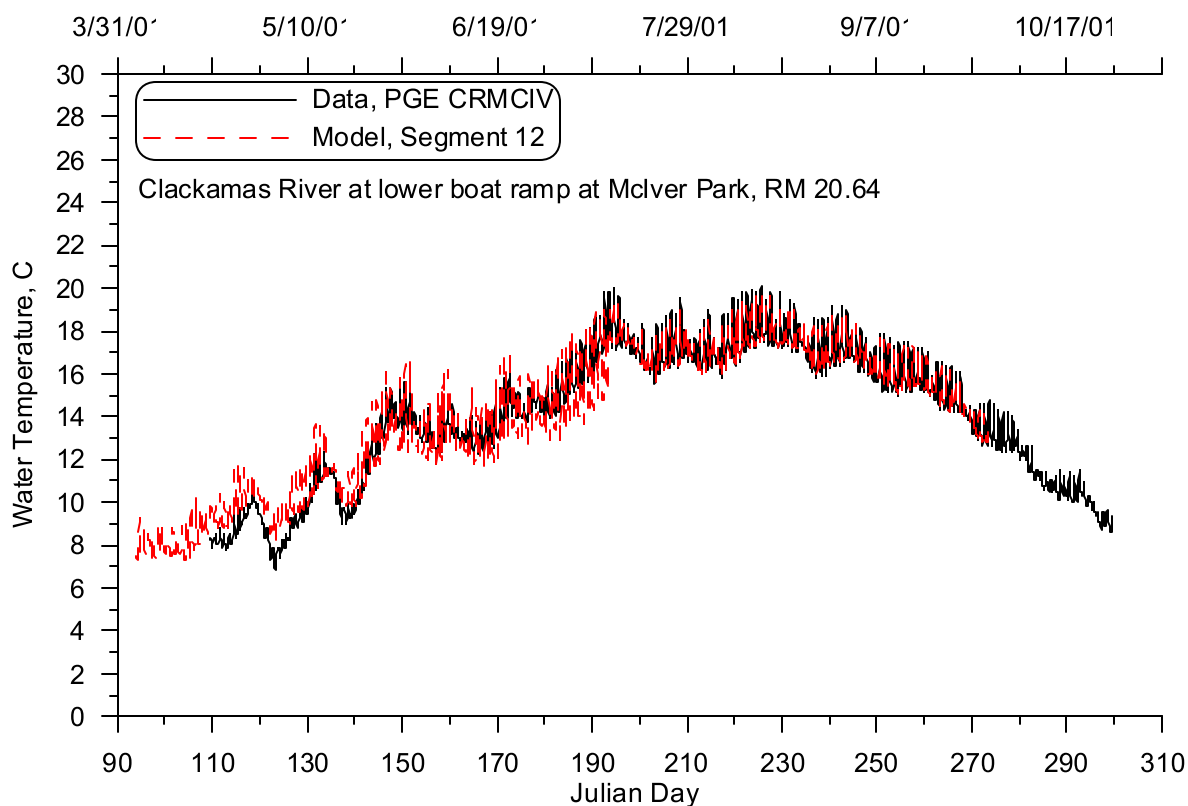
Figure 278: Clackamas River at Mclver Park model-data continuous temperature comparison, 2001
