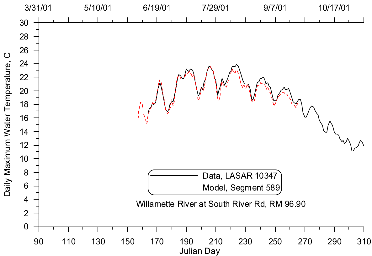
Figure 249: Upper Willamette River at South River Rd model-data daily maximum temperature comparison, 2001
