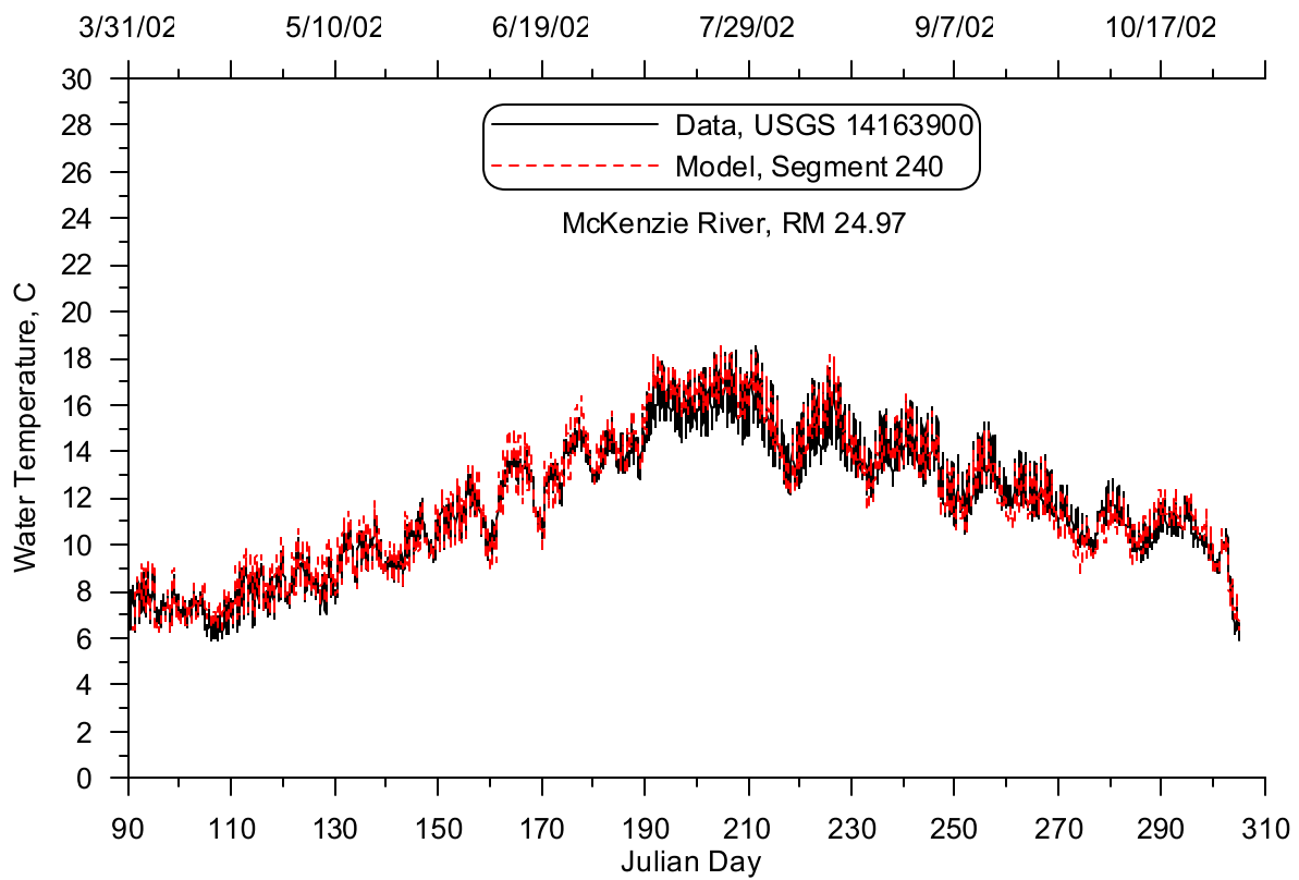
Figure 378: McKenzie River near Walterville model-data continuous temperature comparison, 2002
