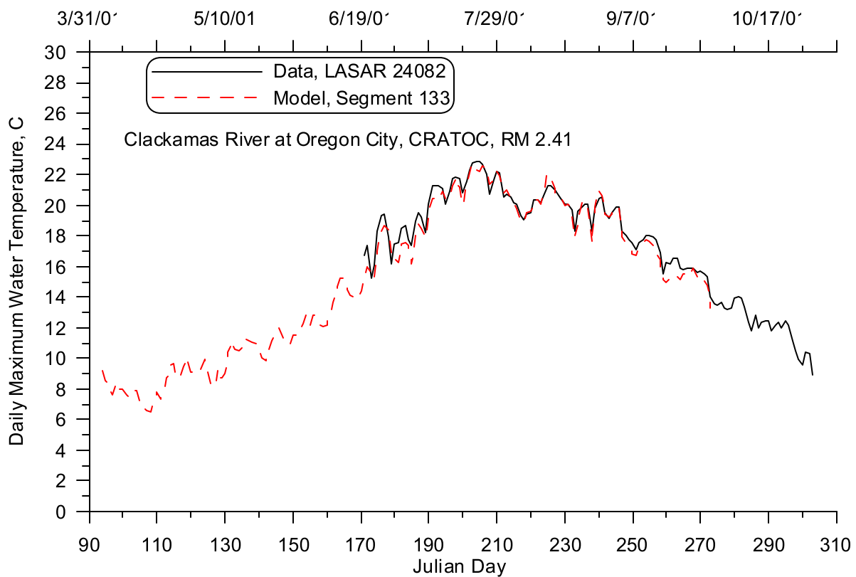
Figure 300: Clackamas River at Oregon City model-data daily maximum temperature comparison, 2002
