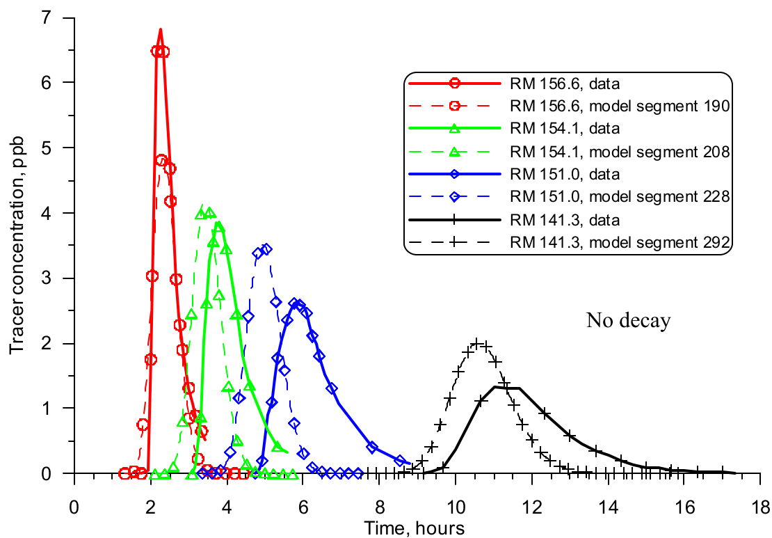
Figure 208: June 10, 1992 dye study model simulation. No decay was simulated
