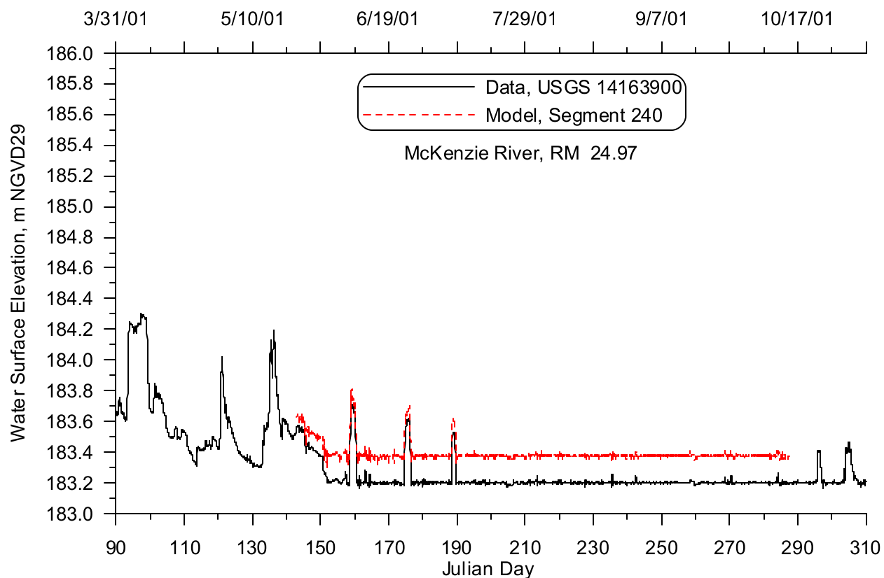
Figure 343: McKenzie River near Waltherville model-data water level comparison, 2001
