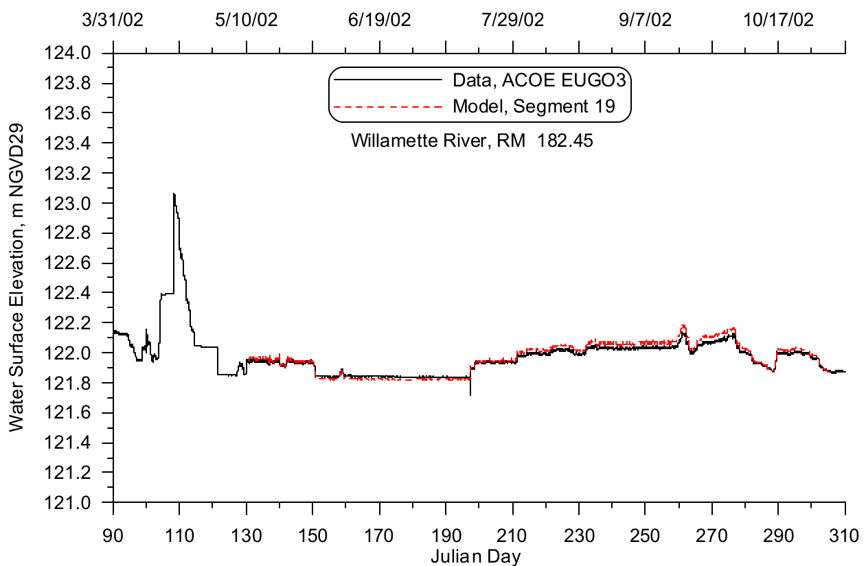
Figure 183: Willamette River at Eugene model-data water level comparison, 2002
