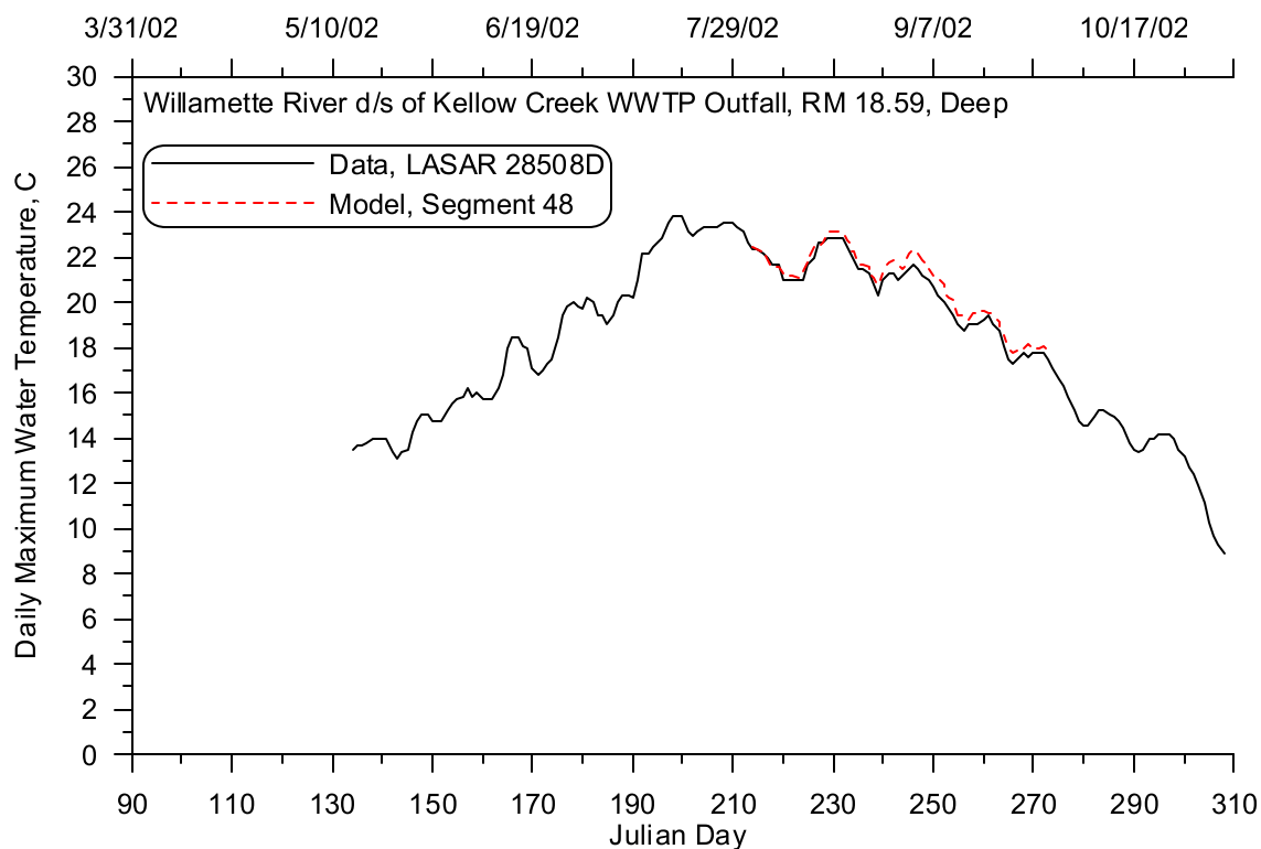
Figure 71: Willamette River downstream of Kellog Creek WWTP outfall (deep) model-data daily maximum temperature comparison, 2002
