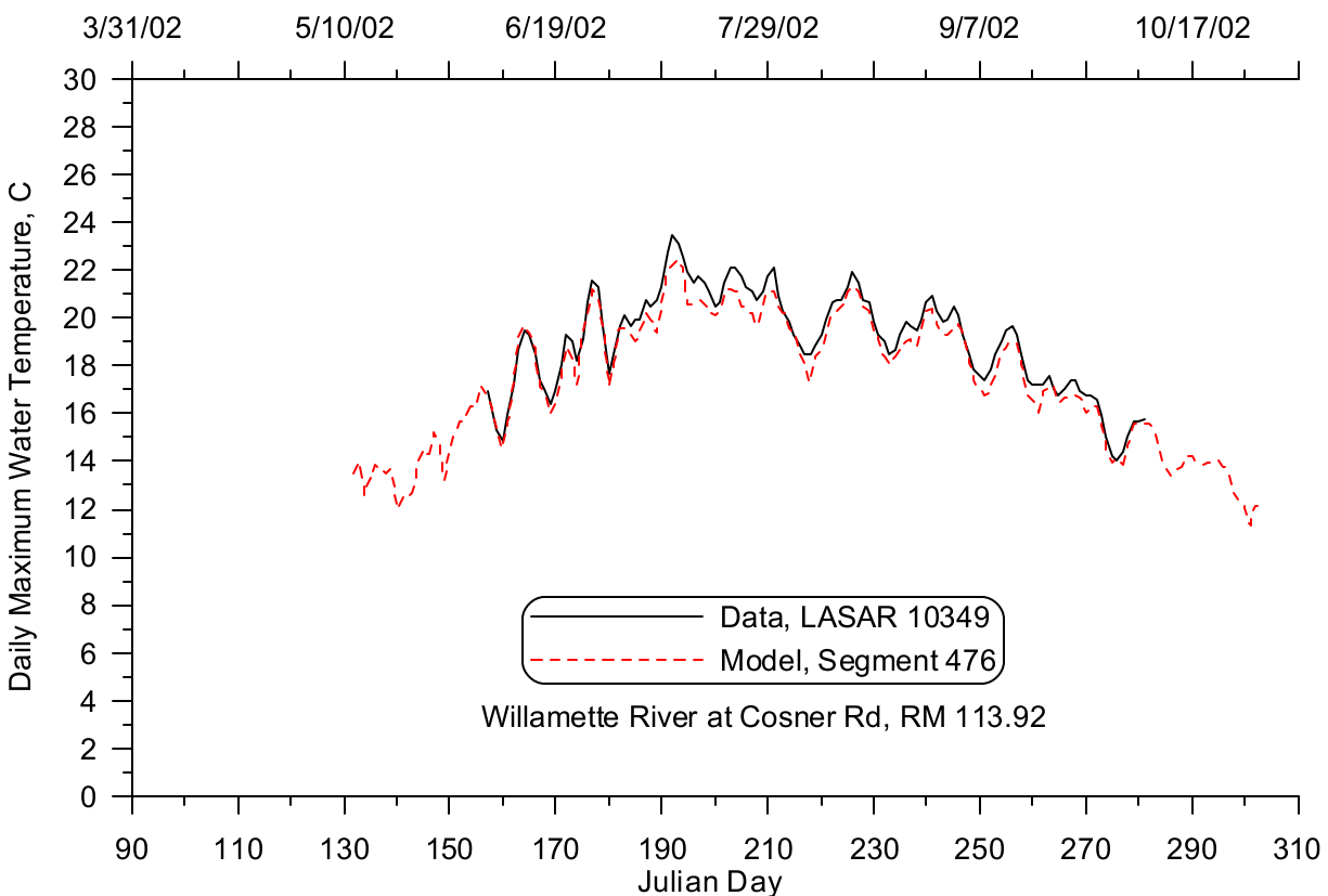
Figure 260: Upper Willamette River at Conser Rd model-data daily maximum temperature comparison, 2002
