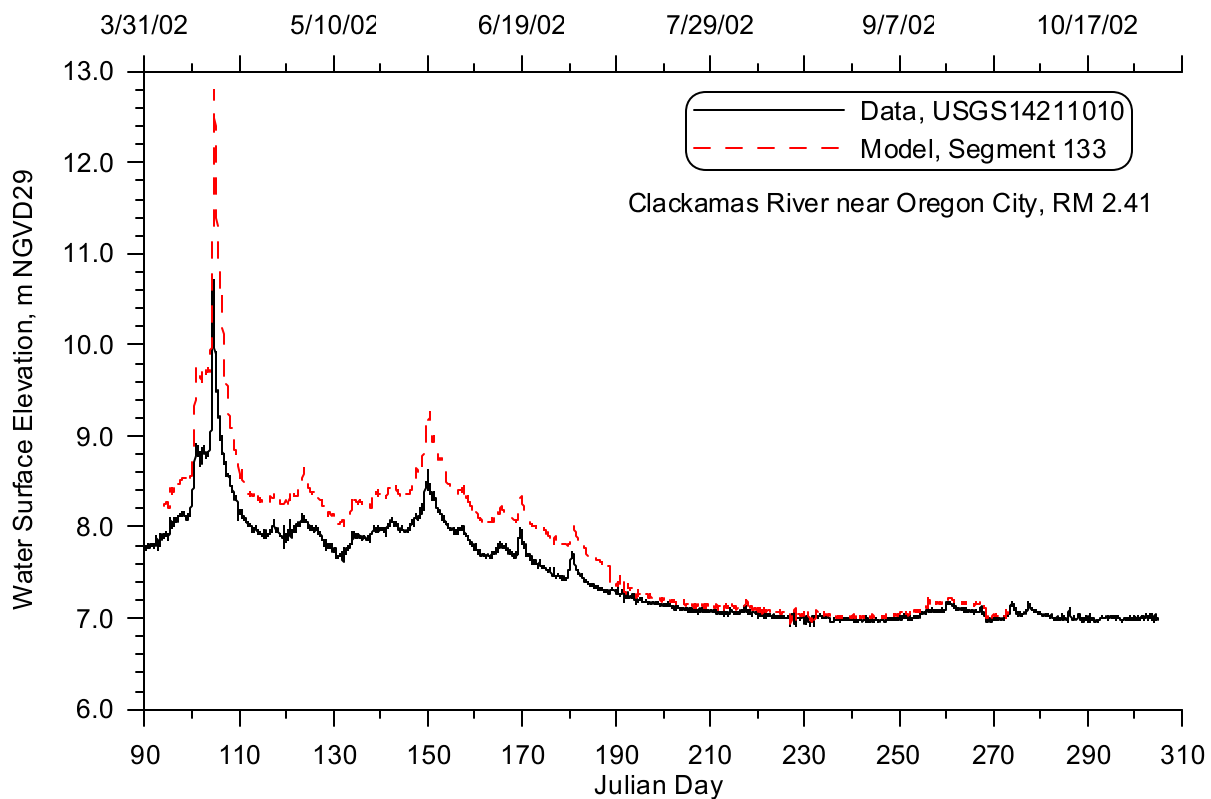
Figure 272: Clackamas River near Oregon City model-data water level comparison, 2002
