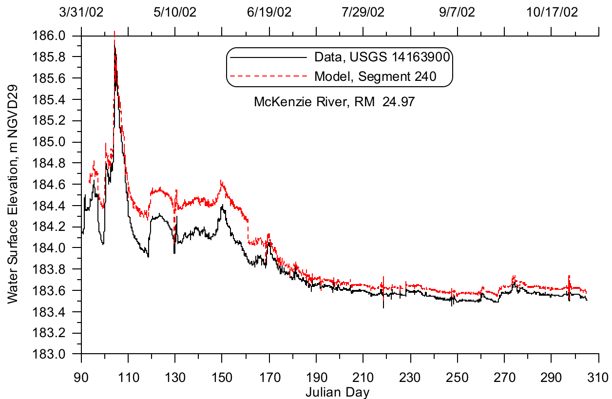
Figure 351: McKenzie River near Waltherville model-data water level comparison, 2002
