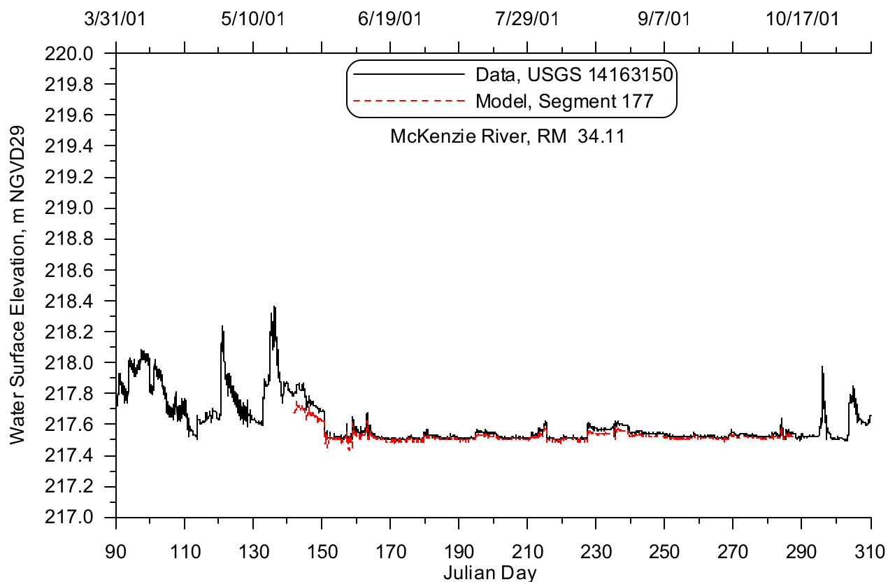
Figure 341: McKenzie River below Leaburg Dam model-data water level comparison, 2001
