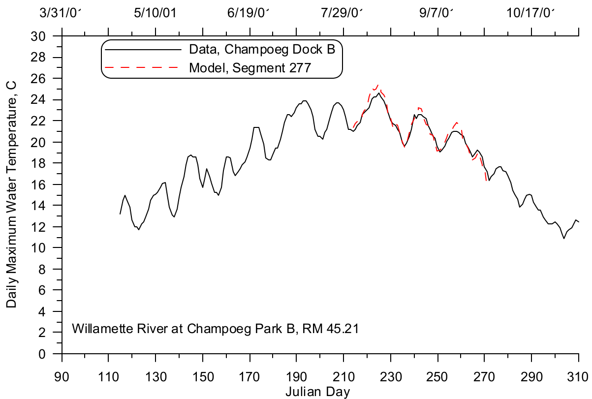
Figure 147: Willamette River at Champoege Park B model-data daily maximum temperature comparison, 2001
