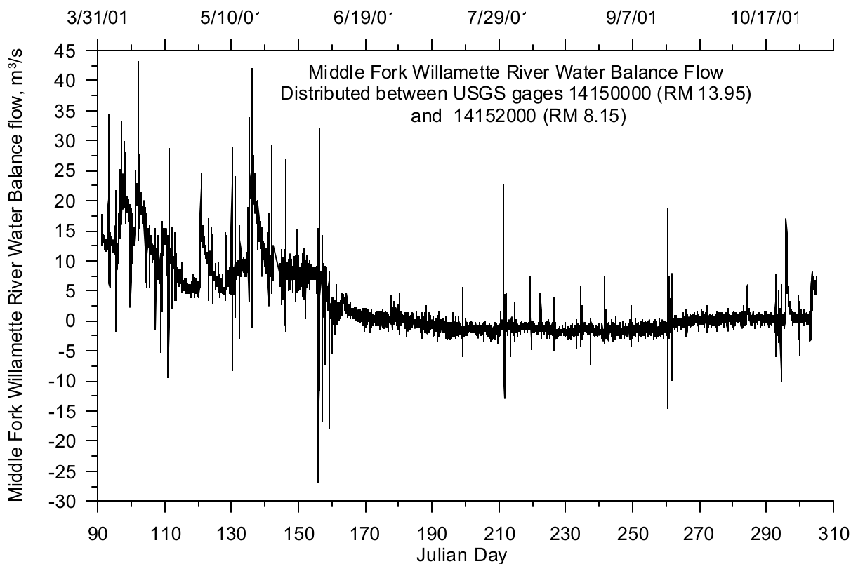
Figure 436: Middle Fork Willamette River water balance flow, 2001
