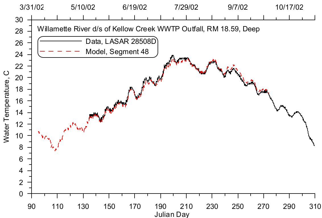
Figure 37: Willamette River downstream of Kellogg Creek WWTP outfall (deep) model-data continuous temperature comparison, 2002
