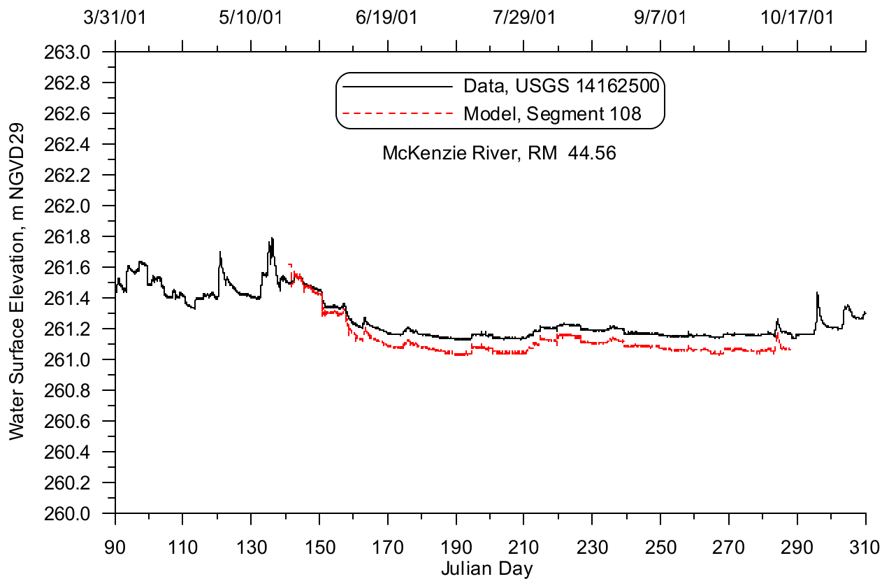
Figure 339: McKenzie River near Vida model-data water level comparison, 2001
