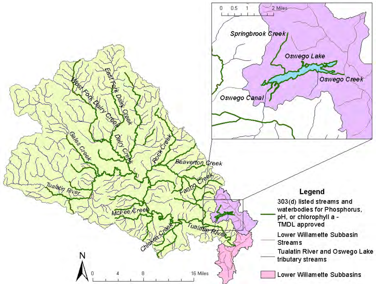
Figure 3-1. 2004/2006 303(d) List for Phosphorus, pH or Chlorophyll a (Bolded Green Lines) in the Tualatin and Oswego Lake Subbasins
