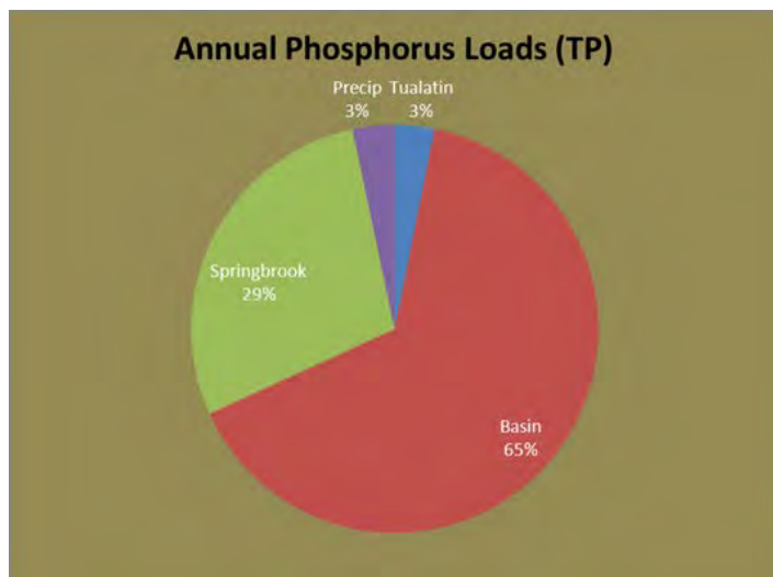
Figure 3-5. Relative source contributions of the annual phosphorus loads to Oswego Lake, which totaled 1116 kg during the 2008-2009 water year. (personal communication, Mark Rosenkranz, Lake Oswego Corporation).
