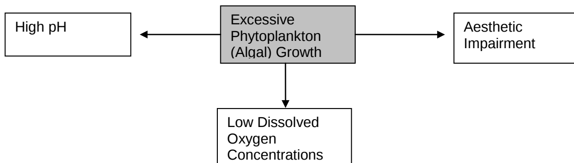
Figure 3-2. Simplified Schematic of Possible Impacts of Excessive Algal Growth
