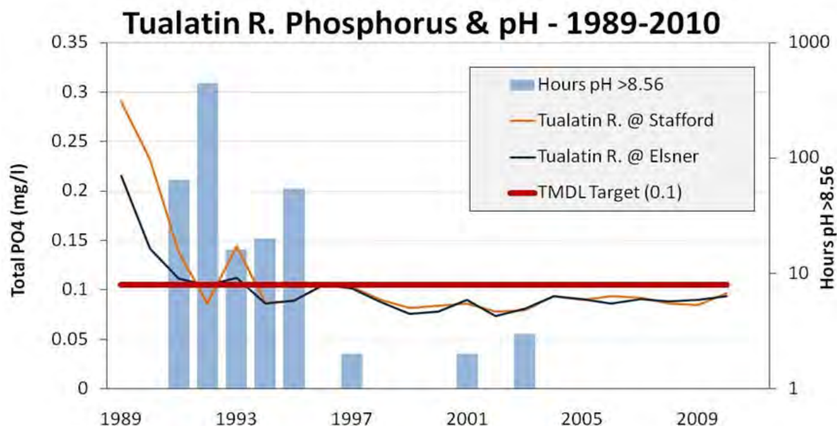
Figure 3-3. Total Phosphorus concentrations at two sites in the Lower Tualatin, juxtaposed with the number of hours of pH violations each summer at the Lake Oswego Diversion Dam. The bar graph reflects zero hours of pH violations since 2004, not missing data. The Elsner and Stafford sites are at river miles 16.5 and 5.4 respectively.
