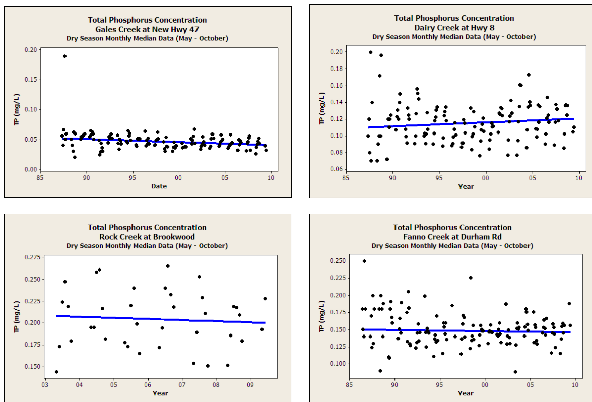
Figure 3-4. Monthly median concentrations of total Phosphorus are plotted over time at four different tributary locations in the Tualatin River Basin. The decrease in Gales Creek and increase in Dairy Creek are significant at the 95% confidence level, using the Seasonal Kendal Tau trend test. No significant trends are present at the Rock Creek and Fanno Creek sites.
