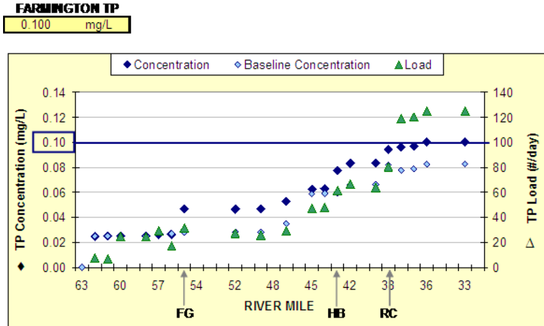
Figure 3-7. Primary TP Mass Balance Results (Median TP Concentration, May through October, 2002-2007) Assumes TP Mass Load \leq 66.1 lb/day, current flow augmentation levels, and tributaries meeting water quality standards.(See Appendix B-1, Exhibit 2-10). Baseline Total P concentration (◇ light blue diamond) reflects current river concentrations, while the Concentration (◇, dark blue diamond) and load (△ green triangle) are projected future conditions based on a future 66.1 lb./day load.
