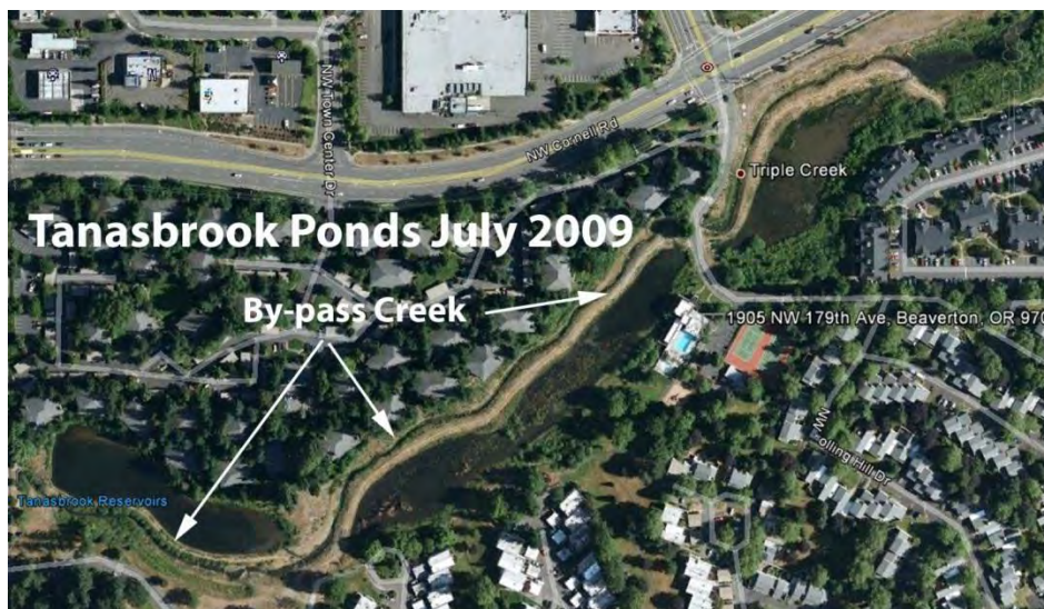
Figure 2 - Tanasbrook Ponds after CWS Bypass Project
