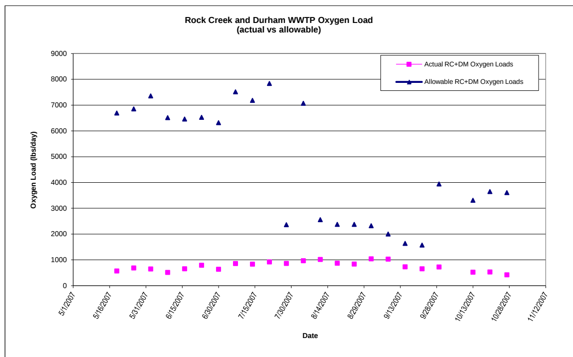
Figure 3-3. The allowable oxygen-demand and the actual oxygen demand for Clean Water Services Rock Creek and Durham Treatment Plants during the TMDL season of 2007. The Y-axis shows the pounds per day of actual and allowable (2005 Watershed Permit) oxygen-demanding substances in discharged water (CBOD + NBOD).
