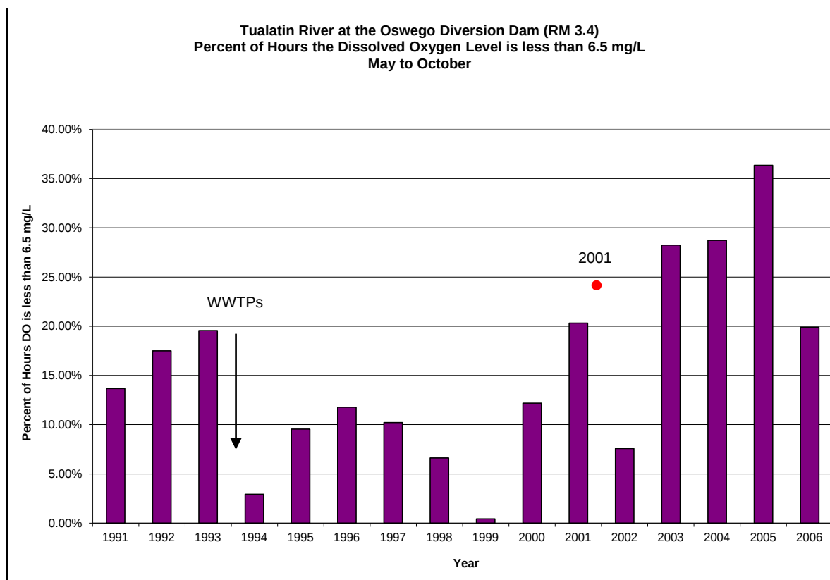
Figure 3-4. The percent of hours in each TMDL season that dissolved oxygen levels were less than 6.5 mg/L at the Oswego Dam at River Mile 3.4 in the Lower Tualatin River.
