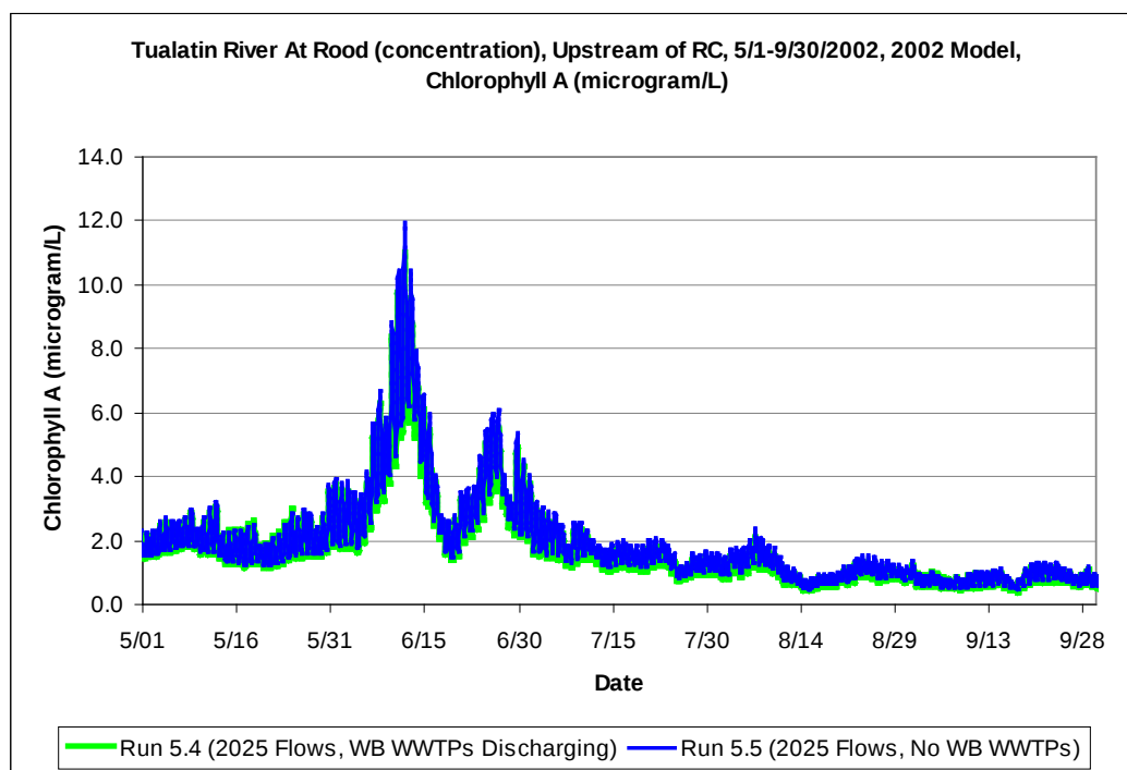
Figure 3-2. Model-predicted Chlorophyll a at Rood Road with and without Forest Grove and Hillsboro waste water treatment facility discharges, taken directly from the Total Phosphorus Modeling Report in Appendix 2-A.
