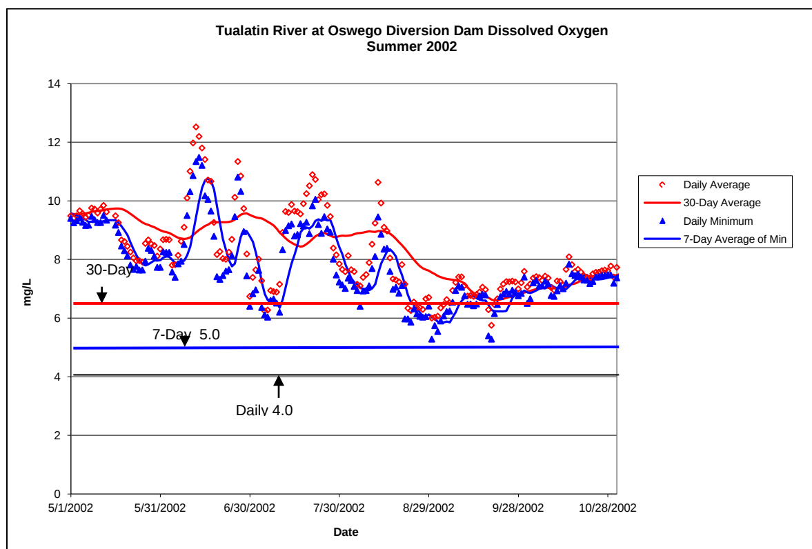
Figure 3-6. Various Dissolved Oxygen Statistics at Oswego Dam (RM 3.4) during the TMDL seasons of 2002 (no oxygen violations) and 2005 (30-day average below 6.5 mg/L criterion).
