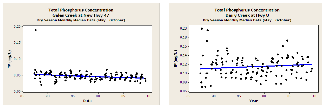
Figure 2-4. Monthly median concentrations of total Phosphorus are plotted over time at four different tributary locations in the Tualatin River Basin. The decrease in Gales Creek and increase in Dairy Creek are significant at the 95% confidence level, using the Seasonal Kendal Tau trend test. No significant trends are present at the Rock Creek and Fanno Creek sites.
