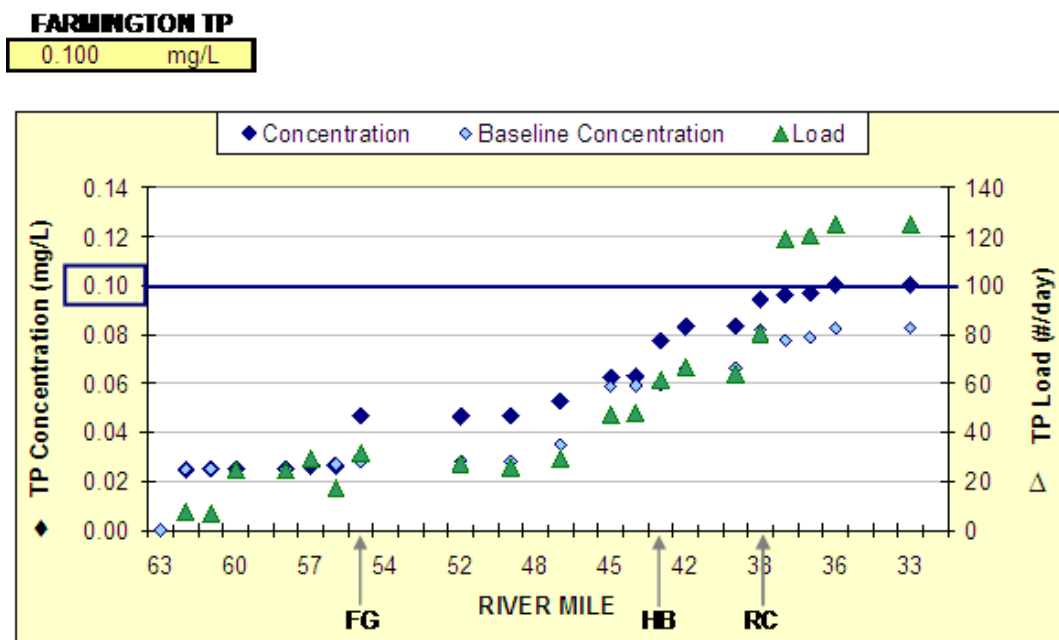
Figure 2-7. Primary TP Mass Balance Results (Median TP Concentration, May through October, 2002-2007) Assumes TP Mass Load \leq 66.1 lb/day, current flow augmentation levels, and tributaries meeting water quality standards.(See Appendix 2-A, Exhibit 2-10). Baseline Total P concentration (◇ light blue diamond) reflects current river concentrations, while the Concentration (◇, dark blue diamond) and load (△ green triangle) are projected future conditions based on a future 66.1 lb./day load.
