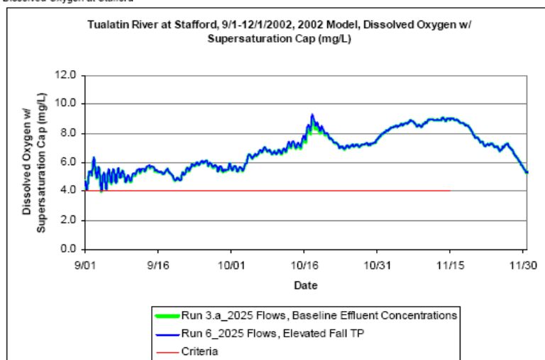
Dissolved Oxygen at Stafford
