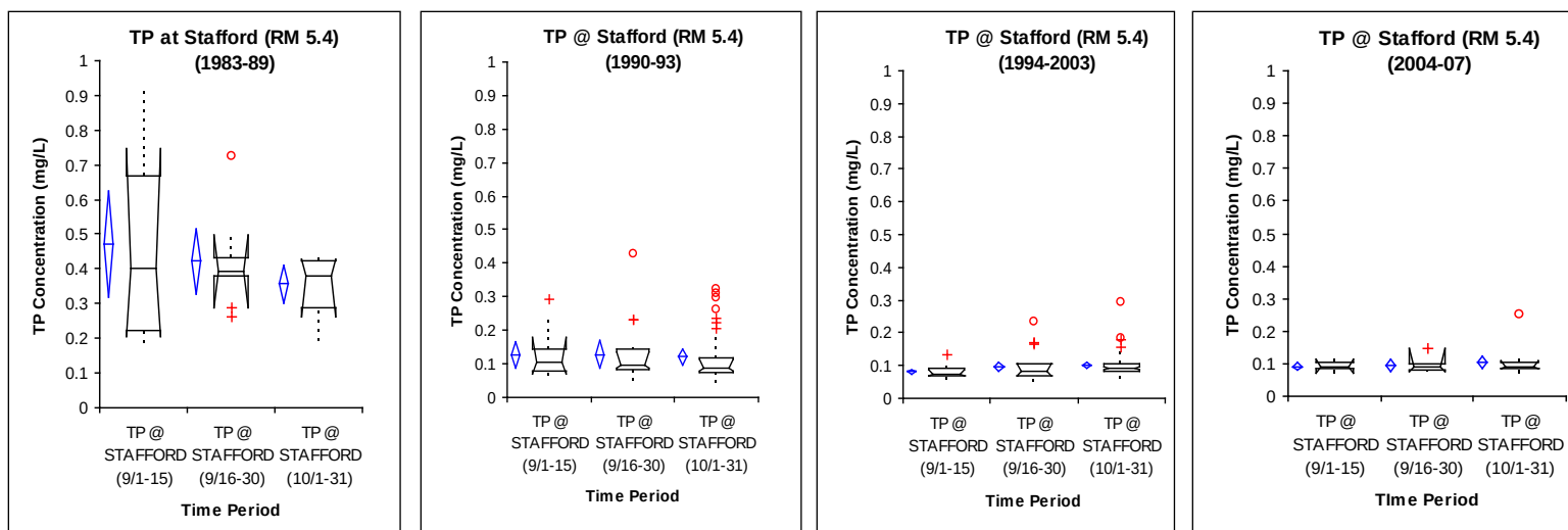
Figures 30, 31, 32 & 33 – Total Phosphorus Levels at Stafford during Various Time Periods (discrete data)
