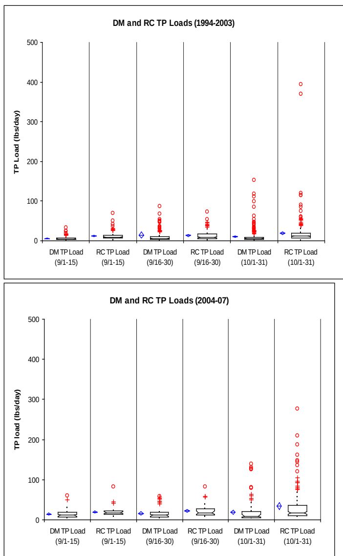
Figures 4, 5, 6, & 7 – Durham and Rock Creek AWWTF Total Phosphorus Loads for Various Time Periods
