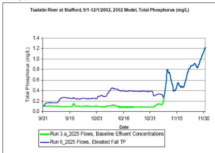
Total Phosphorus at Stafford
