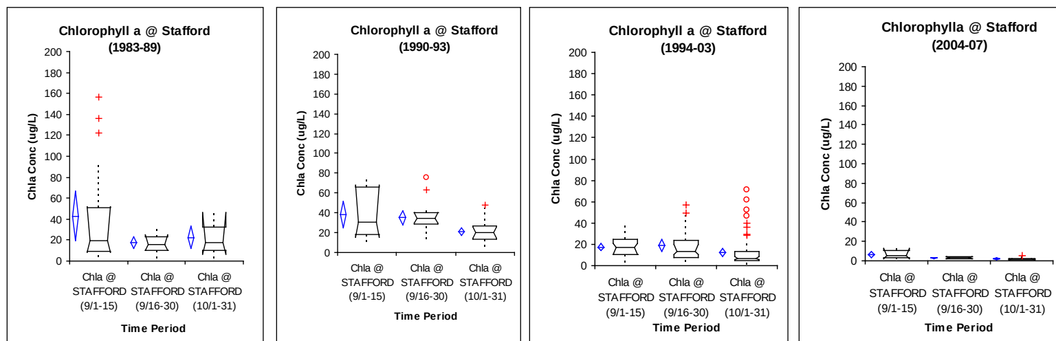
Figures 34, 35, 36 & 37 – Chlorophyll-a Levels at Stafford during Various Time Periods (discrete data)
