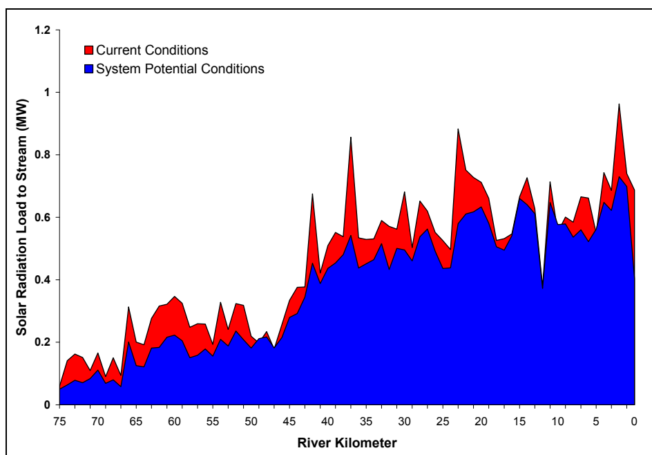
Figure 2 - 7: Comparison of solar radiation loading to the Molalla River under current conditions and system potential conditions, assessed at 100 m intervals.
