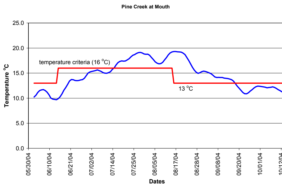
Figure 2 - 19: Moving seven day average of daily maximum temperatures measured in 2004 in Pine Creek, a tributary to the upper Molalla River.
