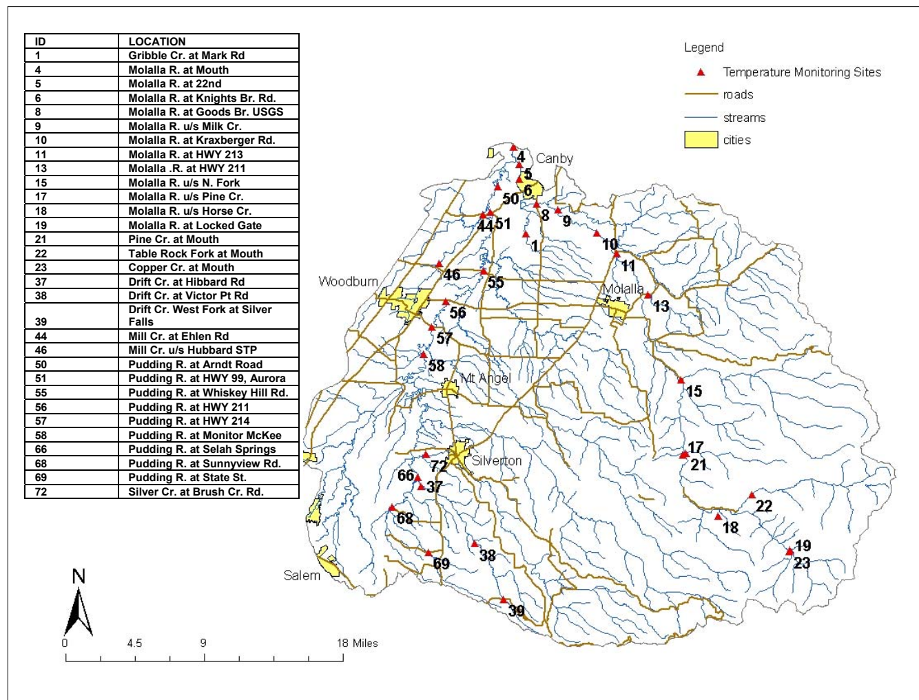
Figure 2 - 1: Locations where DEQ measured continuous temperature in the Molalla-Pudding Subbasin in summer 2004.
