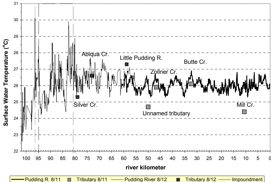
Figure 2 - 3: Longitudinal TIR median temperatures for the Pudding River on August 11 - 12, 2004.
