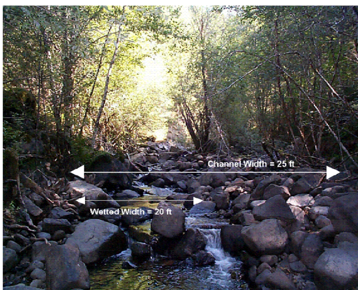
Figure 2 - 32: Illustrated channel width.
