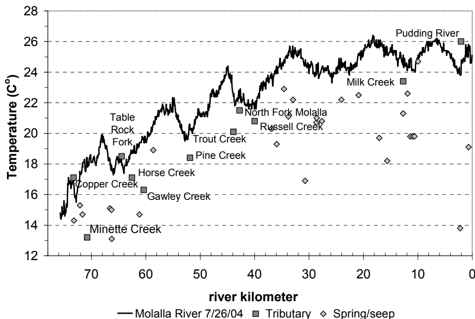
Figure 2 - 2: Longitudinal TIR median temperatures for the Molalla River on July 26, 2004.
