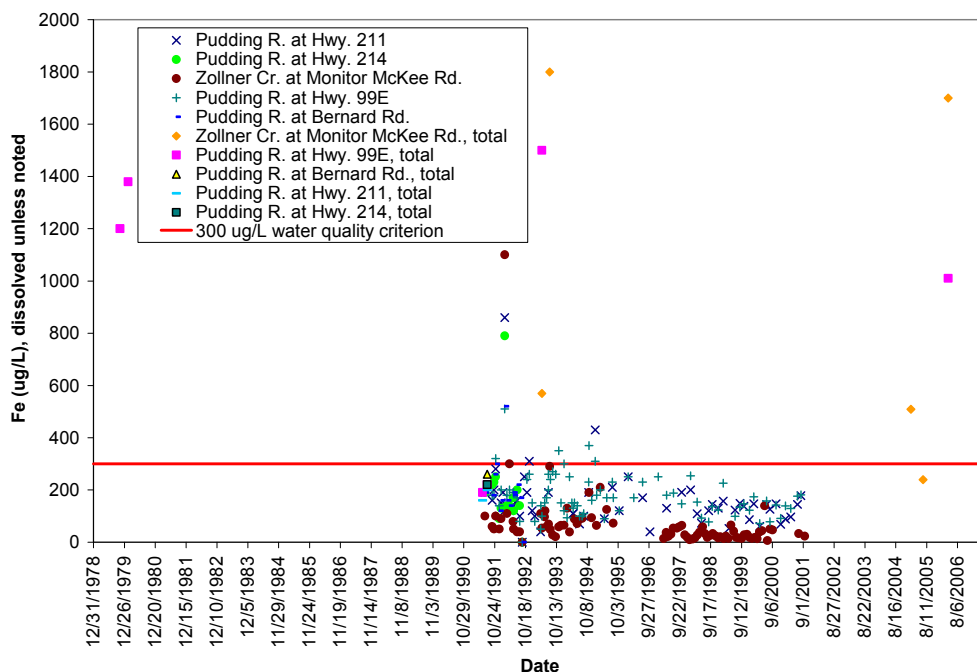
Figure M - 2: Iron concentrations in Pudding River and Zollner Creek, larger scale Y-axis. Two Zollner Creek samples collected in 2005 do not display on this scale. Exceedances occurred at several Pudding River sites on February 19, 1992.
