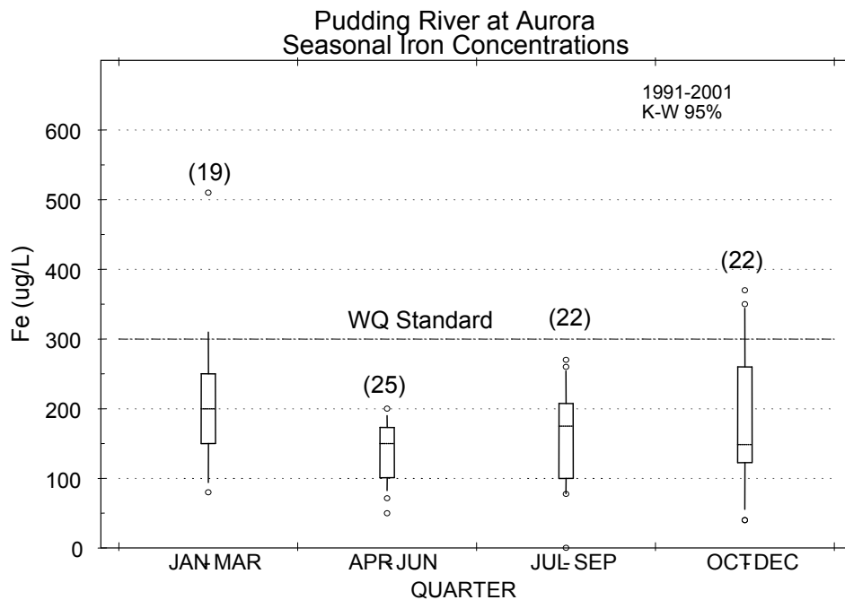
Figure M - 5: Seasonal variation in dissolved iron concentrations measured in samples collected at the Pudding River at Aurora, river mile 8.
