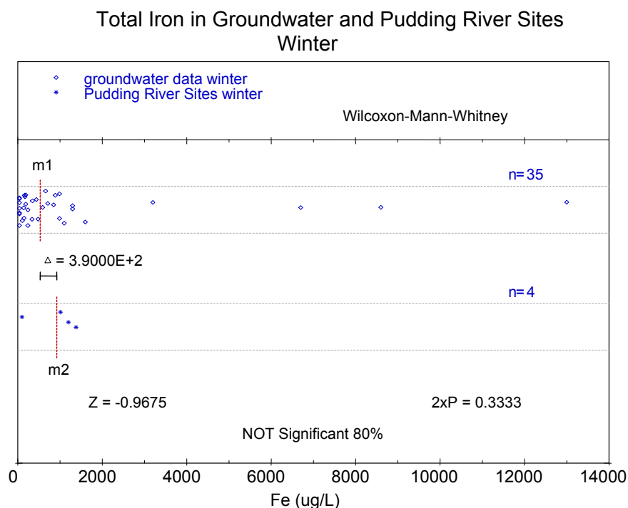
Figure M - 13: Comparison of means between total iron measured in groundwater in the winter months and total iron measured in surface water in the winter months at Pudding River sites (both data sets, DEQ data only).
