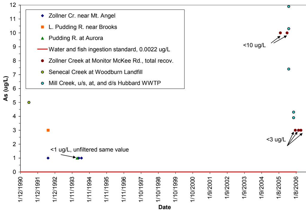
Figure M - 32: All available DEQ and USGS arsenic data from surface water samples in the Molalla-Pudding Subbasin.
