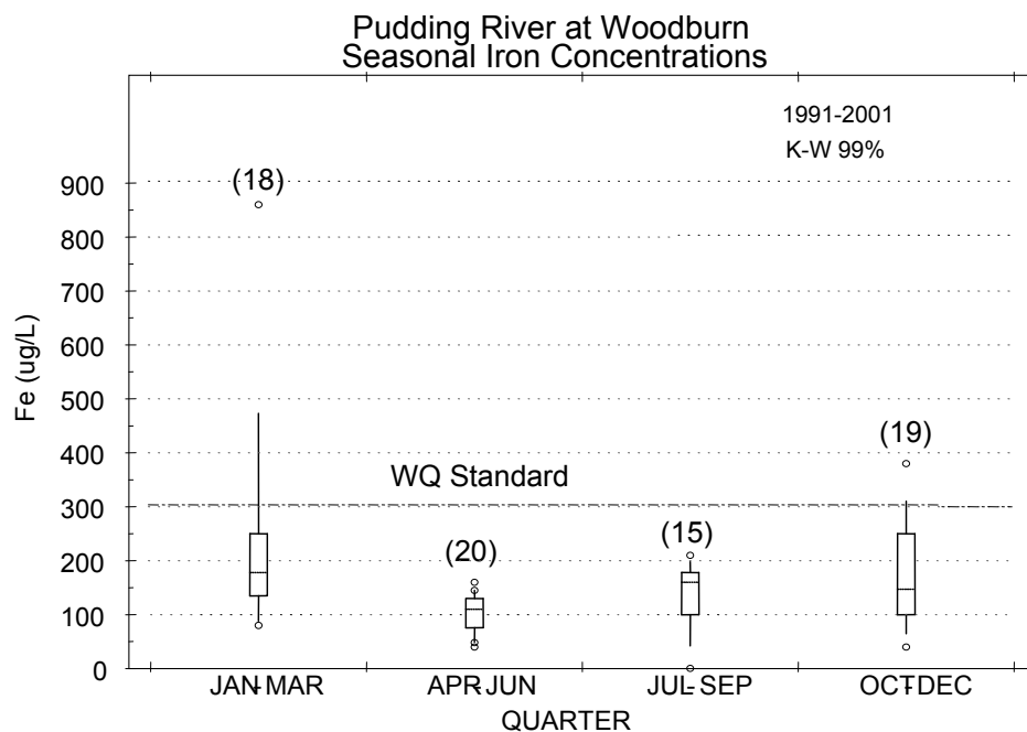
Figure M - 4: Seasonal variation in dissolved iron concentrations measured in samples collected at the Pudding River at Woodburn, river mile 21.
