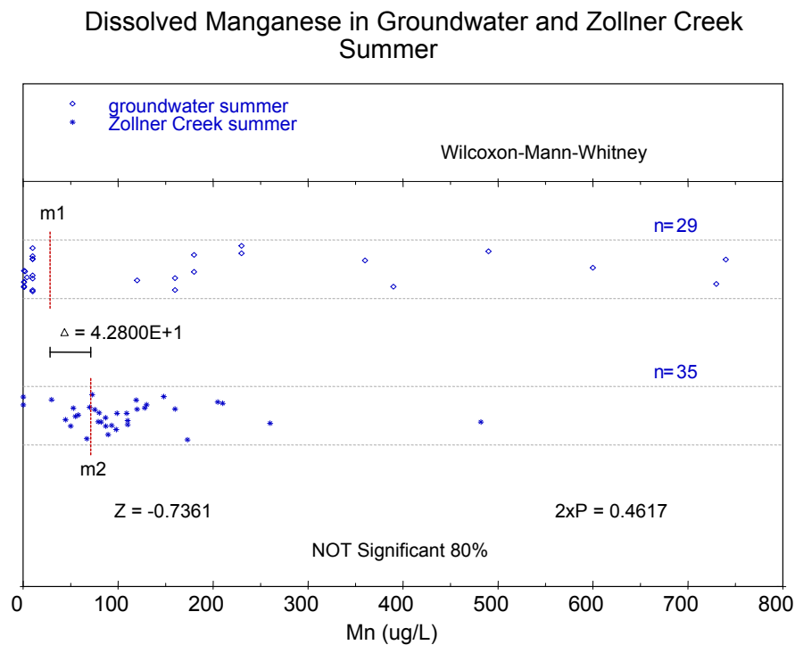
Figure M - 29: A comparison of dissolved manganese concentrations in groundwater to dissolved manganese concentrations measured in Zollner Creek at Monitor-McKee Rd./USGS gauge in the summer.
