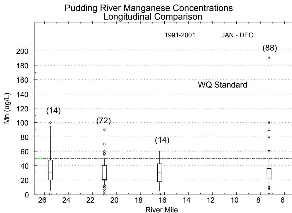
Figure M - 18: A longitudinal comparison of dissolved manganese concentrations from DEQ collected data between 1991 and 2001.
