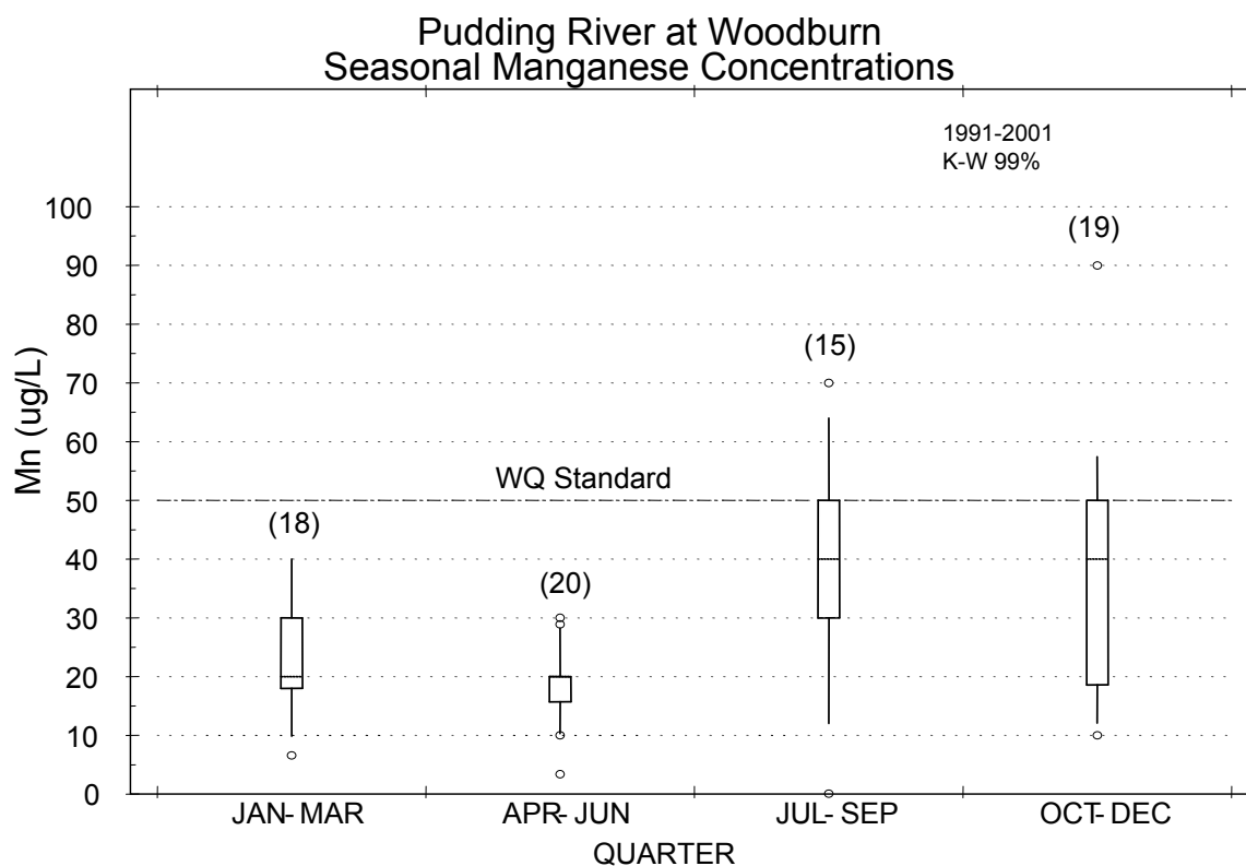
Figure M - 19: Seasonal variability in dissolved manganese concentrations measured in samples collected from the Pudding River at Woodburn/Hwy. 211.
