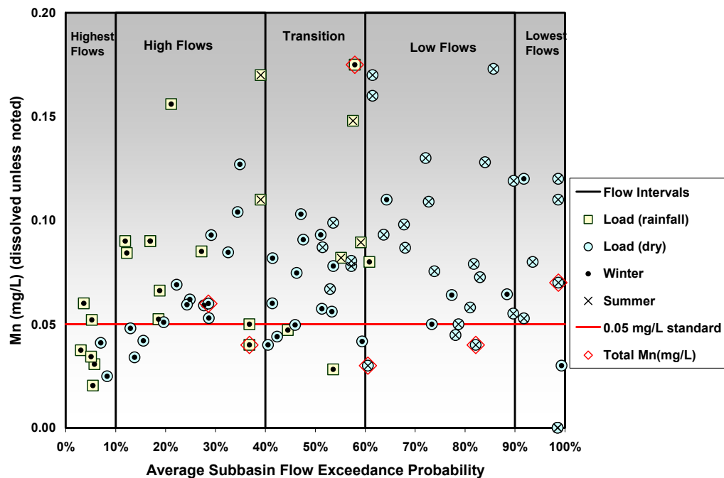
Figure M - 25: Zollner Creek concentration duration curve.
