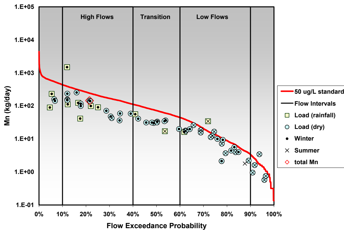
Figure M - 22: Pudding River at Aurora load duration curve based on dissolved concentrations of manganese, except where noted.
