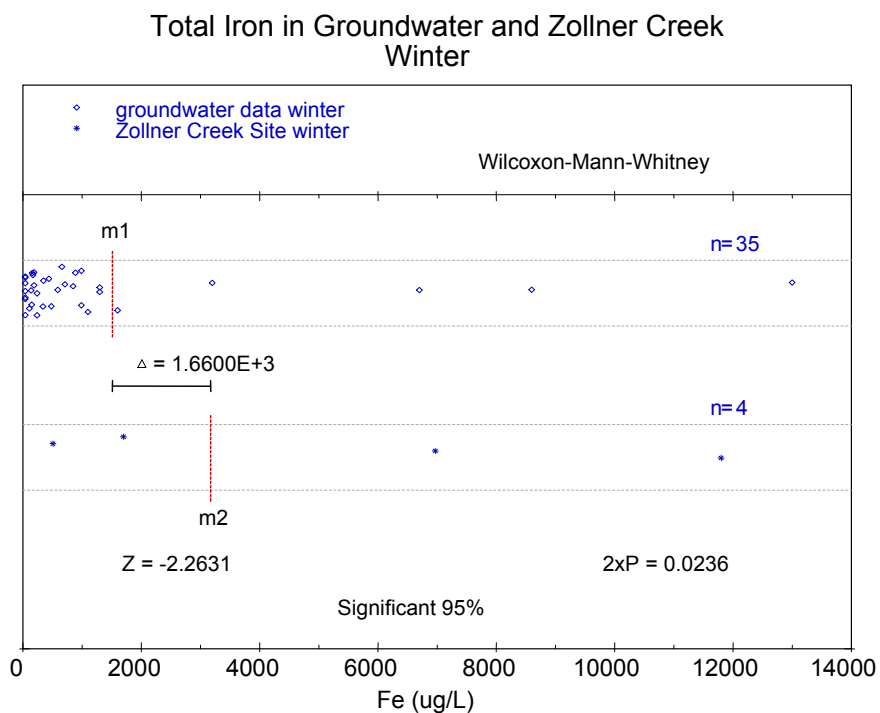
Figure M - 16: Comparison of means between total iron measured in groundwater in the winter months and total iron measured in surface water in the winter months in Zollner Creek (both data sets, DEQ data only).
