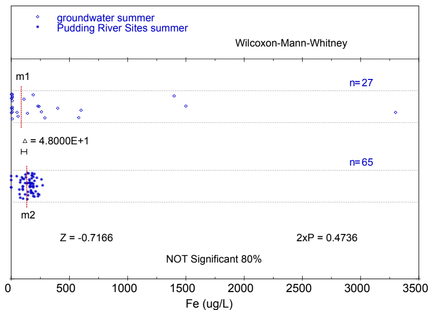
Figure M - 11: Comparison of means between dissolved iron measured in groundwater and Pudding River surface water in the summer months.
