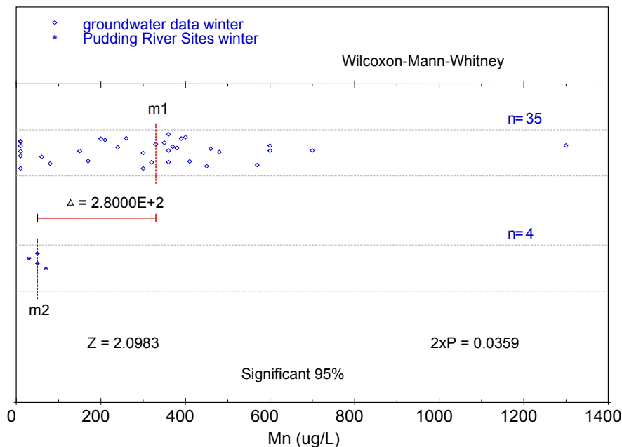
Figure M - 28: A comparison of total groundwater manganese concentrations to those measured in the Pudding River, both in the winter months.
