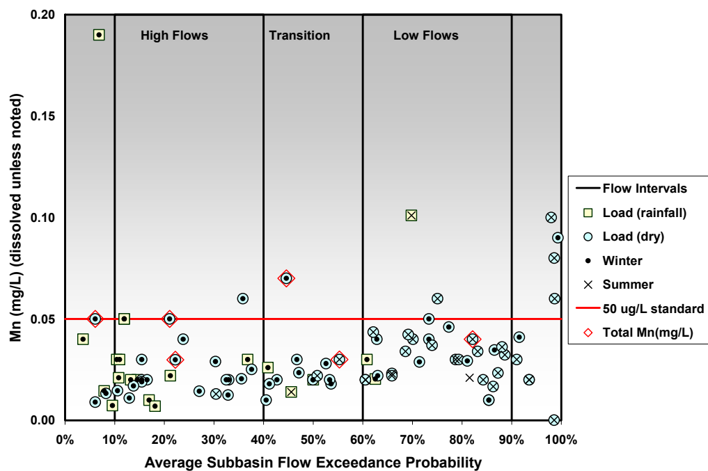
Figure M - 23: Concentration duration curve for Pudding River at Aurora.
