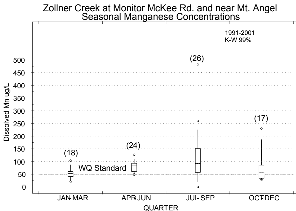
Figure M - 21: Seasonal variability in dissolved manganese concentrations measured in samples collected from Zollner Creek at Monitor McKee Bridge/USGS gauge.
