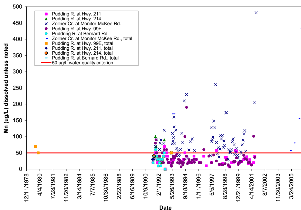
Figure M - 17: Manganese concentrations from Pudding River and Zollner Creek sites.
