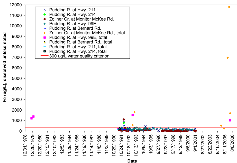
Figure M - 1: Iron concentrations in Pudding River and Zollner Creek.
