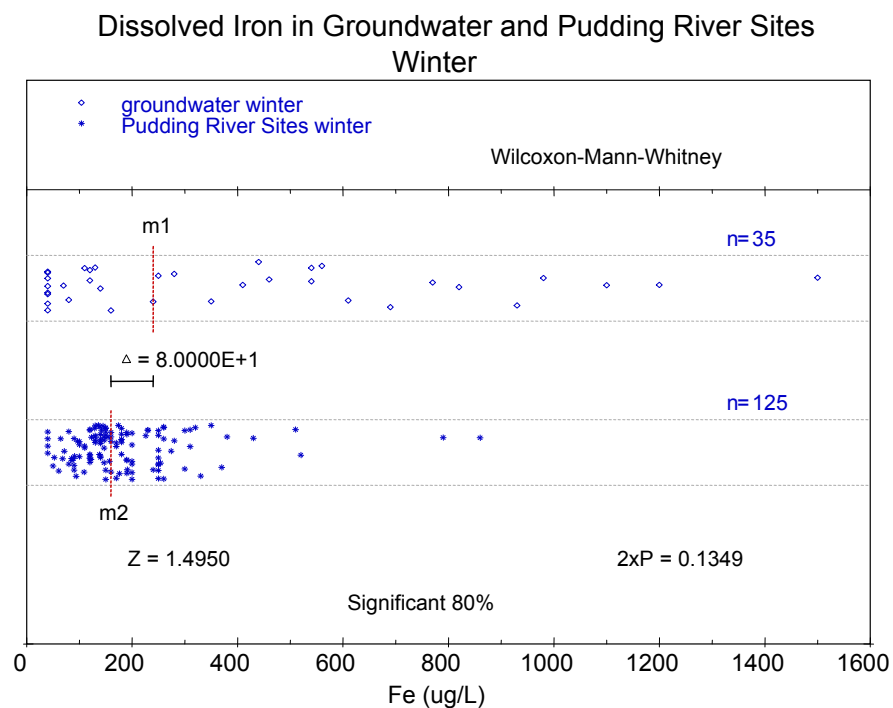
Figure M - 12: Comparison of means between dissolved iron measured in groundwater in the winter months (DEQ data only) and dissolved iron measured in surface water in the winter months at Pudding River sites (both DEQ and USGS data).
