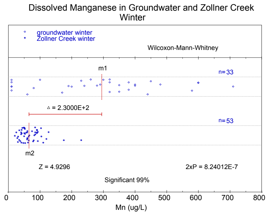
Figure M - 30: Dissolved manganese measurements in Zollner Creek compared with dissolved manganese concentrations in groundwater, both data sets from winter months.
