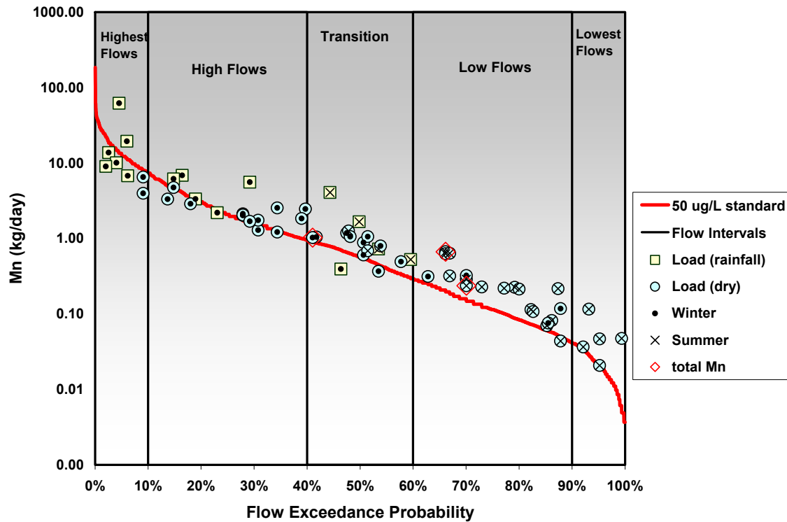
Figure M - 24: Zollner Creek load duration curve.
