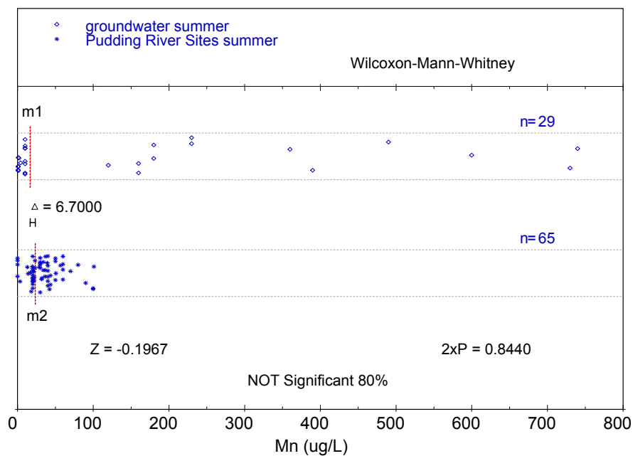
Figure M - 26: A comparison of dissolved groundwater manganese concentrations to those measured in the Pudding River in the summer months.
