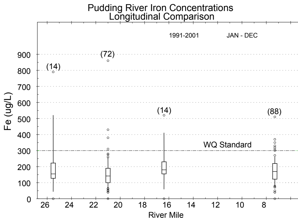
Figure M - 3: Variation in dissolved iron concentrations (DEQ collected data) between and within four Pudding River sites.
