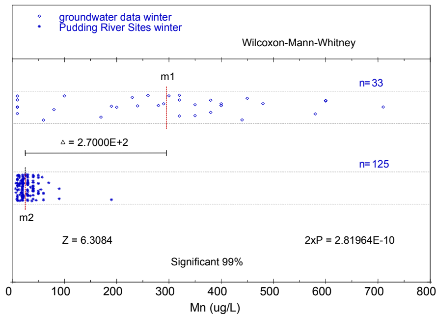
Figure M - 27: A comparison of dissolved groundwater manganese concentrations to those measured in the Pudding River, both in the winter months..
