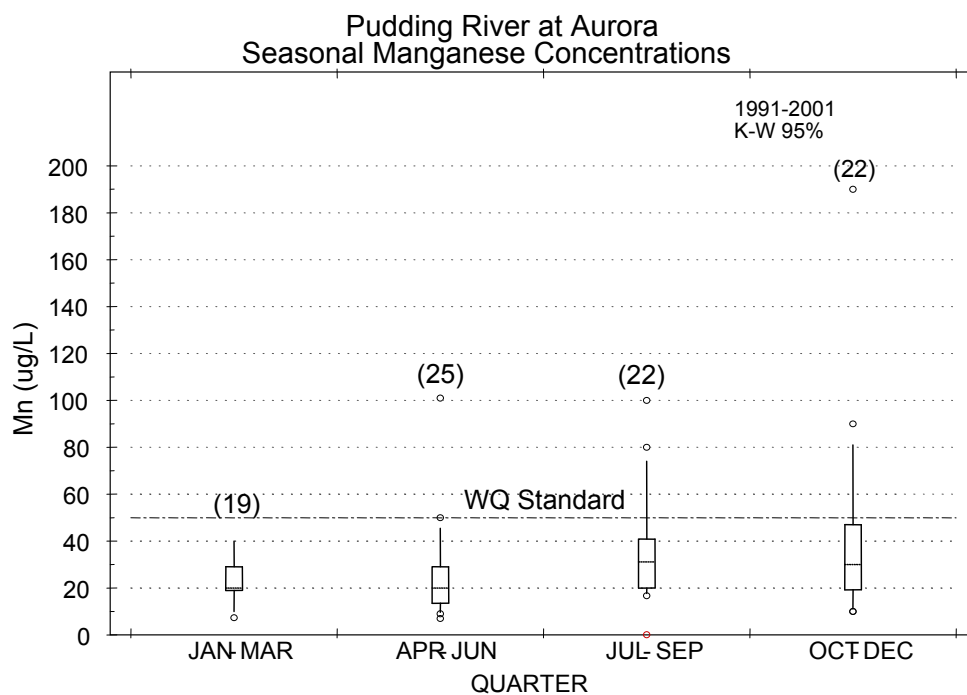
Figure M - 20: Seasonal variability in dissolved manganese concentrations measured in samples collected from the Pudding River at Aurora/Hwy. 99E.
