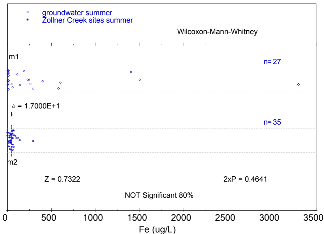
Figure M - 14: Comparison of means between dissolved iron measured in groundwater and Zollner Creek surface water in the summer months.
