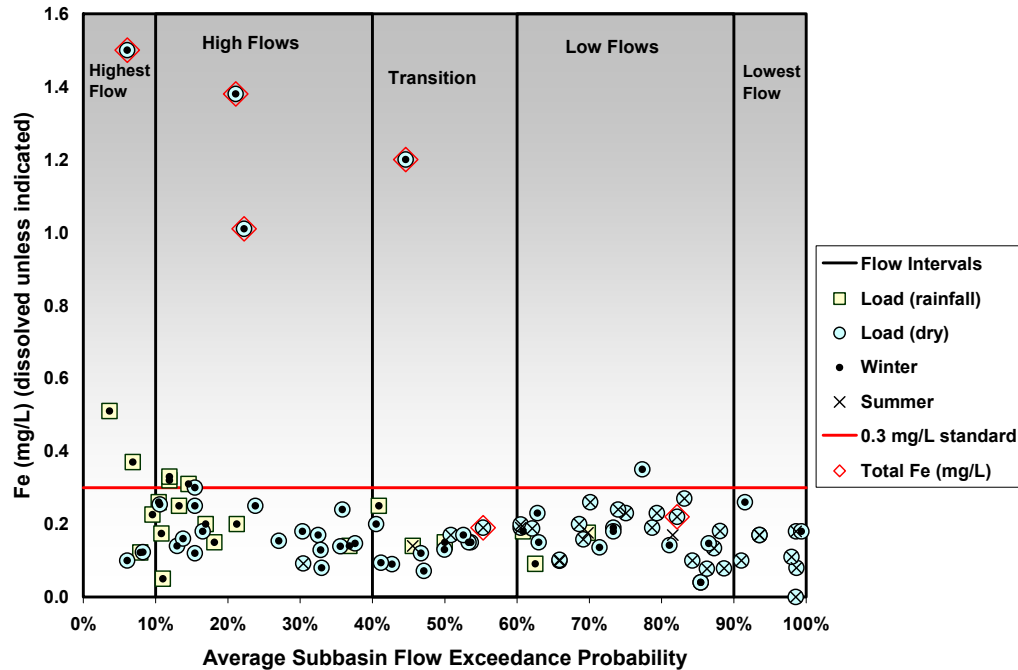
Figure M - 8: Concentration duration curve for Pudding River at Aurora.
