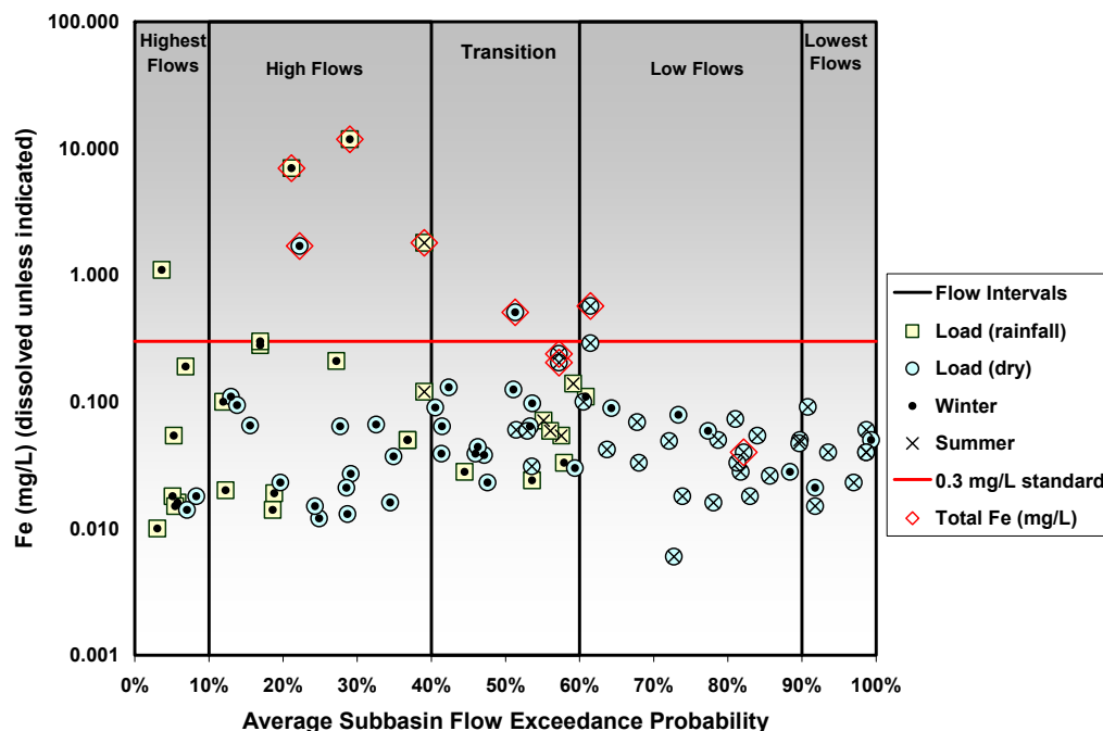
Figure M - 10: Zollner Creek at Monitor-McKee Road concentration duration curve. Data points designated “rainfall” occurred on a day with at least 0.15 inches of precipitation. Data points designated “Winter” occurred October through May.
