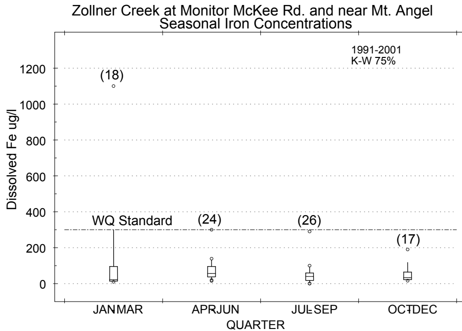
Figure M - 6: Seasonal variation in dissolved iron concentrations measured in samples collected from Zollner Creek.
