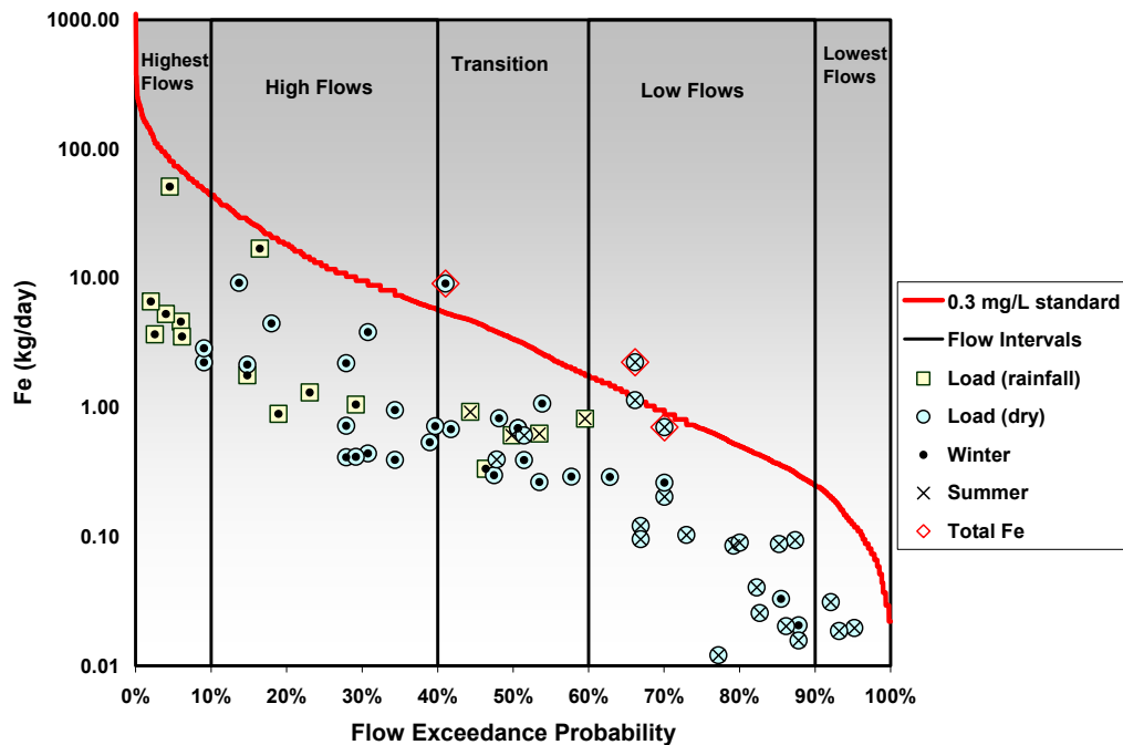
Figure M - 9: Zollner Creek at Monitor McKee Road load duration curve.
