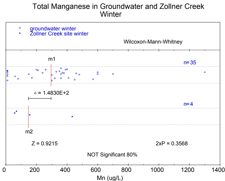
Figure M - 31: A comparison of total groundwater manganese concentrations to those measured in the Zollner Creek, both in the winter months.
