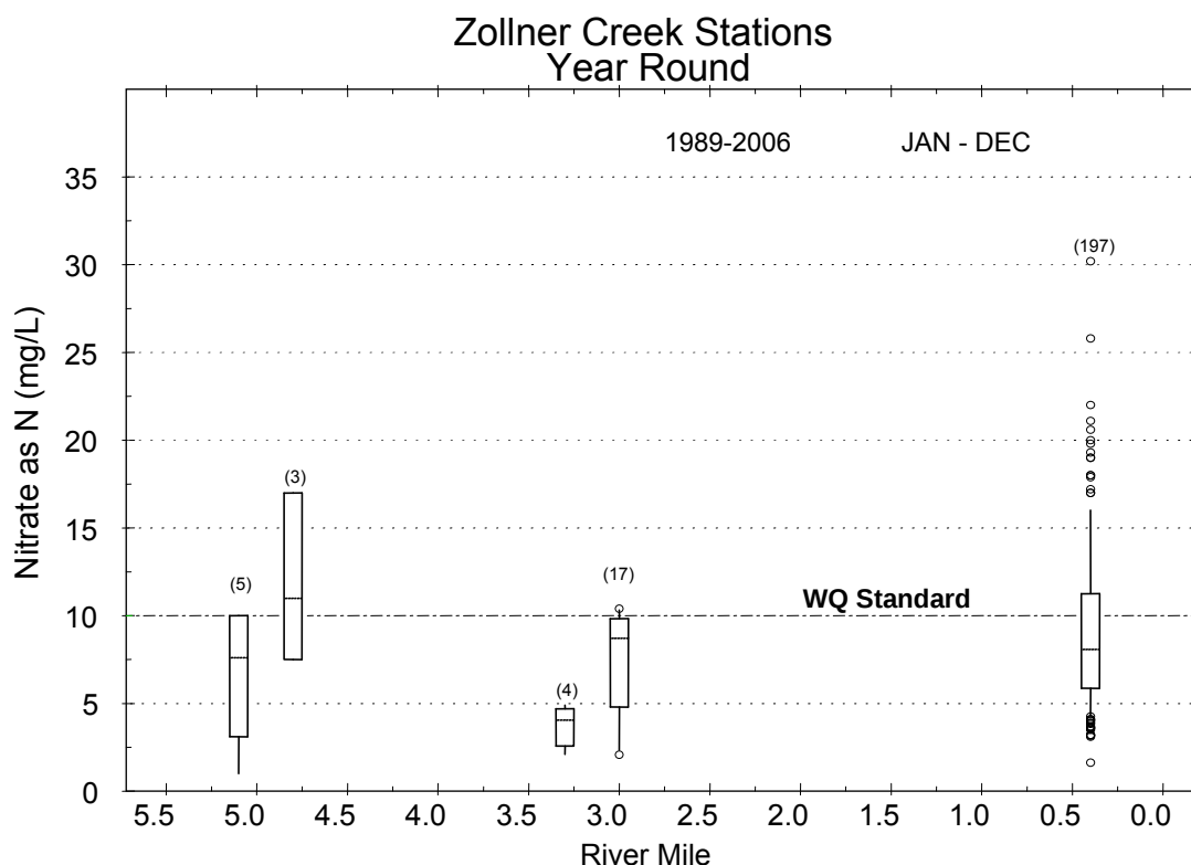
Figure L - 1: Zollner Creek longitudinal plot of nitrate-N concentration distribution.
