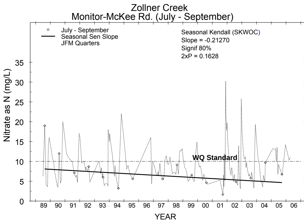
Figure L - 5: Zollner Creek nitrate-N concentrations, July through September, 1989 - 2006. The data indicate a statistically significant downward trend at the 80% confidence level.
