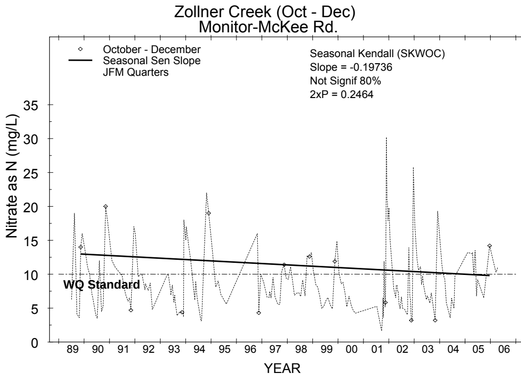
Figure L - 6: Zollner Creek nitrate-N concentrations, October through December 1989 - 2006. The data do not indicate a statistically significant trend at the 80% confidence level.
