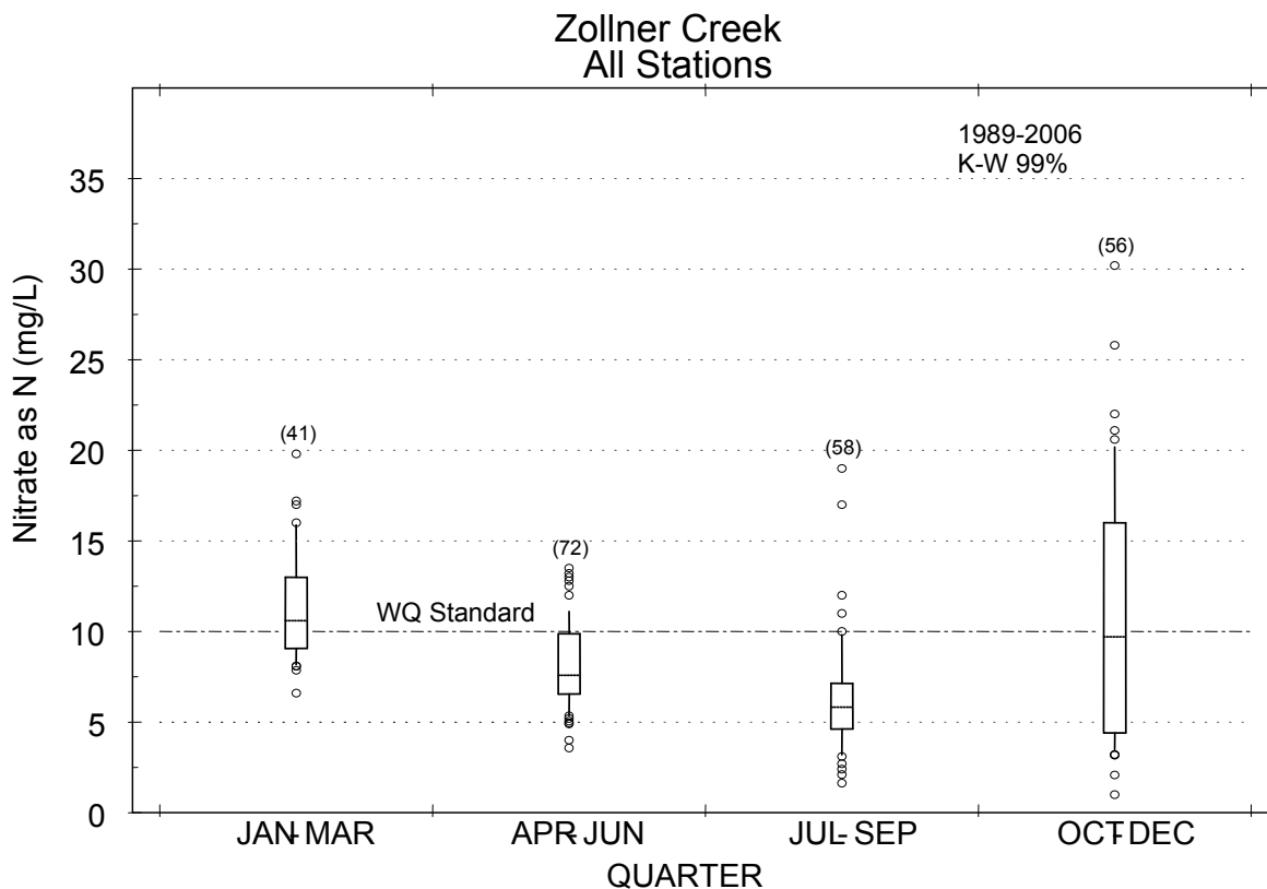
Figure L - 7: Zollner Creek nitrate-N concentration distributions plotted by quarter.
