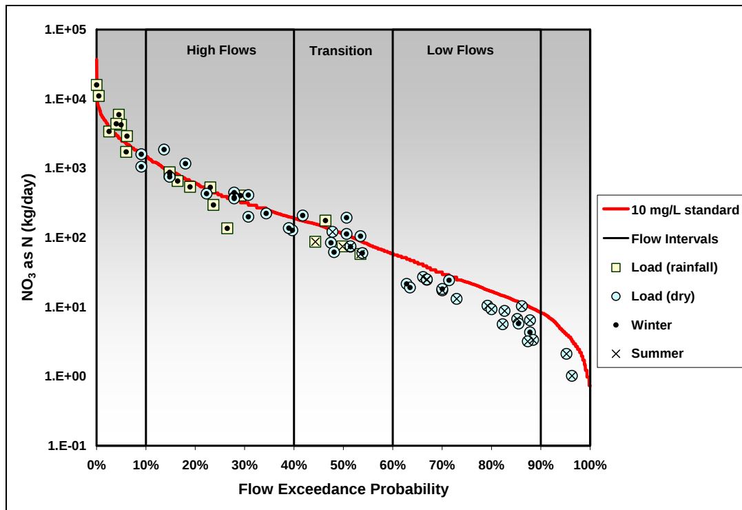
Figure L - 8: Most violations of the water quality standard occur and transition and high stream flows.
