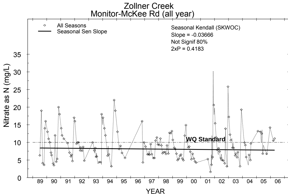
Figure L - 2: Zollner Creek nitrate-N concentrations 1989 and 2006. Data do not show a statistically significant trend at the 80% confidence level.
