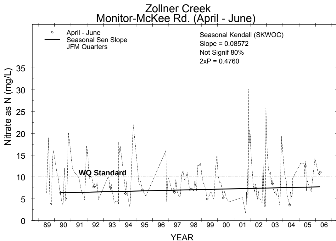
Figure L - 4: Zollner Creek nitrate-N concentrations, April through June, 1989 - 2006. The data do not indicate a statistically significant trend.
