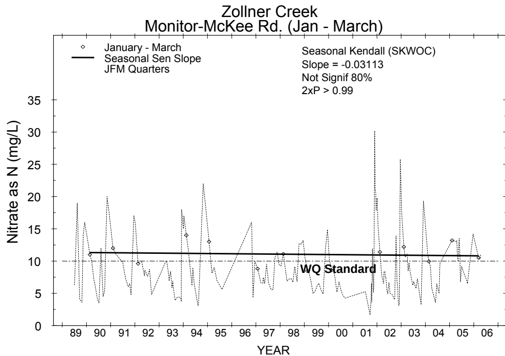
Figure L - 3: Zollner Creek nitrate concentrations, January through March 1989 - 2006. The data do not indicate a statistically significant trend.
