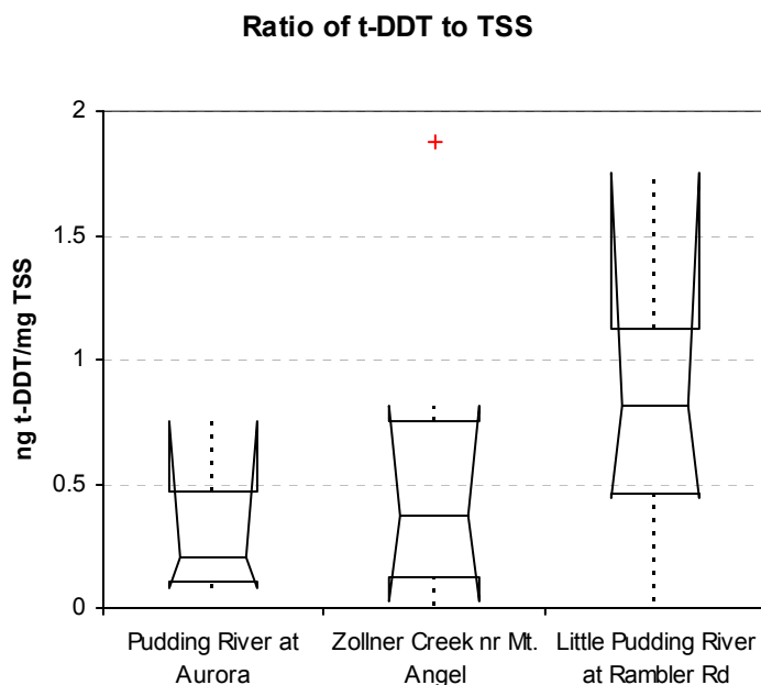
Figure J- 3: ODEQ t-DDT:TSS ratios for 3 sites
