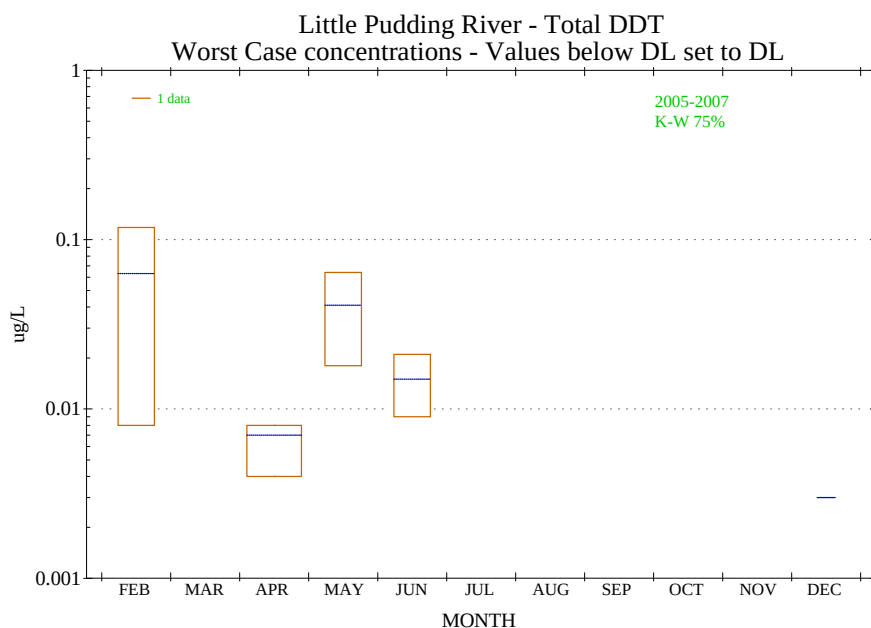
Figure J- 5: Little Pudding River - Total DDT - Aggregated by month
