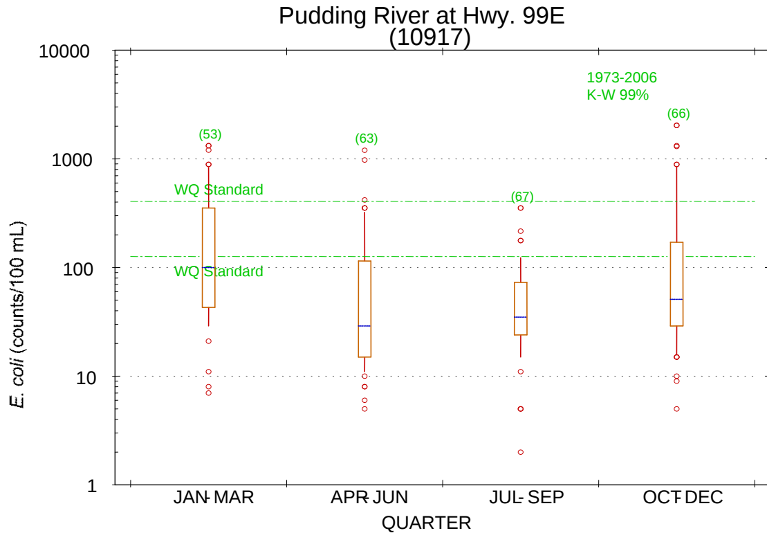
Figure G- 4: Quarterly variation in bacterial counts measured in the Pudding River at Highway 99E, river mile 7.3.
