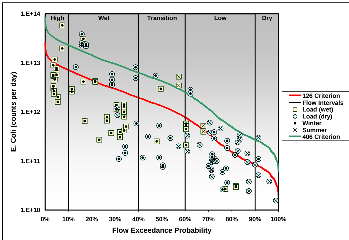
Figure G- 17: Load duration curve for Pudding River at Highway 211, RM 21, from 1969 – 2006 data. USGS Gage Pudding River near Woodburn.
