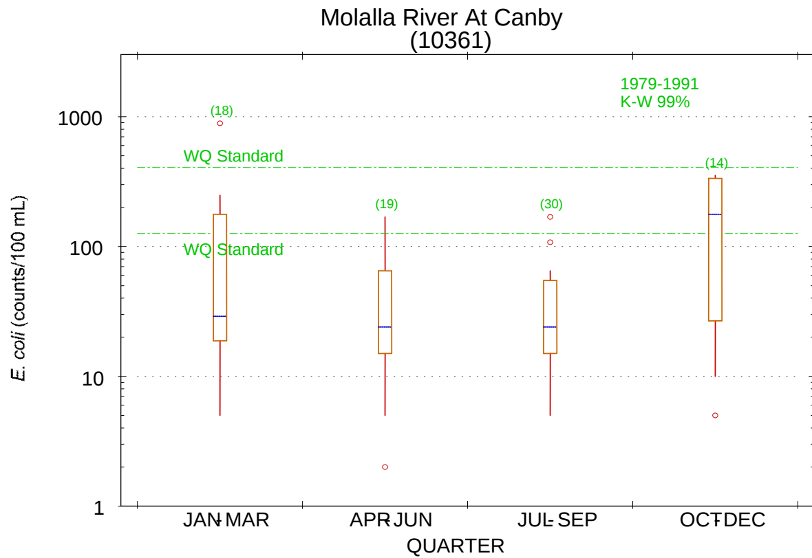
Figure G- 14: Seasonal distribution of bacteria data collected from Molalla River at Canby. Fecal coliform data have been converted to E. coli equivalents.
