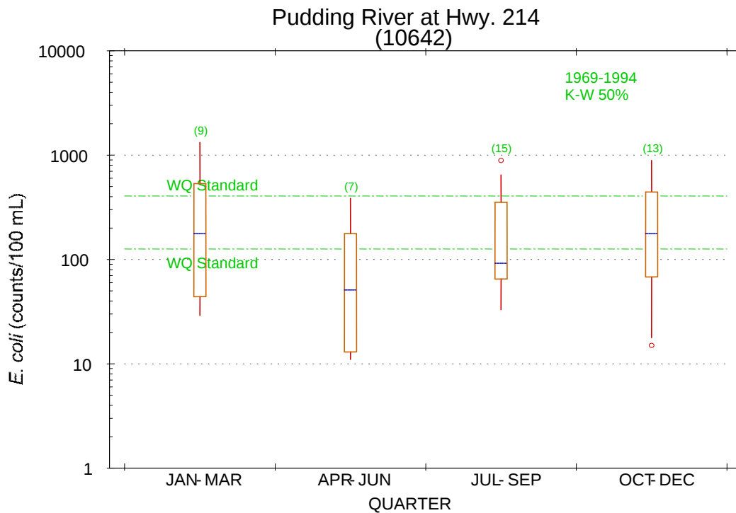
Figure G- 6: Quarterly variation in bacterial counts measured in the Pudding River at Highway 214, river mile 25.5.
