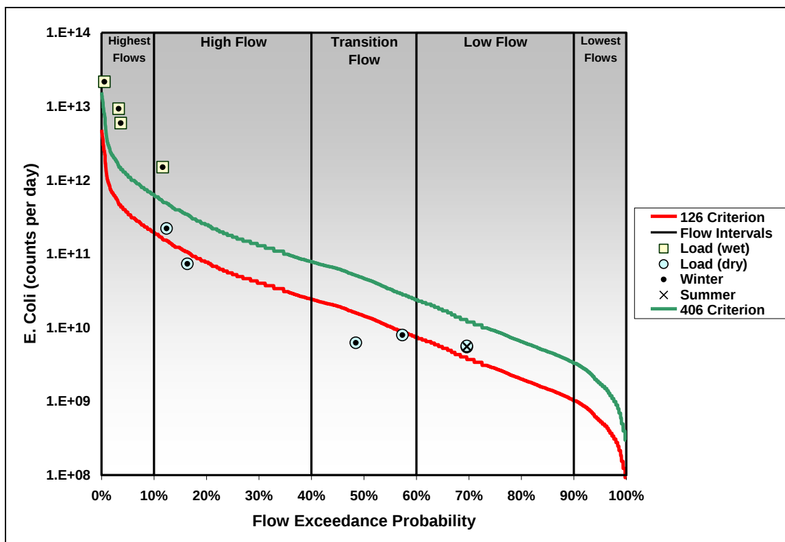
Figure G- 19: Load duration curve for Zollner Creek at Monitor McKee Road from 2004 – 2006 data. USGS gage Zollner Creek near Mt. Angel.
