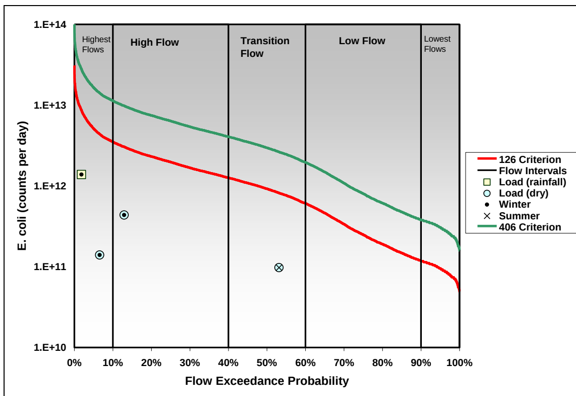
Figure G- 24: Load duration curve for Molalla River upstream of North Fork Molalla, river mile 25. Data period 2004 – 2006. USGS gage Molalla River near Wilhoit and estimated from Molalla River near Canby.
