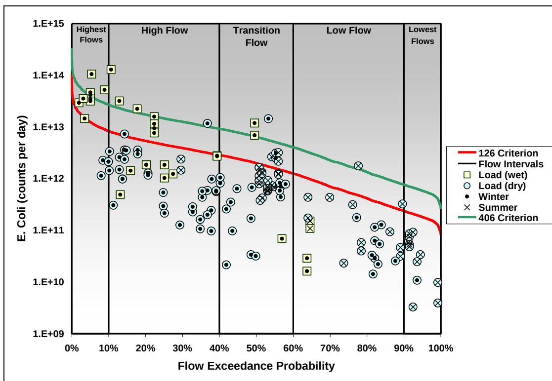
Figure G- 23: Load duration curve for Molalla River at Knights Bridge Road, from 1968 – 2006 data. USGS Gage Molalla River near Canby.
