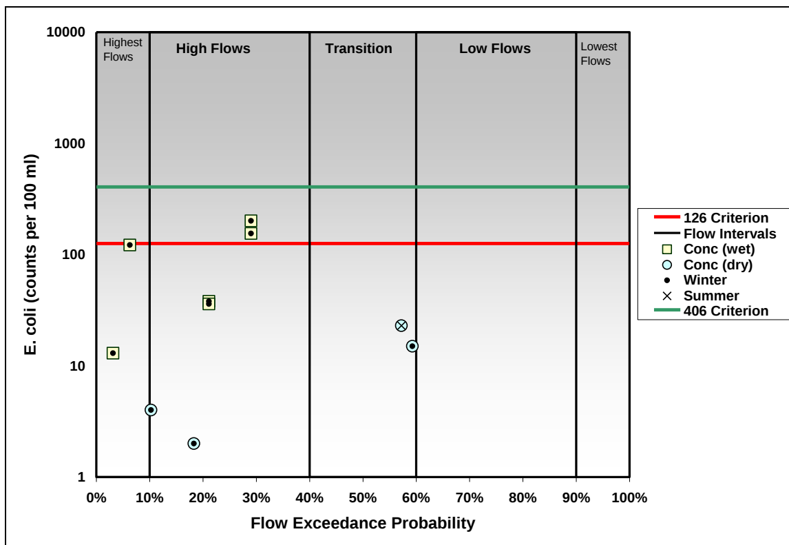
Figure G- 22: Concentration duration curve from Butte Creek at Butte Creek Road, representative of mainly forestry land use.
