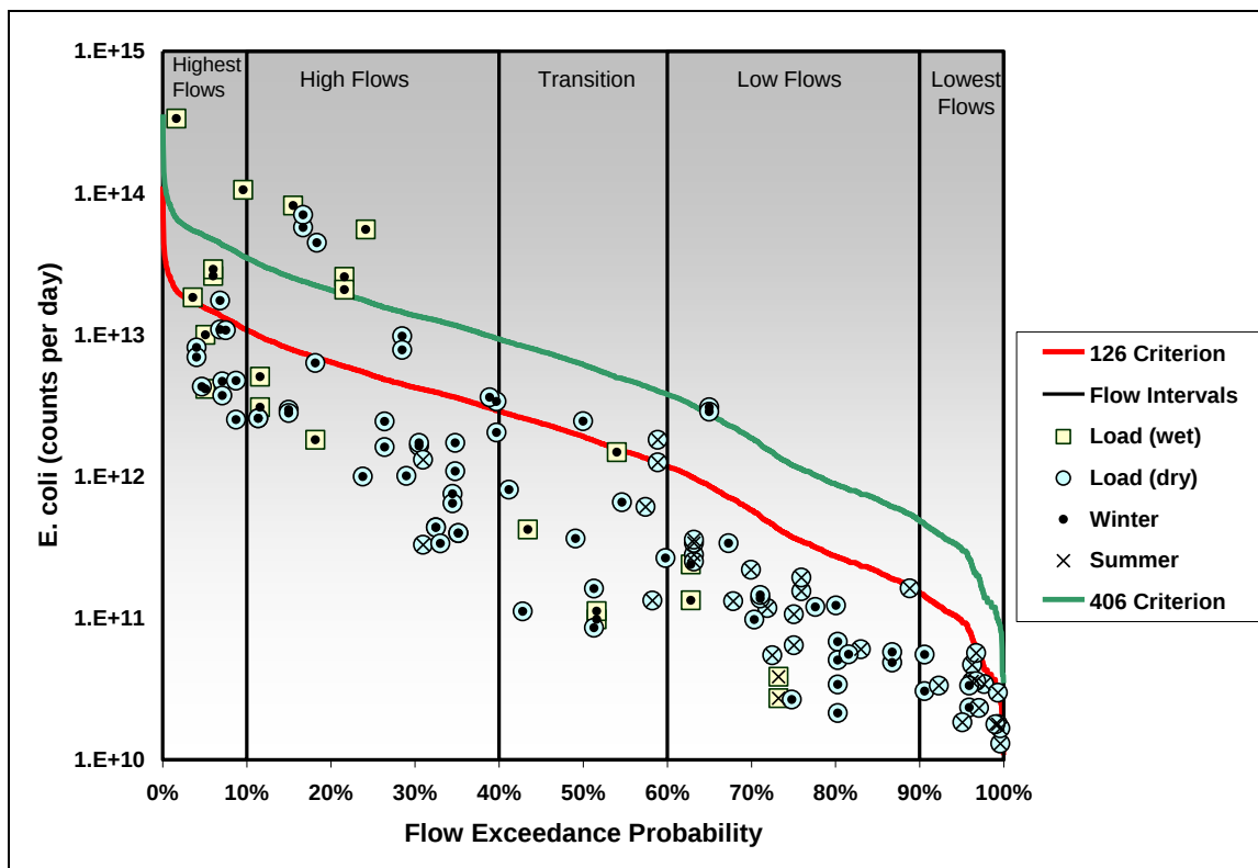
Figure G- 16: Load duration curve for Pudding River at Highway 99E, RM 7.3, from 1973 – 2006 data. USGS gage Pudding River at Aurora.
