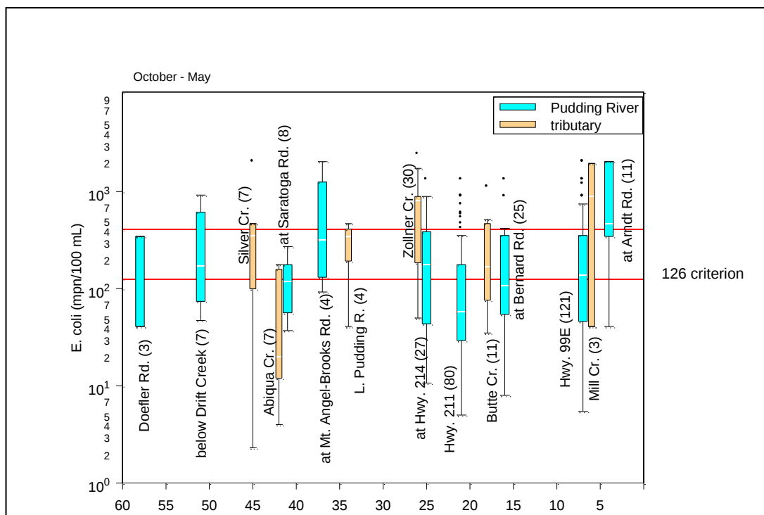
Figure G- 2: Pudding River and tributary bacteria concentration distributions measured in winter months (October – May) 1969 - 2006.
