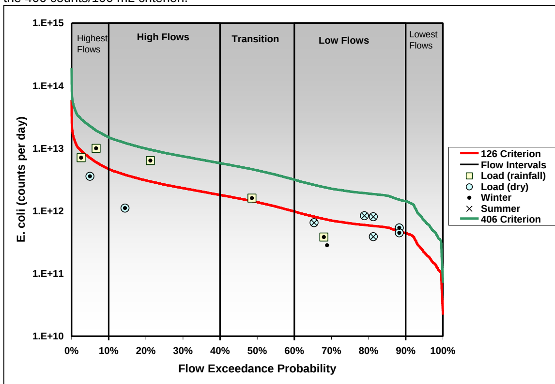
Figure G- 18: Load duration curve with data points combined from Pudding River at Saratoga Road (river mile 41) and Pudding River at Nusom Road (river mile 44). Data period 1989 - 2006. Flow estimated from three USGS gages: Pudding River at Aurora, Molalla River at Canby, and Molalla River near Wilhoit.
