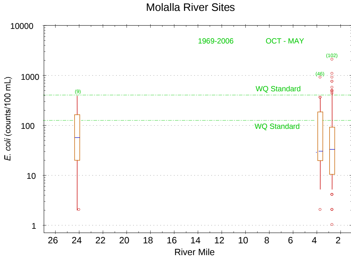
Figure G- 11: Distribution of bacterial concentrations measured in winter months (October – May) along the lower Molalla River.
