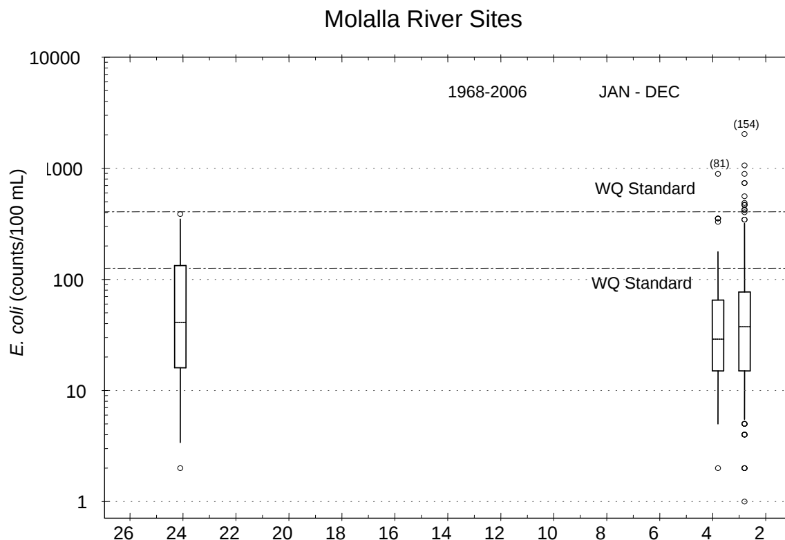
Figure G- 10: Distribution of bacterial concentrations measured year-round along the lower Molalla River. Fecal coliform data have been converted to equivalent E. coli counts. Horizontal lines indicate the two numeric E. coli bacteria criteria, the 126 log mean criterion and the single sample 406 criterion.
