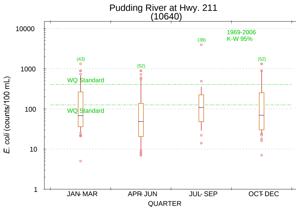
Figure G- 5: Quarterly variation in bacterial counts measured in the Pudding River at Highway 211, river mile 21.
