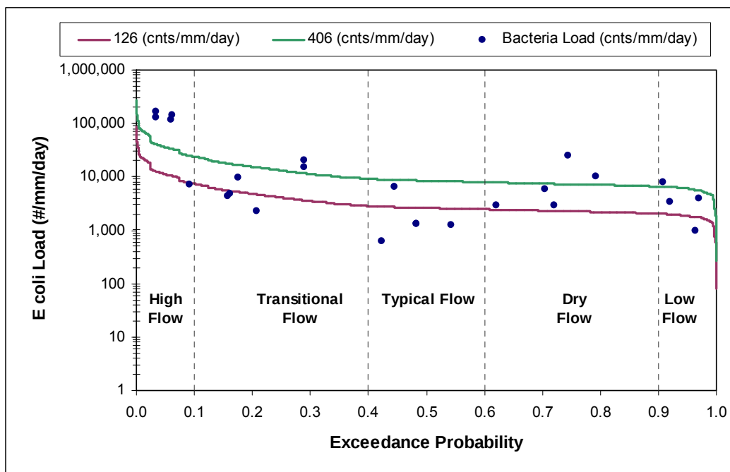
Figure F- 4: Example Load Duration Curve showing the loading capacity and calculated event loads.
