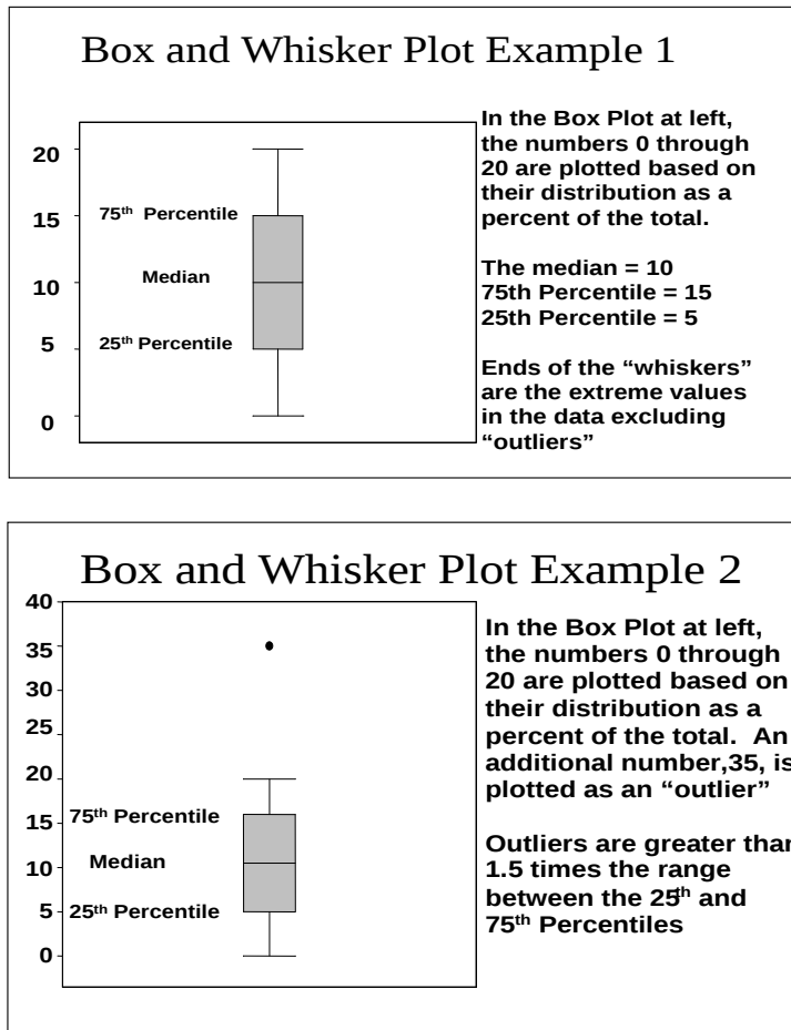
Figure F- 3: Two box and Whisker Plot examples.
