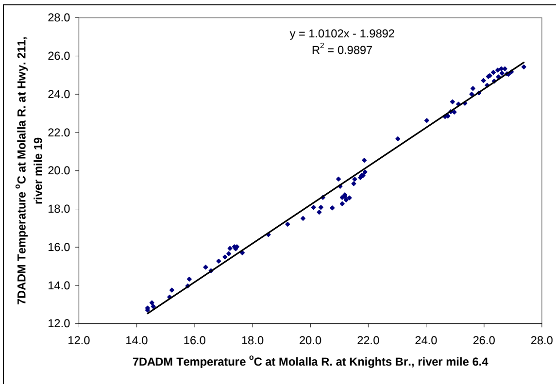
Figure E- 13: Comparison of 2004 7DADM temperatures from Molalla River at Knights Bridge Rd. (river mile 6.4) and Molalla River at Hwy. 211 (river mile 19).
