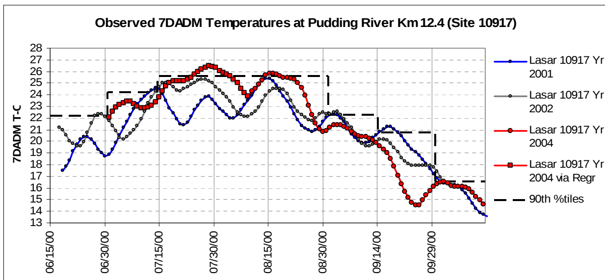
Figure E- 6: Ambient river temperatures and seasonal 90th percentiles (with July 15 to Aug 31 combined).
