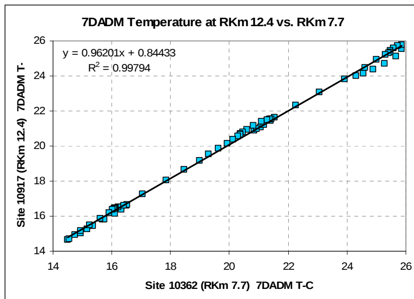
Figure E- 4: Correlation of 7DADM temperature at Aurora to temperature at RKm 7.7
