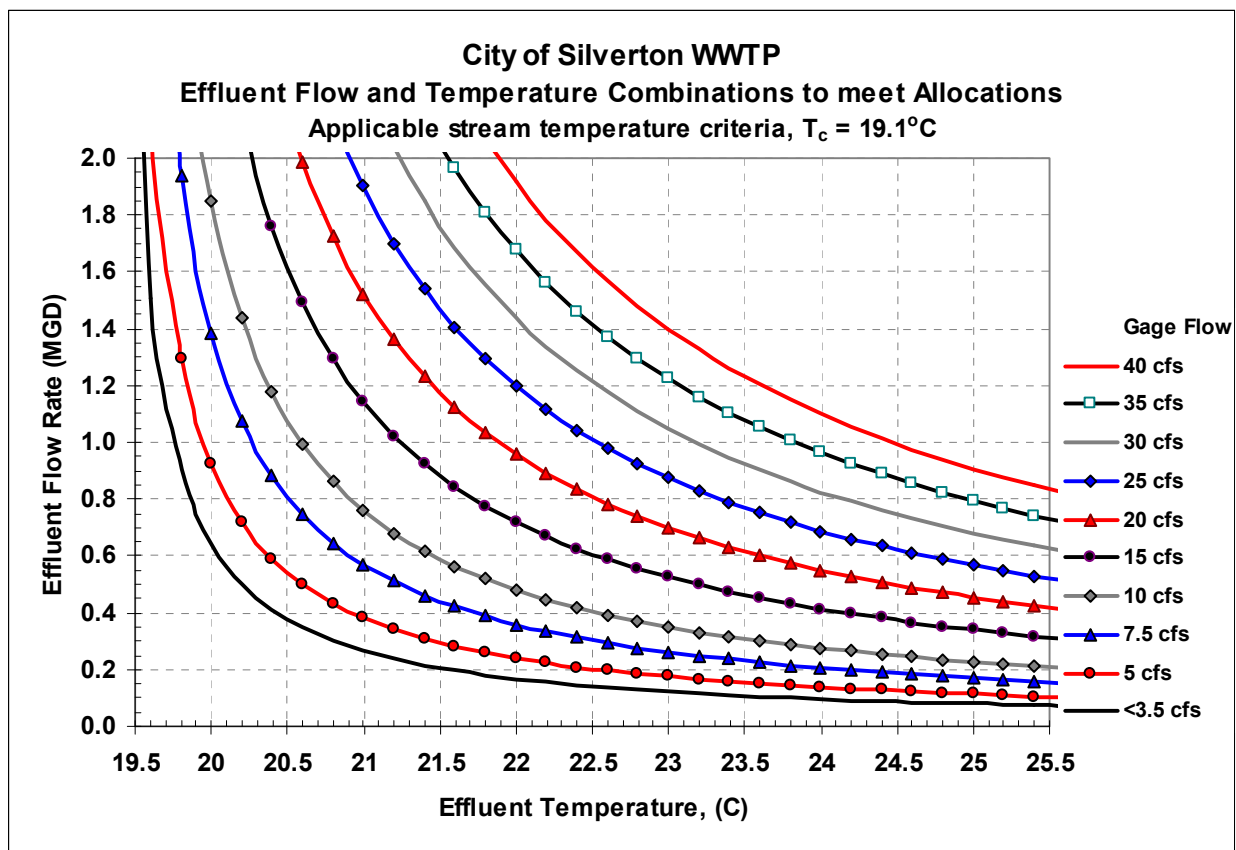
Figure D- 7: Effluent flow and temperature combinations for Silverton WWTP that meet allocation for applicable criteria, T_c=19.1^\circ\text{C} .
