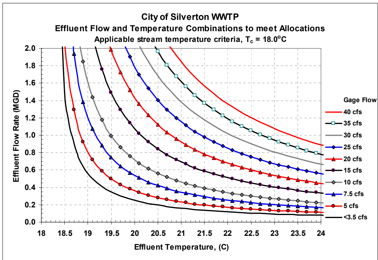
Figure D- 8: Effluent flow and temperature combinations for Silverton WWTP that meet allocation for applicable criteria, T_c=18.0^\circ\text{C} .
