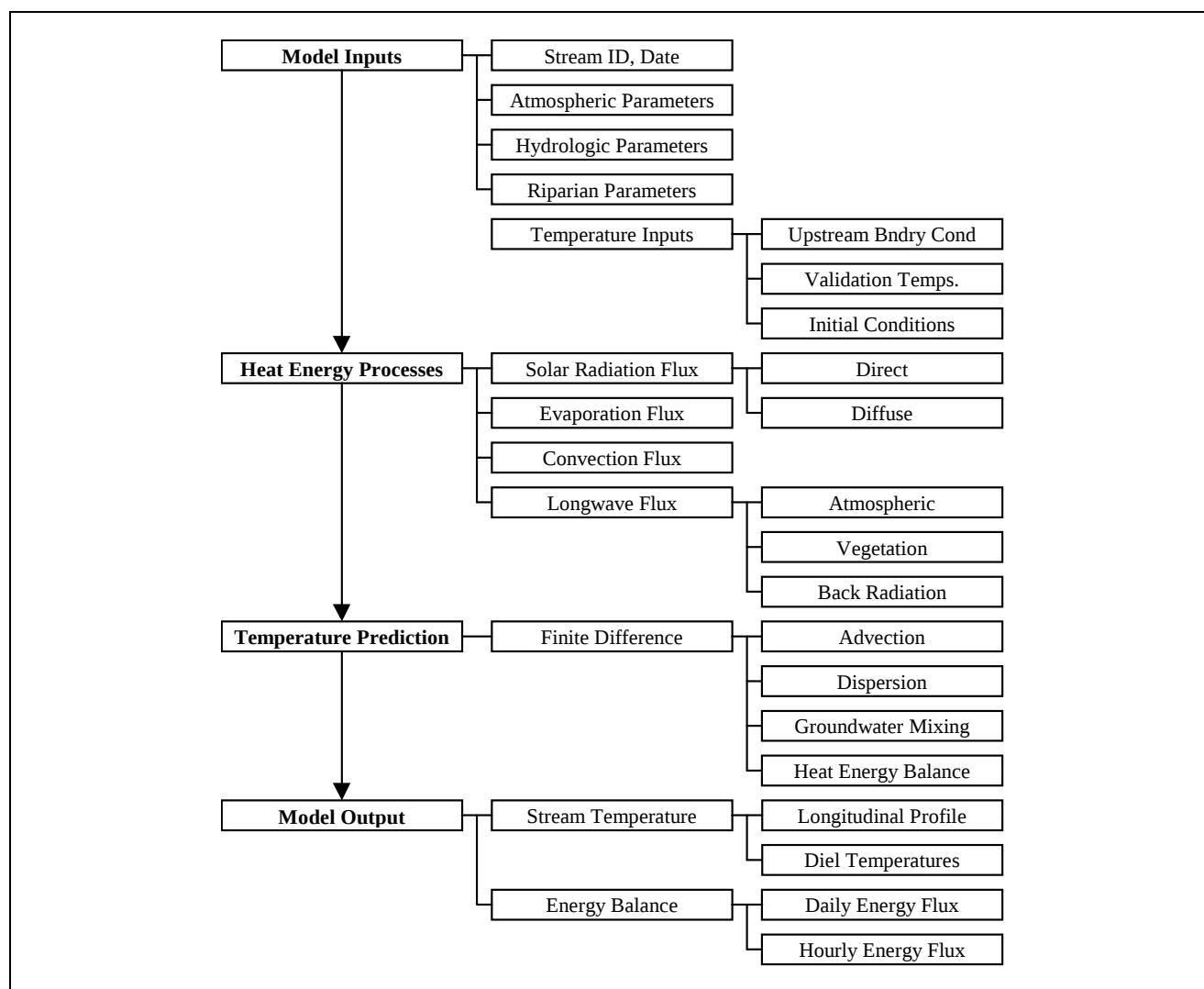
Figure C- 1: Heat source temperature model flow chart.
