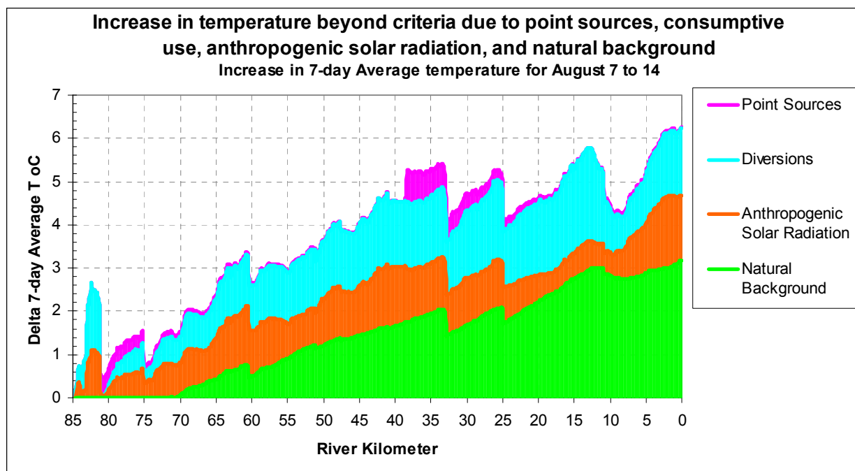
Figure A- 77. Increase in 7-day average river temperature above biological criterion due to various categories
