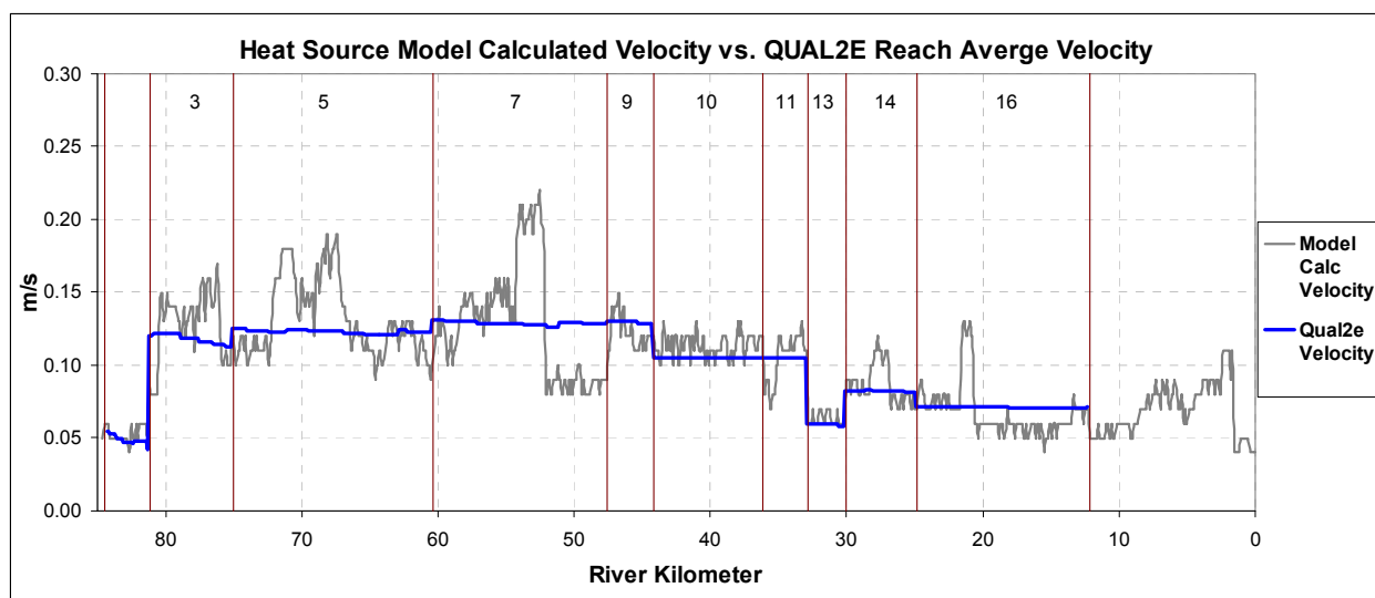
Figure A- 33. Pudding River model velocity calibration.
