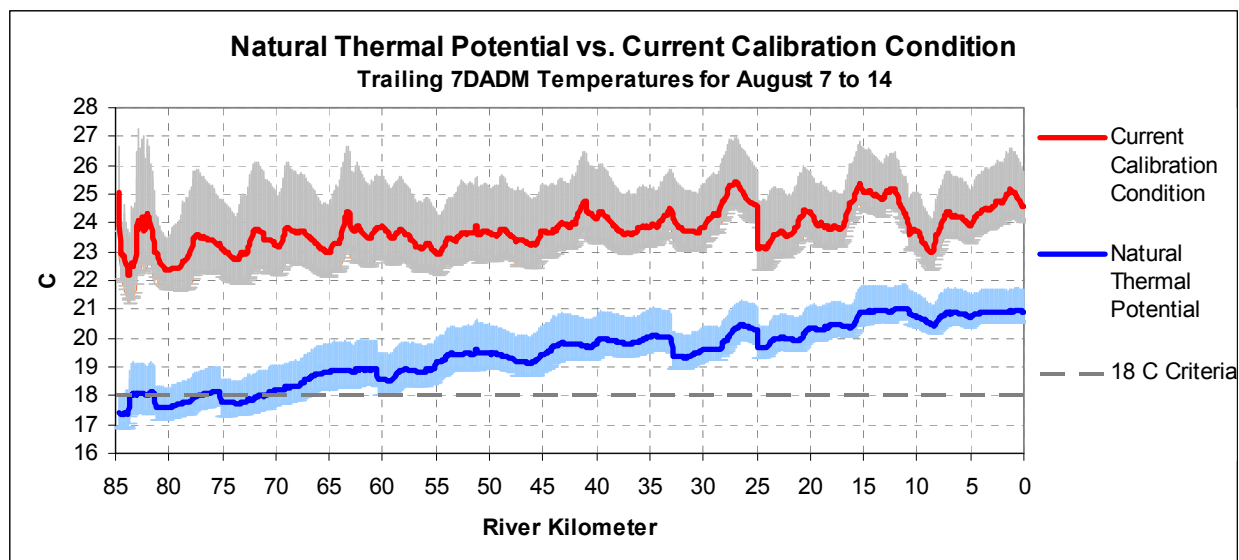
Figure A- 64: Natural thermal potential river temperatures
