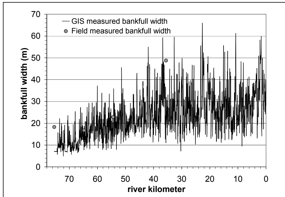
Figure A- 23: Remotely measured bankfull width and field measured bankfull width.
