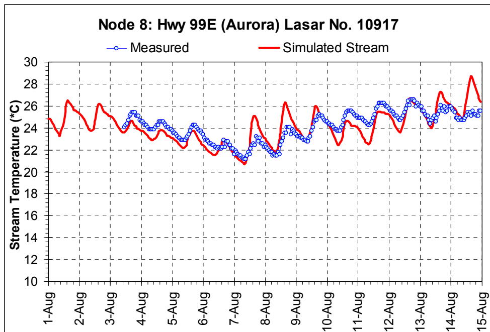
Figure A- 39: Model calculated vs. observed hourly temperatures – river km 12.4 (river mile 7.7).
