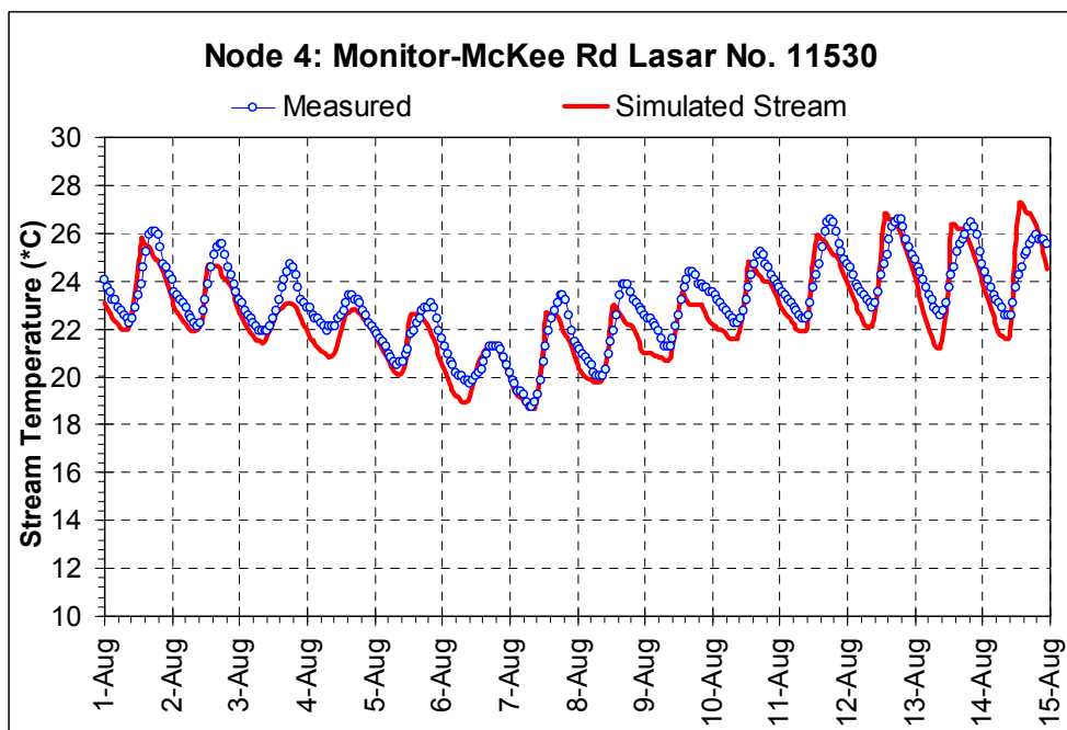
Figure A- 36: Model calculated vs. observed hourly temperatures – river km 51.7 (river mile 32.1).
