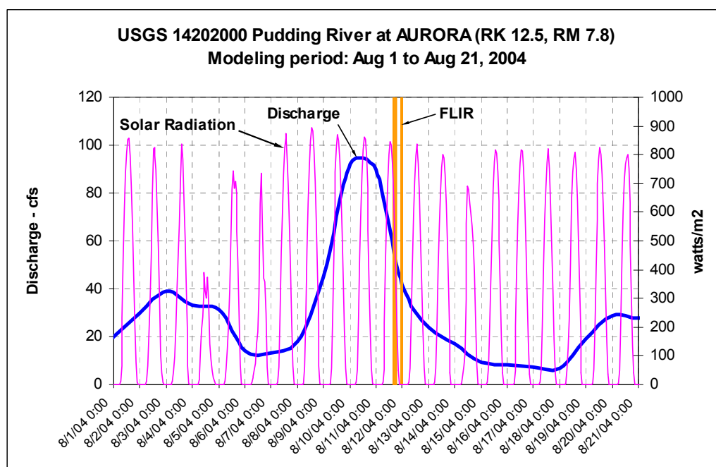
Figure A- 25. Pudding River discharge and solar radiation at USGS Gage at Aurora
