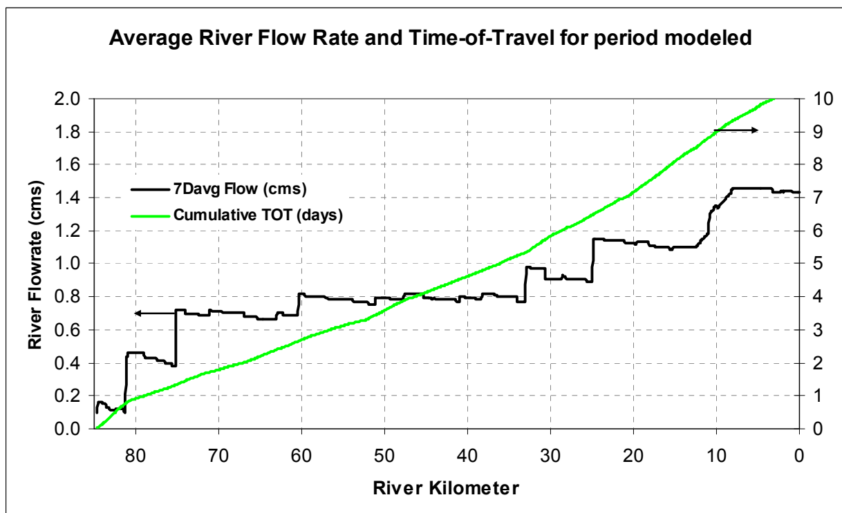
Figure A- 70. Average River flow rates and times-of-travel for August 1 to 14, 2004 calibration period
