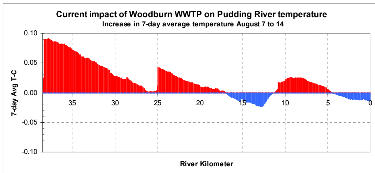
Figure A- 53: Current far-field impacts of Woodburn effluent on average river temperature.
