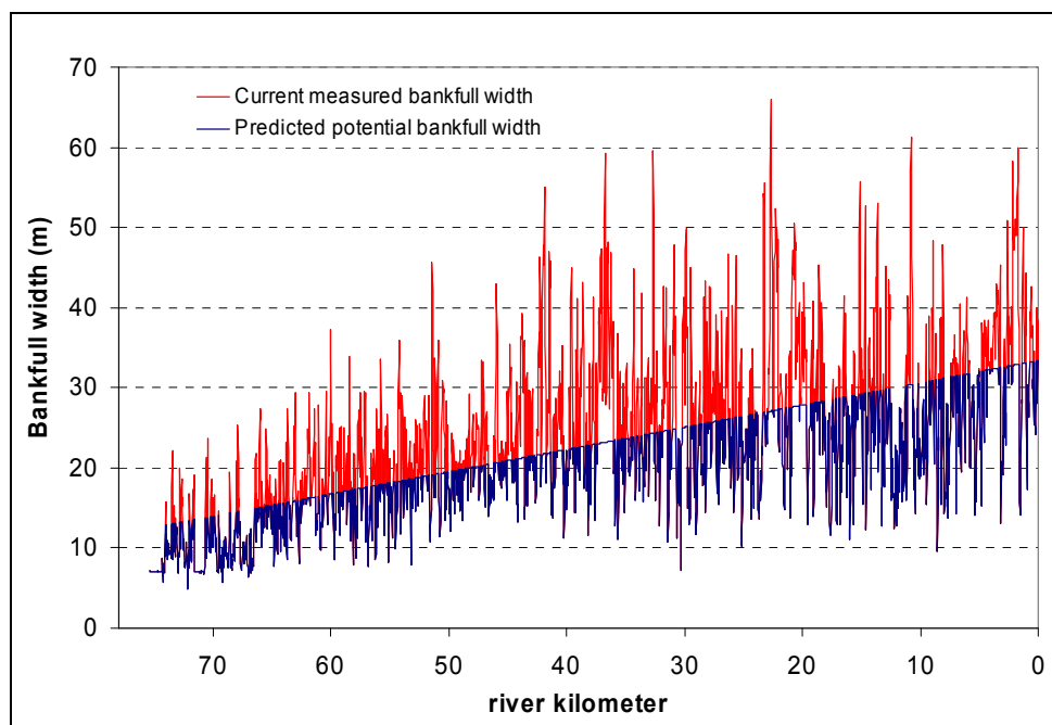
Figure A- 43: Current GIS measured bankfull width compared with predicted bankfull width.
