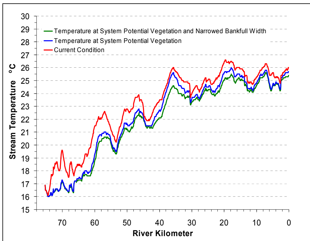
Figure A- 44: Predicted Molalla River stream temperatures resulting from a simulated narrowing of the Molalla River channel bankfull width.
