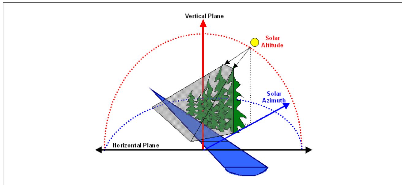
Figure A- 6: Effective shade defined.
