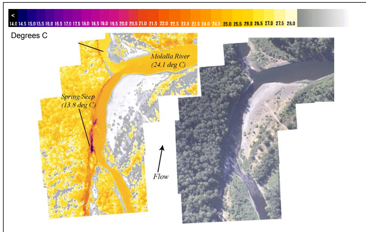
Figure A- 2: TIR/color video image pair showing the location of a spring or seep near the confluence of the Molalla and Pudding Rivers, July 26, 2004.
