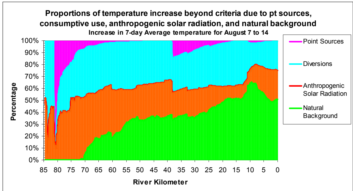
Figure A- 78. Proportions of 7-day average river temperature increase above biological criterion due to various categories
