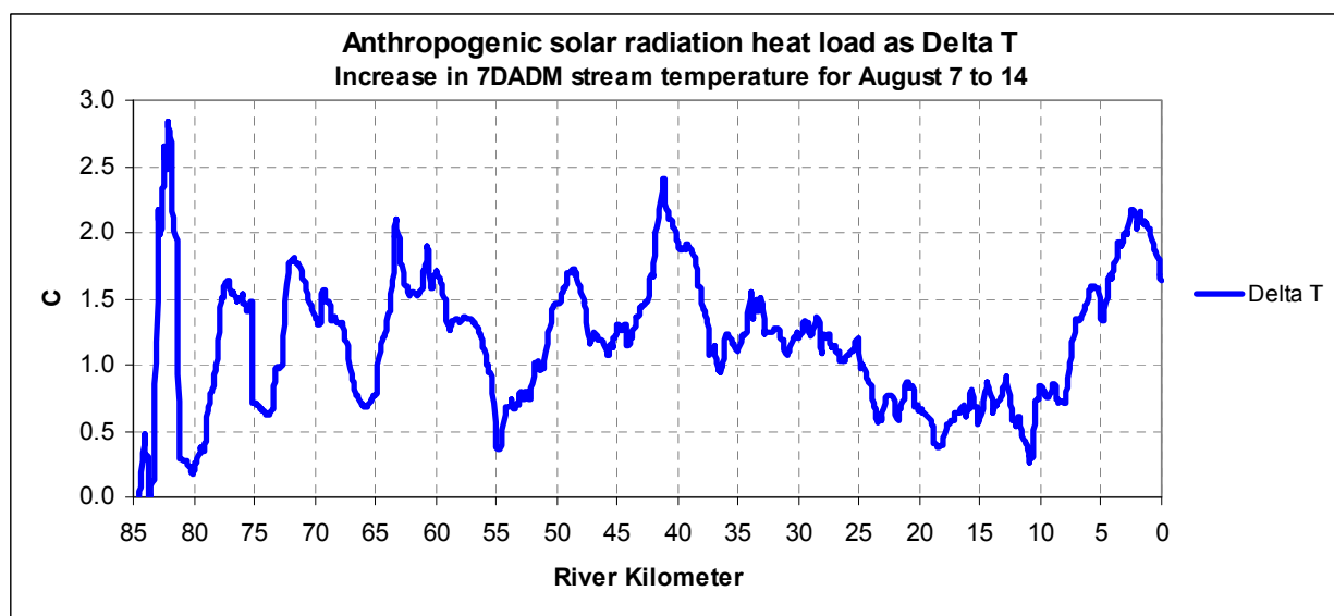
Figure A- 56: Impact on stream temperature of anthropogenic heat load.
