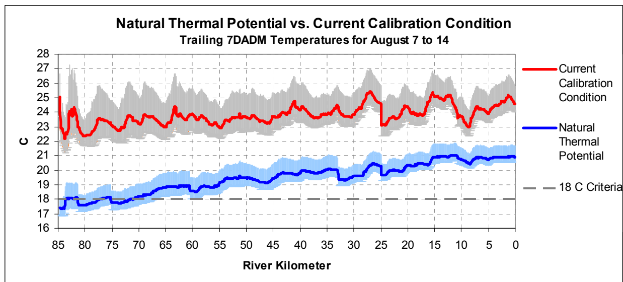
Figure A- 74: Model calculated natural thermal potential 7DADM Temperatures
