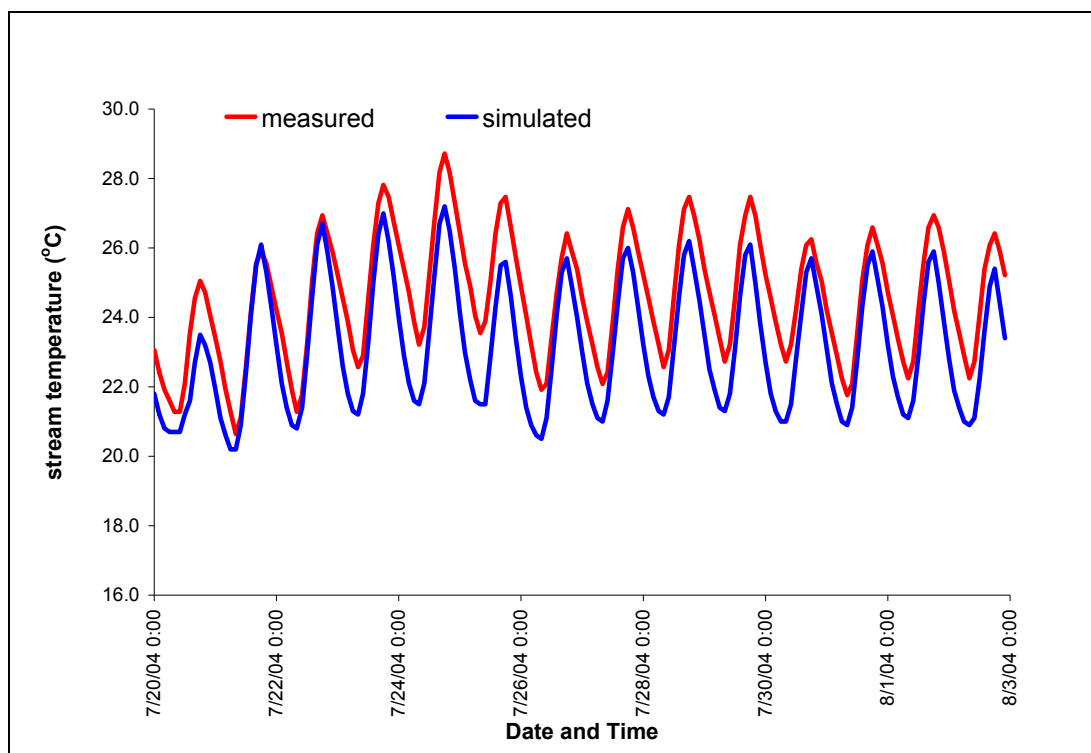
Figure A- 15: Continuous temperature measured and simulated at Molalla River upstream of Milk Creek, river kilometer 13.6 (8.5 river miles).
