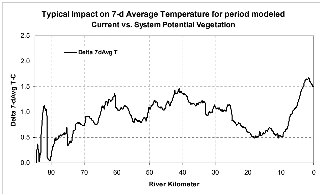
Figure A- 72. Effect of anthropogenic solar radiation on 7-day average stream temperature.
