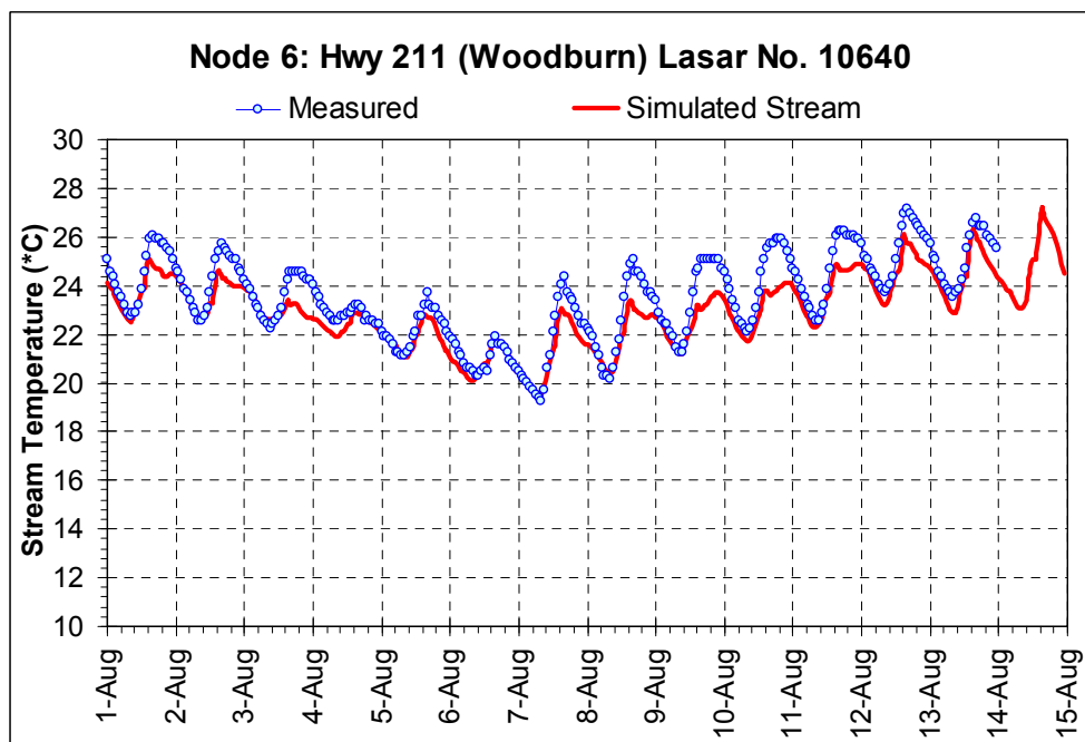
Figure A- 38: Model calculated vs. observed hourly temperatures – river km 36.2 (river mile 22.5).
