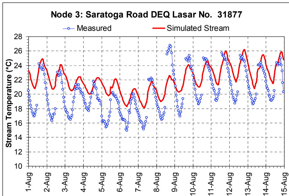
Figure A- 35: Model calculated vs. observed hourly temperatures – river km 66.3 (river mile 41.2).
