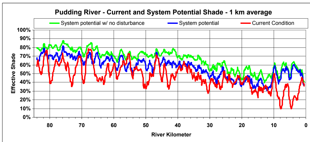
Figure A- 57: Current, system potential, and system potential without disturbance shade levels
