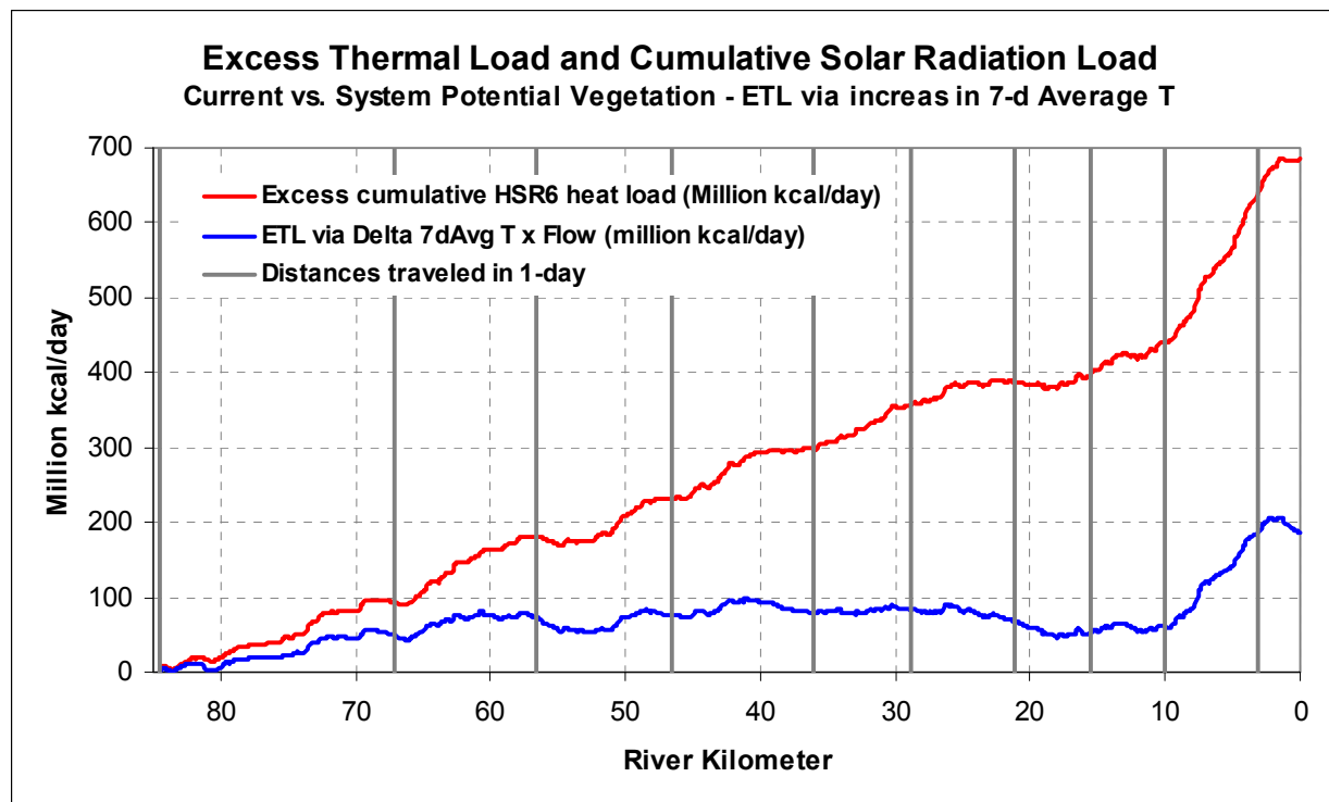
Figure A- 73. Cumulative solar radiation load and excess thermal load based on daily average temperatures.
