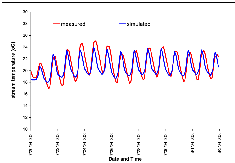
Figure A- 12: Continuous temperature measured and simulated at Molalla River upstream of North Fork Molalla River, river kilometer 45 (28 river miles).
