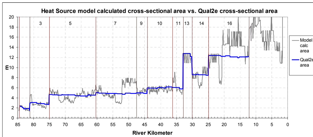
Figure A- 32. Pudding River model cross-sectional area calibration.
