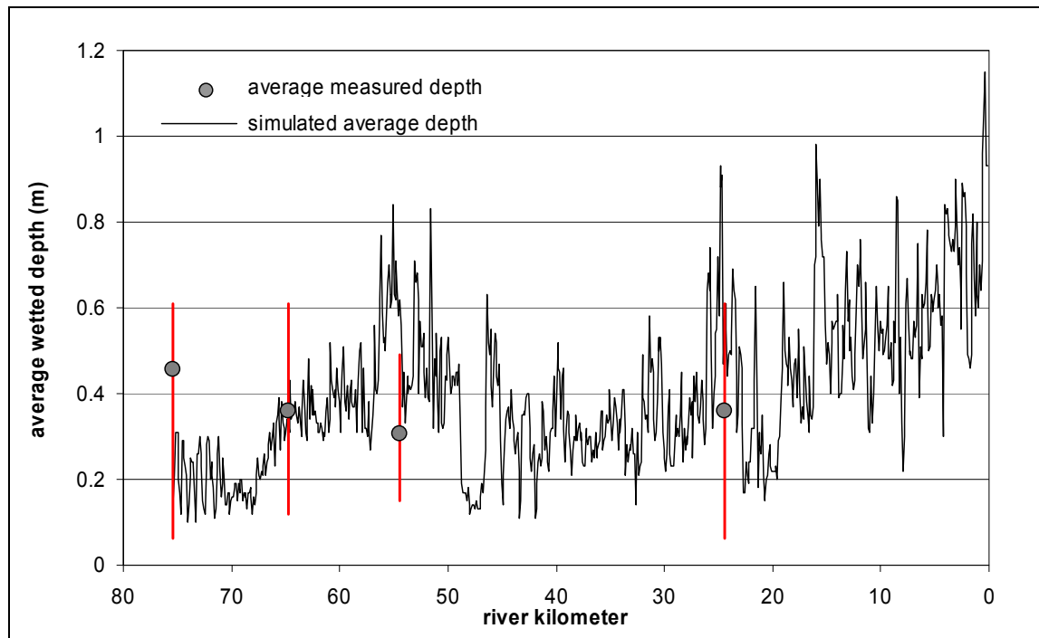
Figure A- 21: Simulated Molalla River wetted depth and average depth measurements.
