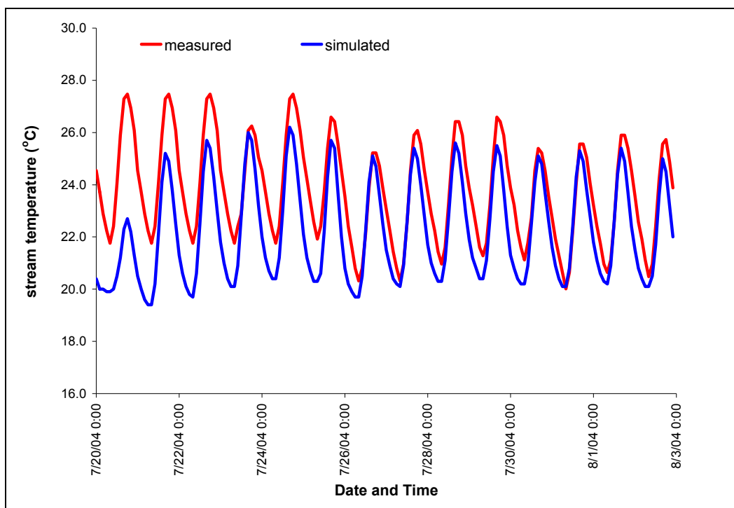
Figure A- 13: Continuous temperature measured and simulated at Molalla River at Highway 213, river kilometer 24.4 (15.2 river miles).
