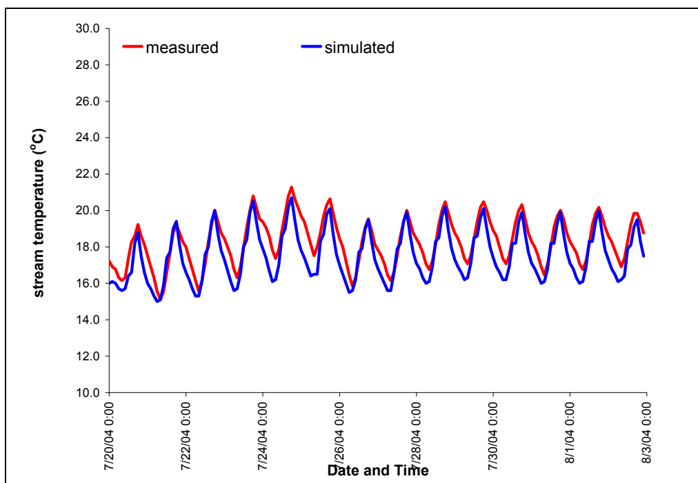
Figure A- 10: Continuous temperature measured and simulated at Molalla River upstream of Horse Creek, river kilometer 64.8 (40.3 river miles).
