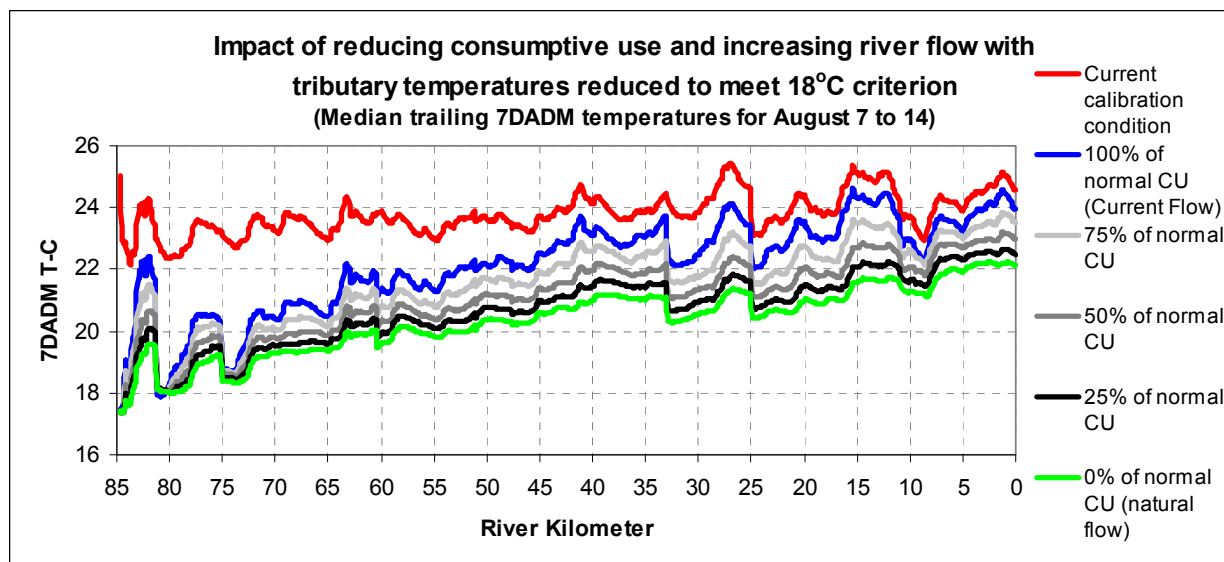
Figure A- 63. Impact on temperature of reducing CU (with tributary temperatures reduced to meet 18° criterion).
