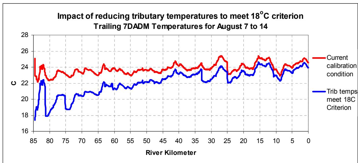
Figure A- 60: Impact of reducing tributary temperatures enough to meet 18^{\circ}\text{C} biological criterion.
