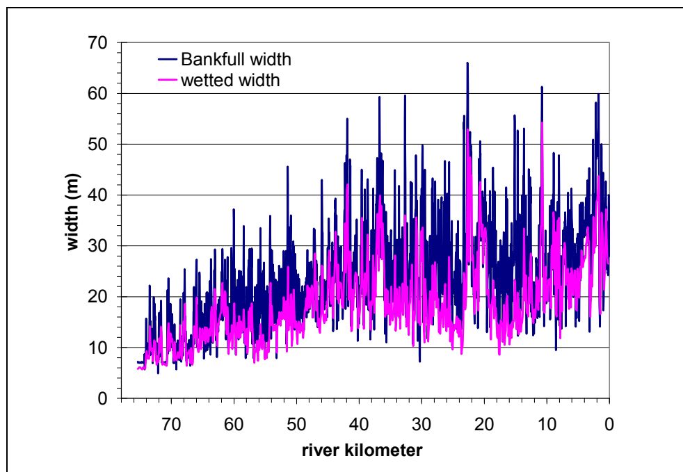
Figure A- 24: Comparison of bankfull width and simulated wetted width of the Molalla River
