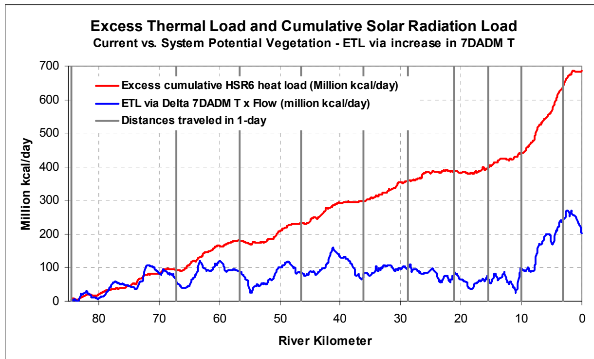
Figure A- 67. Cumulative solar radiation load vs. excess thermal load based on daily max temperatures.
