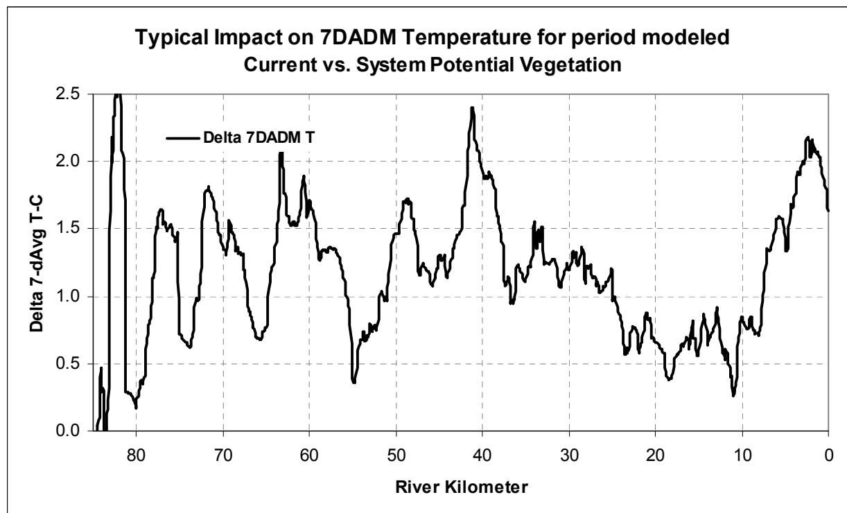
Figure A- 69. Effect of anthropogenic solar radiation on 7DADM stream temperature.
