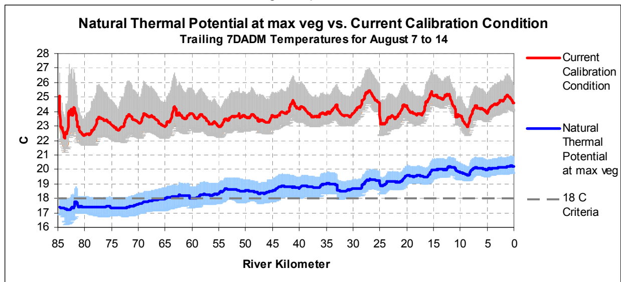
Figure A- 65: River temperatures for natural thermal potential scenario with vegetation at maximum levels.
