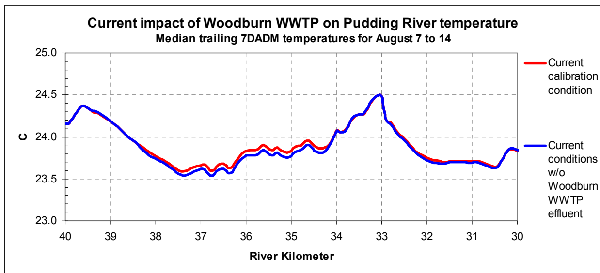
Figure A- 48: Increase in river temperature due to Woodburn WWTP.
