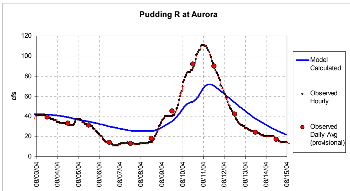
Figure A- 28: Model flow calibration, Pudding R at Aurora, river km 13 (river mile 8.1).
