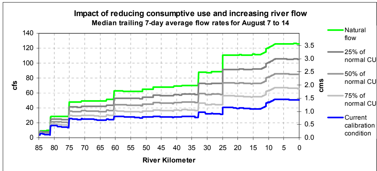
Figure A- 61: Flow rates for five consumptive use scenarios
