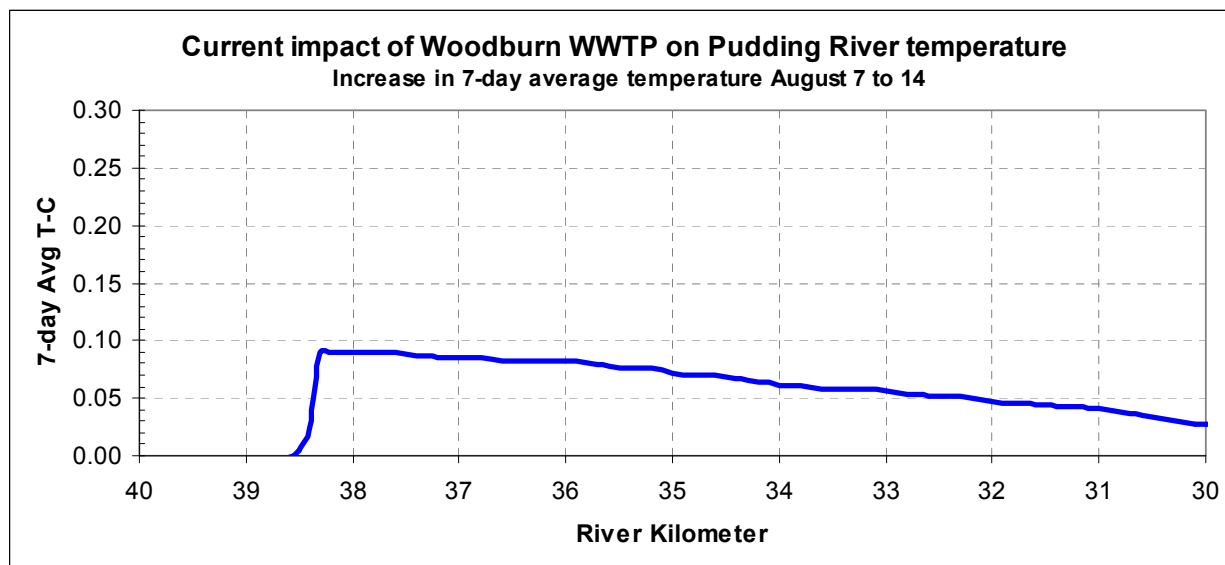
Figure A- 52: Current increase in average river temperature due to Woodburn WWTP.
