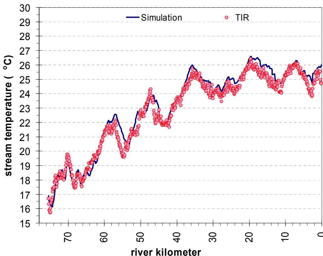
Figure A- 8: Thermal Infrared Radiometry measured temperature compared with model simulated temperature. Periodic temperature decreases may indicate the influence of cooler tributaries, springs, seeps, and groundwater interaction.
