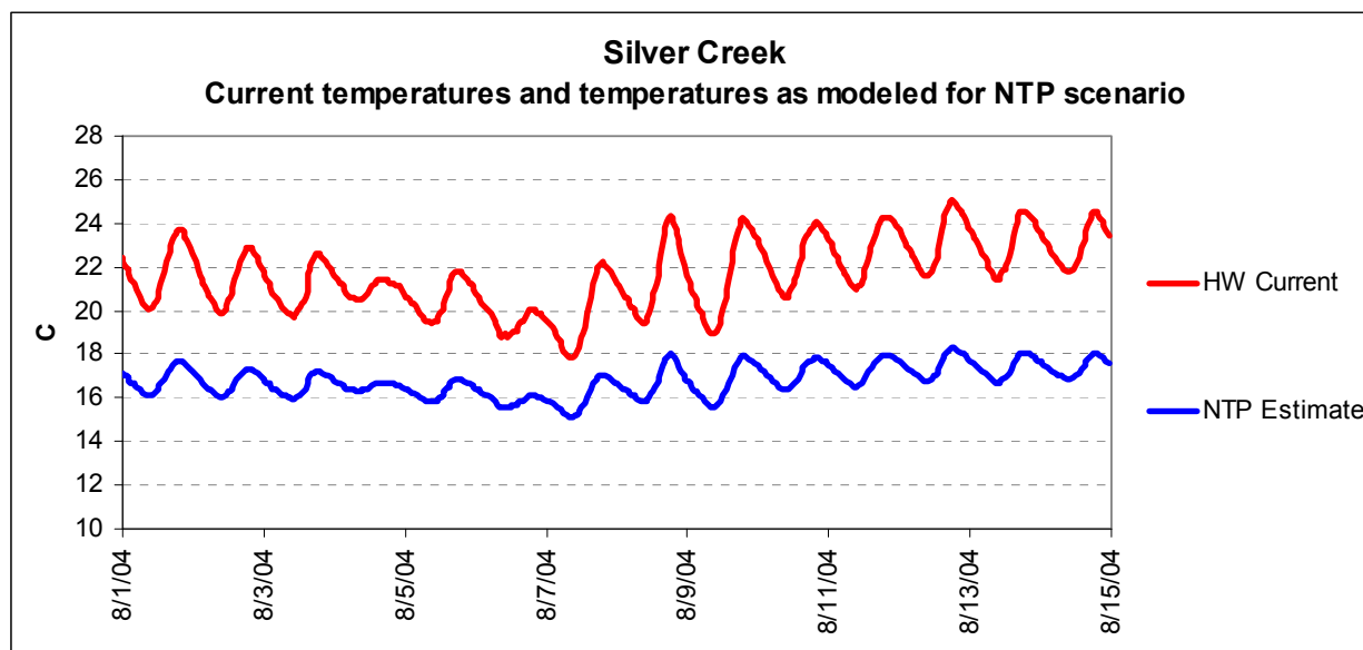
Figure A- 59: Theoretical tributary temperatures that meet the 18^{\circ}\text{C} biological criterion.
