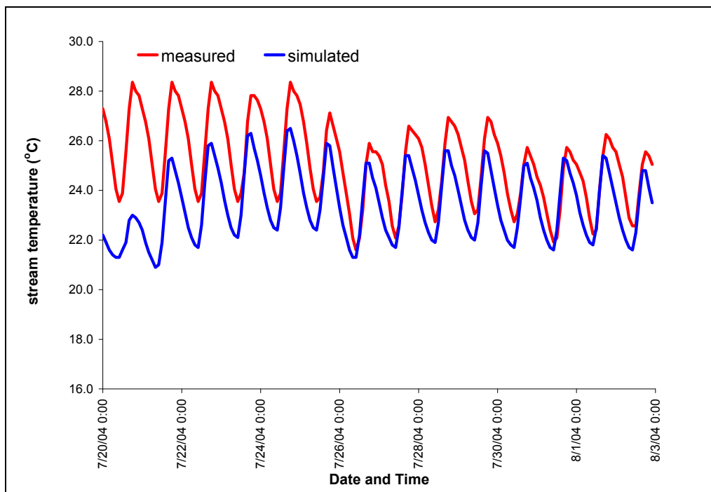
Figure A- 18: Continuous temperature measured and simulated at Molalla River at 22 nd , river kilometer 3.2 (2 river miles).
