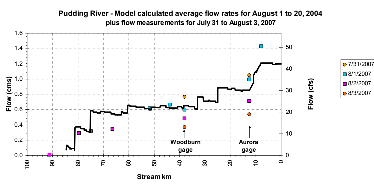
Figure A- 29. Flow rates used for hydraulics calibration and comparisons to Pudding River QUAL2E model
