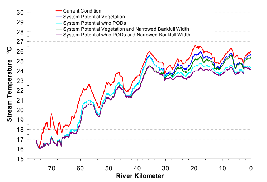
Figure A- 45: Predicted stream temperatures resulting from a simulated narrowing of the Molalla River channel bankfull width, system potential vegetation, and natural stream flows.
