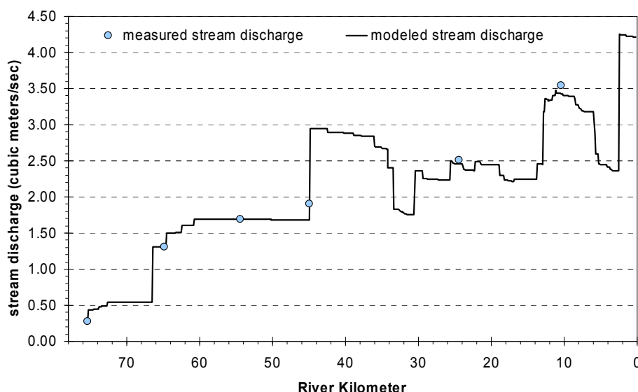
Figure A- 20: Modeled and measured stream discharge on the Molalla River. Stream discharge measurements were collected on July 20 and 22, 2004. The model simulates stream discharge on July 26.
