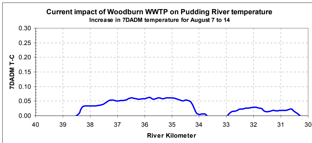
Figure A- 49: Current increase in daily maximum river temperature due to Woodburn WWTP.
