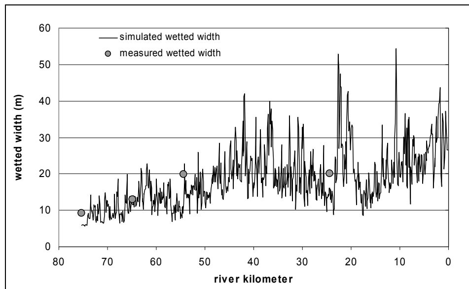
Figure A- 22: Simulated Molalla River wetted width and wetted width measurements.
