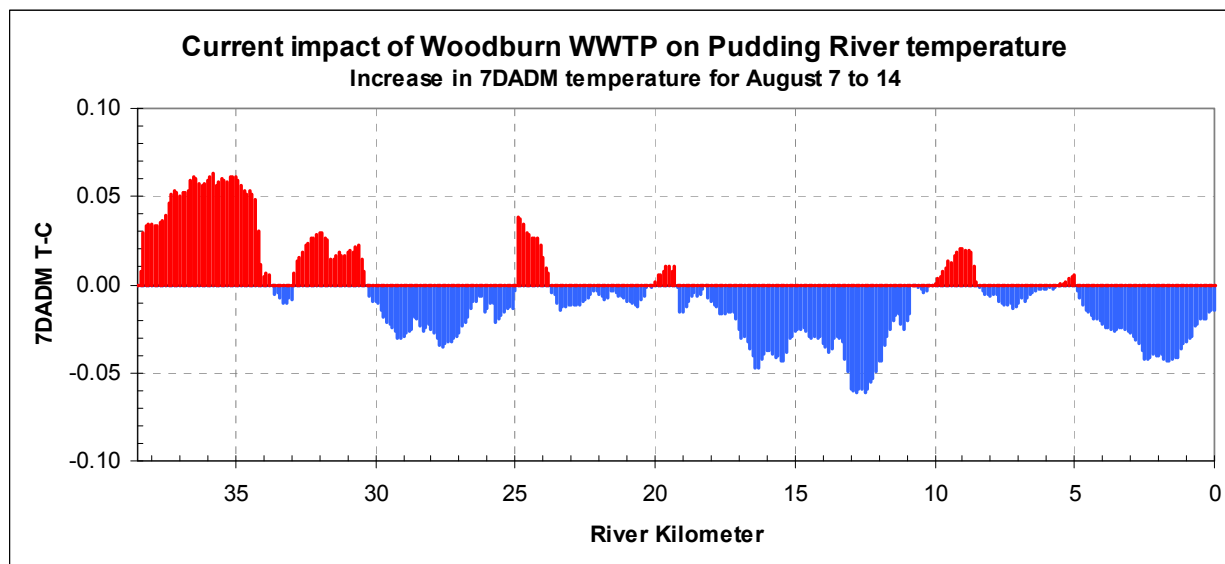
Figure A- 51: Current far-field impacts of Woodburn effluent on daily maximum river temperature.
