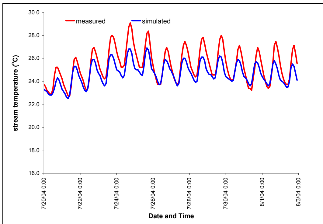
Figure A- 19: Continuous temperature measured and simulated at Molalla River at mouth, river kilometer 0.3 (0.2 river miles).
