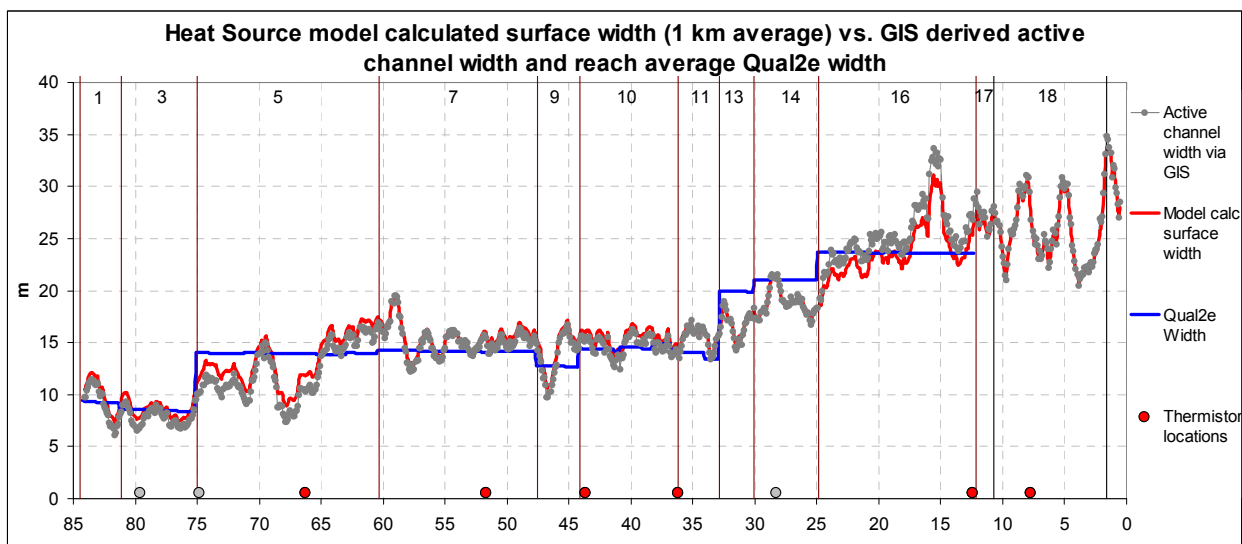
Figure A- 30. Pudding River model width calibration.
