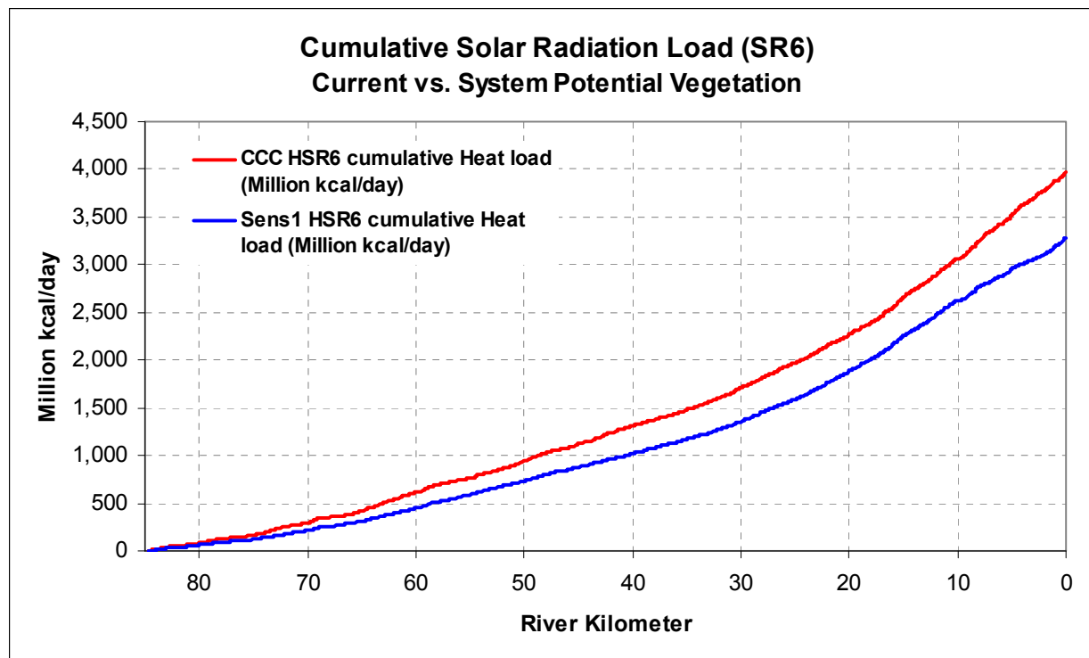
Figure A- 66. Cumulative solar radiation load for current and system potential shade conditions.
