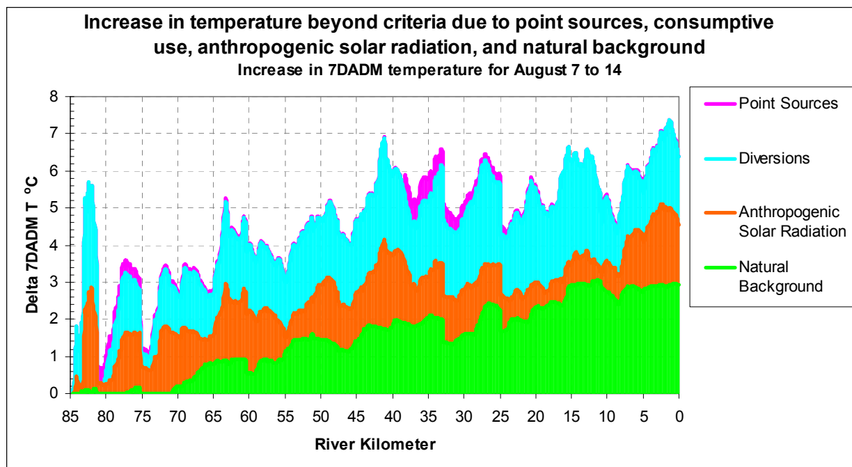
Figure A- 75. Increase in 7DADM river temperature above biological criterion due to various categories
