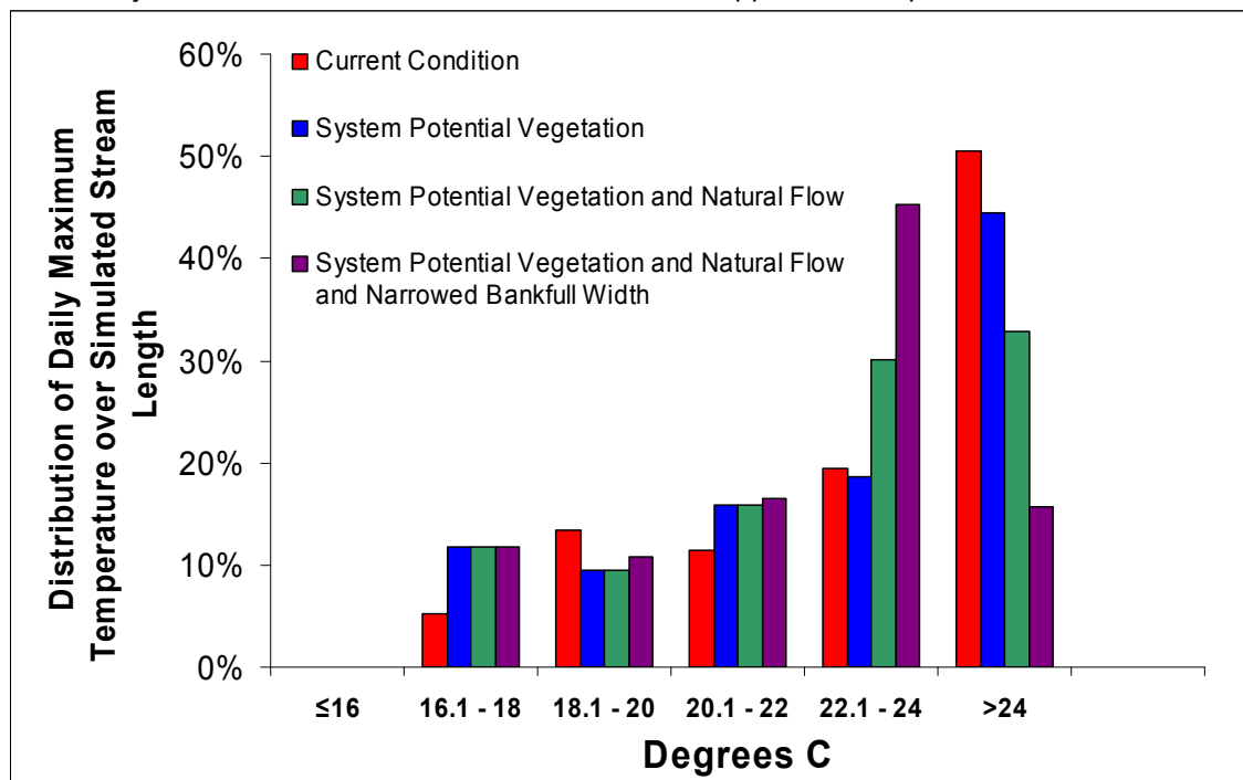
Figure A- 46: Molalla River distribution of maximum daily stream temperatures at current conditions, system potential vegetation, and system potential vegetation with natural flow. Natural flow was simulated by reducing all water withdrawals to zero.
