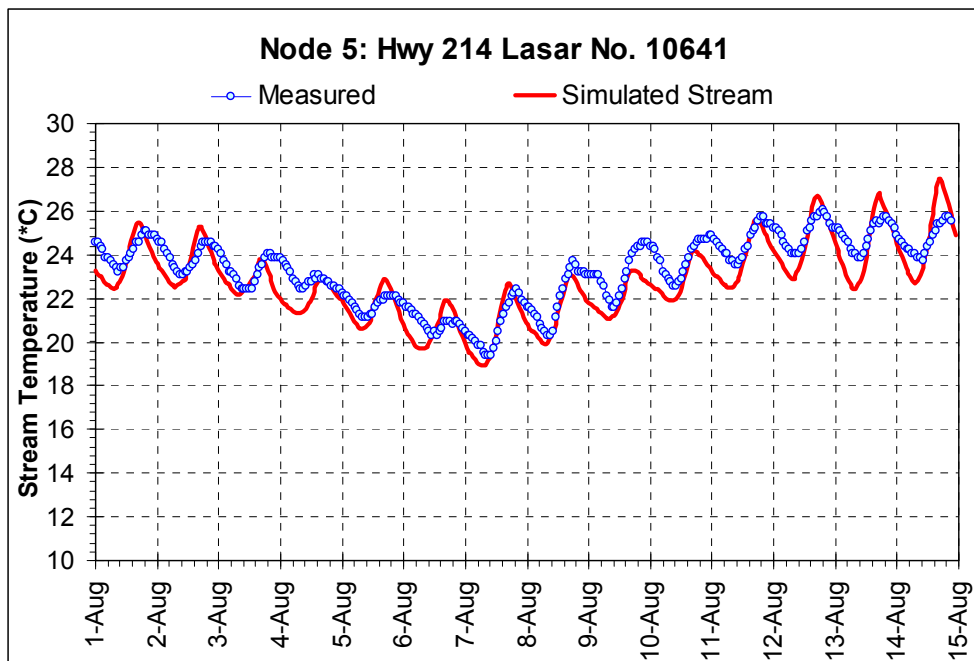
Figure A- 37: Model calculated vs. observed hourly temperatures – river km 43.7 (river mile 27.1)
