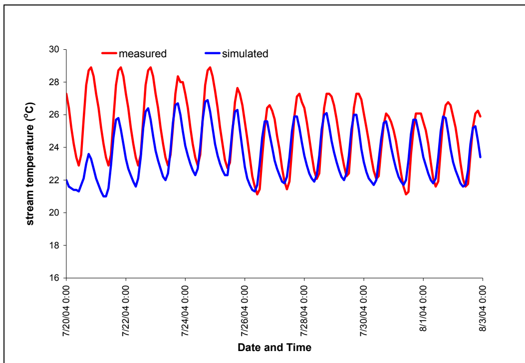
Figure A- 17: Continuous temperature measured and simulated at Molalla River at Knights Bridge Rd., river kilometer 4.8 (3 river miles).
