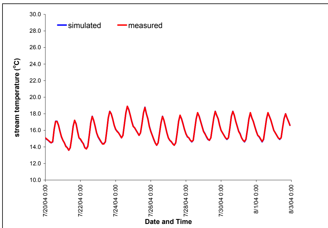
Figure A- 9: Continuous temperature measured and simulated at Molalla River at Locked Gate, river kilometer 75.4 (46.8 river miles).
