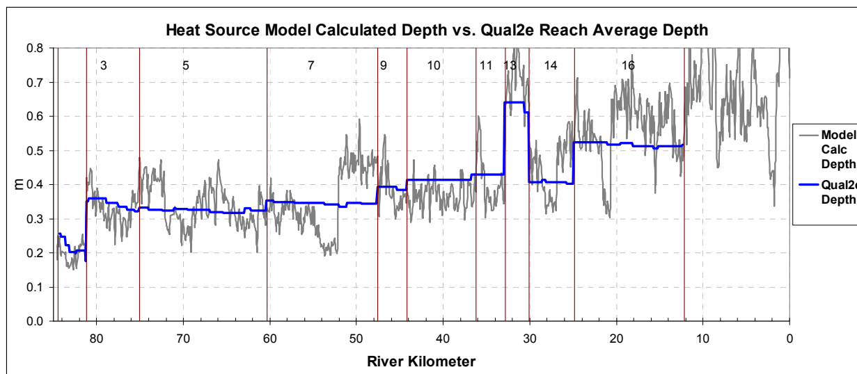
Figure A- 31. Pudding River model depth calibration.
