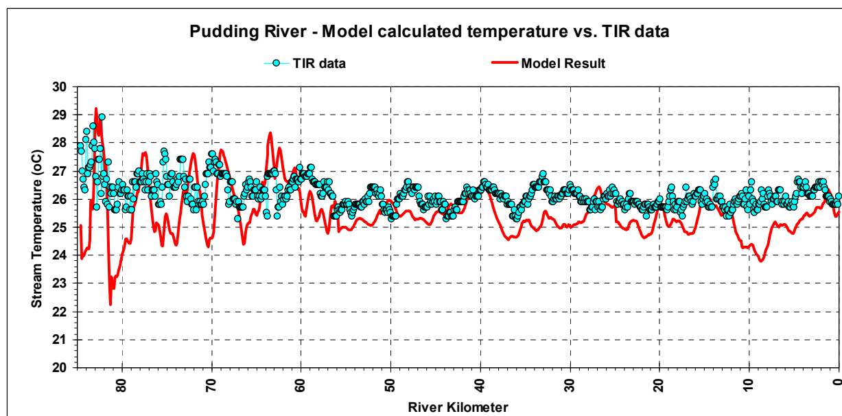
Figure A- 34: Pudding River model temperature calibration, TIR daily maximum temperatures for August 11 and 12.
