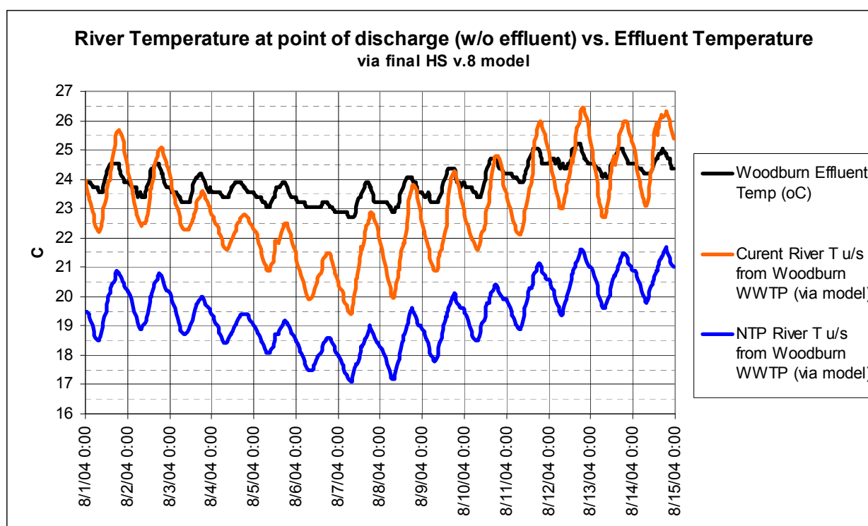
Figure A- 50: Woodburn effluent temperature relative to current and NTP river temperature.
