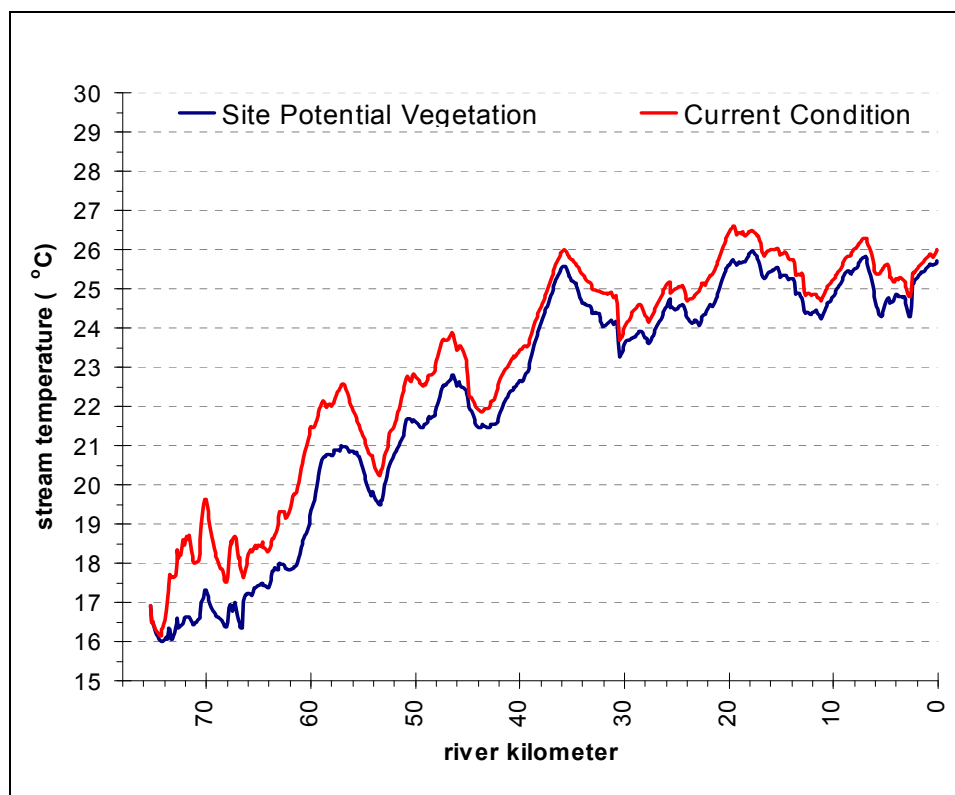
Figure A- 41: Simulated Molalla River temperature decrease resulting from system potential vegetation shading. Upland forest coverage is simulated in the upper half of the watershed and mixed forest/savannah/prairie in the lower half of the watershed.
