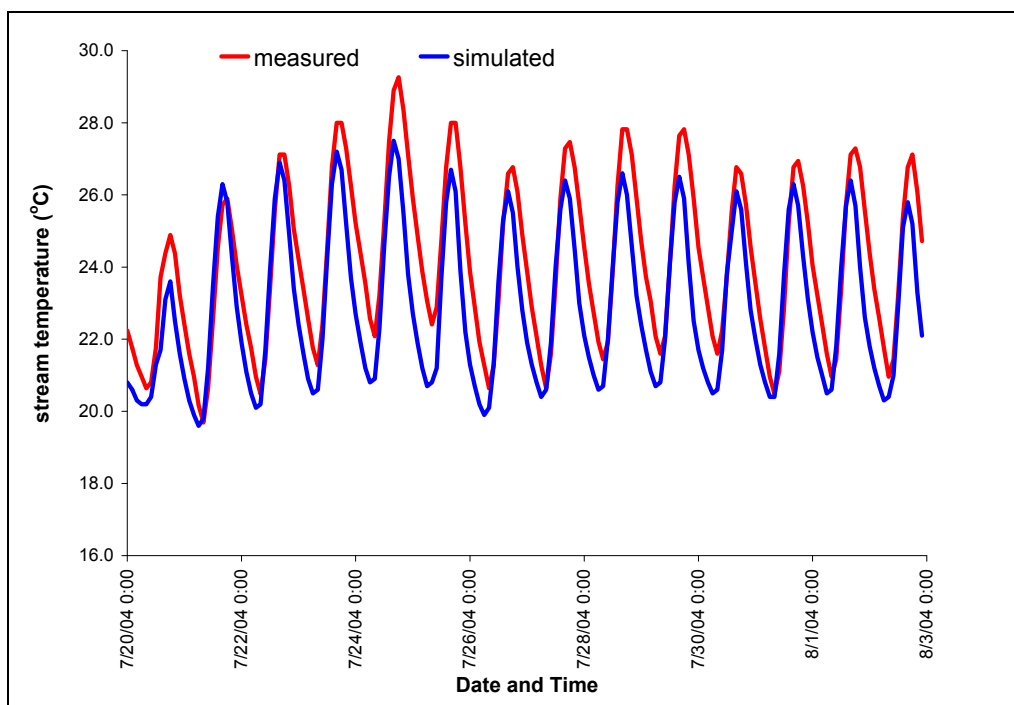
Figure A- 14: Continuous temperature measured and simulated at Molalla River at Kraxberger Rd., river kilometer 20.5 (12.7 river miles).
