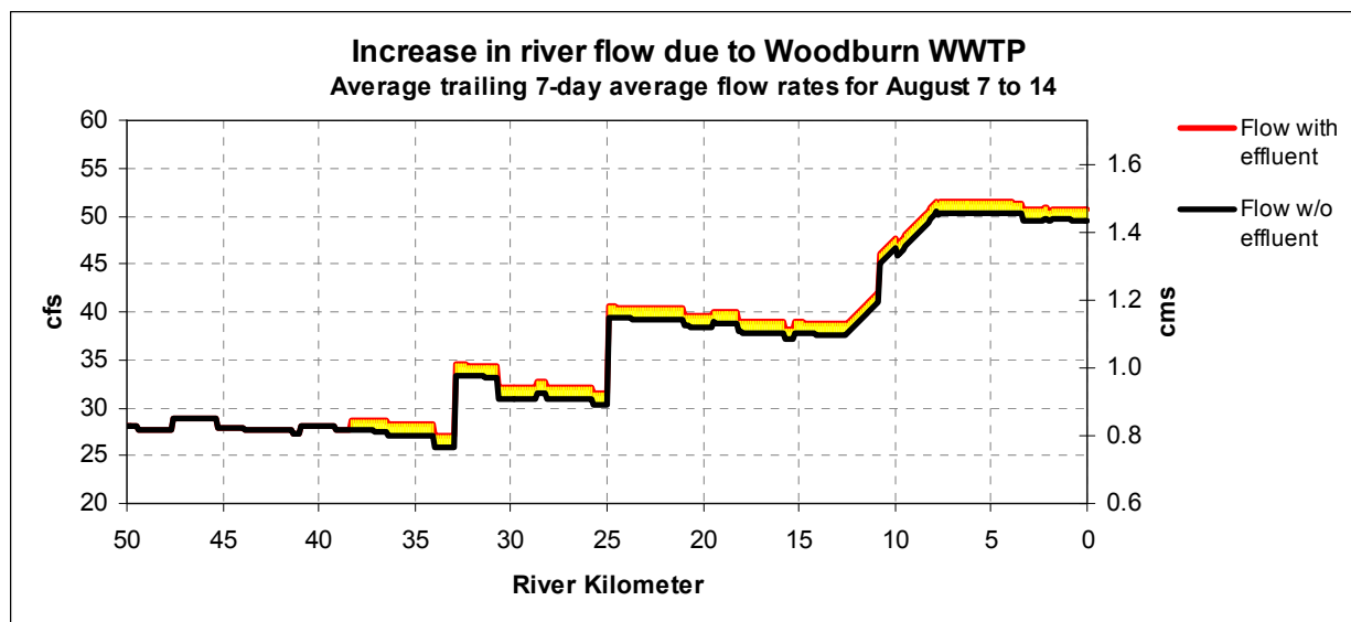
Figure A- 47: Increase in river flow due to Woodburn WWTP
