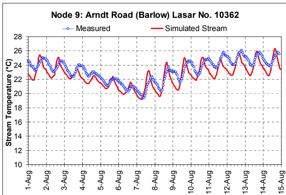
Figure A- 40: Model calculated vs. observed hourly temperatures – river km 7.7 (river mile 4.8).
