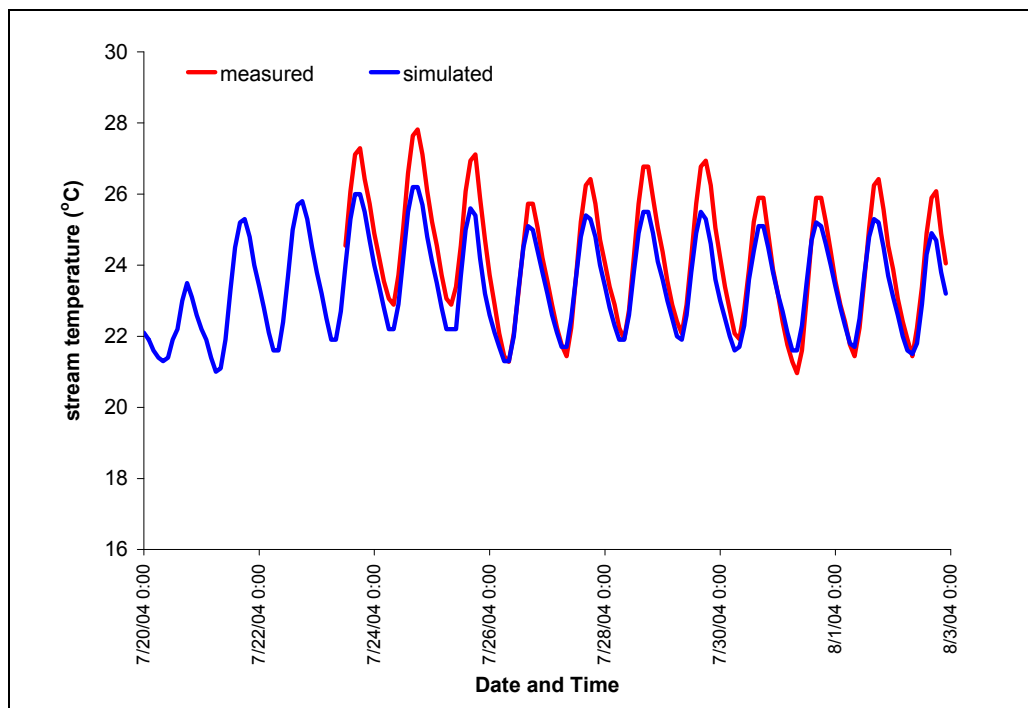
Figure A- 16: Continuous temperature measured and simulated at Molalla River at Goods Bridge, river kilometer 10.4 (6.5 river miles).
