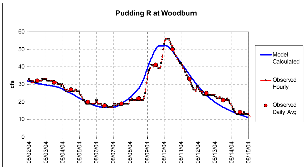
Figure A- 27. Model flow calibration, Pudding River near Woodburn, river km 37.5 (river mile 23.3).
