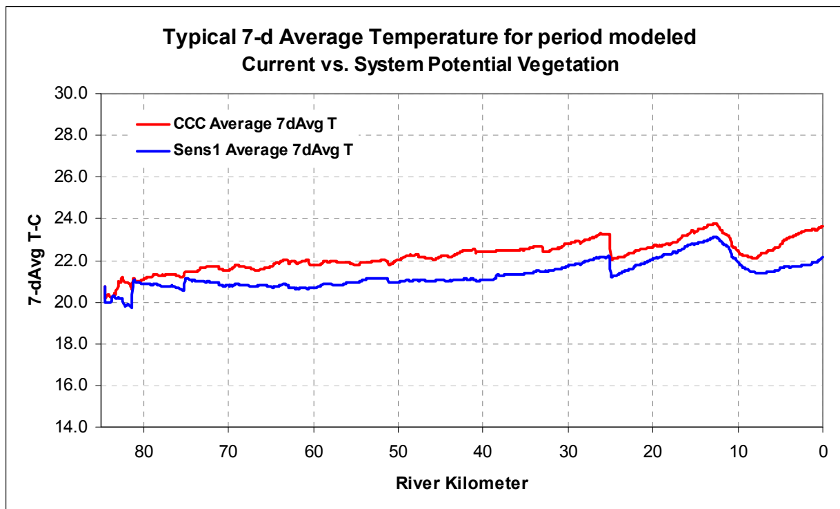
Figure A- 71. Model calculated 7-day average temperature for current and system potential vegetation.
