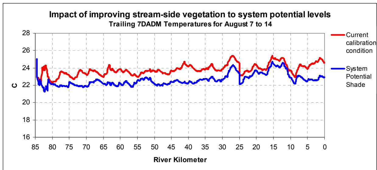
Figure A- 55: Impact on temperature of improving riparian vegetation to system potential levels
