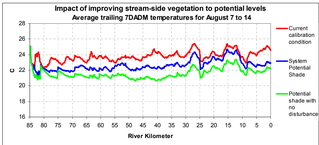
Figure A- 58. Impact of improving riparian vegetation to system potential levels with and without disturbance
