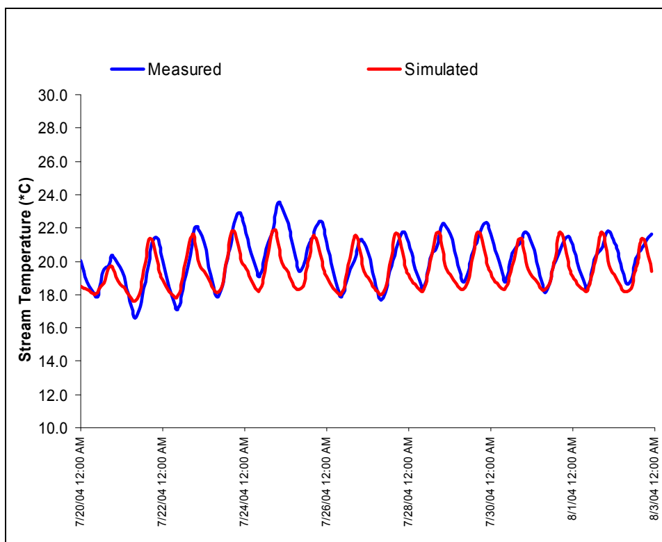
Figure A- 11: Continuous temperature measured and simulated at Molalla River upstream of Pine Creek, river kilometer 54.4 (33.8 river miles).
