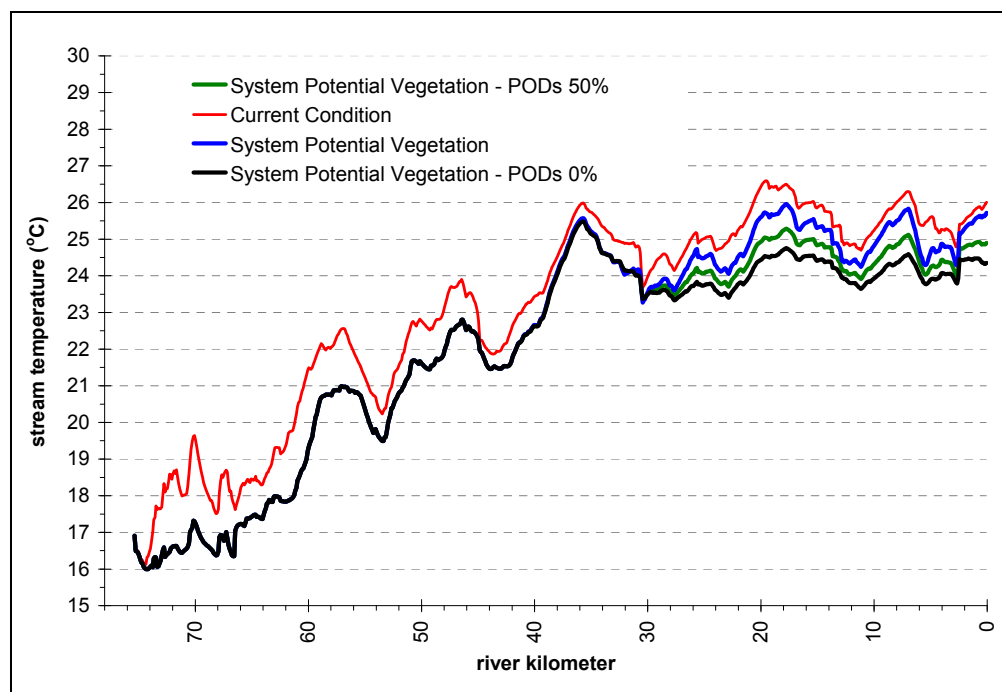
Figure A- 42: Simulated Molalla River temperature decrease from reducing surface water withdrawals. System potential vegetation modeled as upland forest in the upper half of the Molalla River watershed and mixed forest/savannah/prairie in the lower half.
