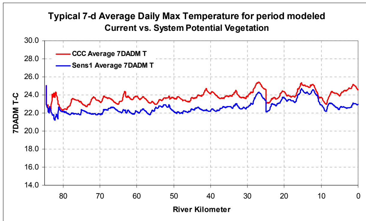
Figure A- 68. Model calculated 7DADM temperature for current and system potential vegetation.
