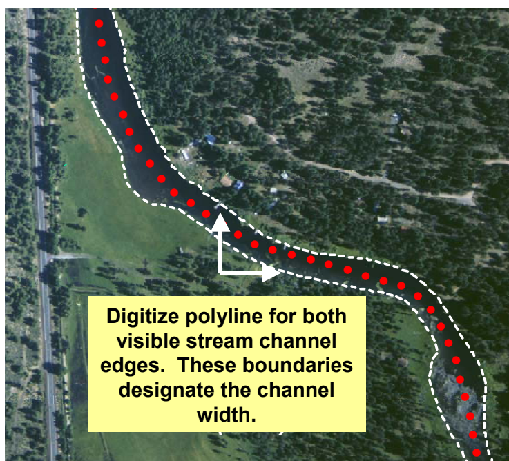
Figure A- 4: Example of digitized channel width from 1:5000 digital ortho quad aerial photograph.
