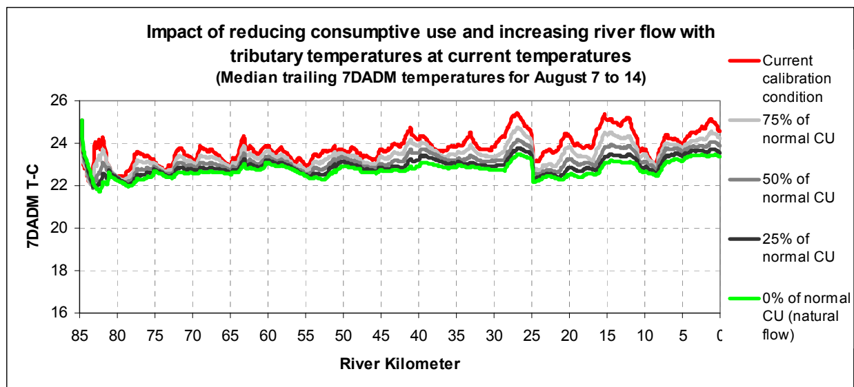
Figure A- 62. Impact on temperature of reducing consumptive use (with no change in tributary temperatures).
