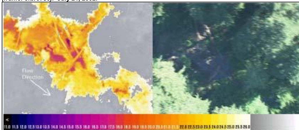
Figure 13.3 TIR/color video image pair showing a spring (14.2°C) along the left bank of Big River (17.2°C) at RM 6.6 (frame: cibr0730). July 21, 2002.
