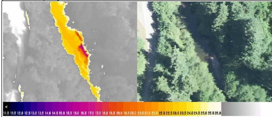
Figure 13.8 TIR/color video image showing Mosby Creek (22.4°C) at RM 12.4. The flow direction is from the top to bottom of the image. A possible spring (16.1°C) is visible along the LB (looking downstream). Although visible shadows make classification difficult, the location has visible surface water and is considerably cooler than other shadowed areas (frame: mos0699). July 21, 2002.
