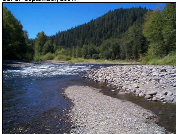
Figure 12.3 Middle Fork Willamette River, upstream of Dexter Reservoir, at RM 53, shows lack of riparian vegetation and an increase in stream channel width. USFS. September, 2001.
