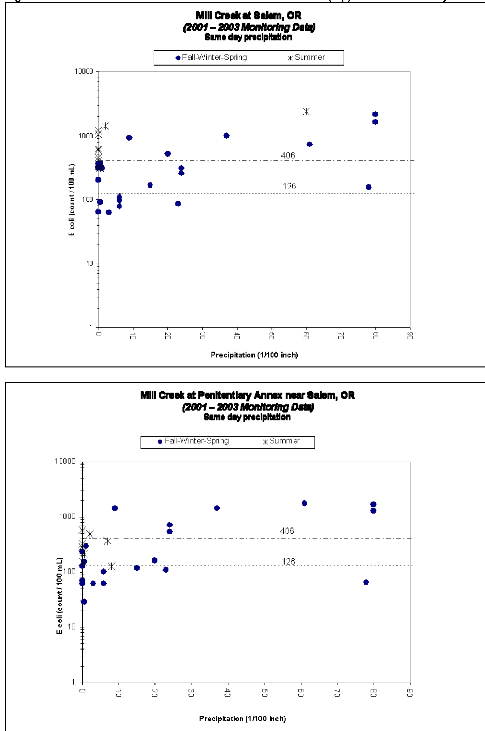
Figure 7.19 E. coli Concentrations on Mill Creek at Salem (top) and at Penitentiary Annex (bottom).
