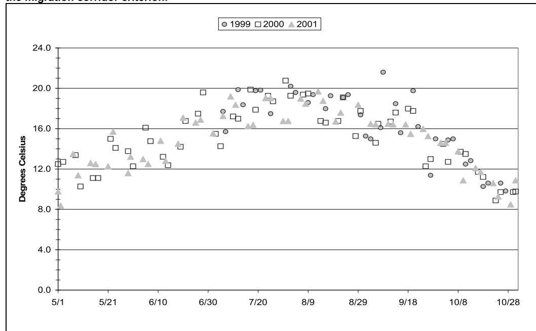
Figure 7.3 Rickreall Creek Summertime Daily Stream Temperatures, Upstream of Dallas STP, are typically below 20^{\circ}\text{C} , the migration corridor criterion.
