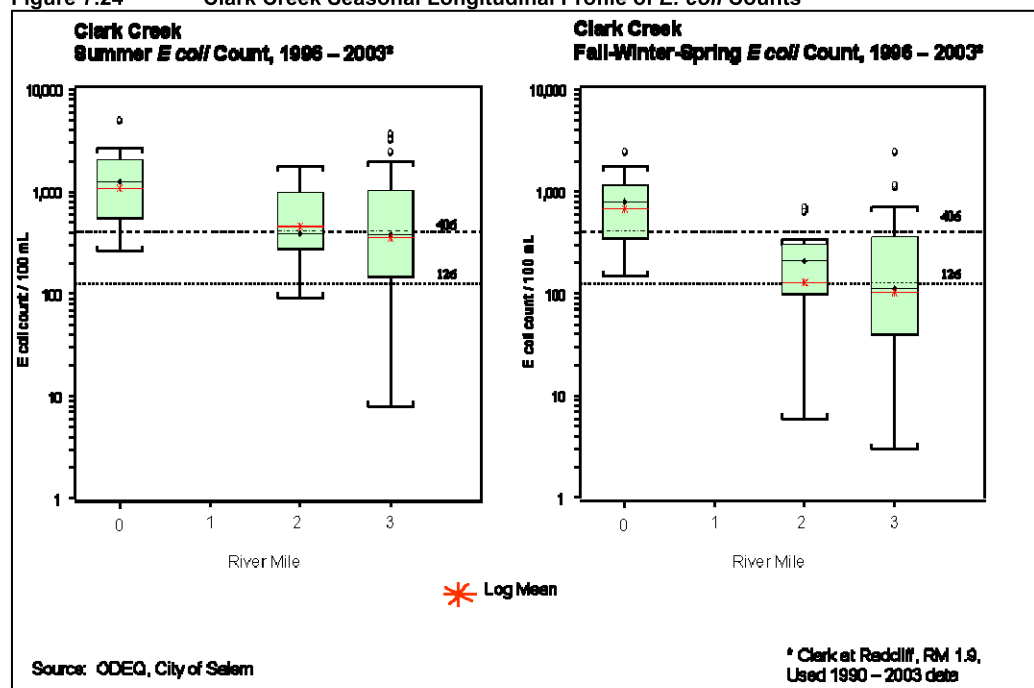
Figure 7.24 Clark Creek Seasonal Longitudinal Profile of E. coli Counts
