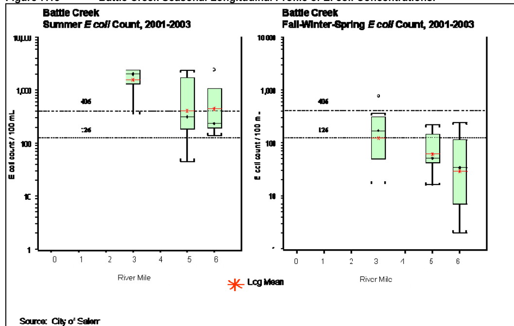
Figure 7.15 Battle Creek Seasonal Longitudinal Profile of E. coli Concentrations.
