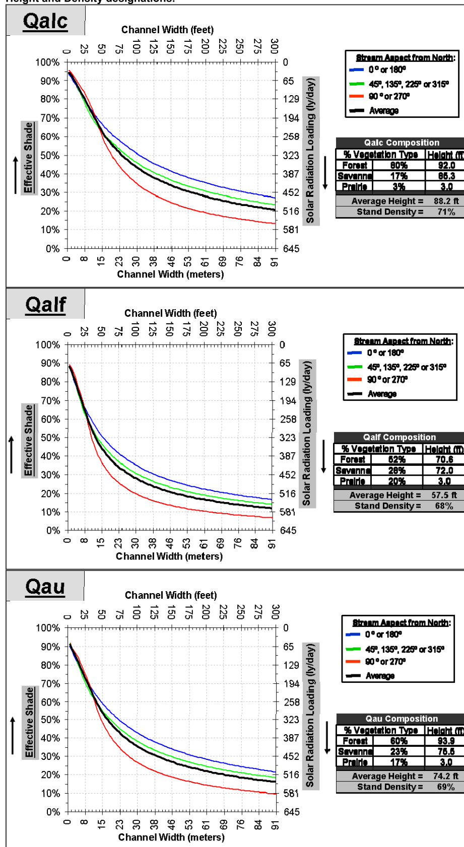
Figure 7.8 Shade Curves by Geomorphic Classifications that apply to the Middle Willamette Subbasin with vegetation Height and Density designations.
