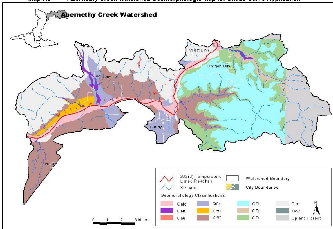
Map 7.8 Abernethy Creek Watershed Geomorphologic Map for Shade Curve Application
