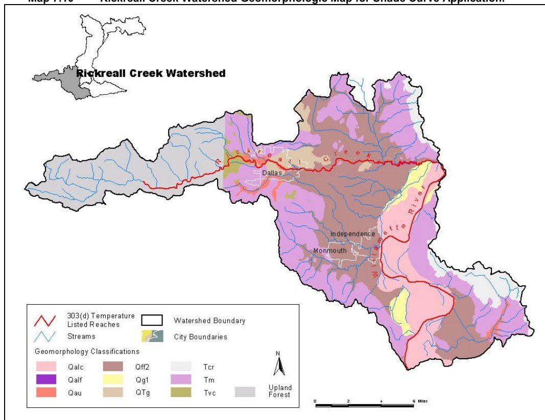
Map 7.10 Rickreall Creek Watershed Geomorphologic Map for Shade Curve Application.
