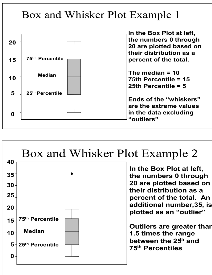
Figure 7.9 Two Box and Whisker Plot Examples.
