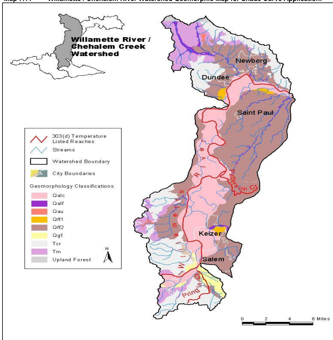
Map 7.11 Willamette / Chehalem River Watershed Geomorphic Map for Shade Curve Application.
