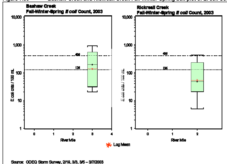
Figure 7.30 Bashaw Creek and Rickreall Creek Fall-Winter-Spring box plot of E. coli Counts
