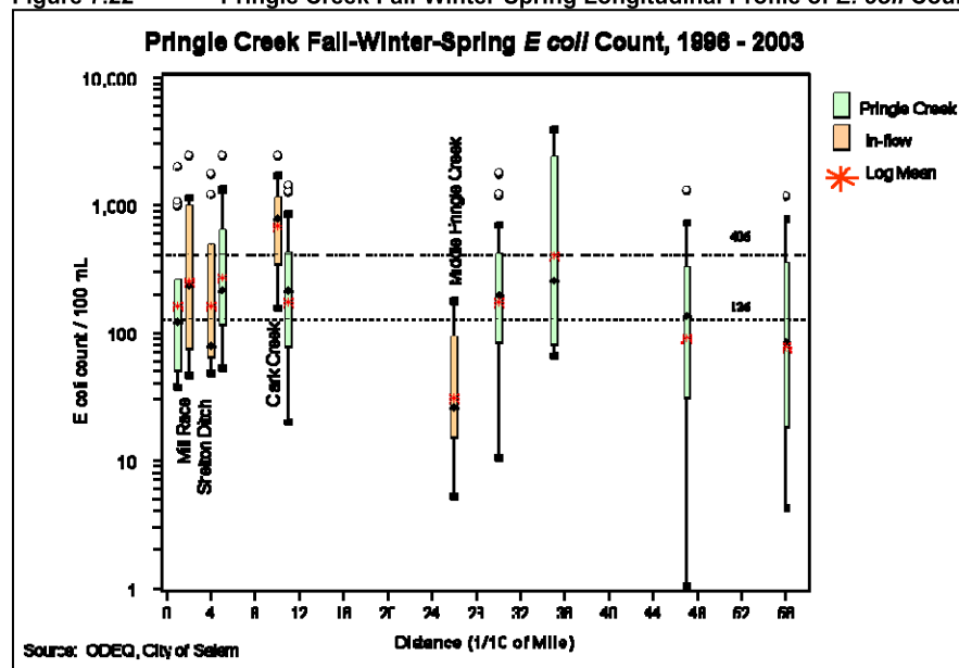
Figure 7.22 Pringle Creek Fall-Winter-Spring Longitudinal Profile of E. coli Counts
