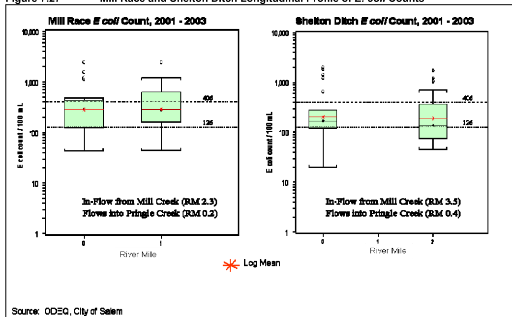
Figure 7.27 Mill Race and Shelton Ditch Longitudinal Profile of E. coli Counts
