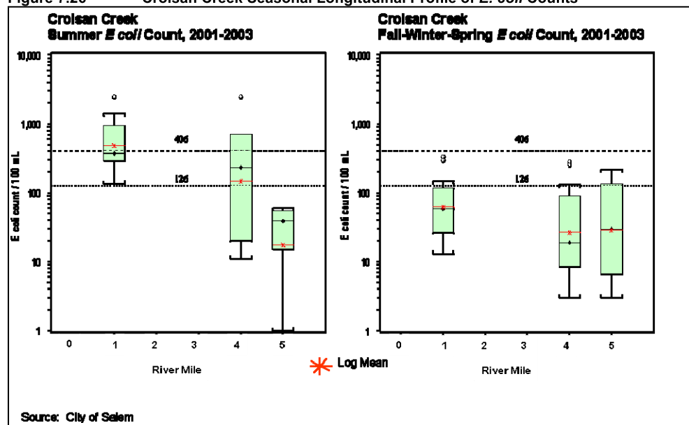
Figure 7.26 Croisan Creek Seasonal Longitudinal Profile of E. coli Counts
