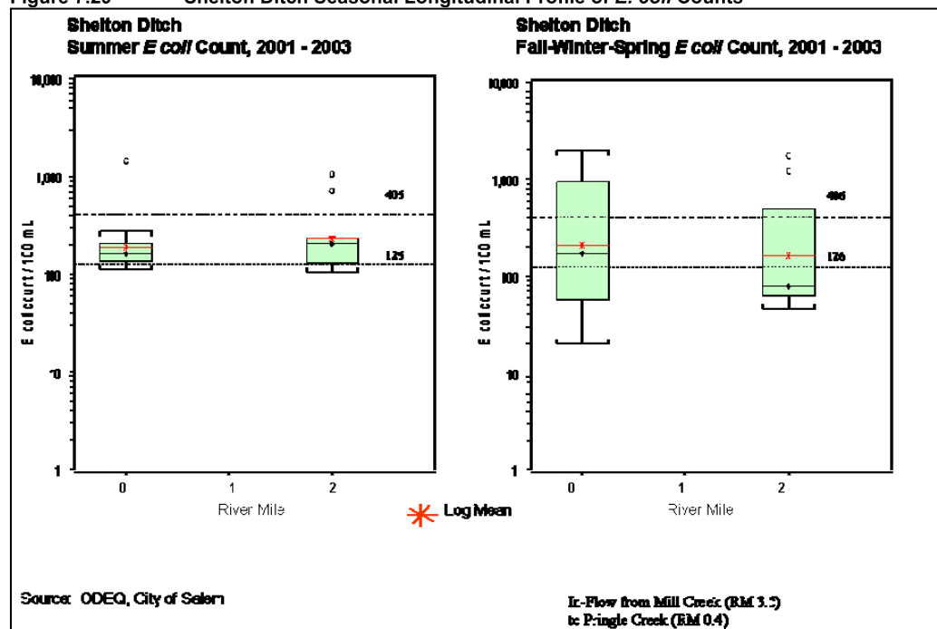
Figure 7.29 Shelton Ditch Seasonal Longitudinal Profile of E. coli Counts
