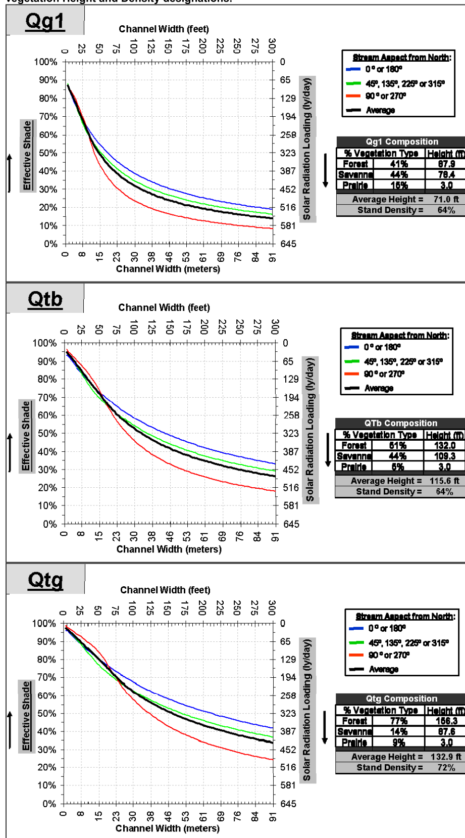
Figure 7.8. (Continued) Shade Curves by Geomorphic Classifications that apply to the Middle Willamette Subbasin with vegetation Height and Density designations.
