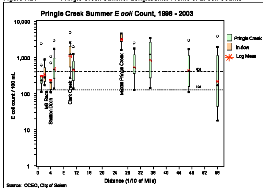
Figure 7.21 Pringle Creek Summer Longitudinal Profile of E. coli Counts
