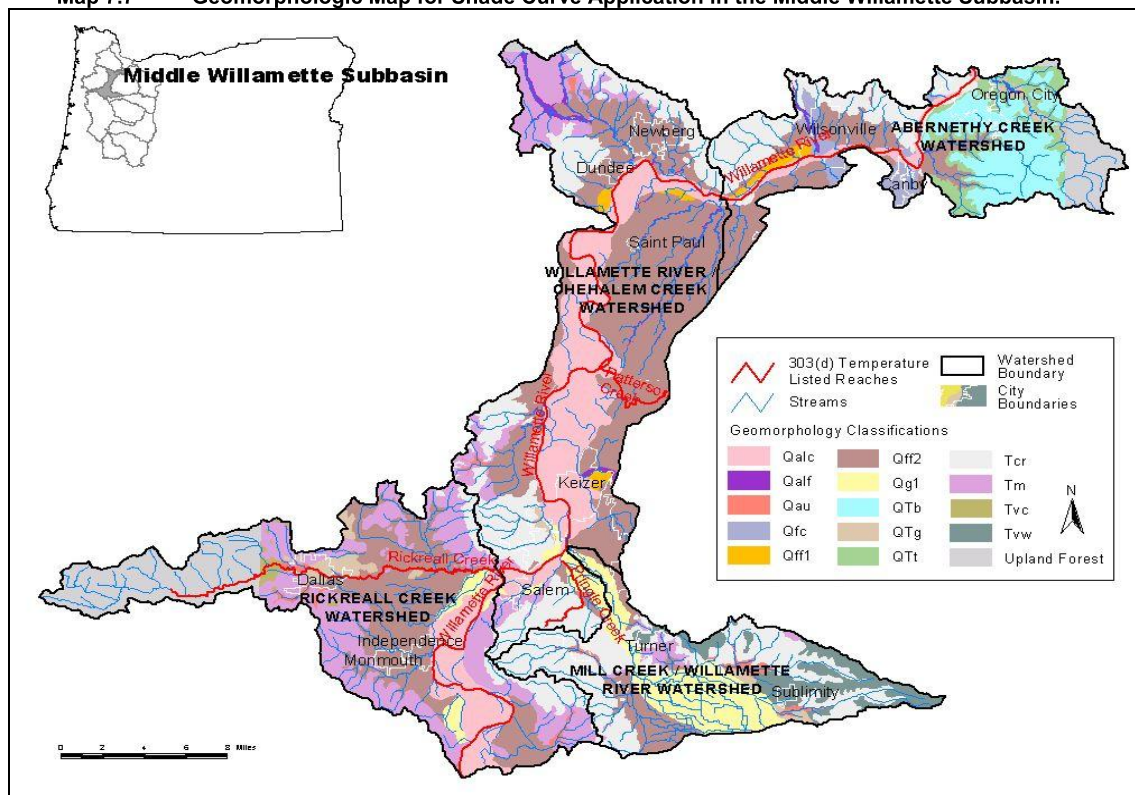
Map 7.7 Geomorphologic Map for Shade Curve Application in the Middle Willamette Subbasin.
