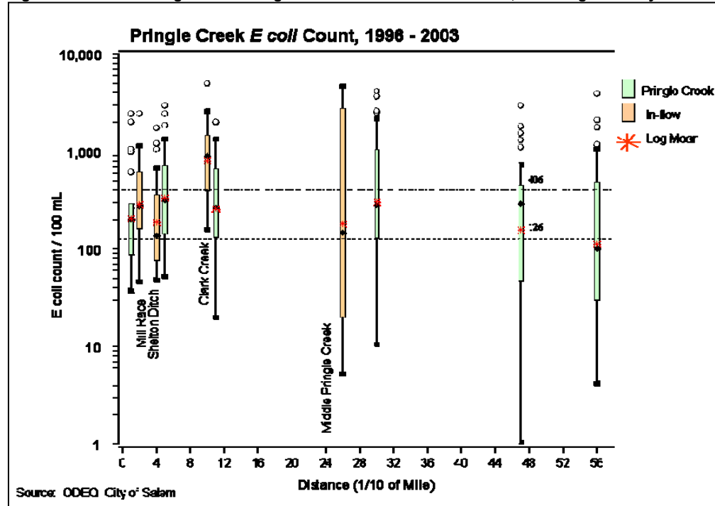
Figure 7.20 Pringle Creek Longitudinal Profile of E. coli Counts, including Tributary In-Flows
