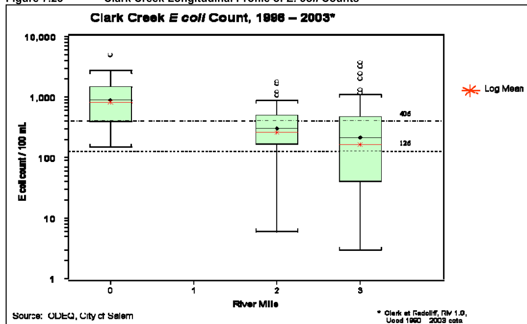
Figure 7.23 Clark Creek Longitudinal Profile of E. coli Counts
