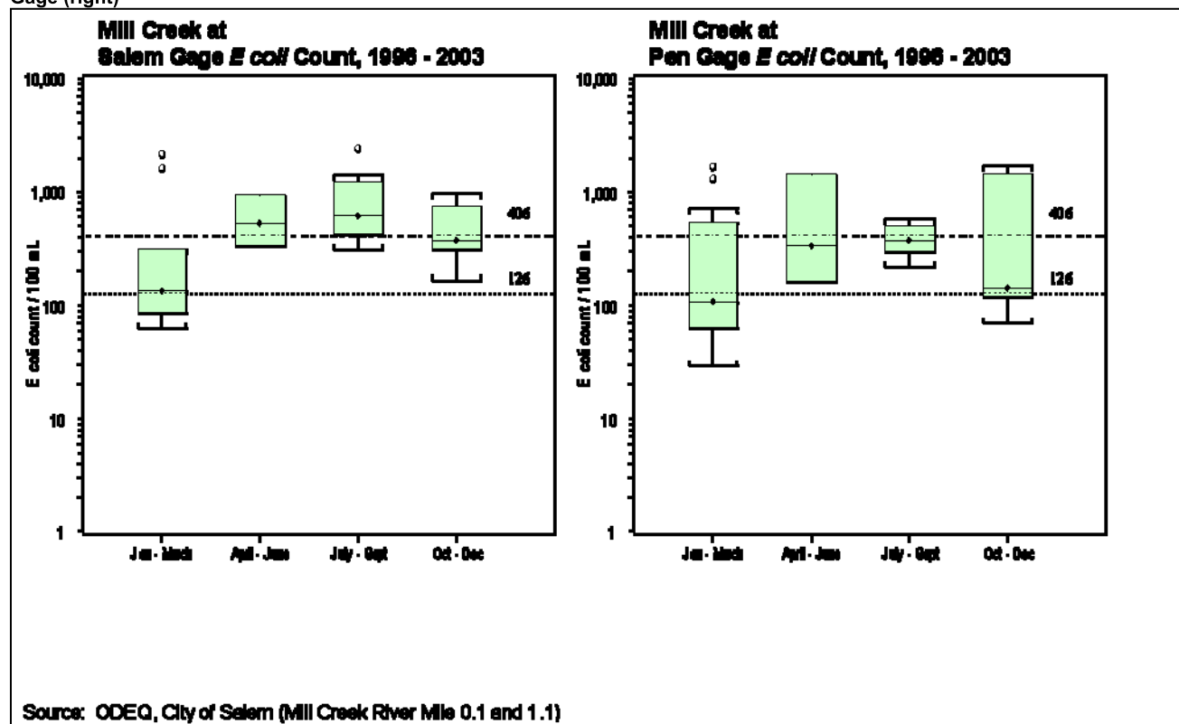
Figure 7.18 Seasonal Comparison of E. coli Counts at Mill Creek at Salem Flow Gage (left), Penitentiary Annex Flow Gage (right)
