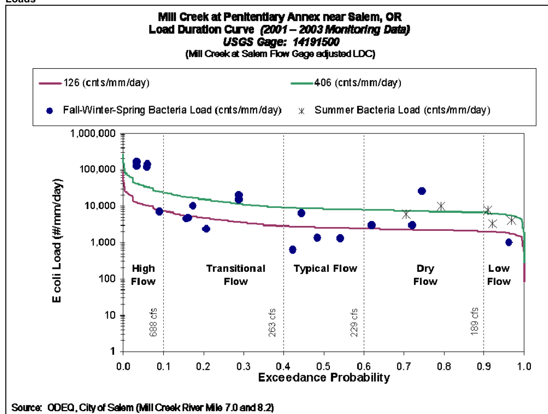
Figure 7.17 Mill Creek at Penitentiary Annex Load Duration Curve, Showing the Loading Capacity and Calculated Event Loads
