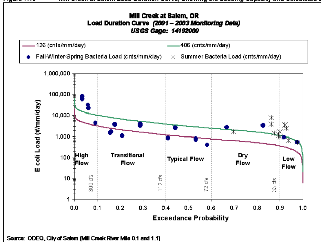
Figure 7.16 Mill Creek at Salem Load Duration Curve, Showing the Loading Capacity and Calculated Event Loads
