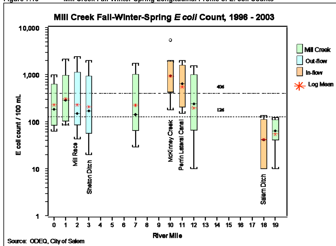
Figure 7.13 Mill Creek Fall-Winter-Spring Longitudinal Profile of E. coli Counts
