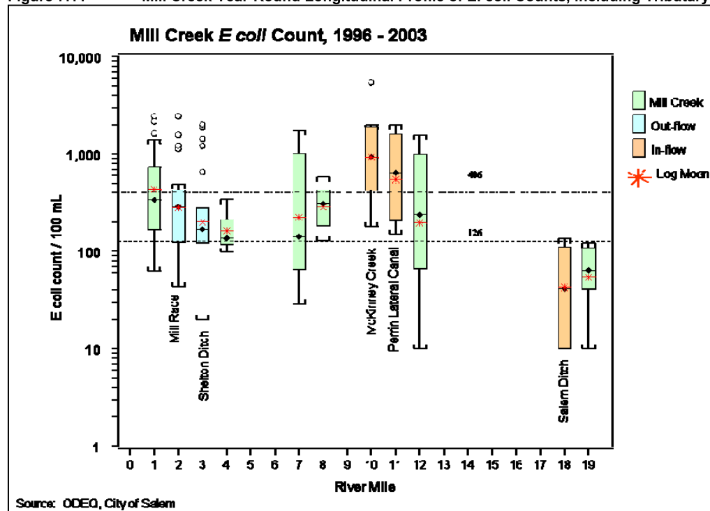
Figure 7.11 Mill Creek Year-Round Longitudinal Profile of E. coli Counts, including Tributary In-Flows and Out-Flows
