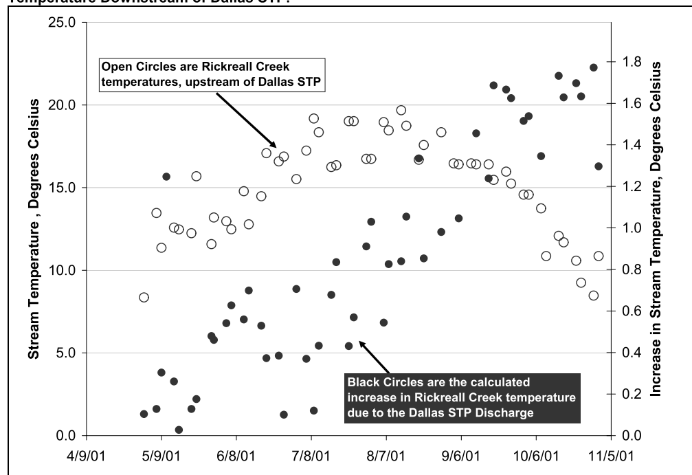
Figure 7.4 Rickreall Creek Summer Stream Temperatures Upstream of Dallas STP, and Increase in Stream Temperature Downstream of Dallas STP.
