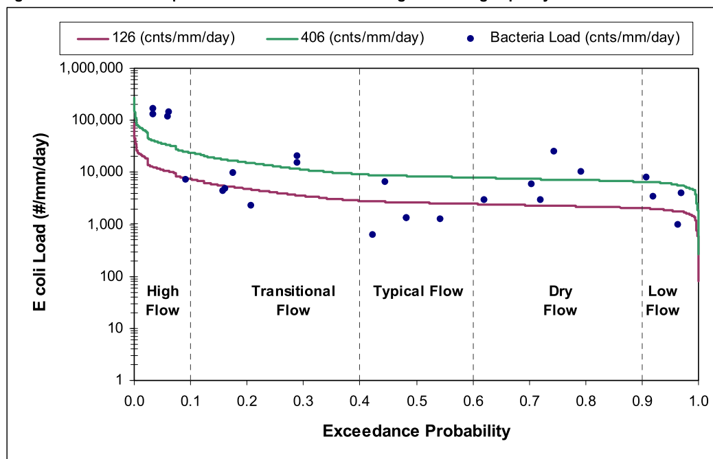
Figure 7.10 Example Load Duration Curve showing the loading capacity and calculated event loads
