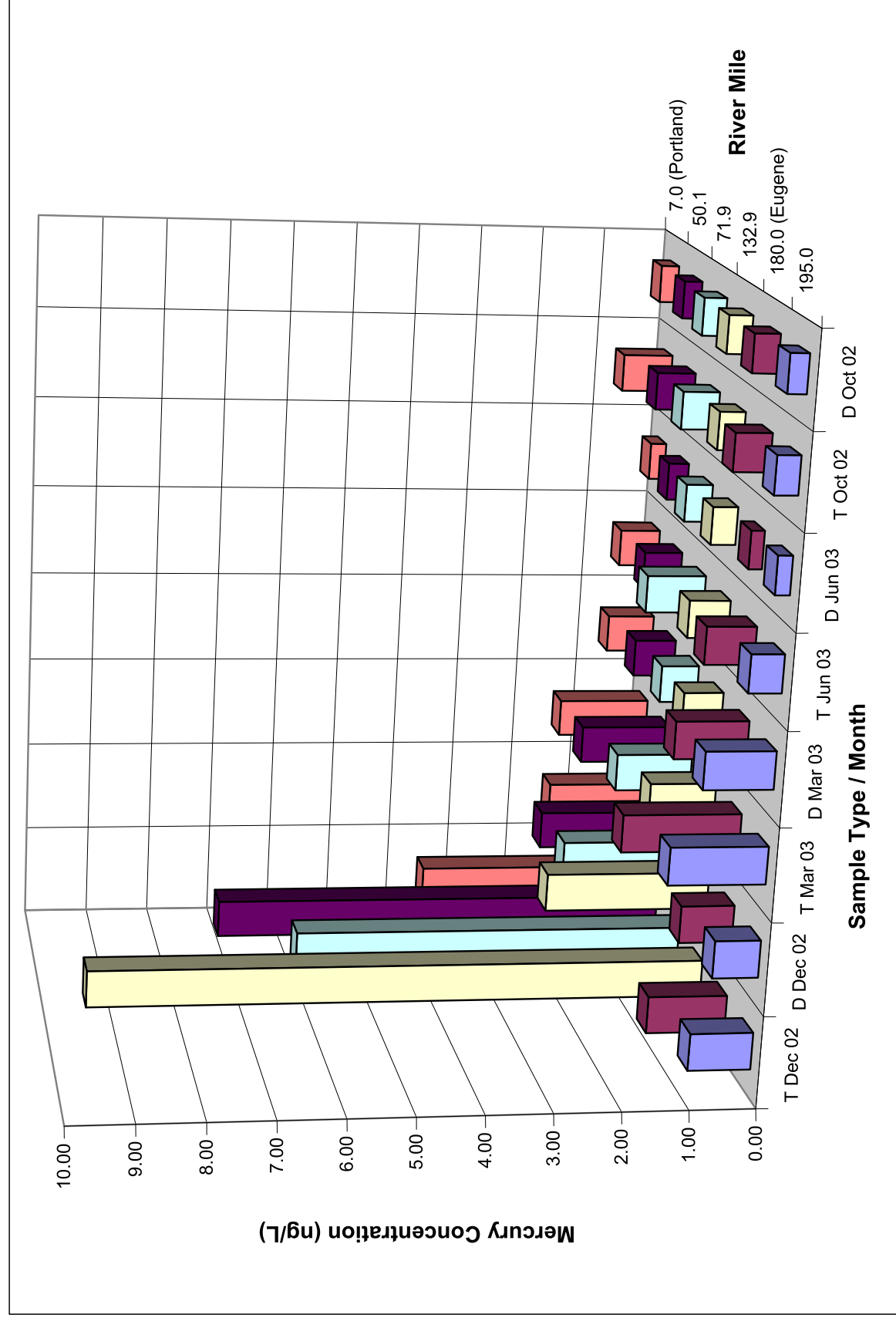
Figure 3.9 Seasonal and Spatial Trends in Total (T) and Dissolved (D) Mercury Concentrations in the Mainstem Willamette River.
