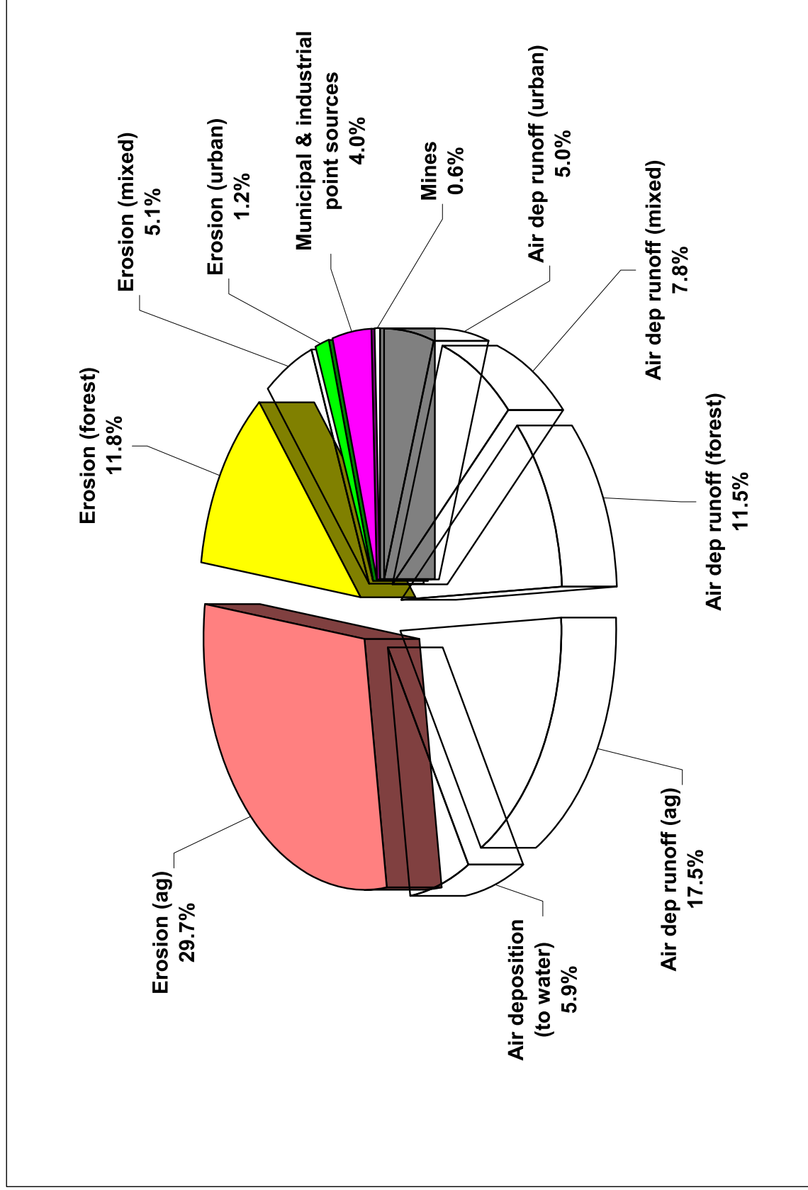
Figure 3.4 Relative Load Contributions for the Mainstem Willamette River System by Land Use Category (Total Load = 128.5 kg/yr).
