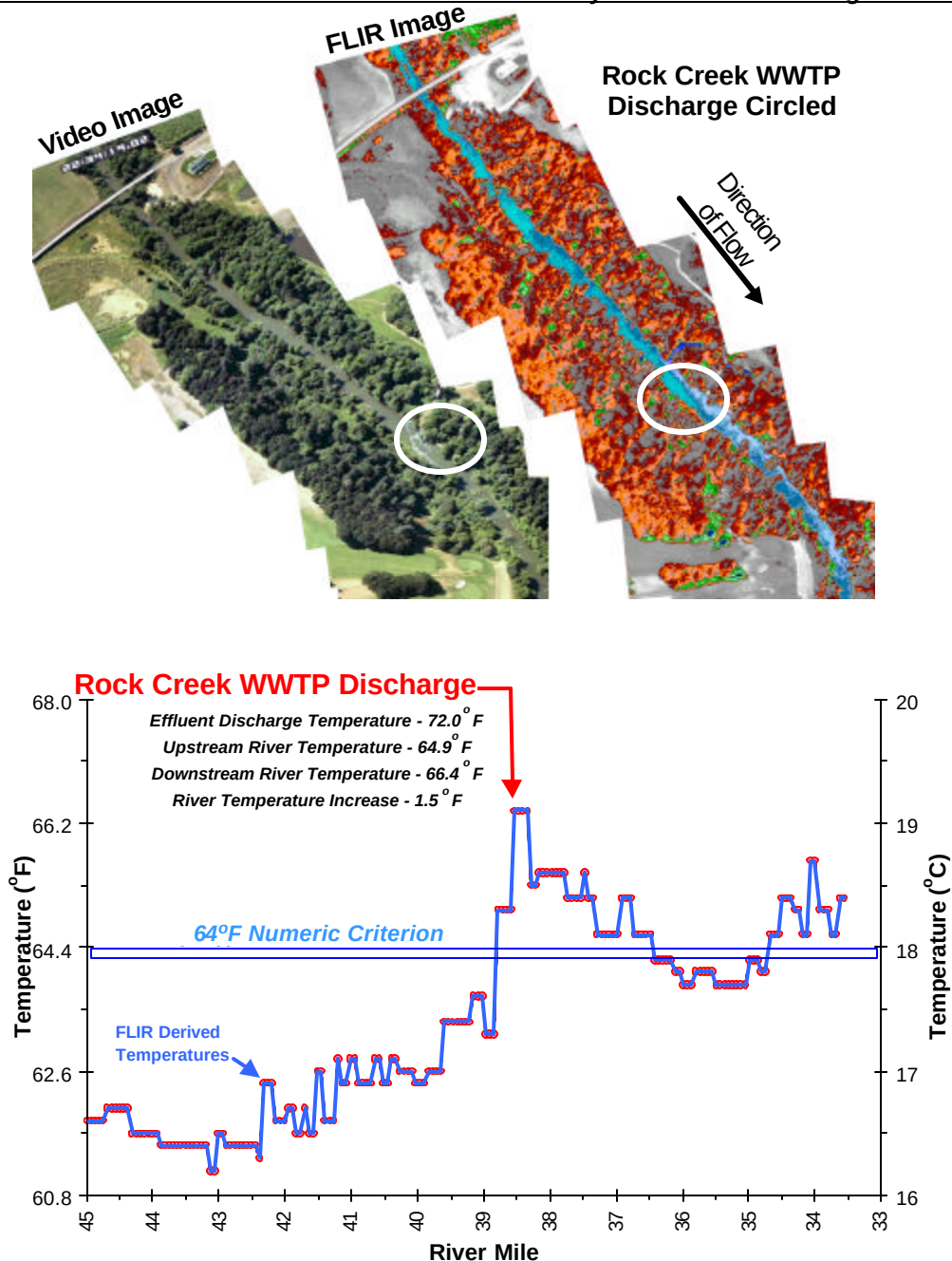
Figure 14. Rock Creek Waste Water Treatment Plant Day Video and FLIR Image Mosaics*
