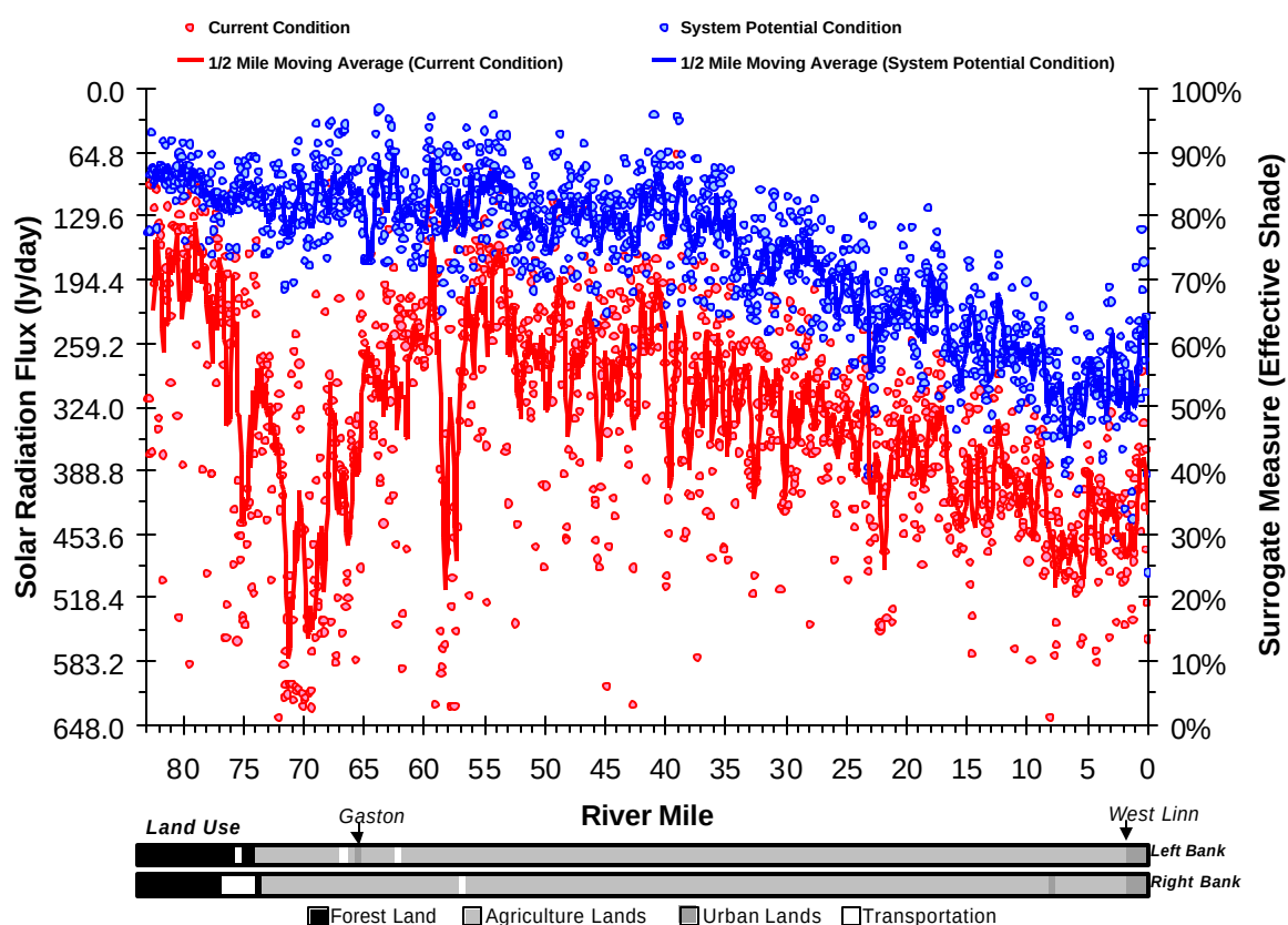
Figure 19. Tualatin River Percent Effective Shade Surrogate Measures
