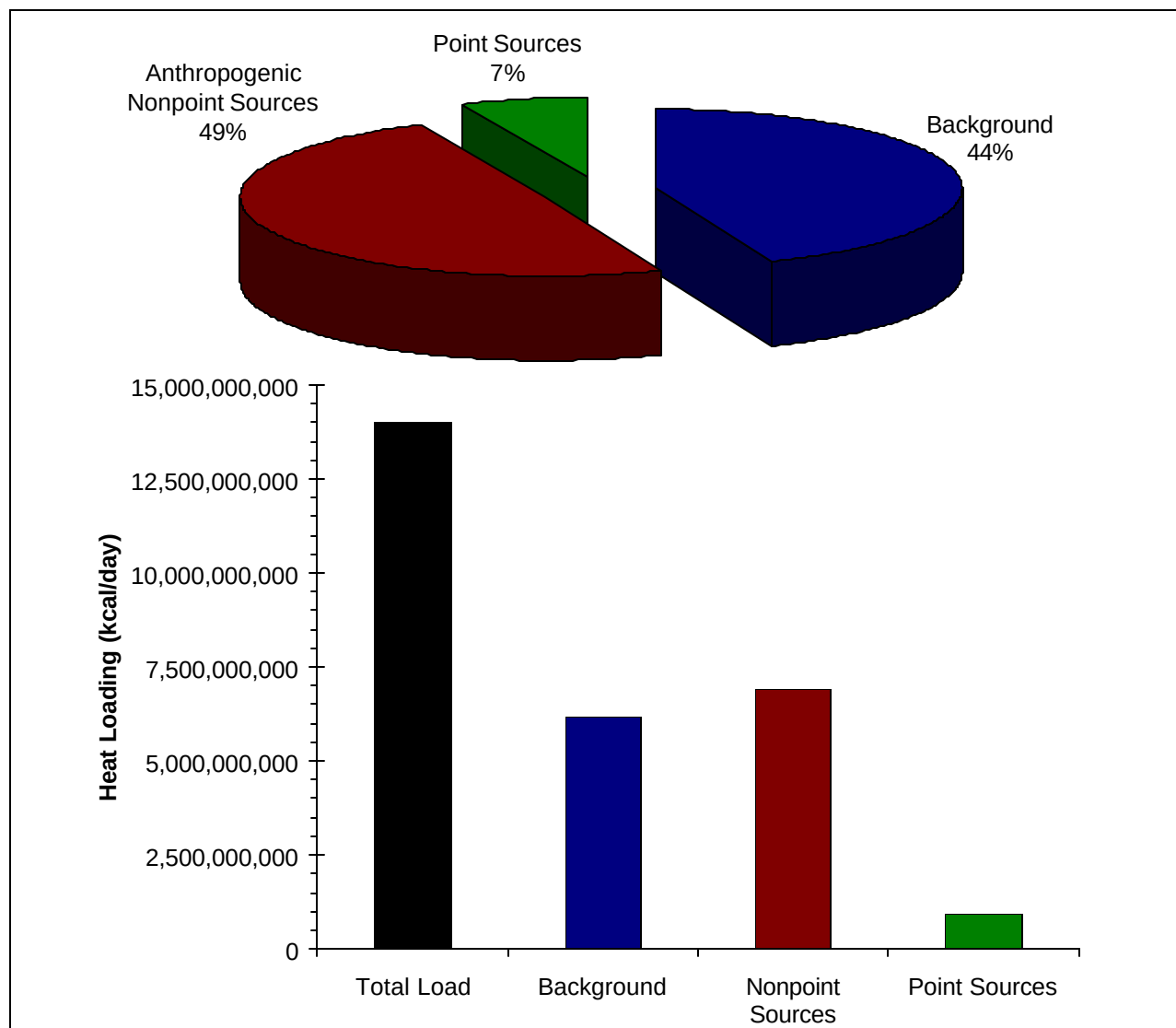
Figure 8. Distribution of Current Condition Heat Loading
