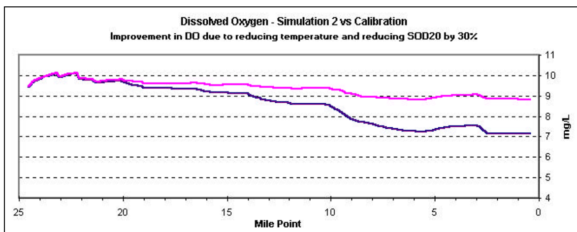
Figure 53. Dissolved Oxygen – Simulation with Temperature and SOD Reductions vs. Calibration on Gales Creek
