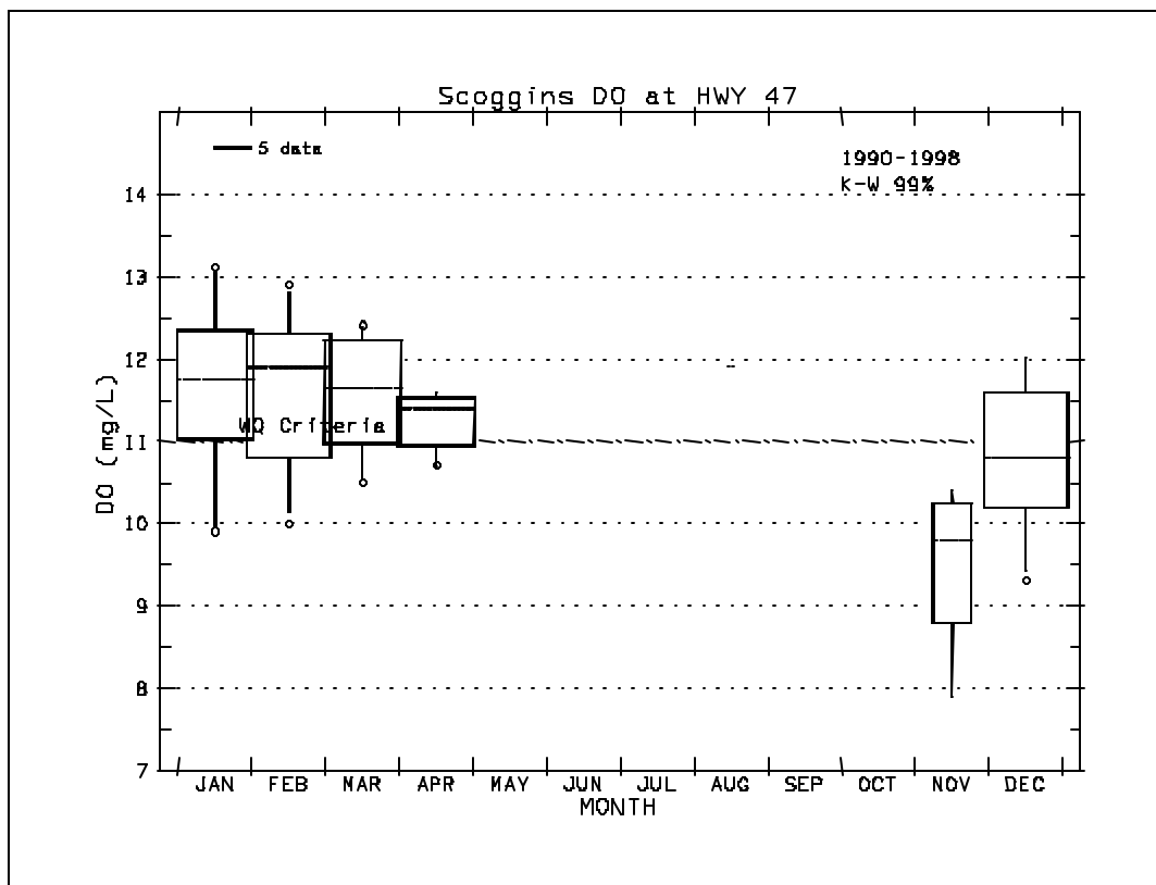
Figure 59. Dissolved Oxygen Concentration Box Plots for Scoggins Creek at Old Highway 47 (1990 - 1998)
