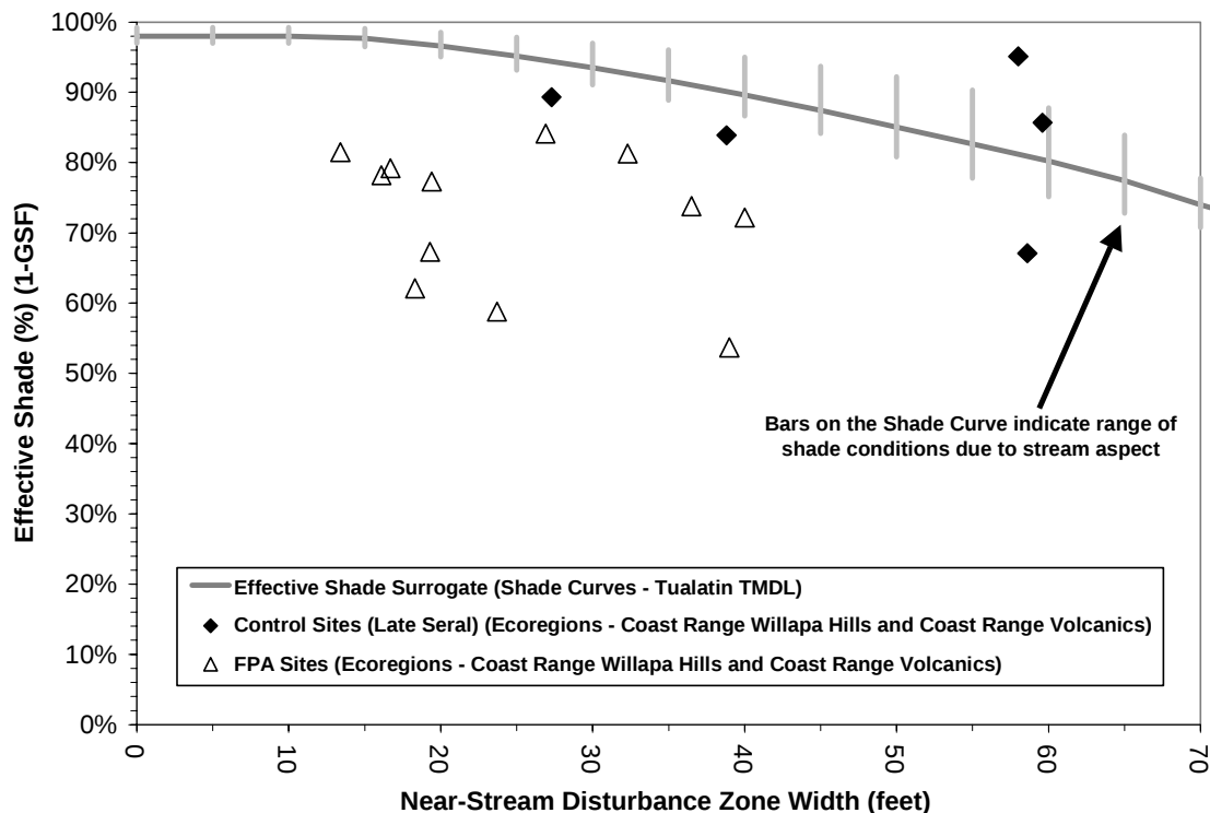
Tualatin River Subbasin TMDL Effective Shade Surrogate Measures (DEQ Data) and Measured Effective Shade Data (ODF Data, 1999)
