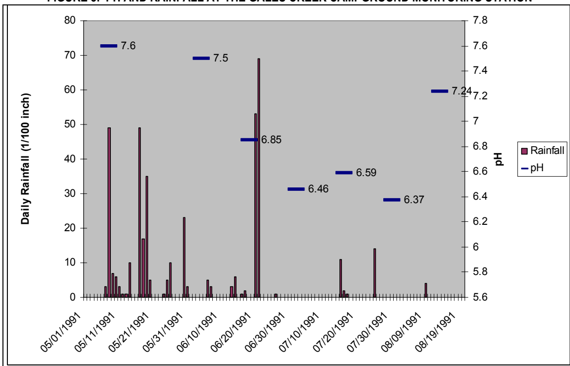
FIGURE 3. PH AND RAINFALL AT THE GALES CREEK CAMPGROUND MONITORING STATION
