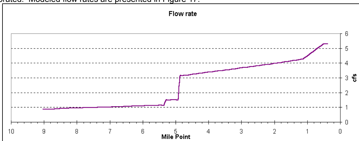
Figure 17. Modeled Flow Rate
