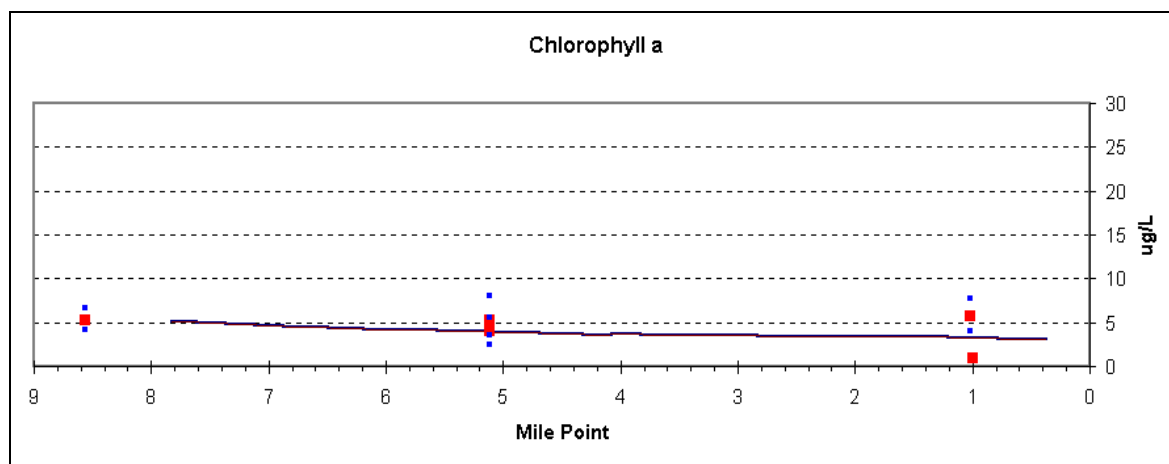
Figure 37. Model Calculated Chlorophyll a (Algae) - Calibration vs. Observations
