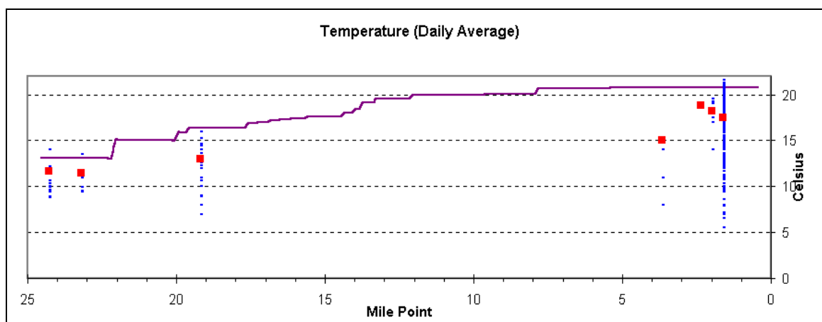
Figure 3. Model Calculated Temperature
