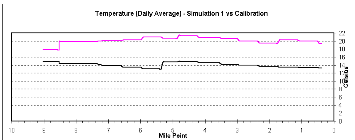
Figure 22. Temperature – Site Potential Shade Scenario vs. Calibration
