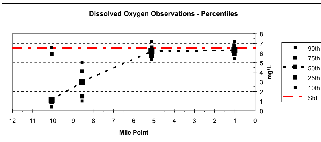
Figure 30. Rock and Beaverton Creek Dissolved Oxygen
