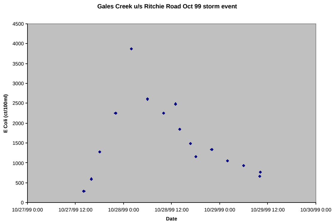
Figure 4: Bacteria Pollutograph from Gales Creek upstream of Ritchie Road (DEQ data)
