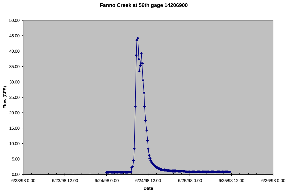
Figure 1: Hydrograph from Fanno Creek at 56 th (USGS gage 14206900)
