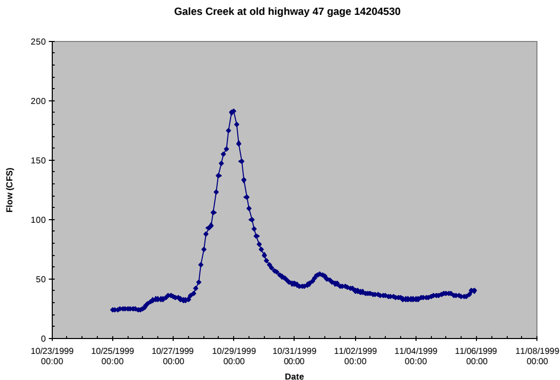
Figure 3: Hydrograph recorded at Gales Creek at old highway 47 (WRD gage 14204530)
