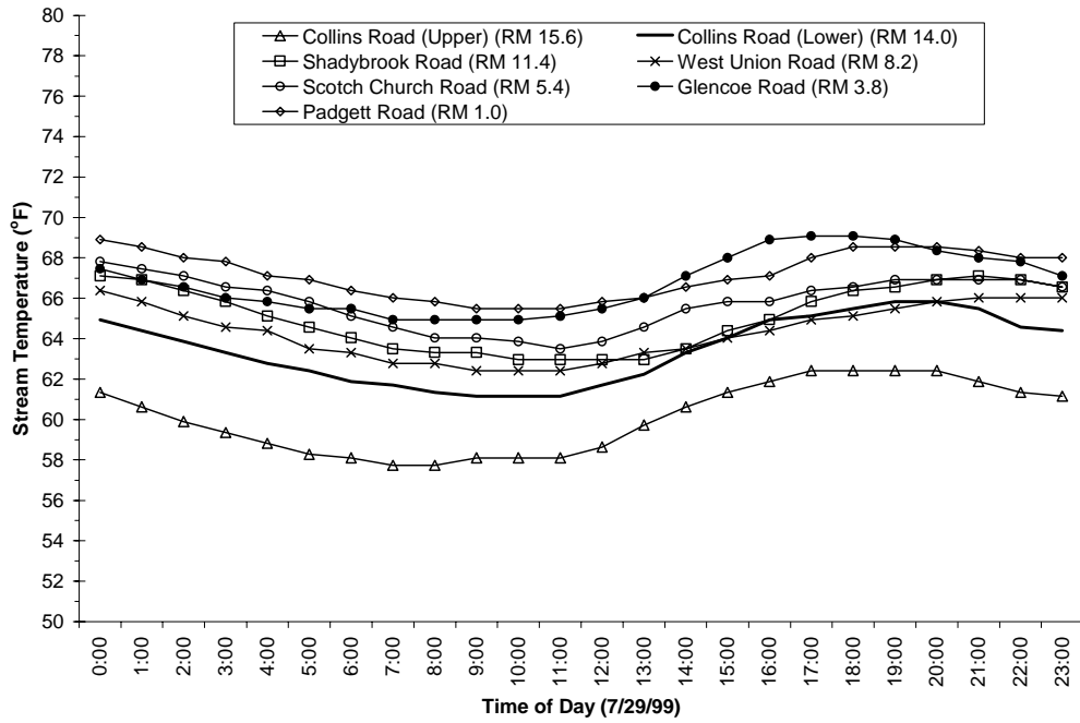
Figure A-127. Diurnal Temperature Trends Observed in McKay Creek on July 29, 1999.
