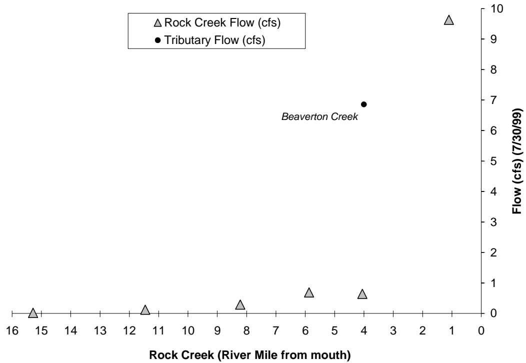
Figure A-150. Water discharge observed in Rock Creek on July 30, 1999.
