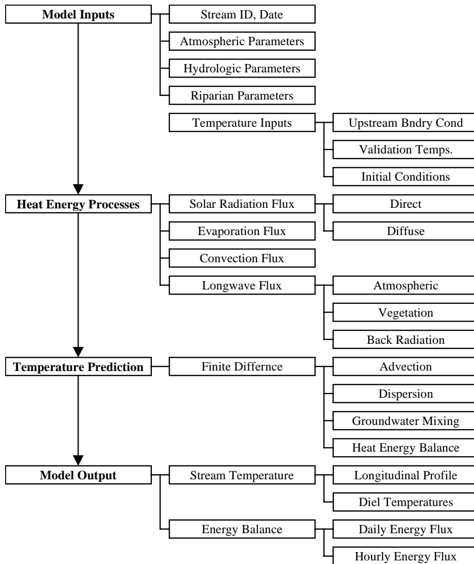
Figure A-20. Temperature Model Flow Chart
