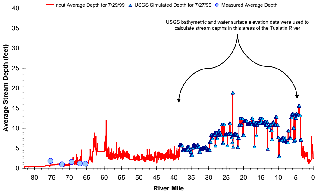
Figure A-45. Tualatin River Measured and Manning's Derived Longitudinal Water Column Depths
