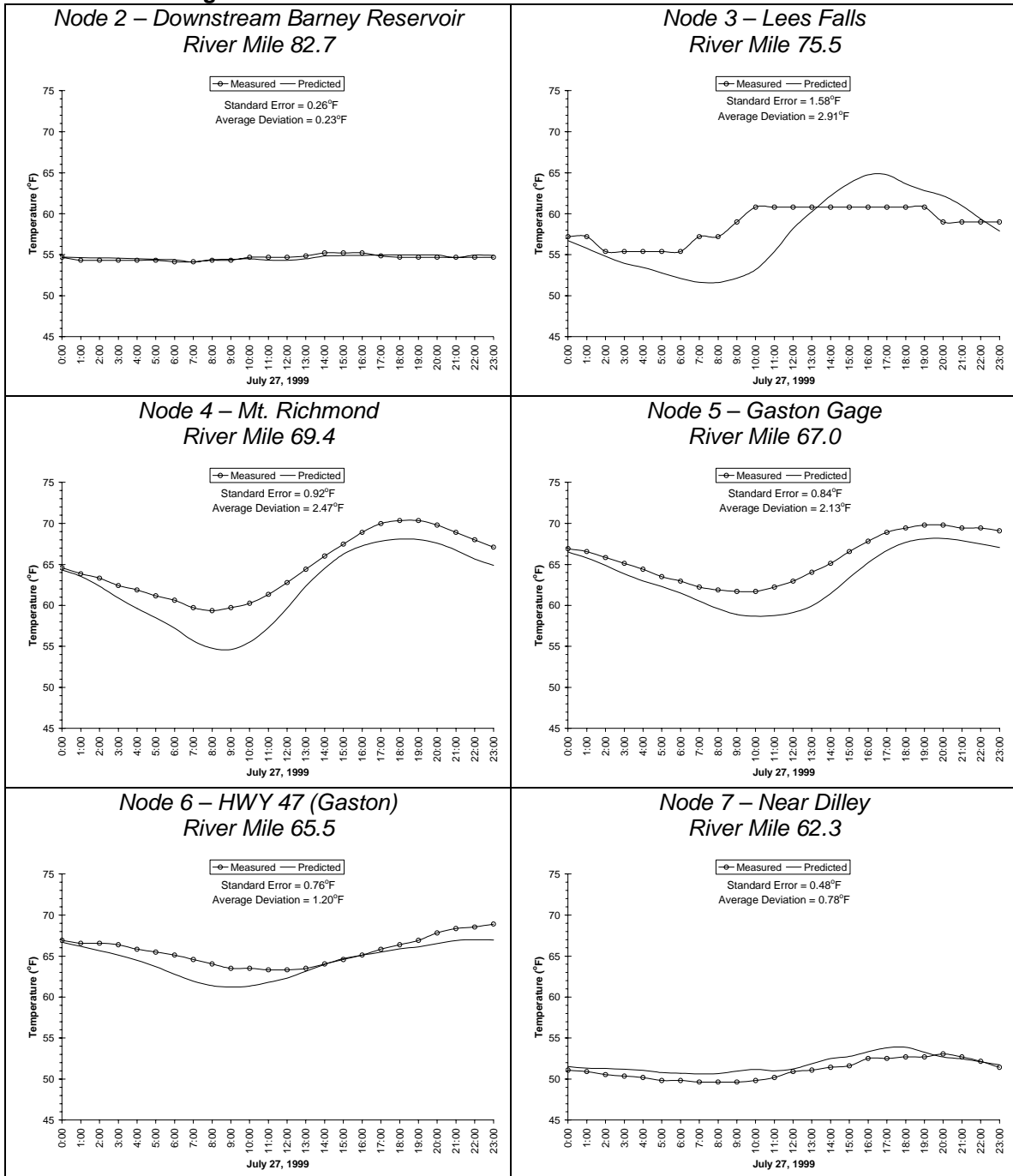
Figure A-47. Tualatin River Model Continuous Data Validation
