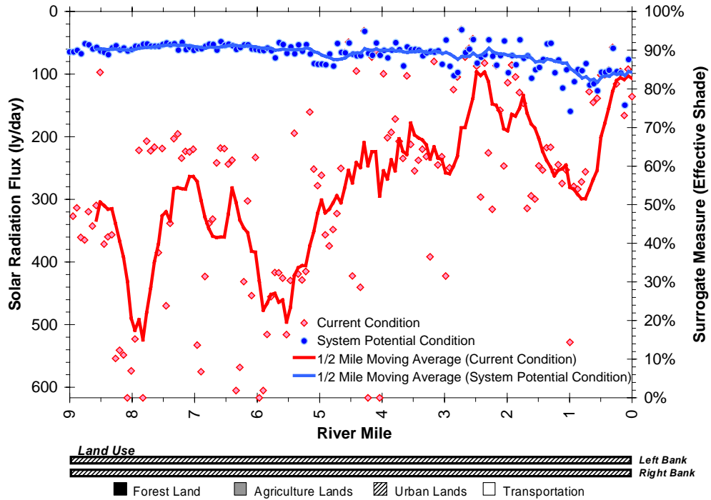
Figure A-190. Fanno Creek Surrogate Measure for Non Point Sources – Effective Shade
