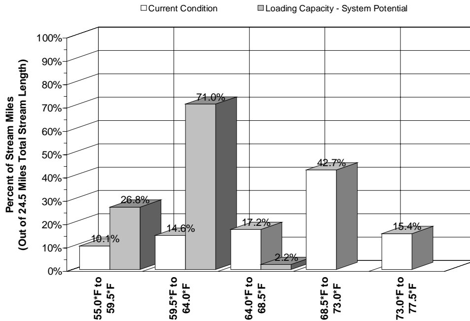
Figure A-73. Gales Creek Current and System Potential (Allocated) Temperature Distributions
