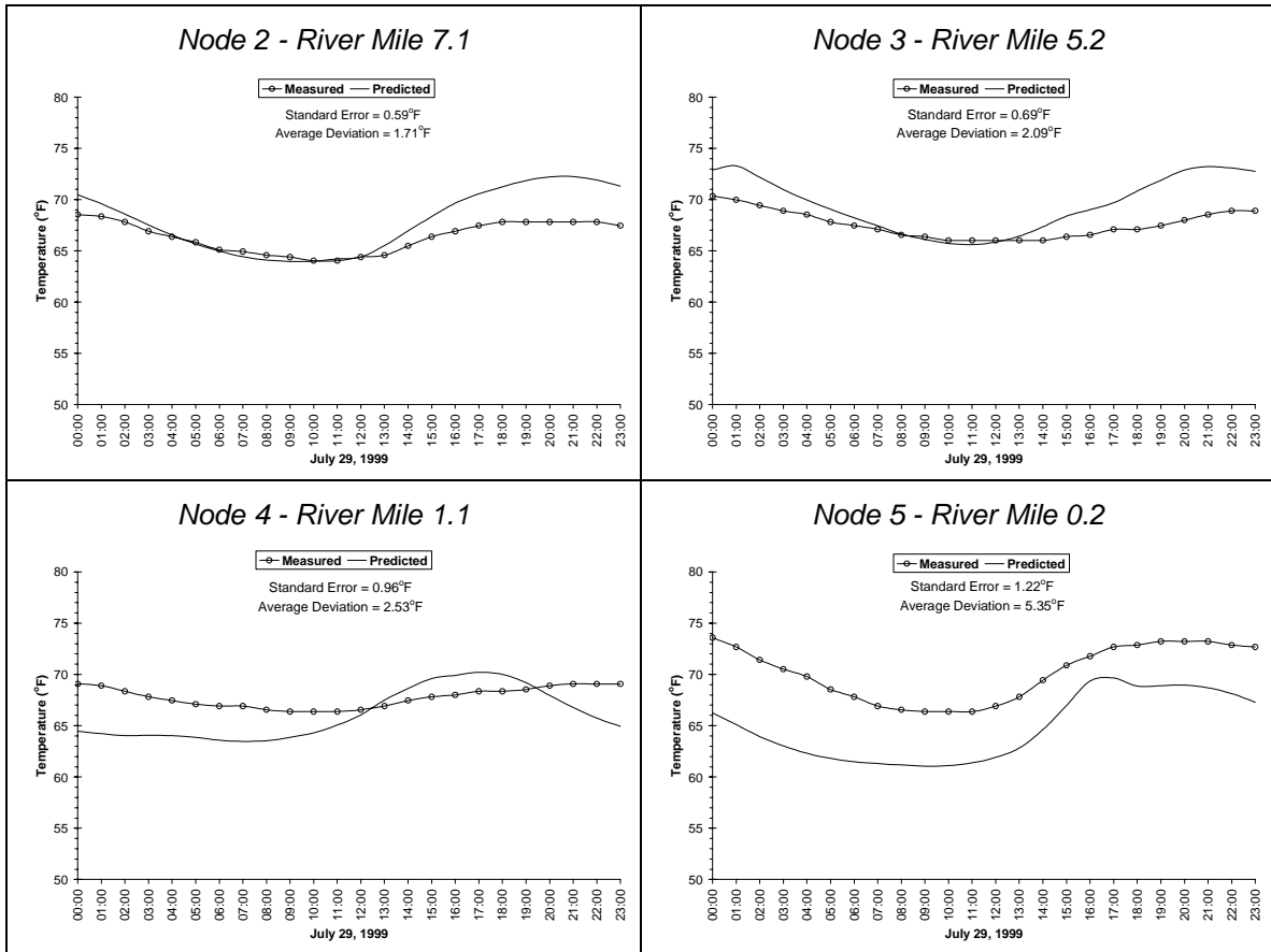
Figure A-188. Fanno Creek Model Continuous Data Validation
