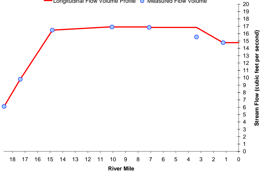
Figure A-85. East Fork Dairy Creek Measured and Interpolated Flow Volume — Longitudinal Flow Volume Profile ● Measured Flow Volume
