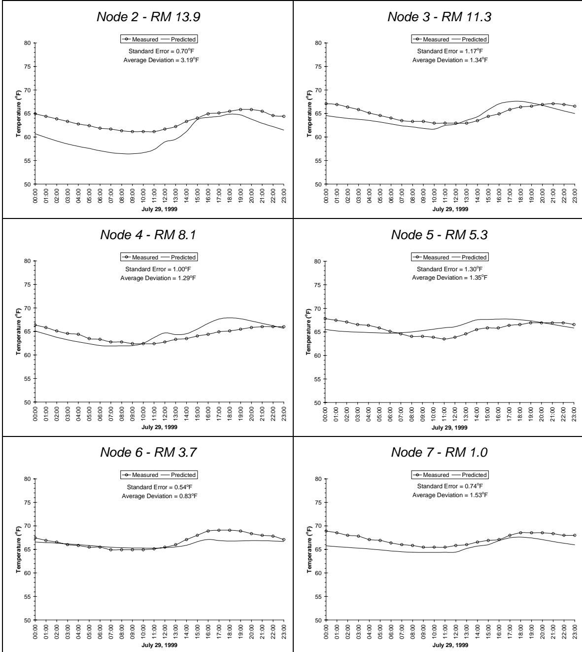
Figure A-139. McKay Creek Model Continuous Data Validation
