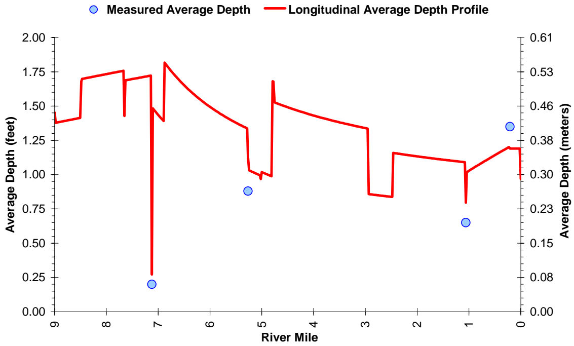
Figure A-186. Fanno Creek Measured and Mannings Derived Longitudinal Water Column Depths
