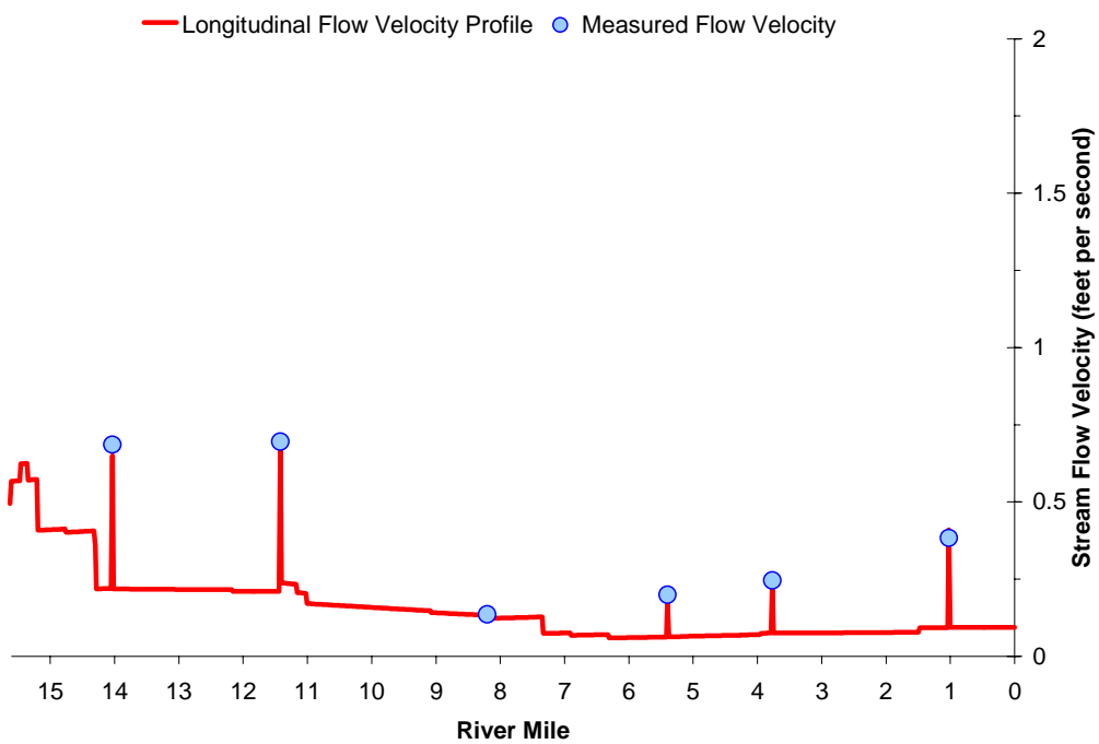
Figure A-136. McKay Creek Measured and Mannings Derived Longitudinal Flow Velocities 13
