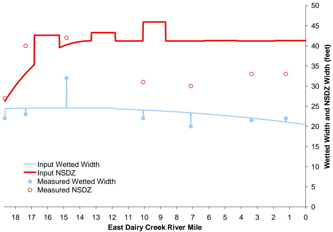
Figure A-82. East Fork Dairy Creek Wetted Widths and NSDZ Widths
