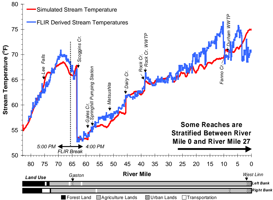
Figure A-46. Tualatin River Observed and Predicted Spatial Temperature Data on 7/27/99.
