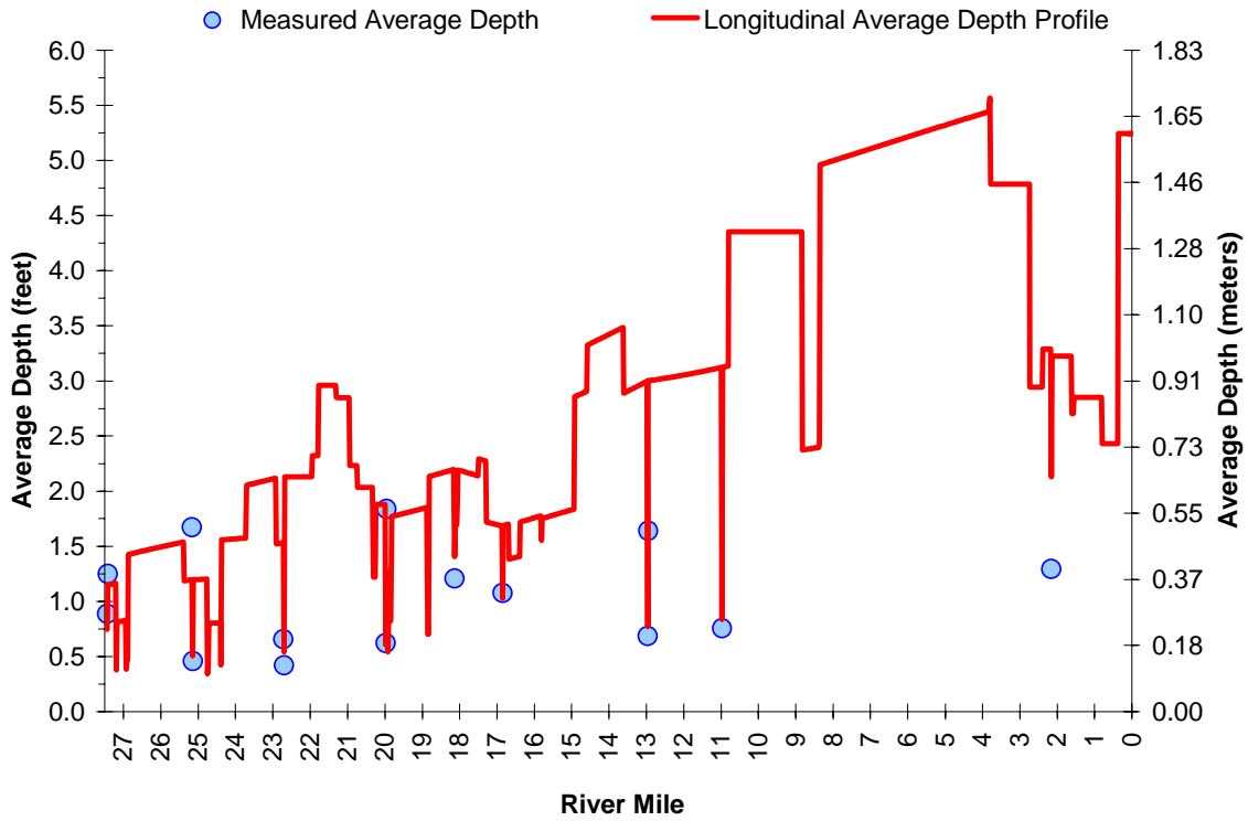
Figure A-115. West Fork Dairy Creek/Dairy Creek Measured and Mannings Derived Longitudinal Water Column Depths.
