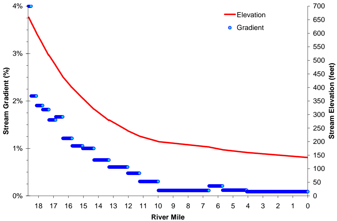
Figure A-80. East Fork Dairy Creek Elevation and Gradient at each 100-foot Model Reach.
