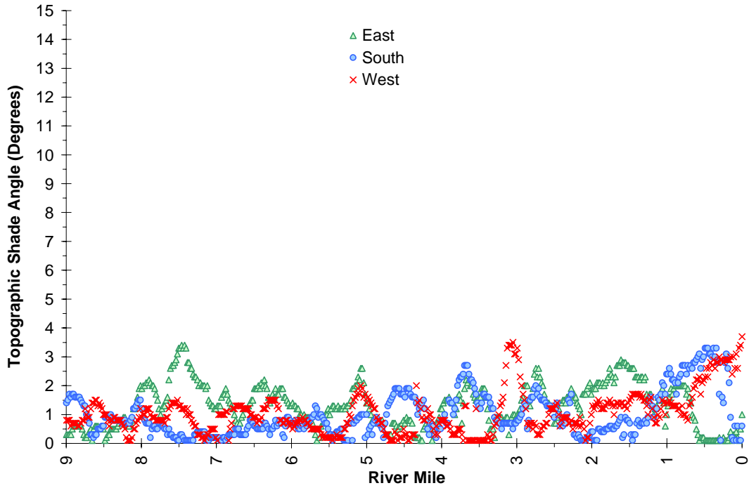
Figure A-182. Fanno Creek Topographic Shade at Each 100-foot Model Reach.
