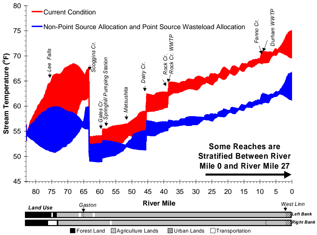
Figure A-52. Tualatin River Daily Temperature Range for Current Conditions Compared with Allocated Measures - July 27, 1999.
