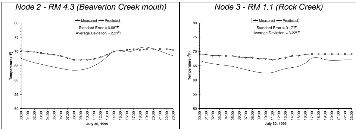
Figure A-166. Rock and Beaverton Creek Model Continuous Data Validation
