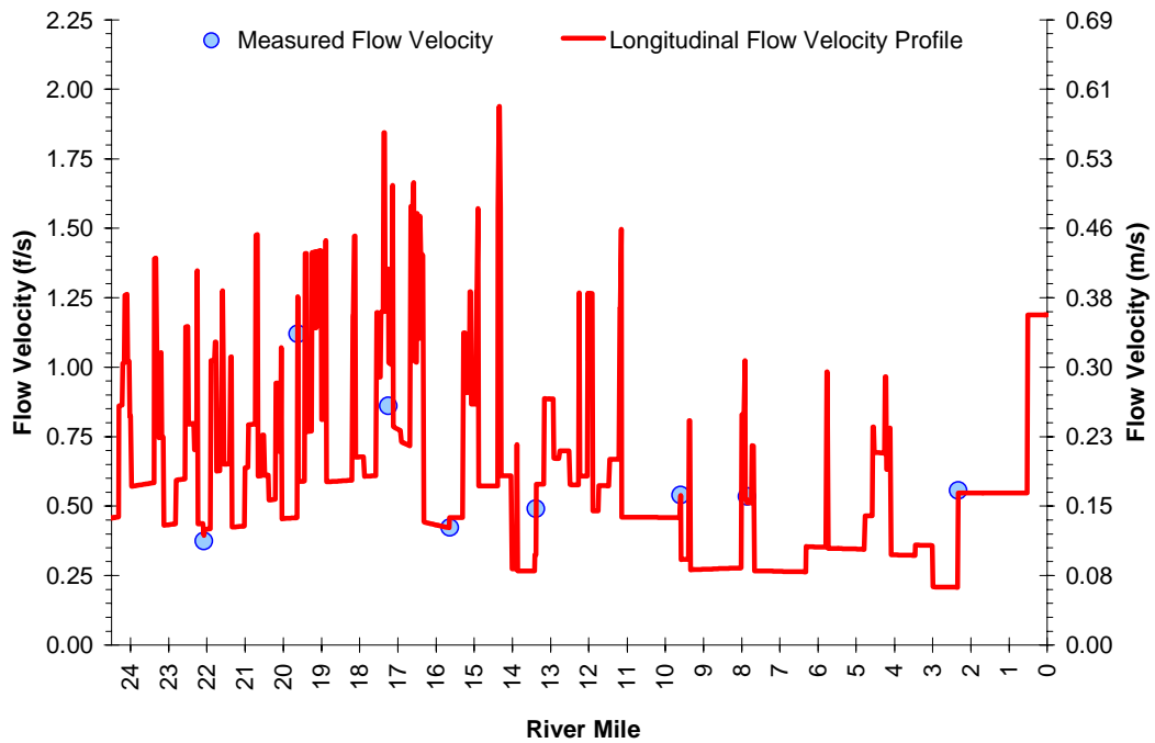
Figure A-66. Gales Creek Measured and Mannings Derived Longitudinal Flow Velocities.
