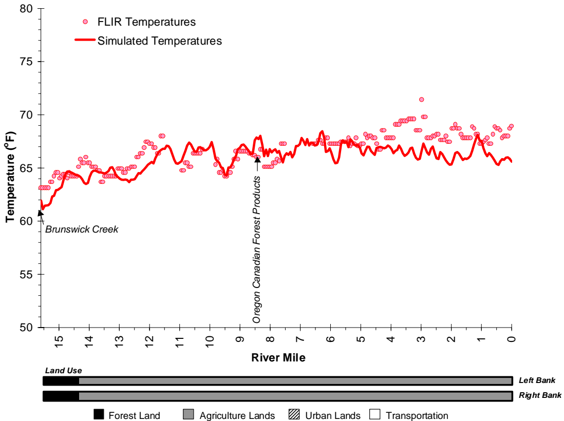
Figure A-138. McKay Creek Observed and Predicted Spatial Temperature Data.
