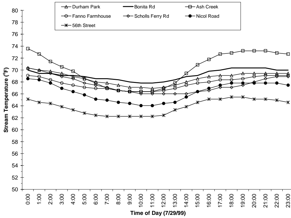
Figure A-176. Diurnal temperature trends observed in Fanno Creek on July 29, 1999.
