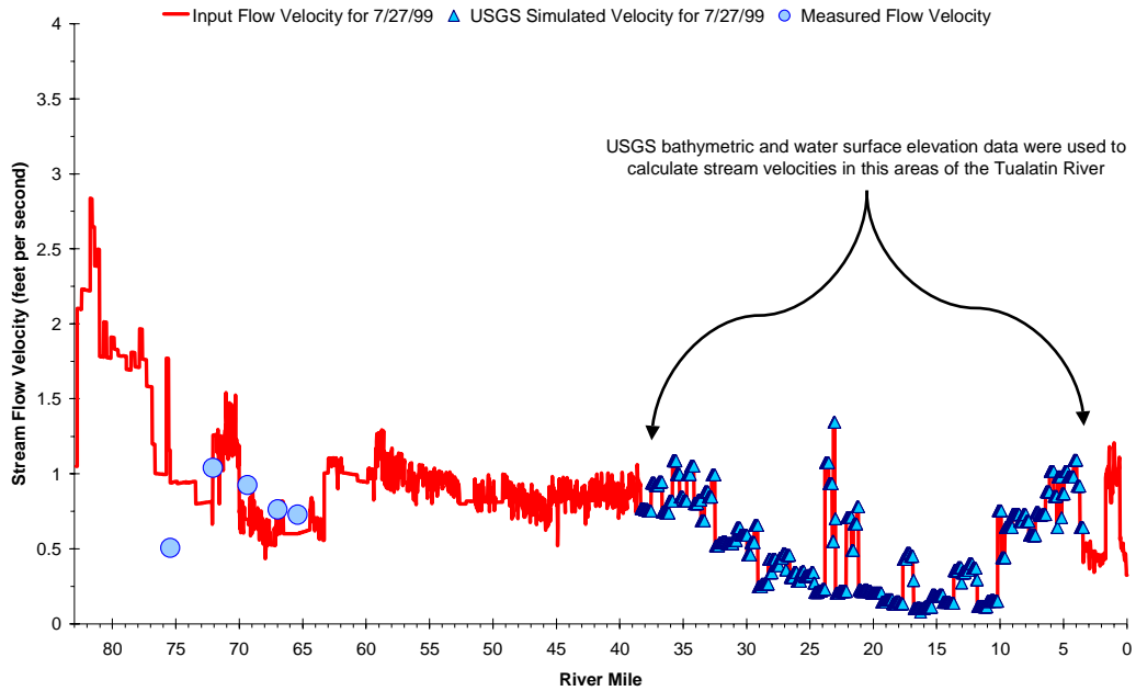
Figure A-44. Tualatin River Measured and Manning's Derived Longitudinal Flow Velocities
