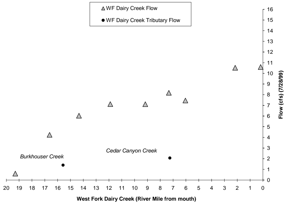
Figure A-98. Stream Flow Observed in West Fork Dairy Creek on July 28, 1999.
