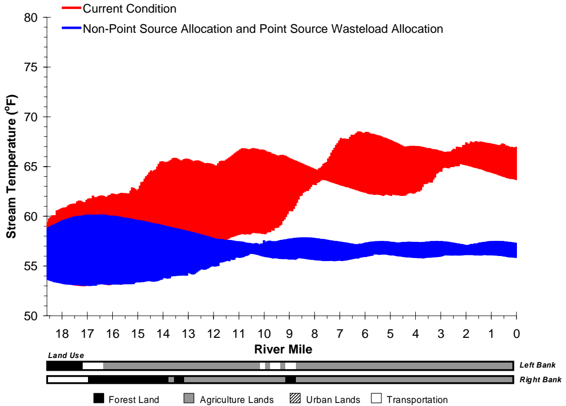
Figure A-92. East Fork Dairy Creek Daily Temperature Range for Current Conditions Compared with Allocated Measures - July 29, 1999.
