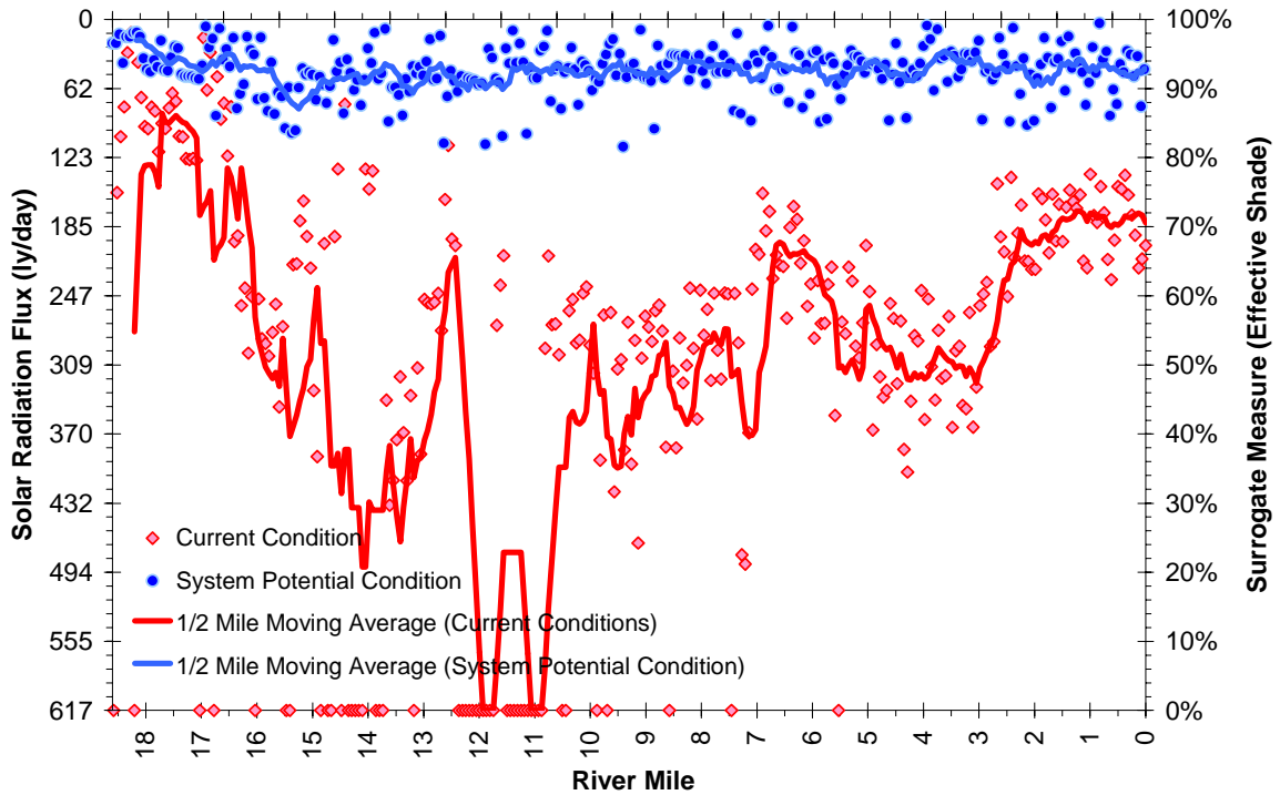
Figure A-91. East Fork Dairy Creek Surrogate Measure for Non Point Sources – Effective Shade
