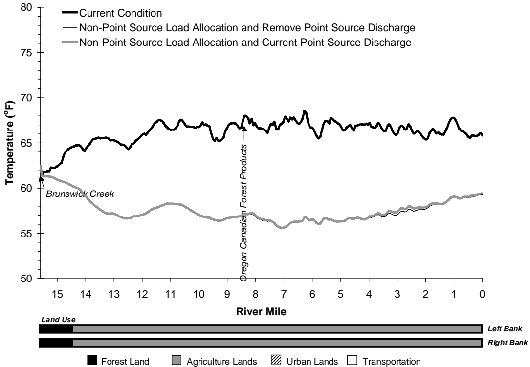
Figure A-142. McKay Creek Longitudinal Temperature Profile - Model Output – 1) Non-Point Source Load Allocation and Current Point Source Discharge, and 2) Non-Point Source Load Allocation and Remove Point Source Discharge – 5:00 PM July 29, 1999.
