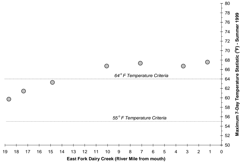
Figure A-76. Observed Maximum 7-Day Temperature Statistics for East Fork Dairy Creek.
