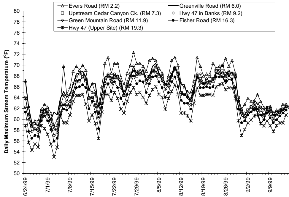
Figure A-95. Observed Daily Maximum Stream Temperatures for West Fork Dairy Creek.
