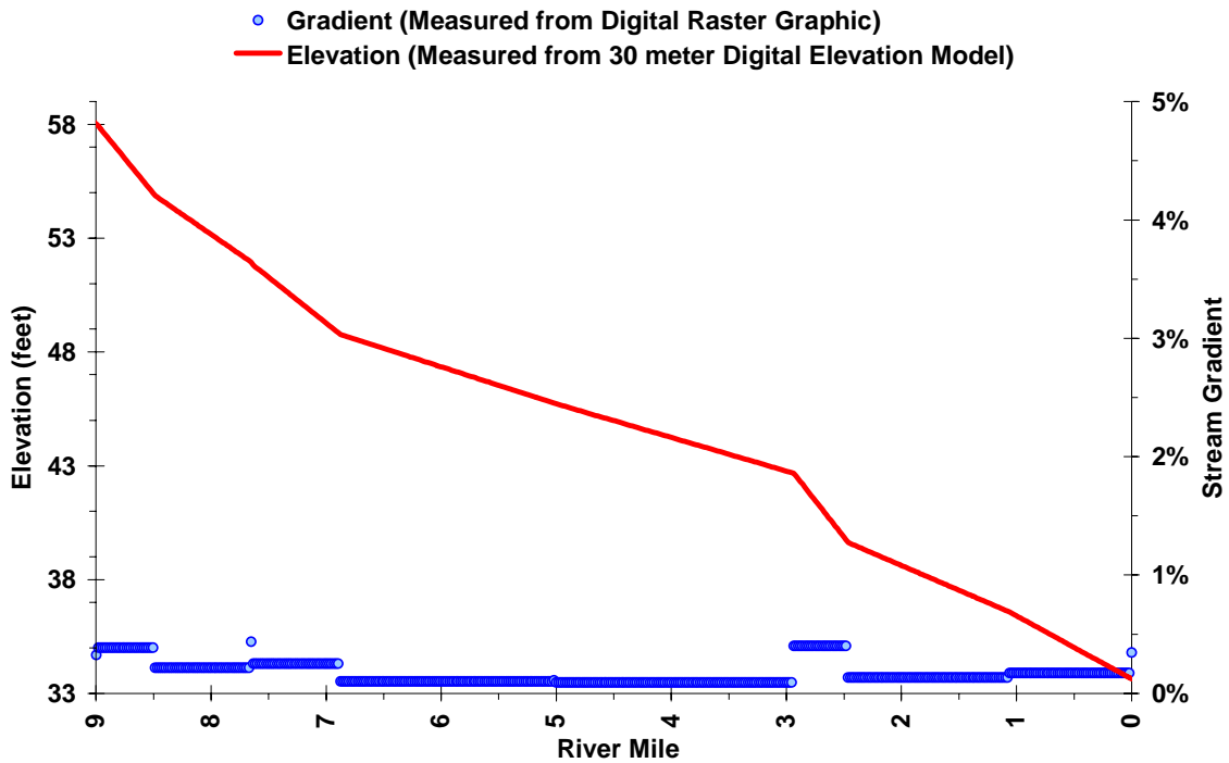
Figure A-179. Fanno Creek Elevation and Gradient at Each 100-foot Model Reach.
