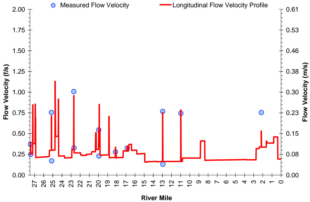
Figure A-114. West Fork Dairy Creek/Dairy Creek Measured and Mannings Derived Longitudinal Flow Velocities.
