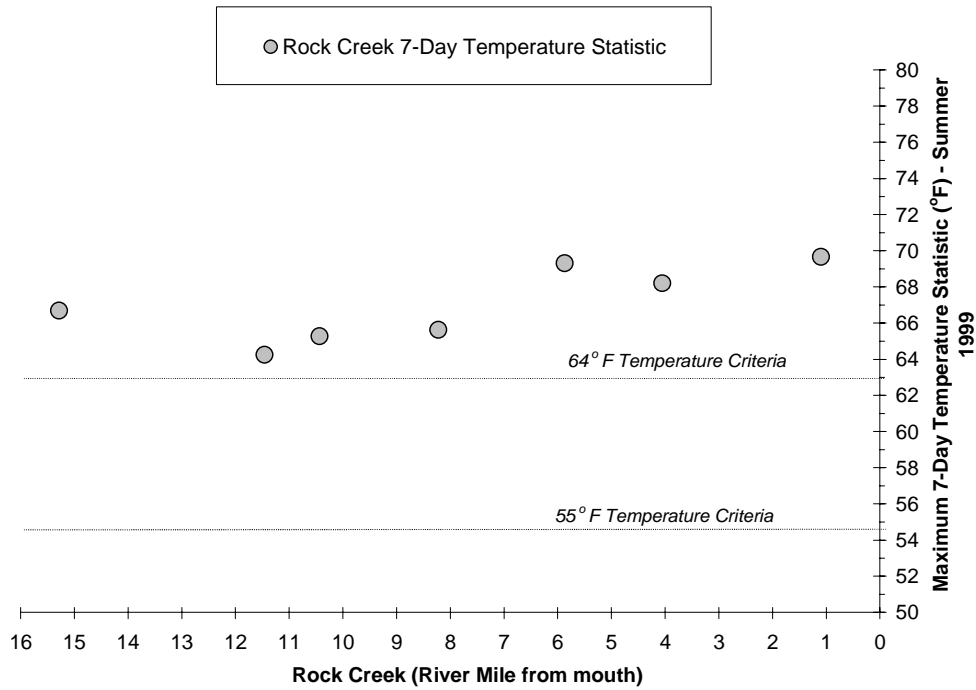
Figure A-148. Observed 7-Day temperature Statistics for Rock Creek during the summer of 1999.
