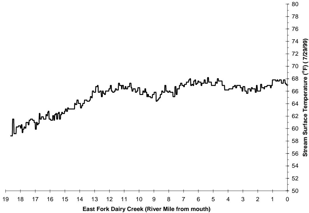
Figure A-79. East Fork Dairy Creek FLIR Temperature Profile (17:00 to 17:23 on 7/29/99)
