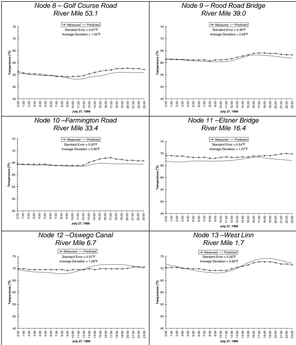
Figure A-47 (continued). Tualatin River Model Continuous Data Validation
