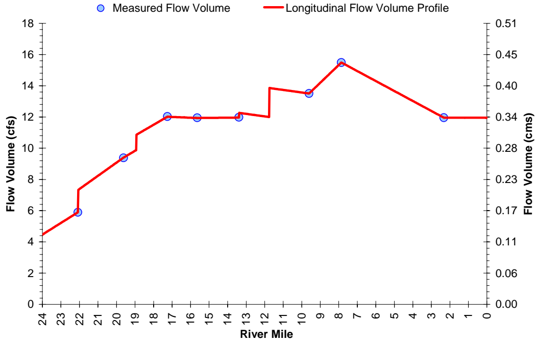
Figure A-65. Gales Creek Measured and Interpolated Longitudinal Flow Volume
