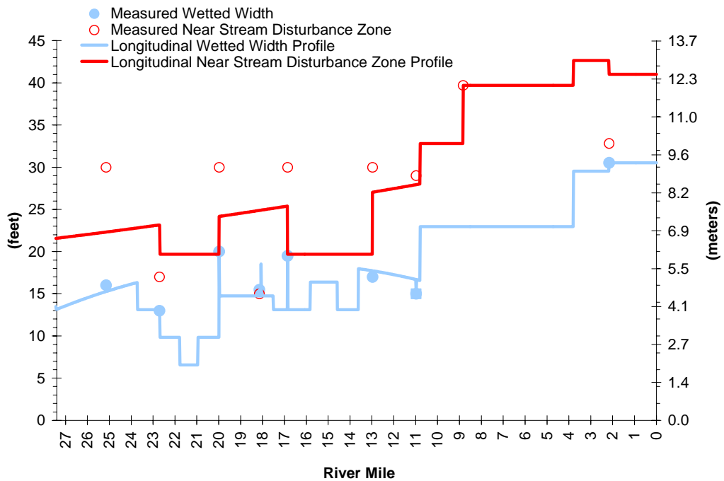
Figure A-108. West Fork Dairy Creek/Dairy Creek Wetted Widths and NSDZ Widths.
