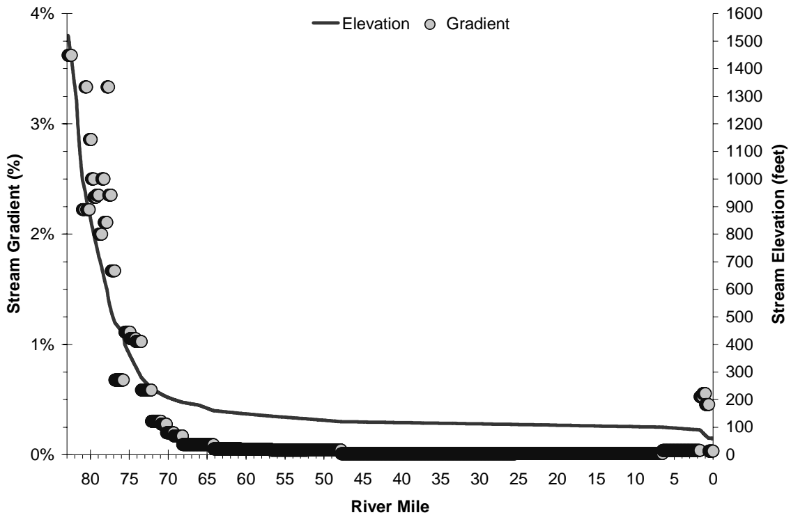
Figure A-38. Tualatin River Elevation and Gradient
