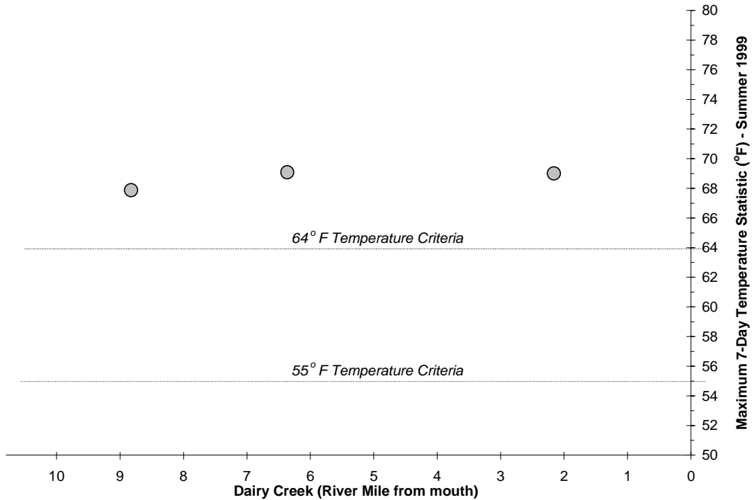
Figure A-102. Observed Maximum 7-Day Temperature Statistics for Dairy Creek.
