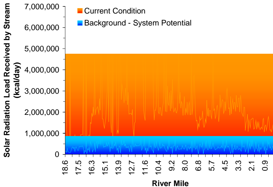
Figure A-90. East Fork Dairy Creek Solar Radiation Load at System Potential and Current Conditions
