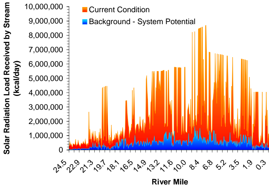
Figure A-70. Gales Creek Solar Radiation Load at System Potential and Current Conditions
