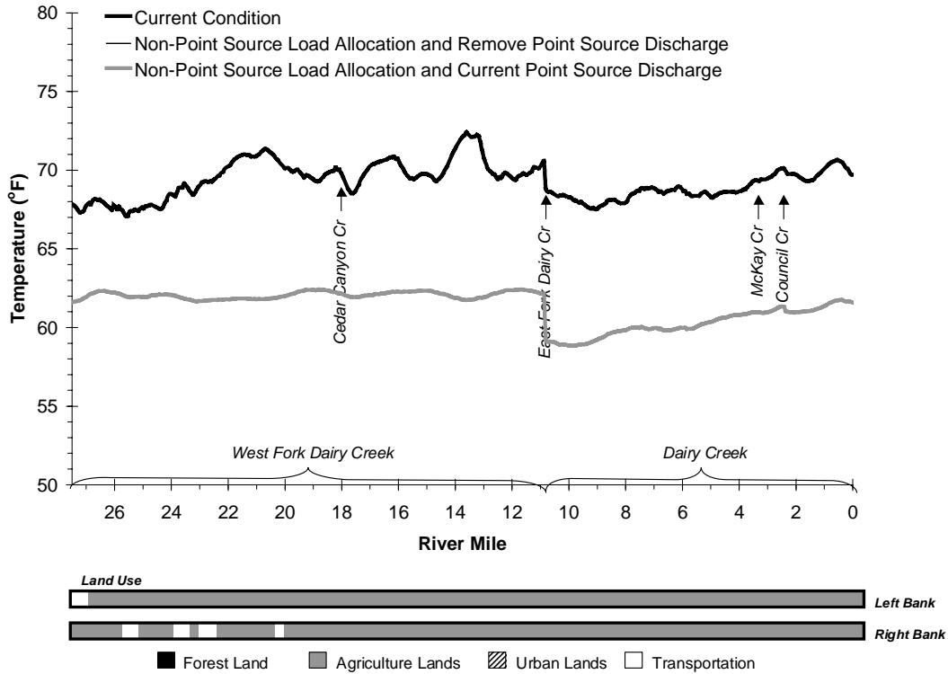
Figure A-120. WF Dairy Creek/Dairy Creek Longitudinal Temperature Profile - Model Output – 1) Non-Point Source Load Allocation and Current Point Source Discharge, and 2) Non-Point Source Load Allocation and Remove Point Source Discharge – 5:00 PM July 29, 1999.
