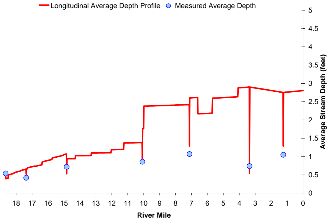
Figure A-87. East Fork Dairy Creek Measured and Mannings Derived Longitudinal Water Column Depths 9
