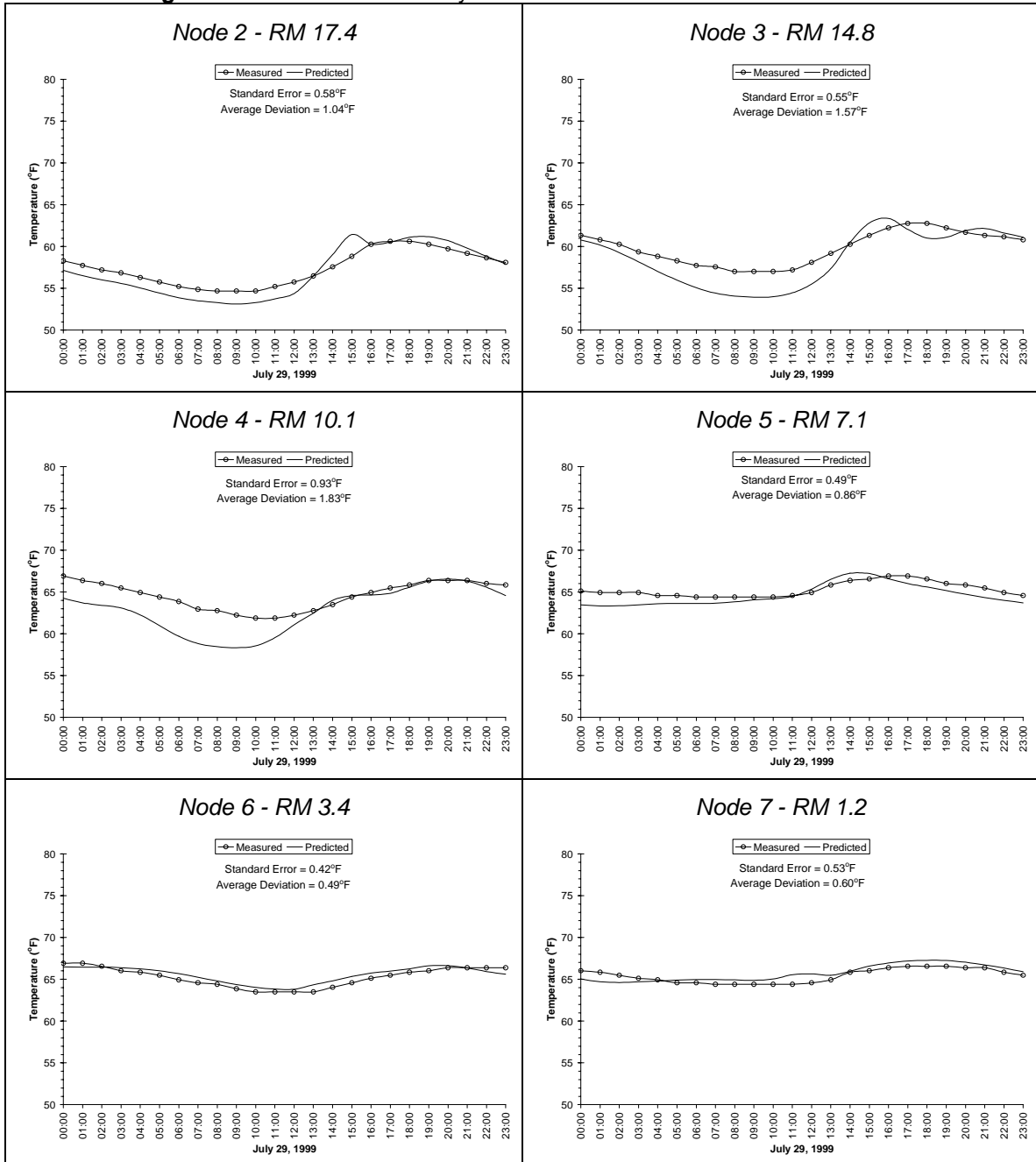
Figure A-89. East Fork Dairy Creek Model Continuous Data Validation.
