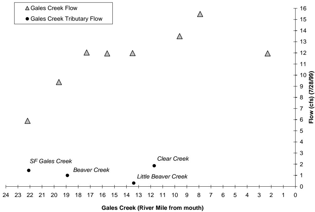
Figure A-58. Water discharge observed in Gales Creek on July 28, 1999.
