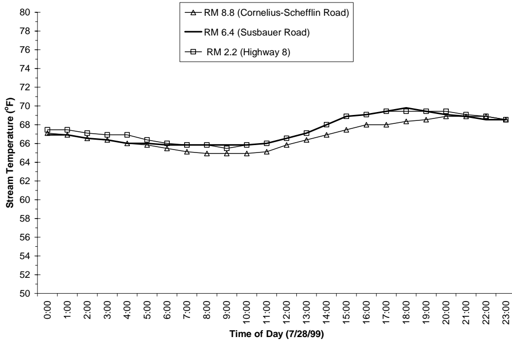
Figure A-103. Diurnal Temperature Trends Observed in Dairy Creek on July 28, 1999.
