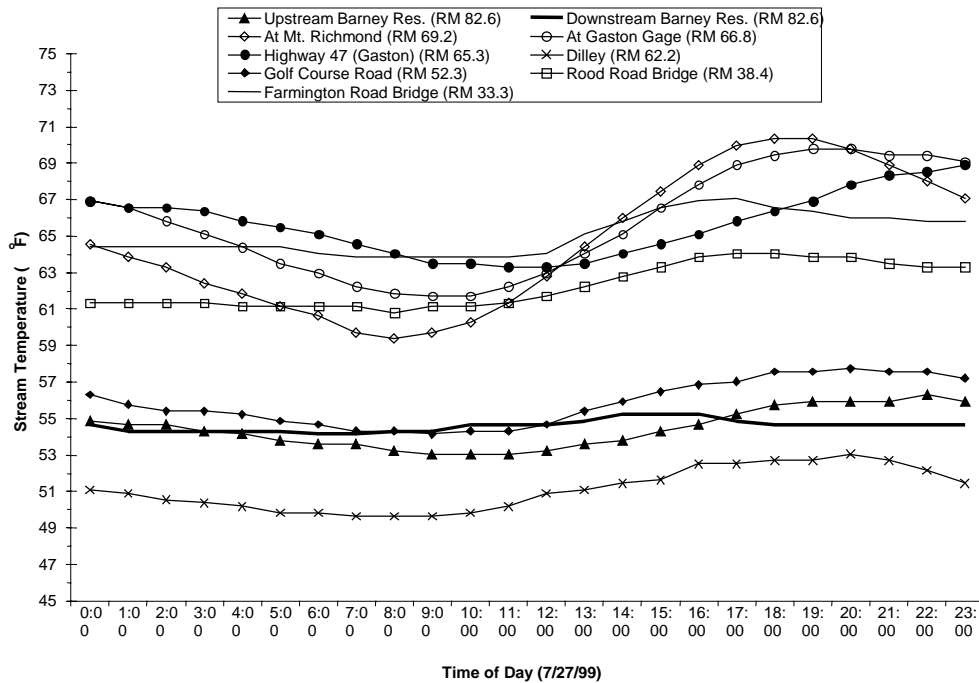
Figure A-35. Diurnal temperature trends observed in the Tualatin River on July 27, 1999.
