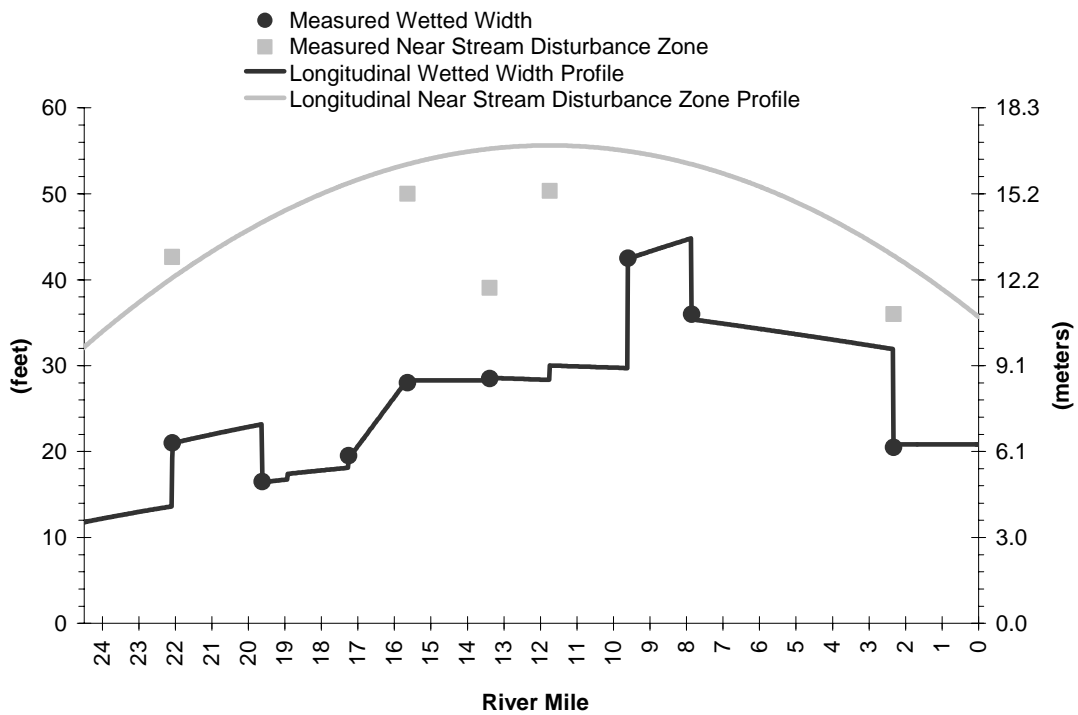
Figure A-62. Gales Creek NSDZ and Wetted Widths.
