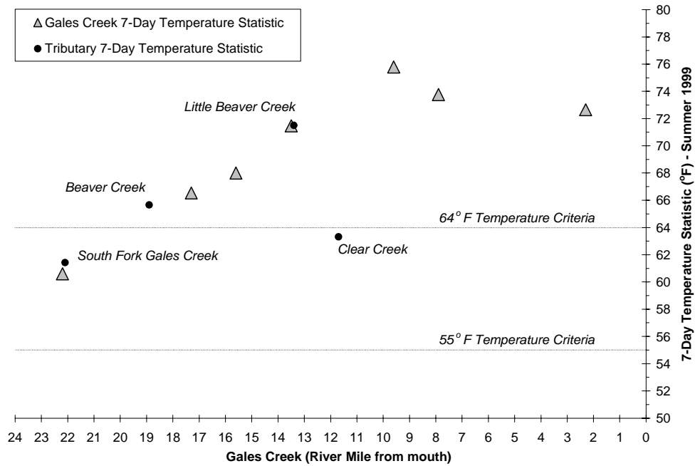
Figure A-56. Observed 7-Day temperature Statistics for Gales Creek during the summer of 1999.
