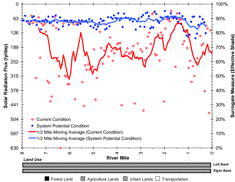
Figure A-168. Rock and Beaverton Creek Surrogate Measure for Non Point Sources - Effective Shade.
