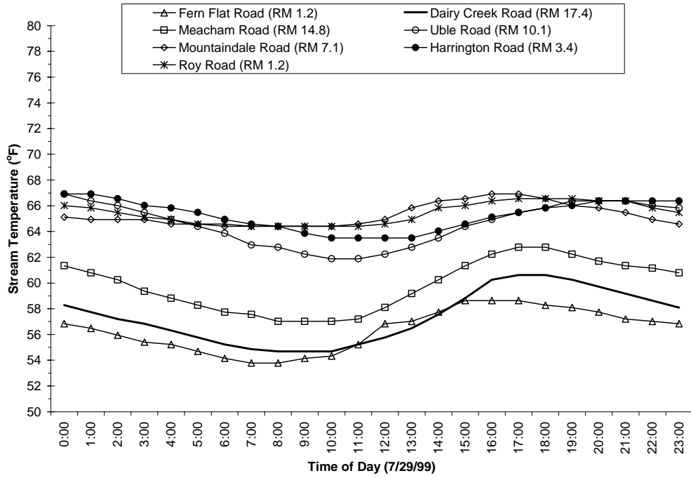
Figure A-77. Diurnal Temperature Trends Observed in East Fork Dairy Creek on July 29, 1999.
