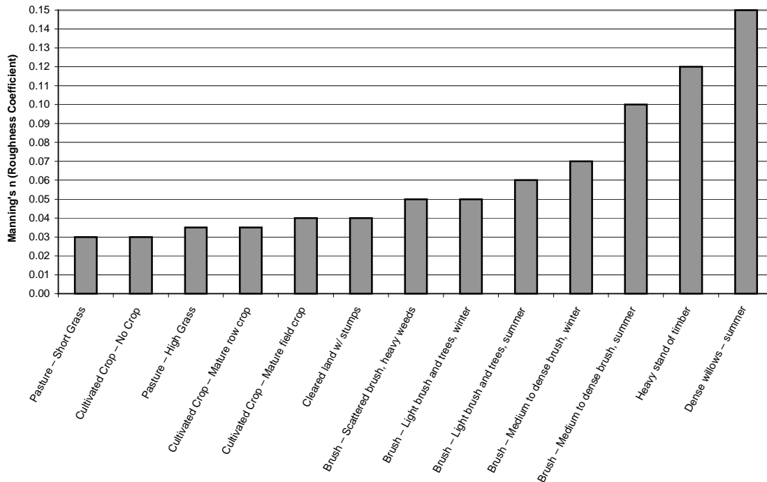
Figure A-17. Manning's n (Roughness Coefficient) Related to Riparian Vegetation
