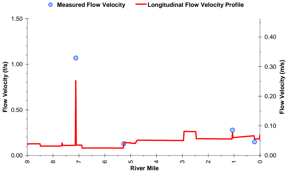
Figure A-185. Fanno Creek Measured and Mannings Derived Longitudinal Flow Velocities.
