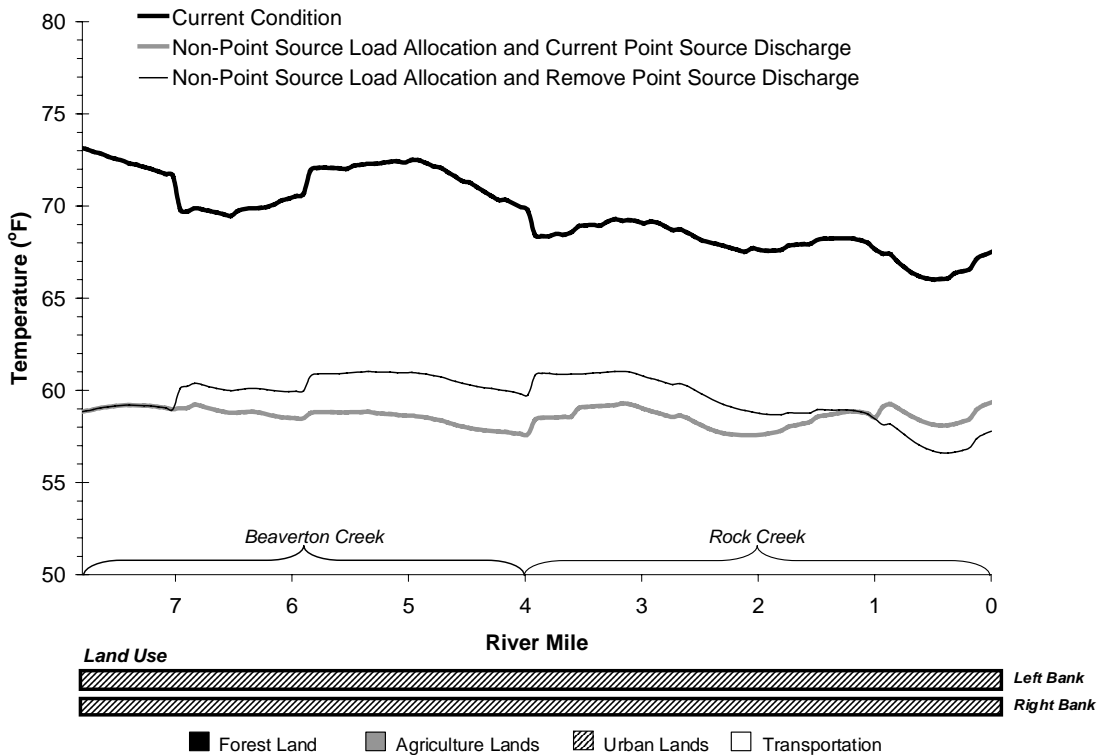
Figure A-169. Rock Creek/Beaverton Creek Longitudinal Temperature Profile - Model Output – 1) Non-Point Source Load Allocation and Current Point Source Discharge, and 2) Non-Point Source Load Allocation and Remove Point Source Discharge – 5:00 PM July 30, 1999.
