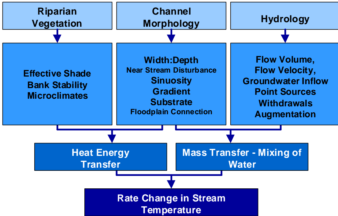
Figure A-1. Stream Heating Processes in the Tualatin River Subbasin
