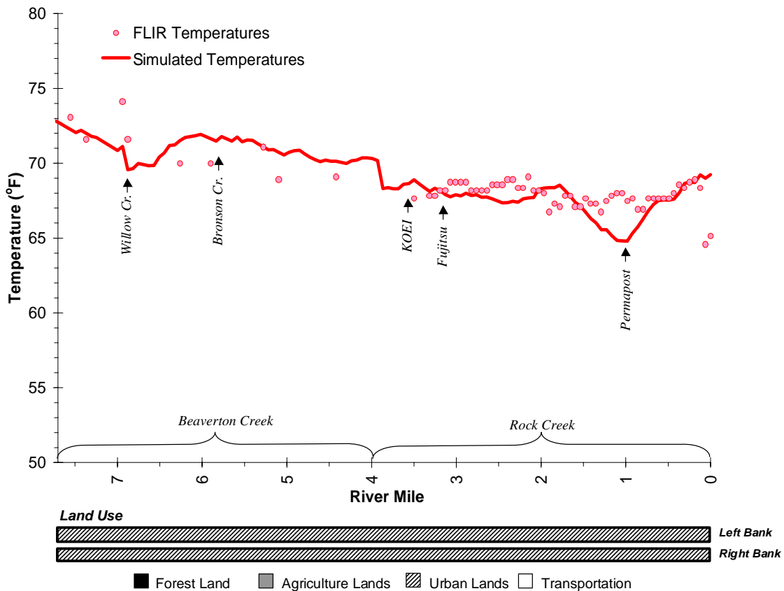
Figure A-165. Rock and Beaverton Creek Observed and Predicted Spatial Temperature Data.
