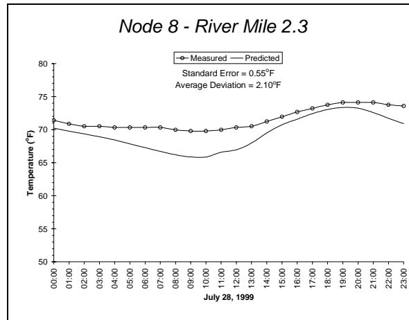
Figure A-69 (continued). Gales Creek Model Continuous Data Validation
