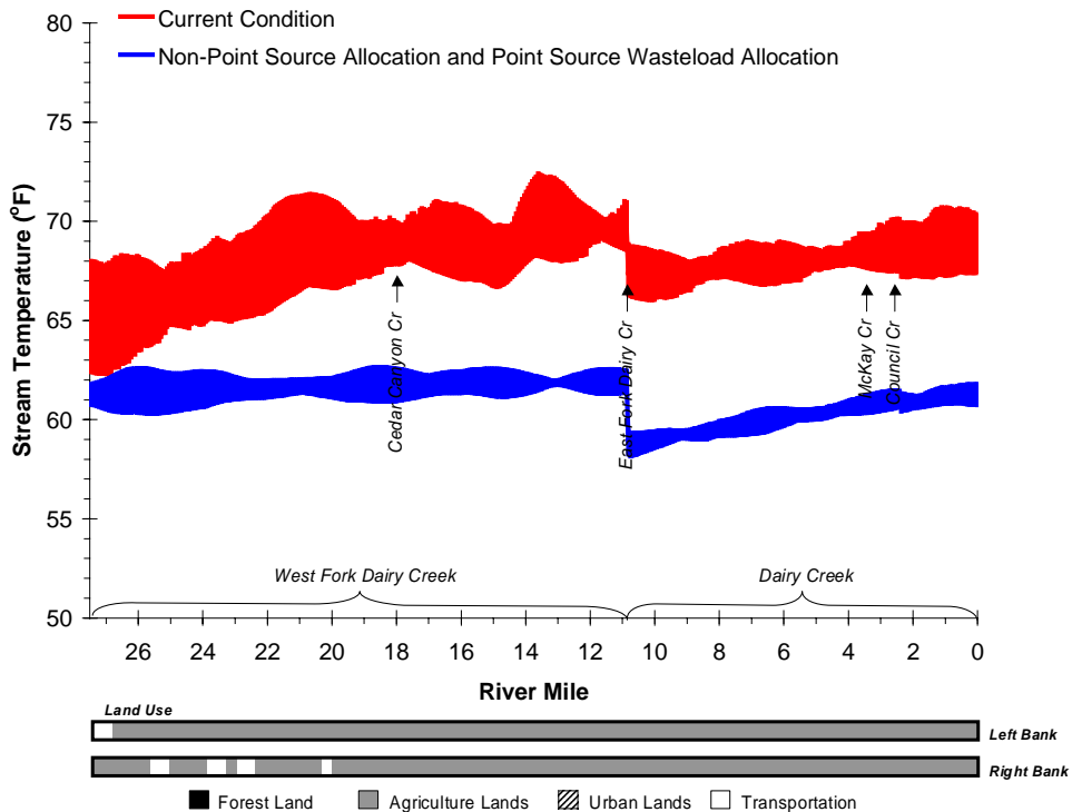
Figure A-122. West Fork Dairy Creek/Dairy Creek Daily Temperature Range for Current Conditions Compared with Allocated Measures - July 28, 1999.
