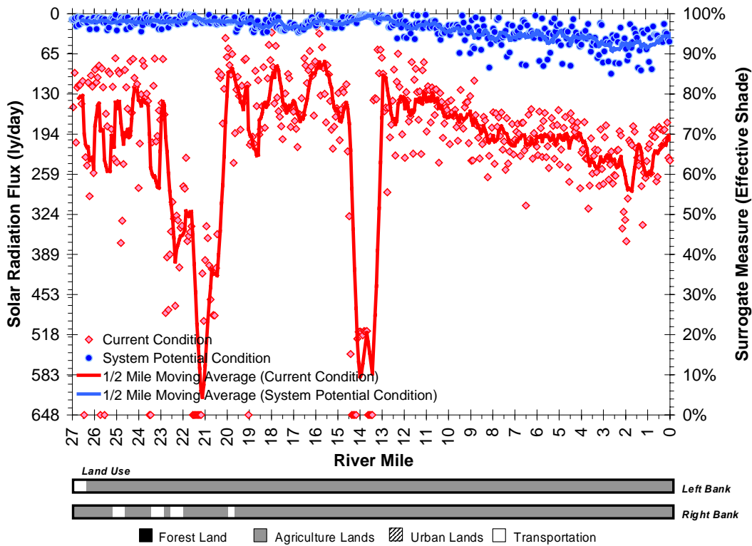
Figure A-119. West Fork Dairy Creek/Dairy Creek Surrogate Measure for Non Point Sources - Effective Shade.
