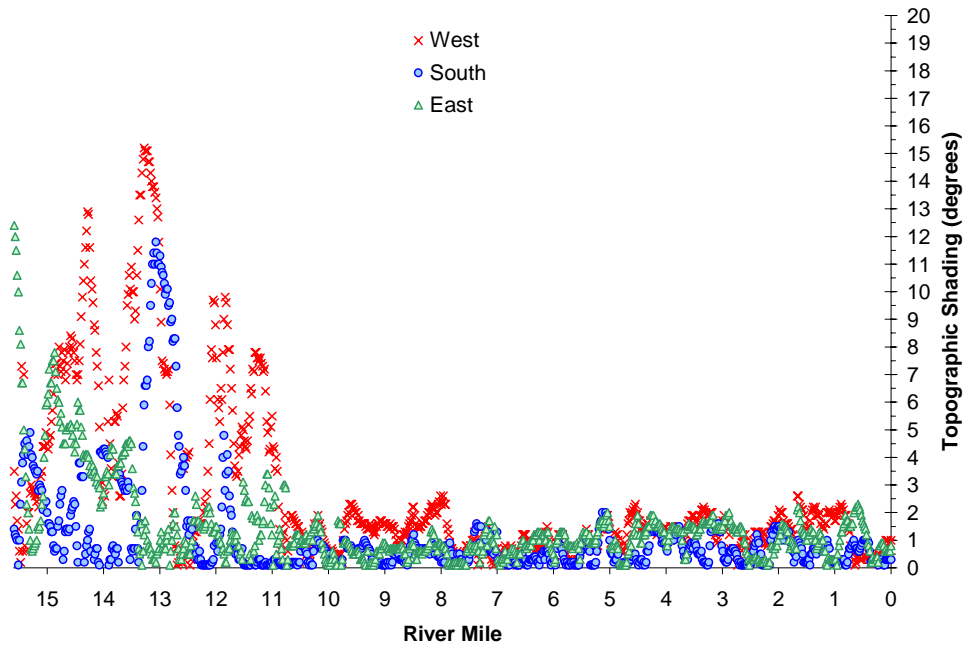
Figure A-133. McKay Creek Topographic Shade at Each 100-foot Model Reach.
