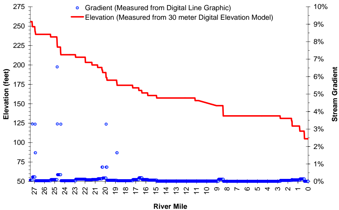
Figure A-106. West Fork Dairy/Dairy Creek Elevation and Gradient at Each 100-foot Model Reach.
