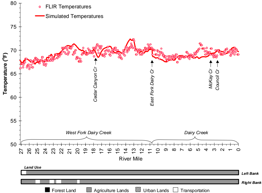
Figure A-116. West Fork Dairy Creek/Dairy Creek Observed and Predicted Spatial Temperature Data.
