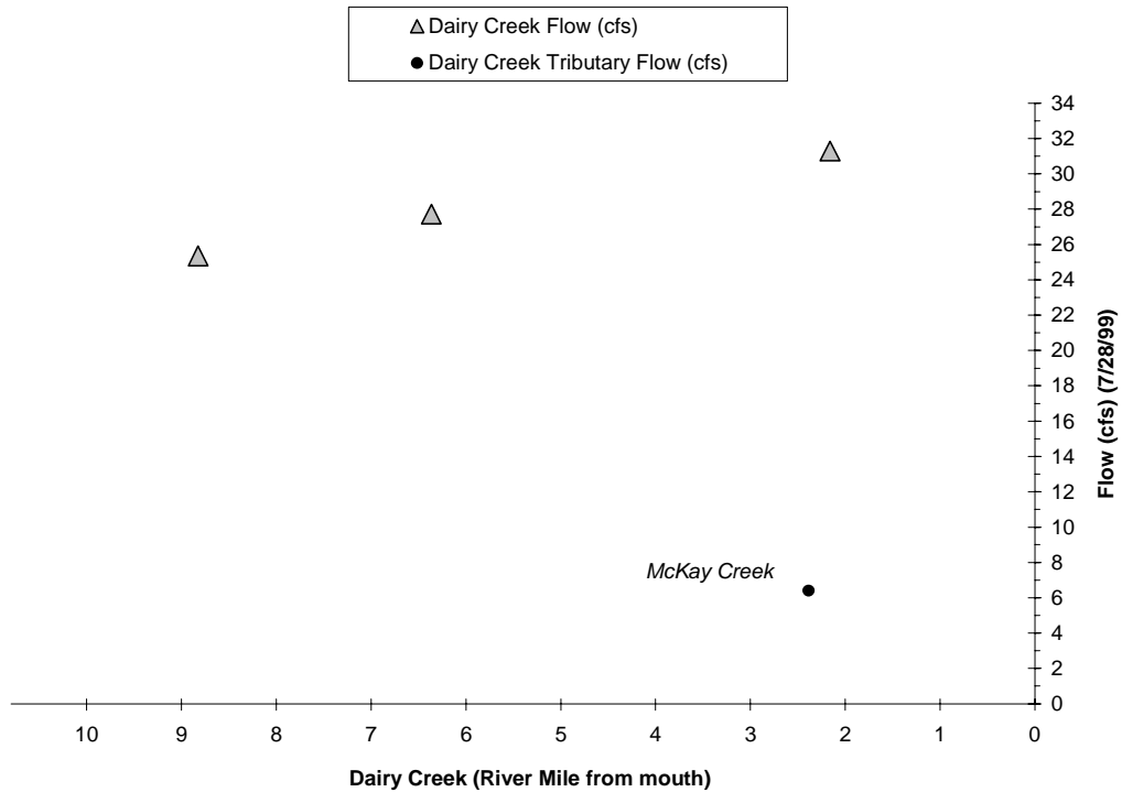
Figure A-104. Stream Flow Observed in Dairy Creek on July 28, 1999.
