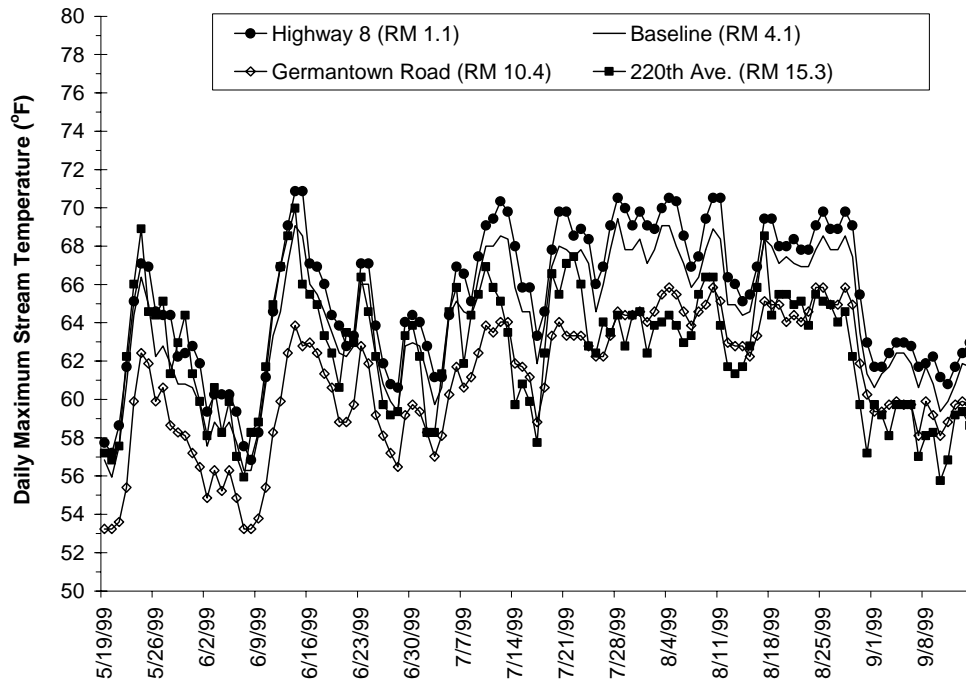
Figure A-147. Observed daily maximum temperatures for Rock Creek in 1999.
