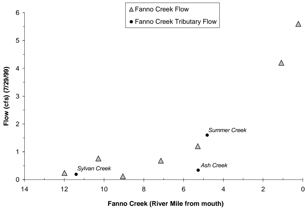
Figure A-177. Water discharge observed in Fanno Creek on July 29, 1999.
