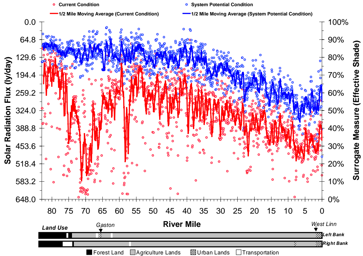
Figure A-49. Tualatin River Surrogate Measure for Non Point Sources – Effective Shade
