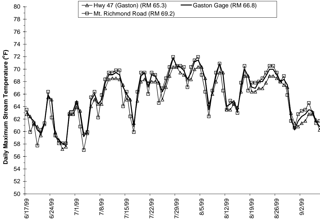
Figure A-33. Observed daily maximum temperatures for the Tualatin River in 1999.
