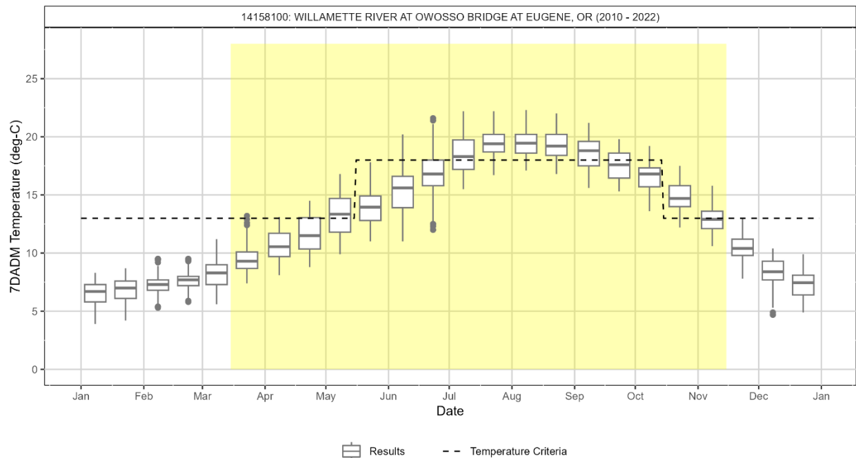
Figure 5-53: Seasonal variation on the Willamette River at Owosso Bridge at Eugene (RM 178.8, 3 miles upstream from McKenzie R) in the Upper Willamette Subbasin.
