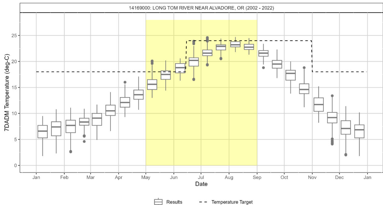
Figure 4-5: Boxplots of bi-monthly 7DADM temperatures for the Long Tom River at USGS station 14169000 near Alvadore, OR. Dashed line is the temperature targets of 24.0°C from June 15 to October 31 and 18.0°C from November 1 to June 14. Yellow shading indicates time periods when the targets are exceeded under current conditions.
