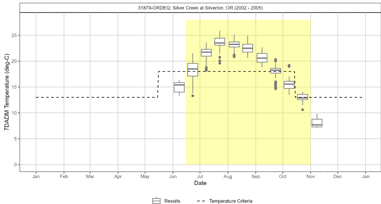
Figure 5-39: Seasonal variation at the Silver Creek at Silverton, Oregon temperature monitoring site in the Molalla-Pudding Subbasin.
