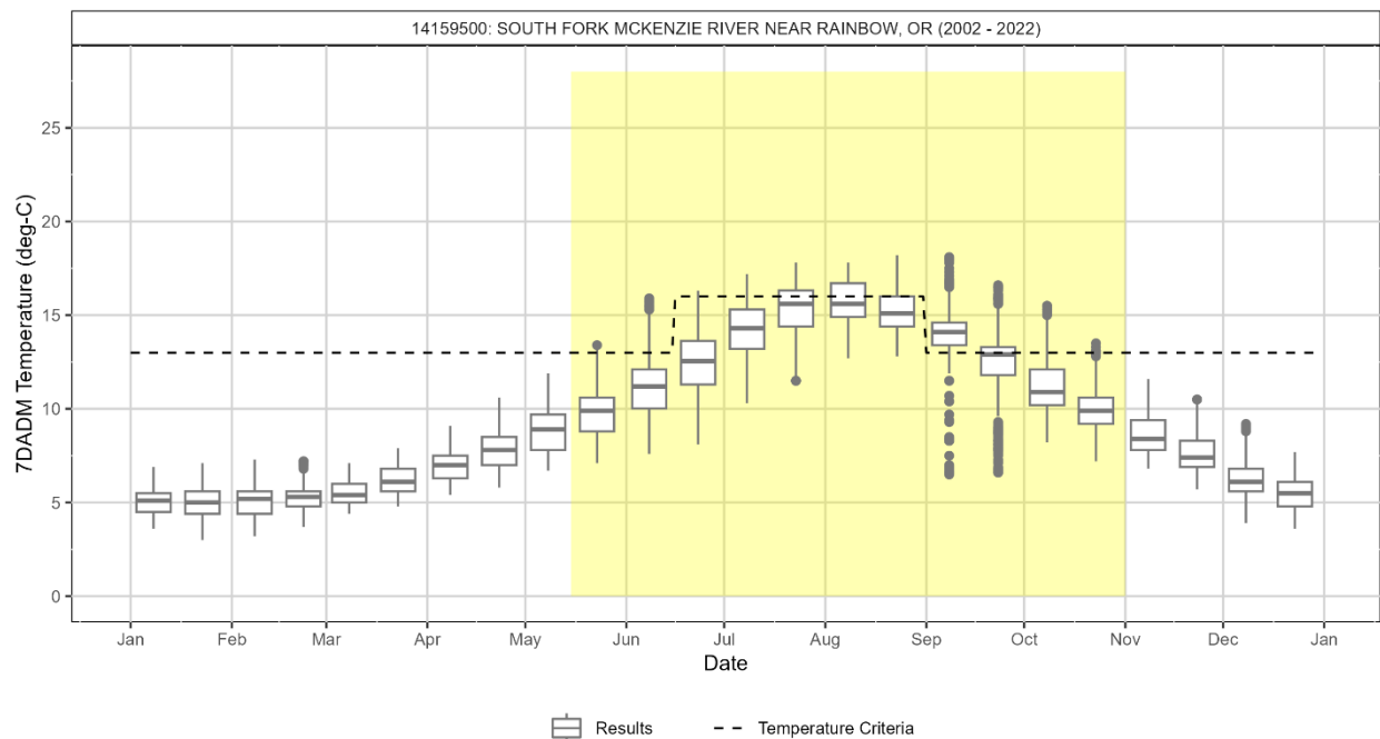
Figure 5-24: Seasonal variation at South Fork McKenzie River near Rainbow (RM 4, just downstream from Cougar Dam) in the McKenzie Subbasin.
