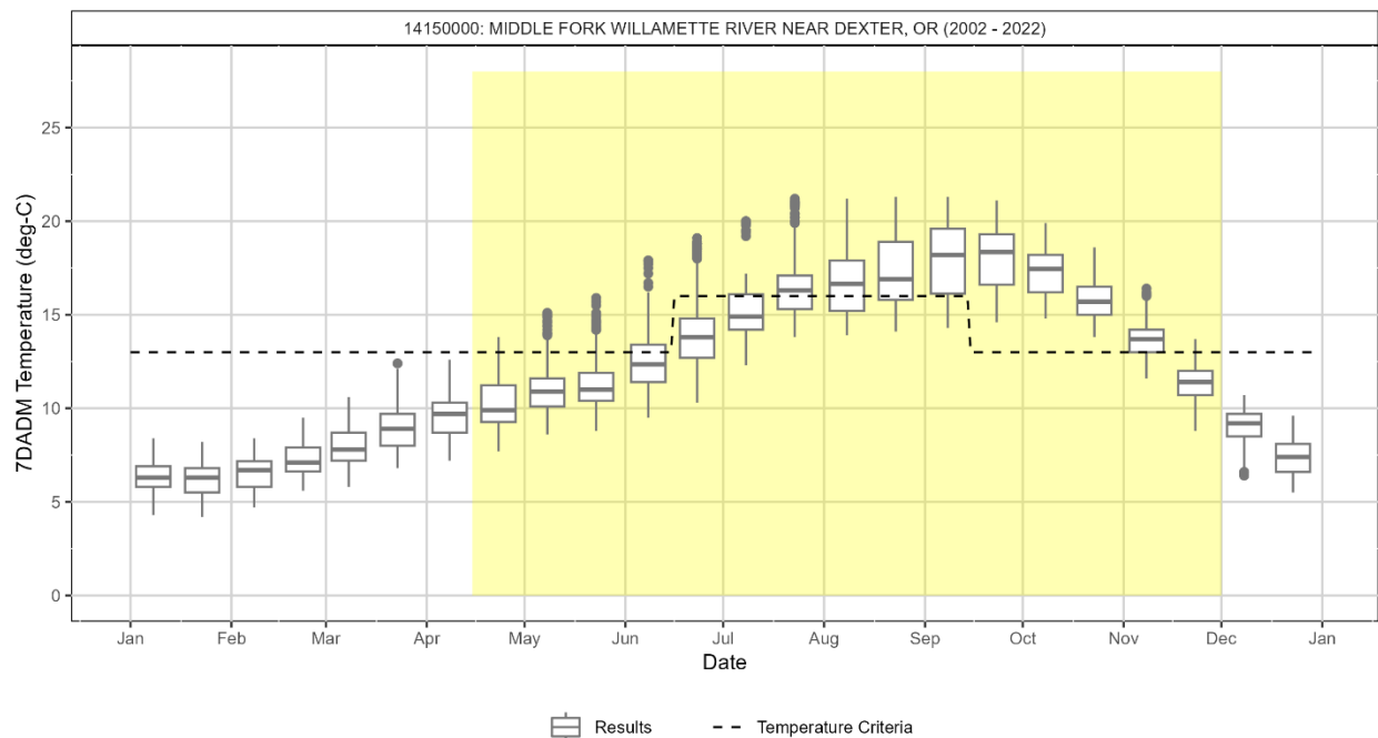
Figure 5-5: Seasonal variation on the Middle Fork Willamette River near Dexter (about 2.5 miles downstream from Dexter Dam at Willamette River RM 201.3) in the Middle Fork Willamette Subbasin.
