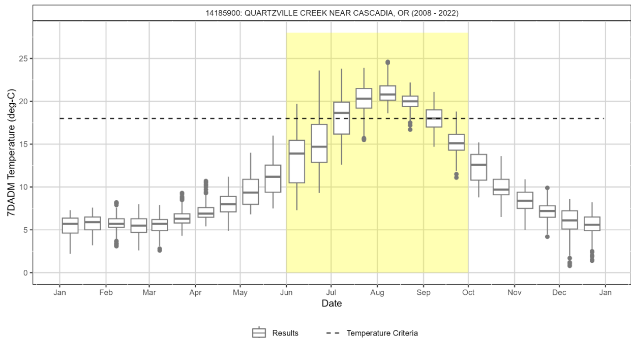
Figure 5-29: Seasonal variation at the Quartzville Creek Near Cascadia monitoring site (upstream of Green Peter Dam) in the South Santiam Subbasin.
