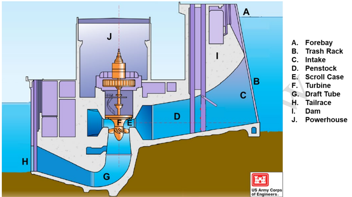
Figure 2-3: Dam Cross Section Diagram
