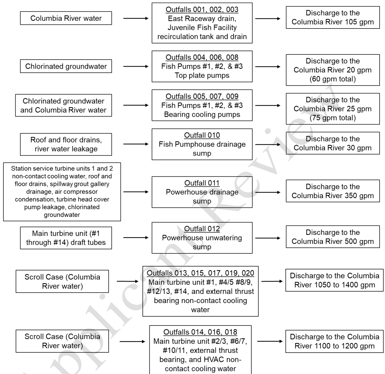
Figure 2-2: Facility Line Drawing
