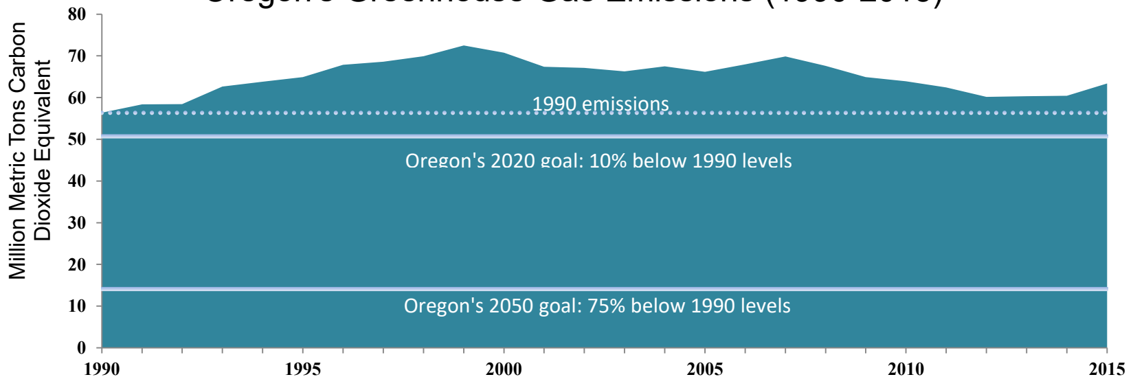
Oregon's Greenhouse Gas Emissions (1990-2015)
