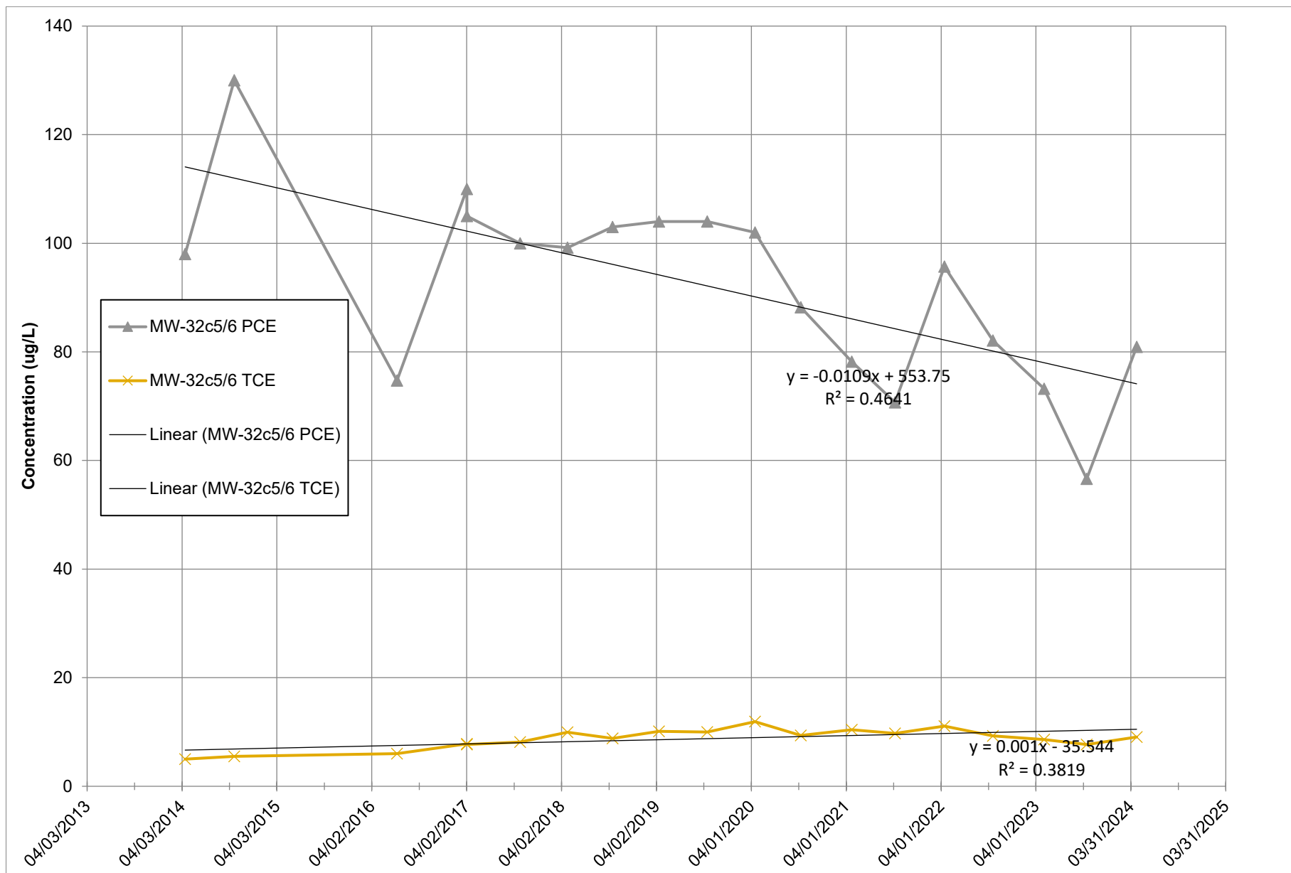
Figure MW-32c5/6 Intermediate PCE and TCE in Groundwater Former Springville Dry Cleaner
