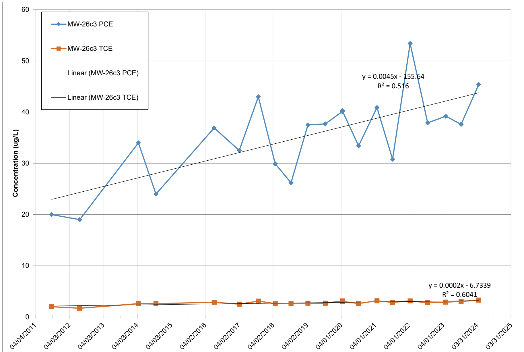
Figure MW-26c3 Intermediate PCE and TCE in Groundwater Former Springville Dry Cleaner
