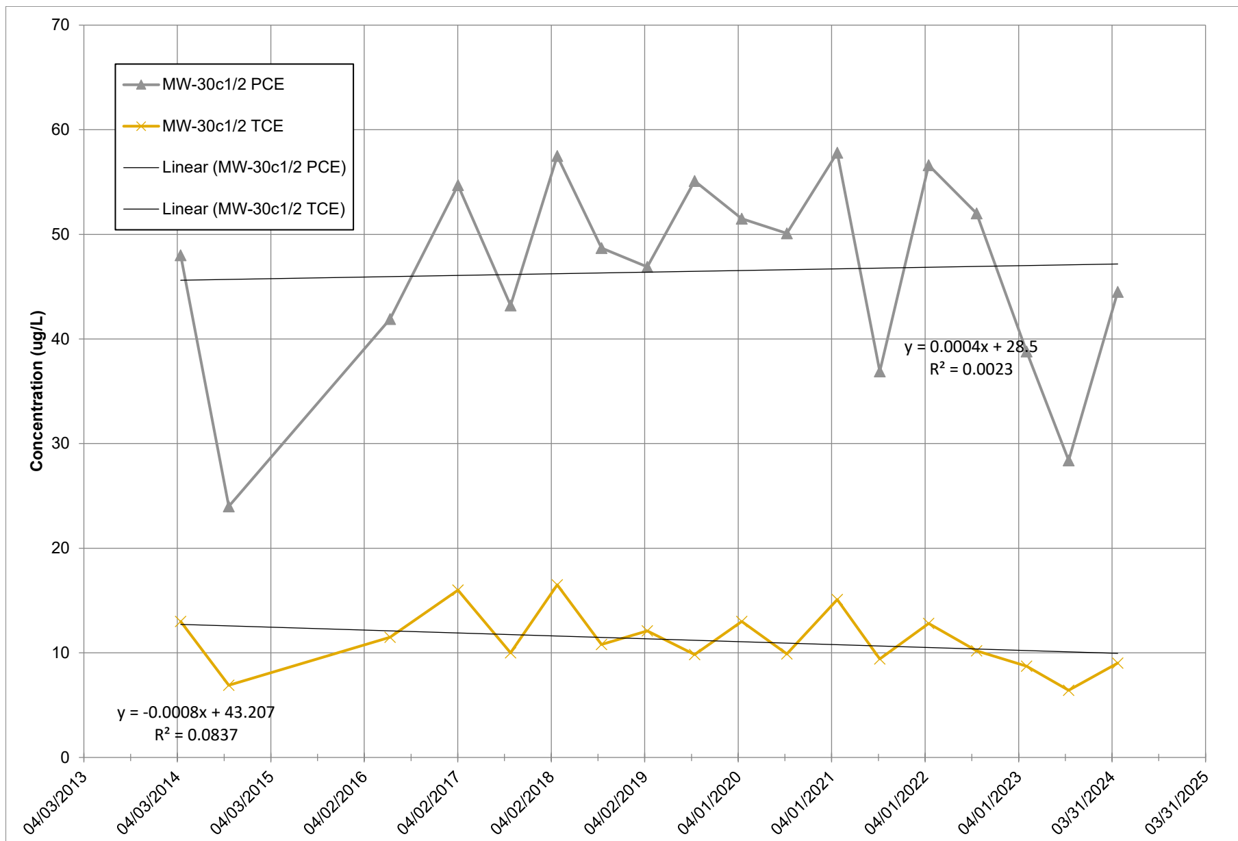
Figure MW-30c1/2 Intermediate PCE and TCE in Groundwater Former Springville Dry Cleaner
