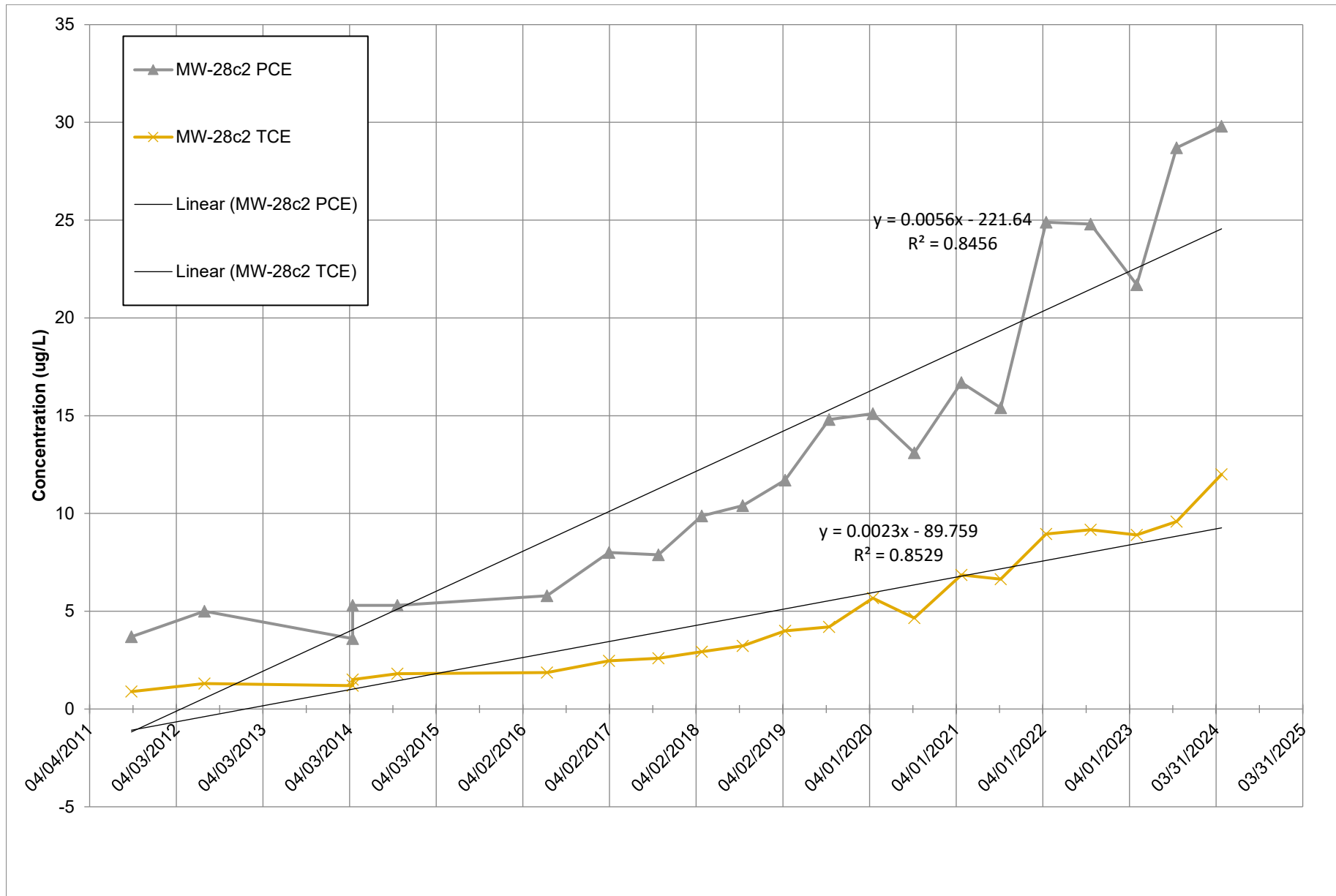
Figure MW-28c2 Intermediate PCE and TCE in Groundwater Former Springville Dry Cleaner
