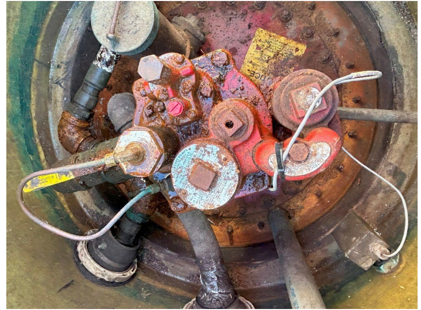
16: Tank top sump #2
