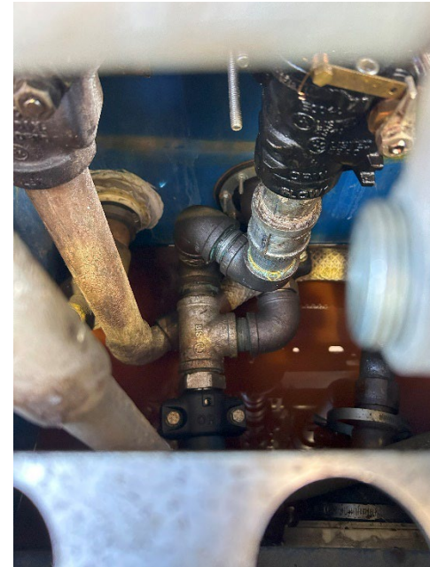
26: UDC – Dispensers 5 & 6 – Liquid in bottom, product mixed with water.
