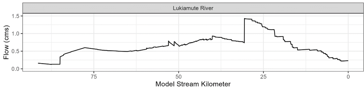
Figure 3-160: Boundary condition and mainstem flow inputs to the Luckiamute River model.
