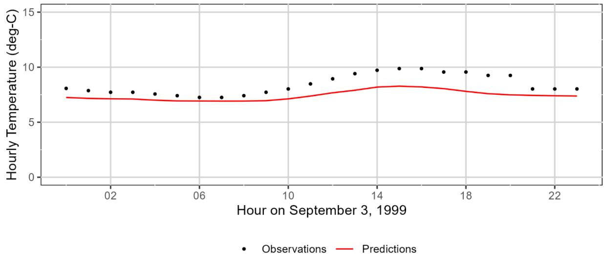
Figure 3-209: Upper McKenzie River measured and model-predicted hourly temperatures at monitoring station 14158850.
