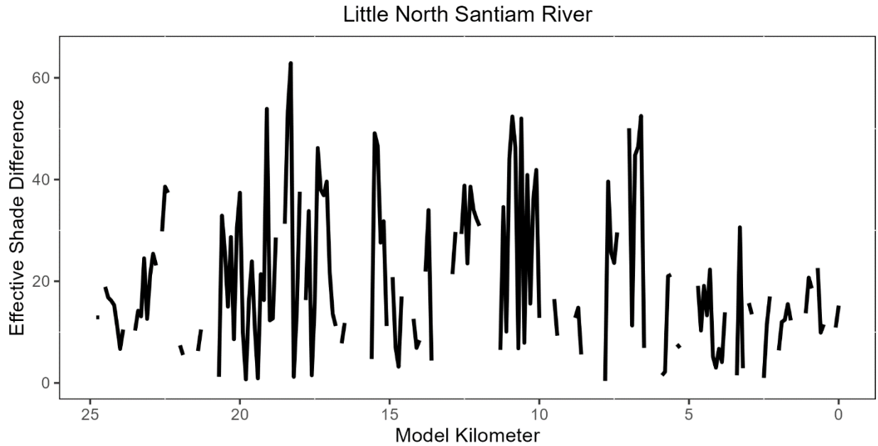
Figure 4-51: Percentage point difference between effective shade from the Current Condition and Restored Vegetation scenarios on 8/1/2000 for the Little North Santiam River. Missing values indicate that the shade difference is negative due to instances of higher effective shade in the Current Condition scenario versus the Restored Vegetation scenario.
