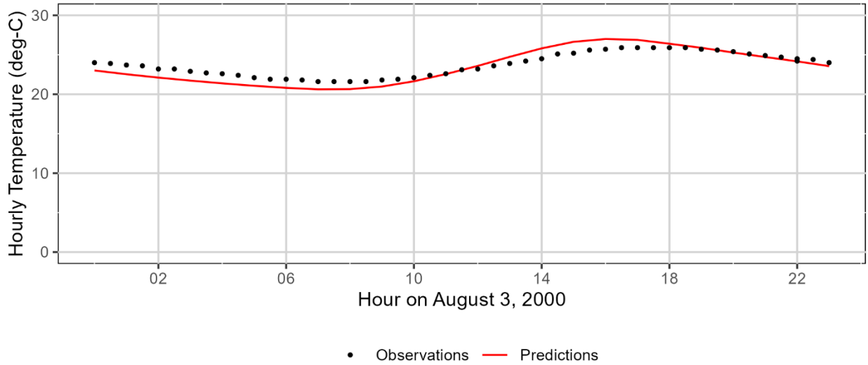
Figure 3-123: Thomas Creek measured and model-predicted hourly temperatures at monitoring station 10783-ORDEQ.
