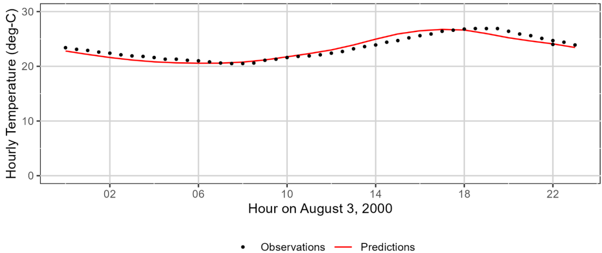
Figure 3-124: Thomas Creek measured and model-predicted hourly temperatures at monitoring station 23785-ORDEQ.
