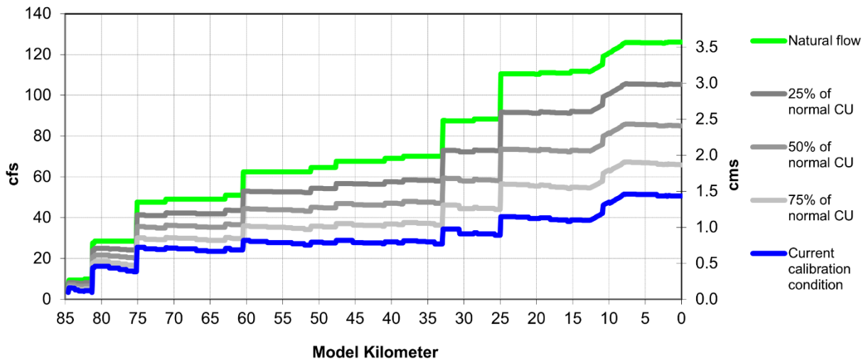
Figure 4-32: Median 7-day average stream flow rates for all Pudding River consumptive use model scenarios.
