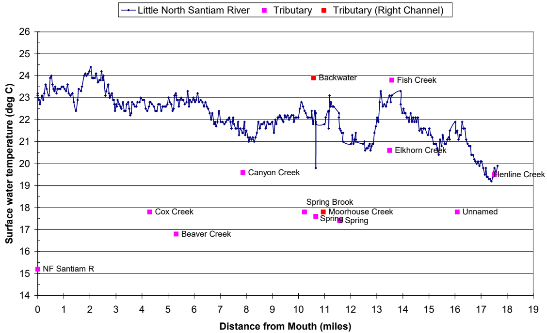
Figure 2-7: TIR temperatures for the Little North Santiam River in the North Santiam Subbasin.
