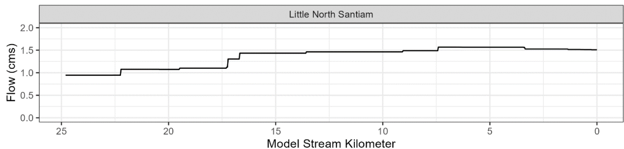
Figure 3-100: Boundary condition and mainstem flow inputs to the Little North Santiam River model.
