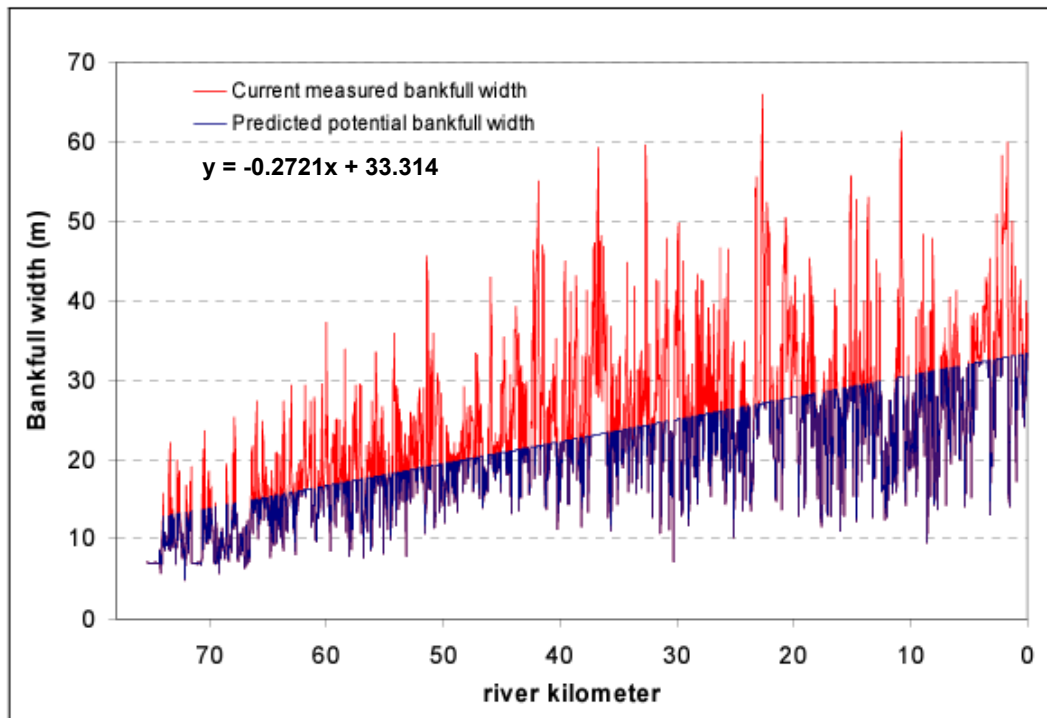
Figure 4-10: GIS measured bankfull width compared with predicted bankfull width. A regression was performed of the moving median of bankfull width from headwaters to mouth. Modified bankfull width entered into the Heat Source model was the measured width, or the predicted width, the demarcating line in this figure, whichever was less.
