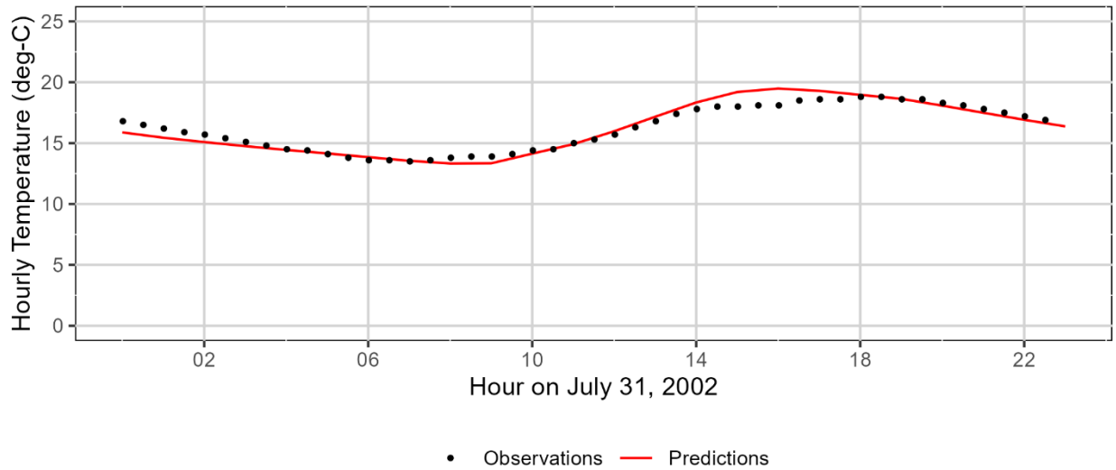
Figure 3-19: Johnson Creek measured and model-predicted hourly temperatures at monitoring station 11626-ORDEQ.
