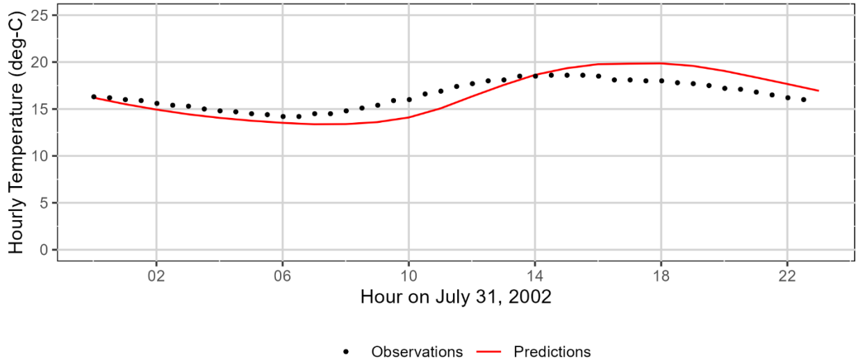
Figure 3-20: Johnson Creek measured and model-predicted hourly temperatures at monitoring station 28730-ORDEQ.
