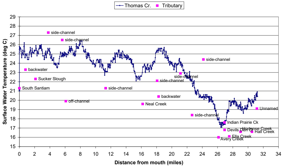
Figure 2-8: TIR Temperatures for Thomas Creek in the South Santiam Subbasin.
