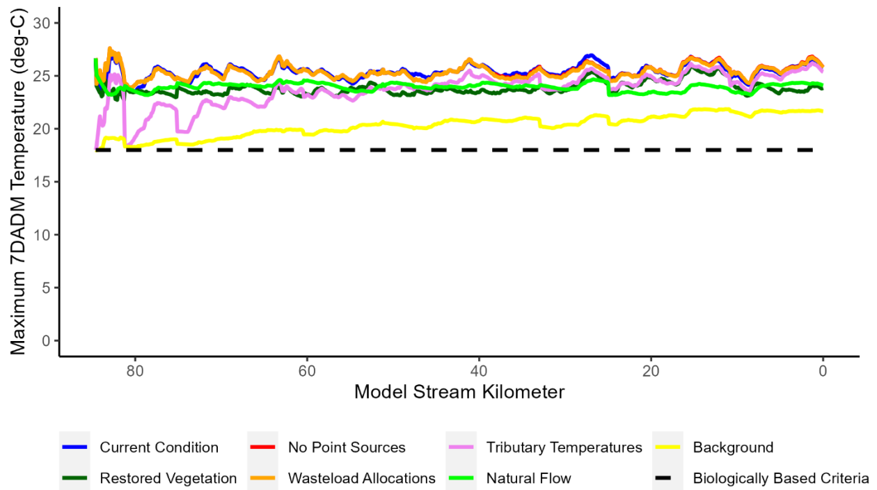
Figure 4-19: Maximum 7DADM stream temperature for all model scenarios for the Pudding River.
