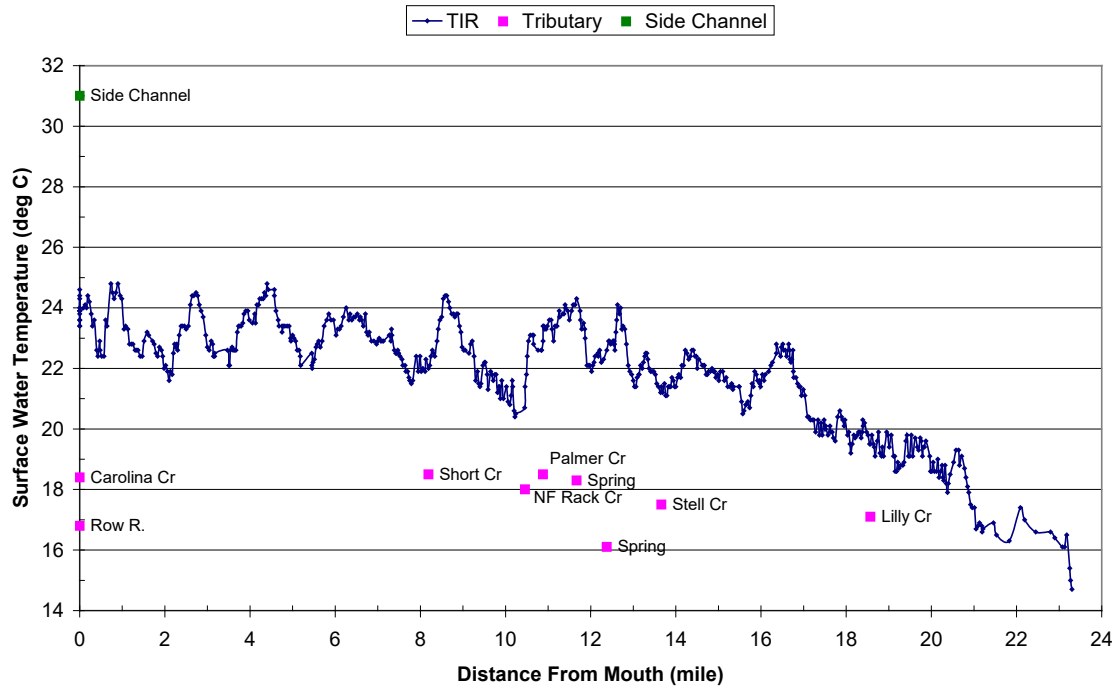
Figure 2-9: TIR temperatures for Mosby Creek in the Coast Fork Willamette Subbasin.
