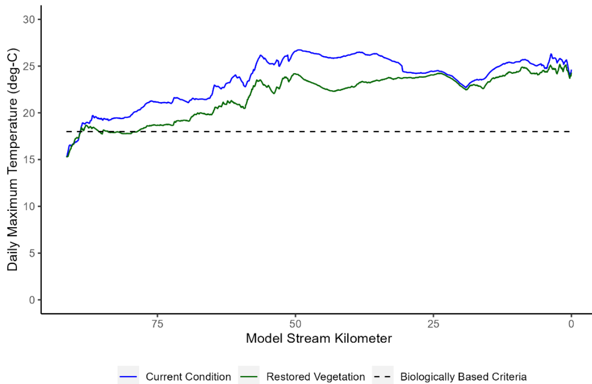
Figure 4-63: Daily maximum stream temperature for the Current Condition and Restored Vegetation model scenarios for the Luckiamute River.
