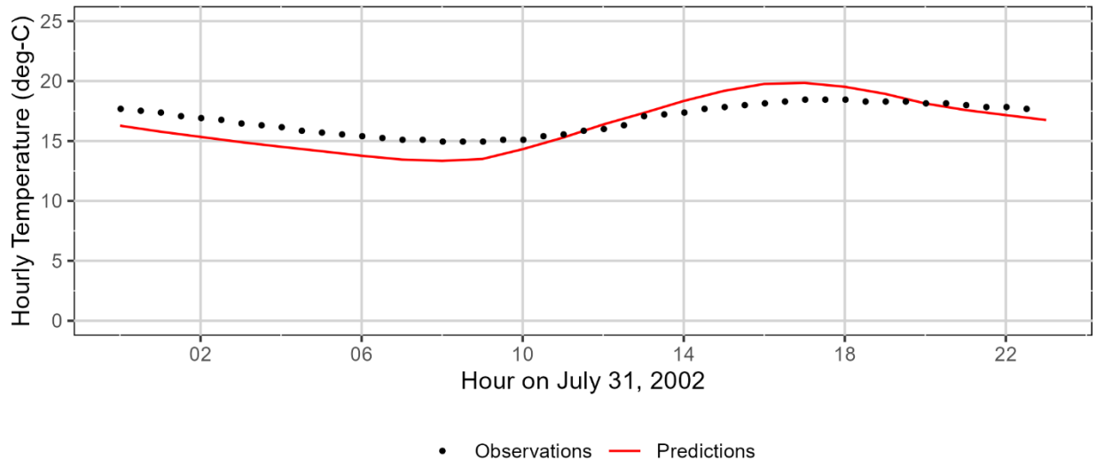
Figure 3-18: Johnson Creek measured and model-predicted hourly temperatures at monitoring station 11327-ORDEQ.
