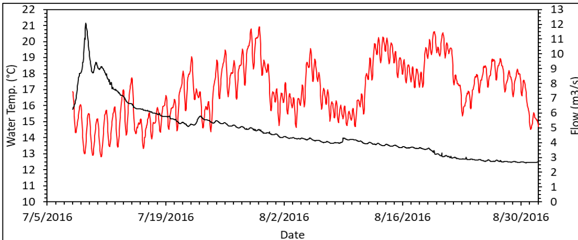
Figure 7-1: No dams scenario temperature and flow time-series, Bull Run River mouth.
