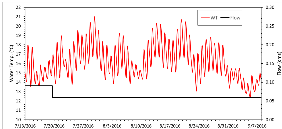
Figure 5-5: WLA_B scenario: ODFW Sandy R. fish hatchery discharge rates and temp. to the Sandy R.
