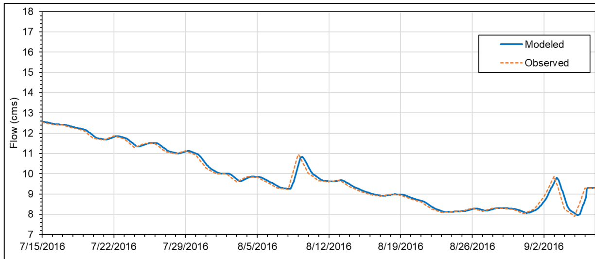
Figure 4-2: Modeled and observed flows, Sandy R. Near Marmot (USGS 14137000, RKM 48.05)
