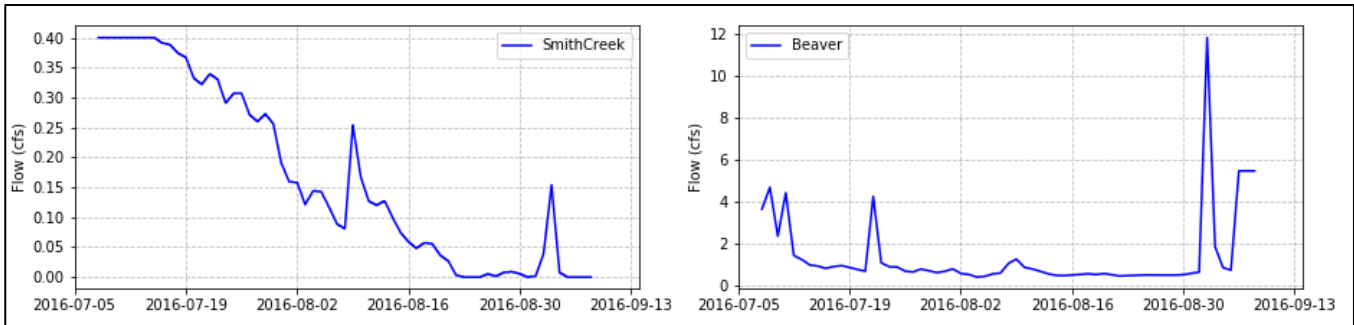
Figure 3-17: Estimated longitudinal flows for model tributaries, 2016 model period
