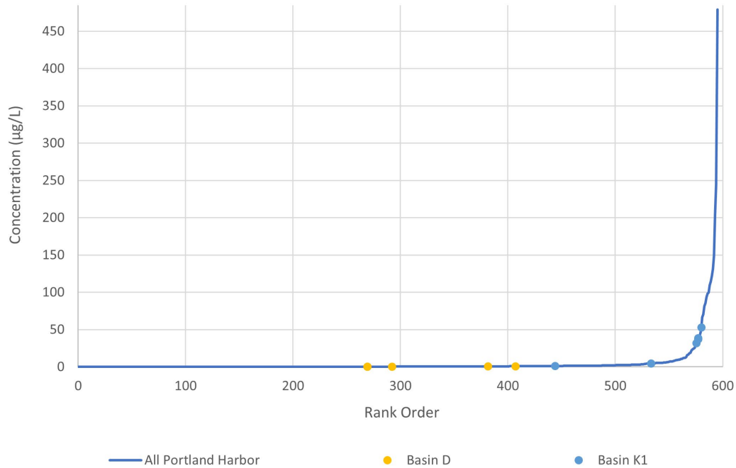
Figure A - 1. Total PAHs in Stormwater at T4 Compared to “Typical” Industrial Stormwater in the Portland Harbor
