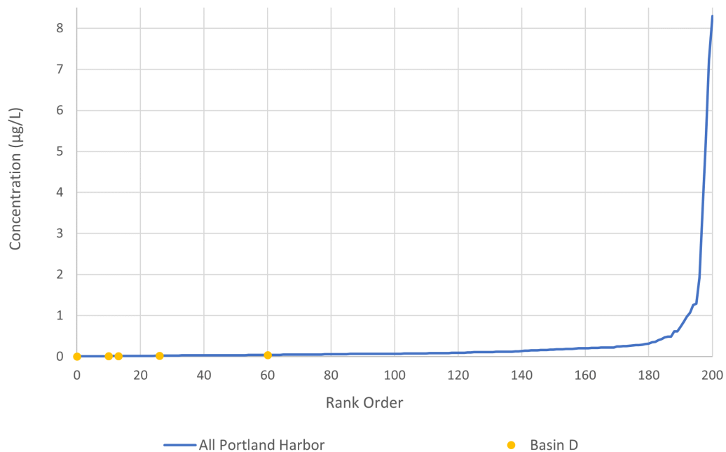
Figure A - 12. Silver in Stormwater at T4 Compared to “Typical” Industrial Stormwater in the Portland Harbor
