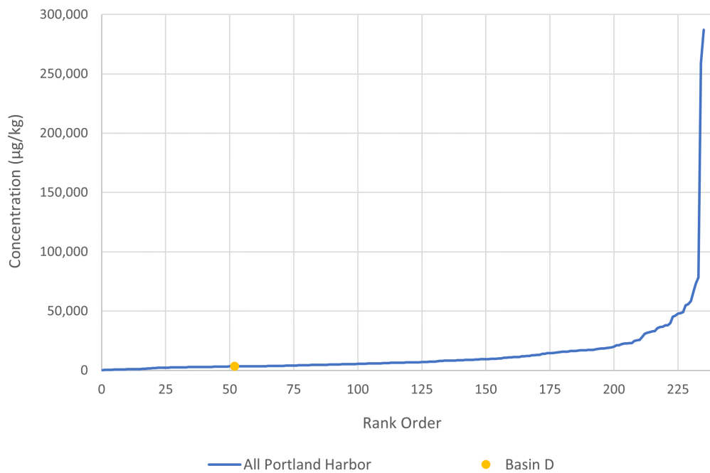
Figure A - 18. Arsenic in Stormwater Solids at T4 Compared to “Typical” Industrial Stormwater in the Portland Harbor
