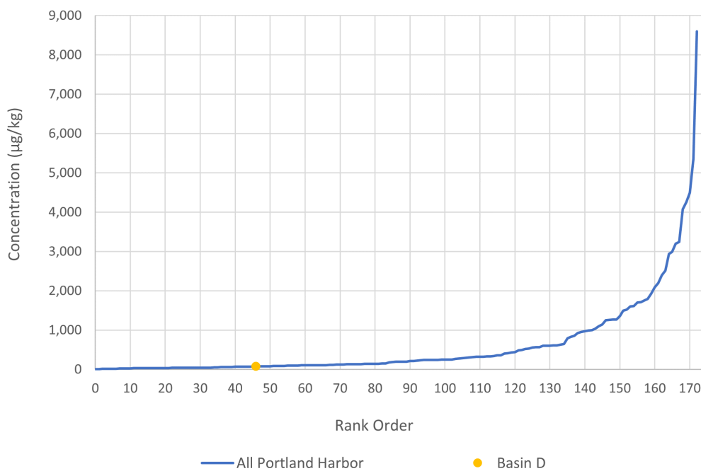
Figure A - 23. Mercury in Stormwater Solids at T4 Compared to “Typical” Industrial Stormwater in the Portland Harbor
