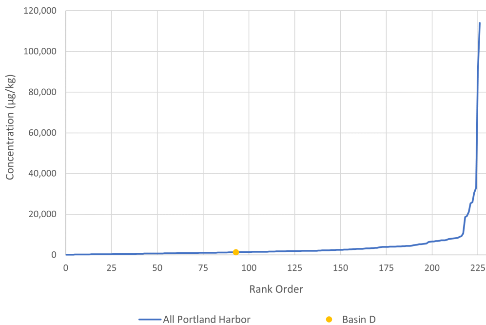
Figure A - 19. Cadmium in Stormwater Solids at T4 Compared to “Typical” Industrial Stormwater in the Portland Harbor
