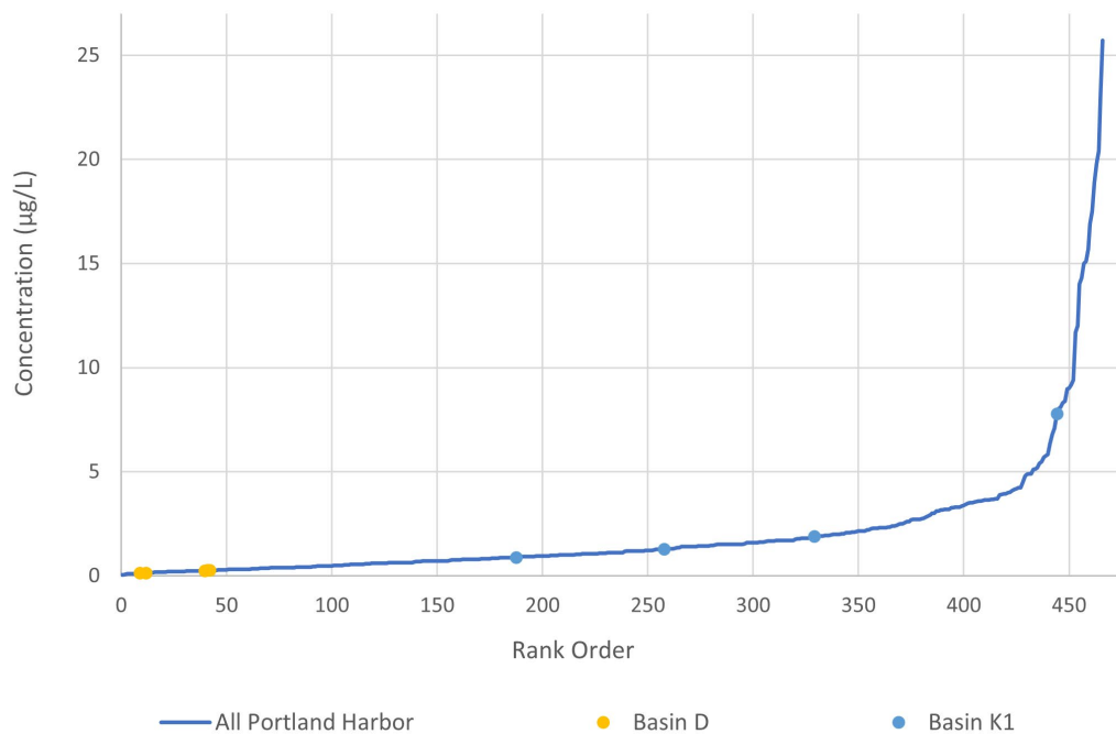
Figure A - 5. Arsenic in Stormwater at T4 Compared to “Typical” Industrial Stormwater in the Portland Harbor
