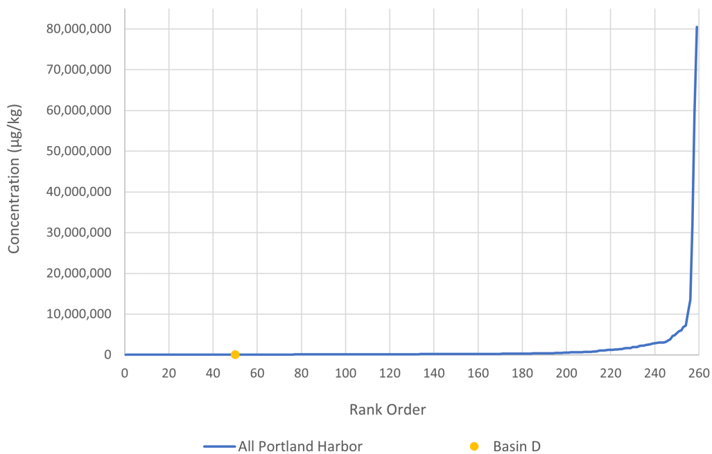
Figure A - 21. Copper in Stormwater Solids at T4 Compared to “Typical” Industrial Stormwater in the Portland Harbor
