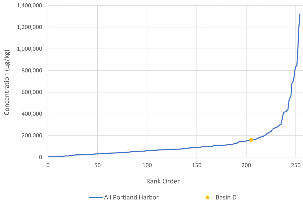
Figure A - 20. Chromium in Stormwater Solids at T4 Compared to “Typical” Industrial Stormwater in the Portland Harbor
