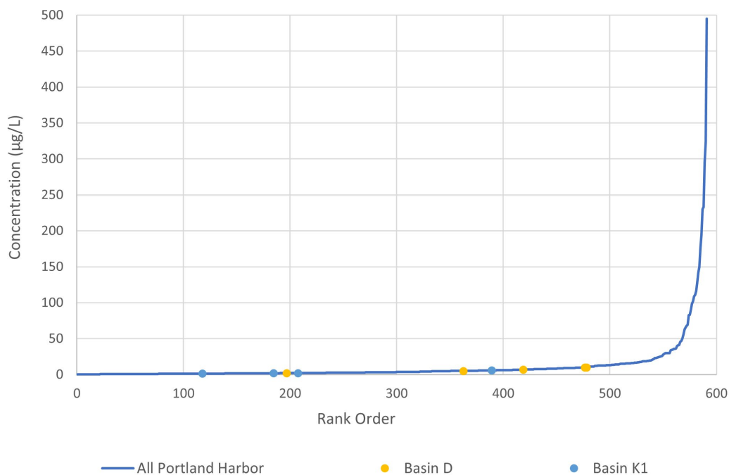
Figure A - 7. Chromium in Stormwater at T4 Compared to “Typical” Industrial Stormwater in the Portland Harbor
