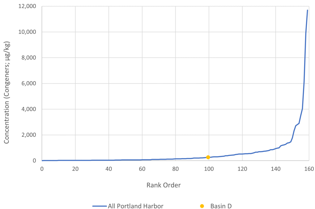
Figure A - 16. PCB Congeners in Stormwater Solids at T4 Compared to “Typical” Industrial Stormwater in the Portland Harbor
