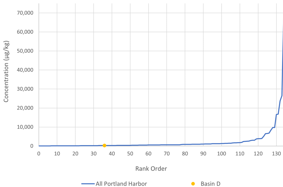
Figure A - 25. Silver in Stormwater Solids at T4 Compared to “Typical” Industrial Stormwater in the Portland Harbor
