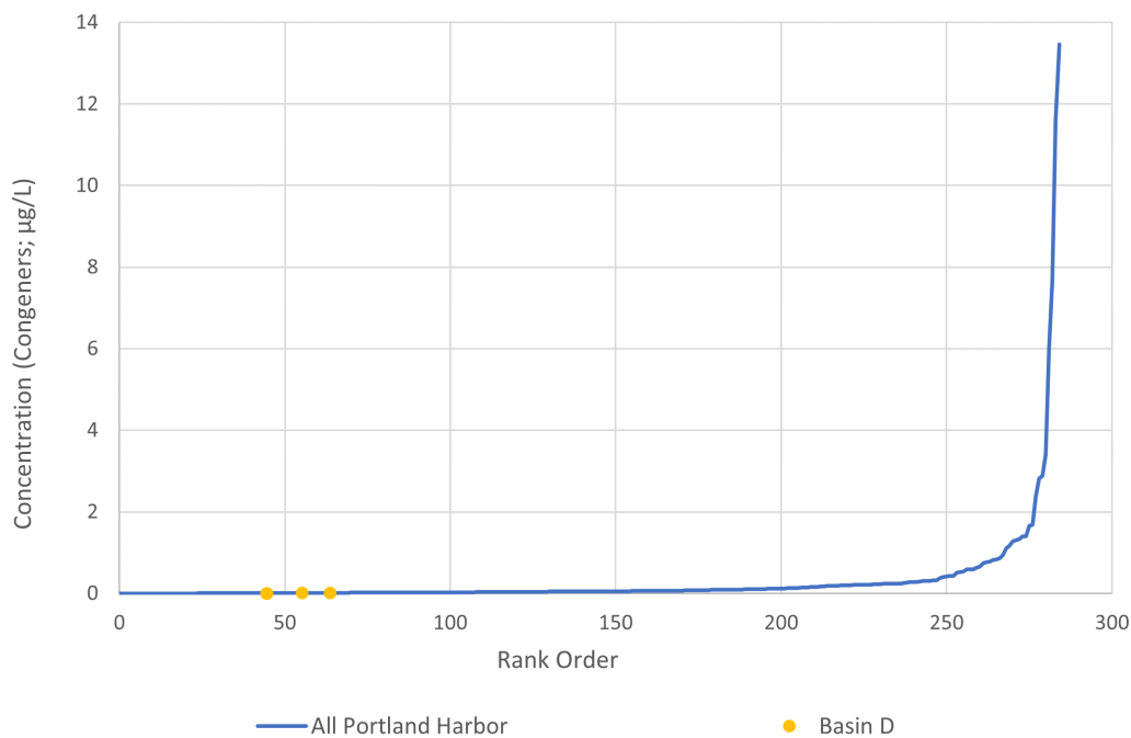
Figure A - 3. Total PCB Congeners in Stormwater at T4 Compared to “Typical” Industrial Stormwater in the Portland Harbor
