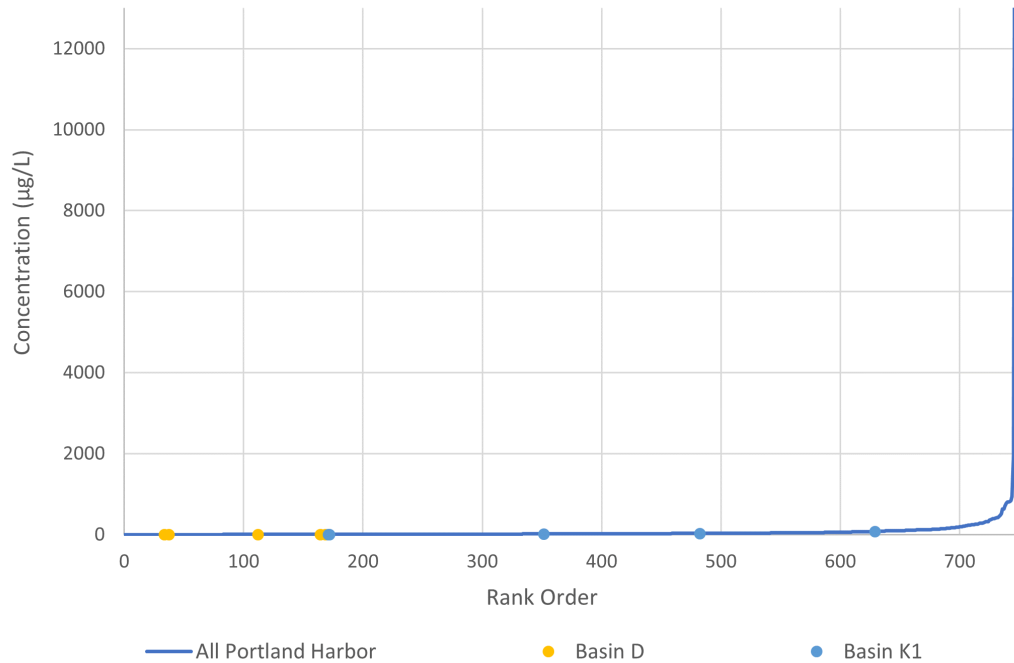
Figure A - 8. Copper in Stormwater at T4 Compared to “Typical” Industrial Stormwater in the Portland Harbor
