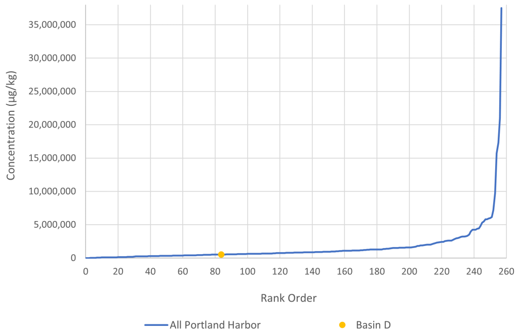
Figure A - 26. Zinc in Stormwater Solids at T4 Compared to “Typical” Industrial Stormwater in the Portland Harbor
