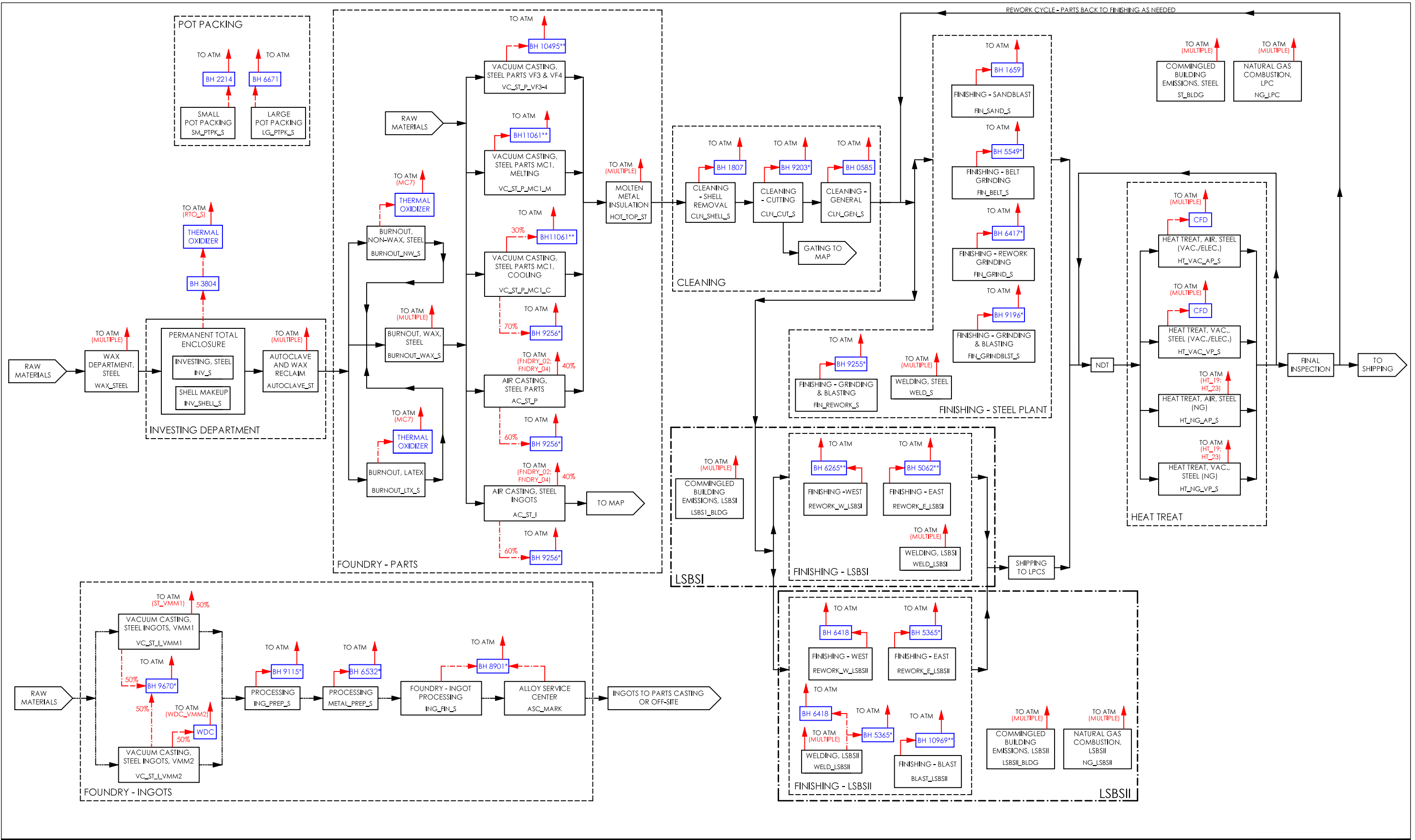
Figure 1 Process Flow Diagram - Steel PCC Structurals - Large Parts Campus Milwaukie, Oregon
