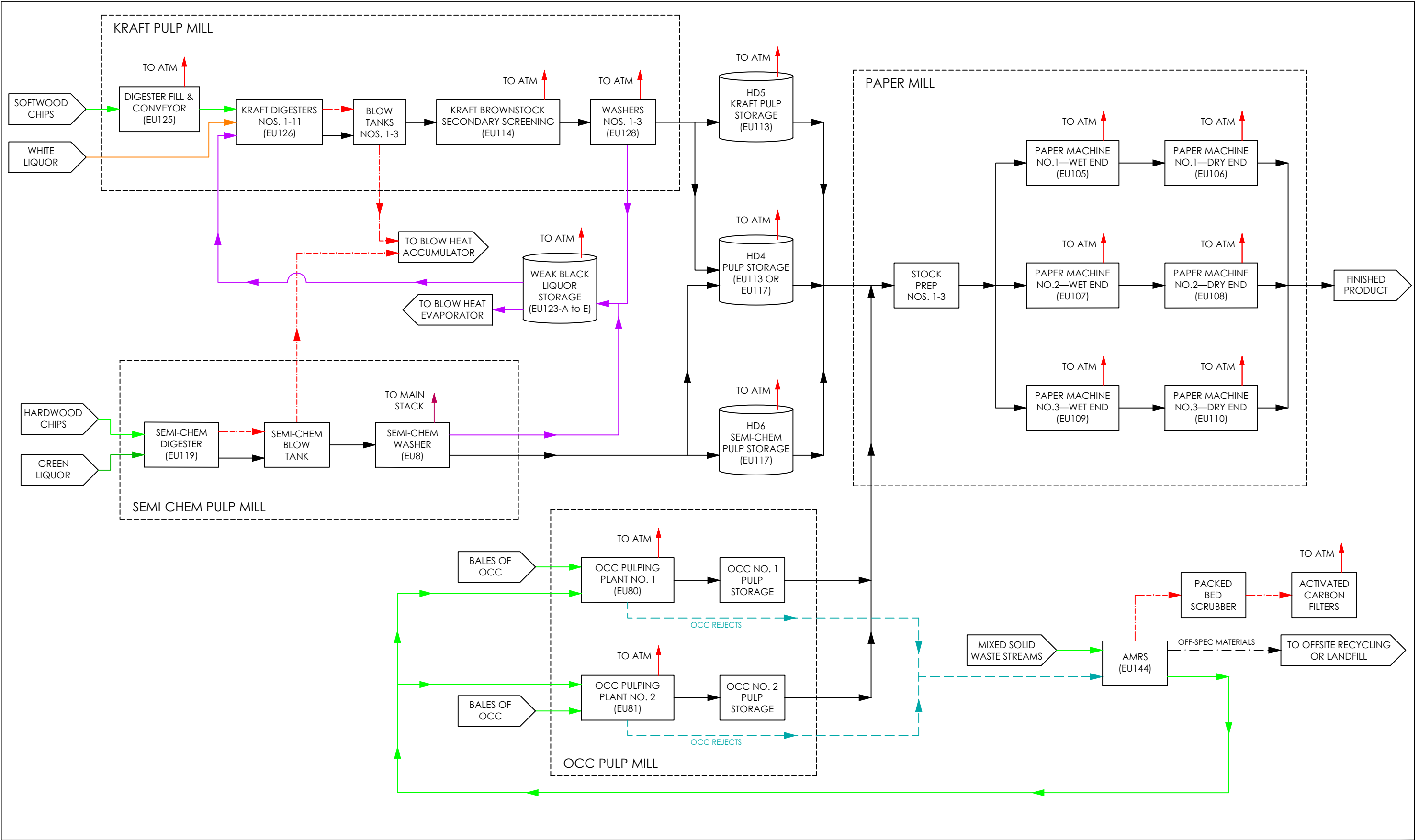
Figure 1 - Process Flow Diagram Pulp and Paper Mills Georgia-Pacific LLC Toledo, Oregon
