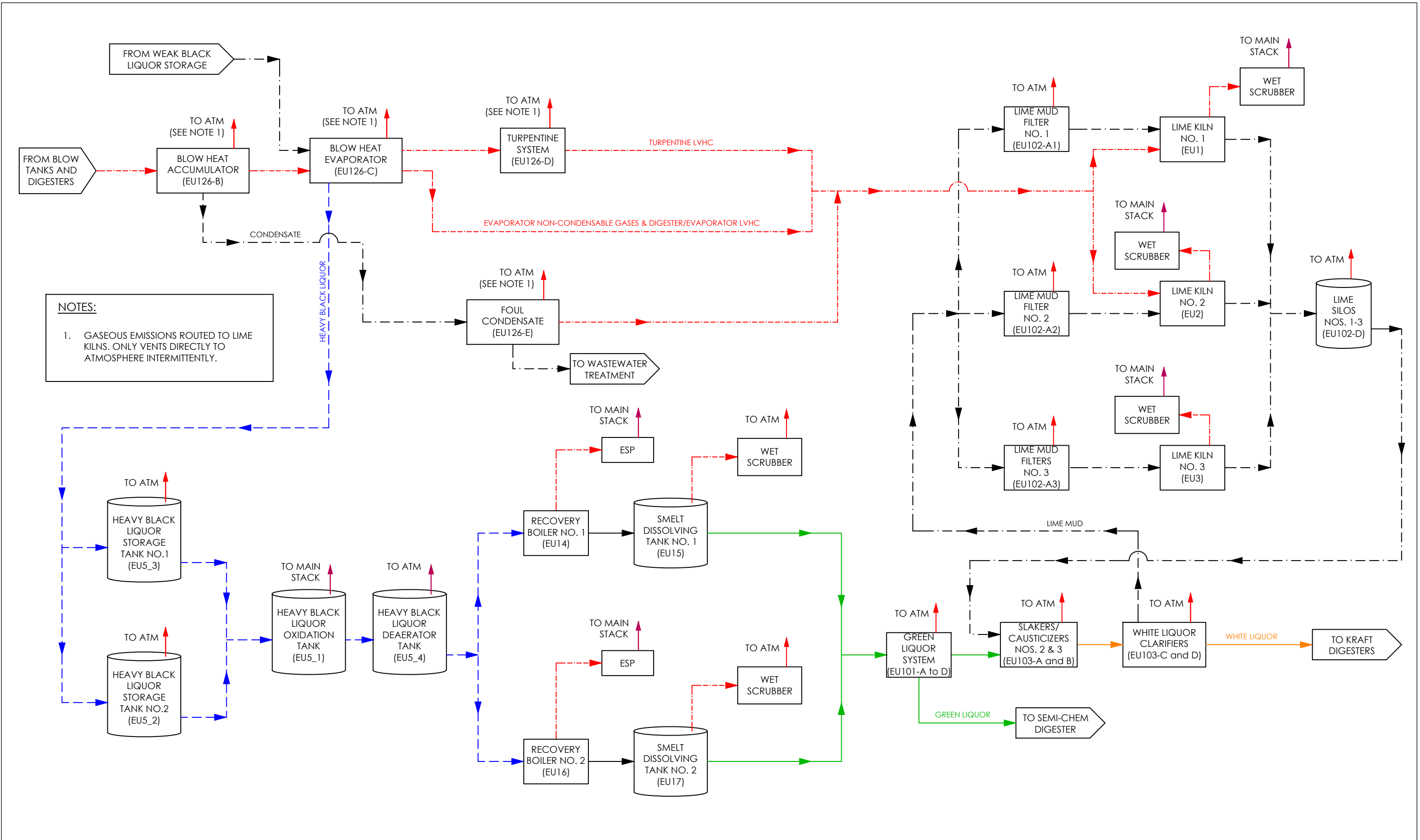
Figure 2 - Process Flow Diagram Chemical Recovery
