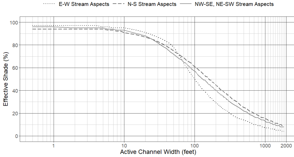
Figure 9-6: Effective shade targets for stream sites in the Qfc mapping unit.
