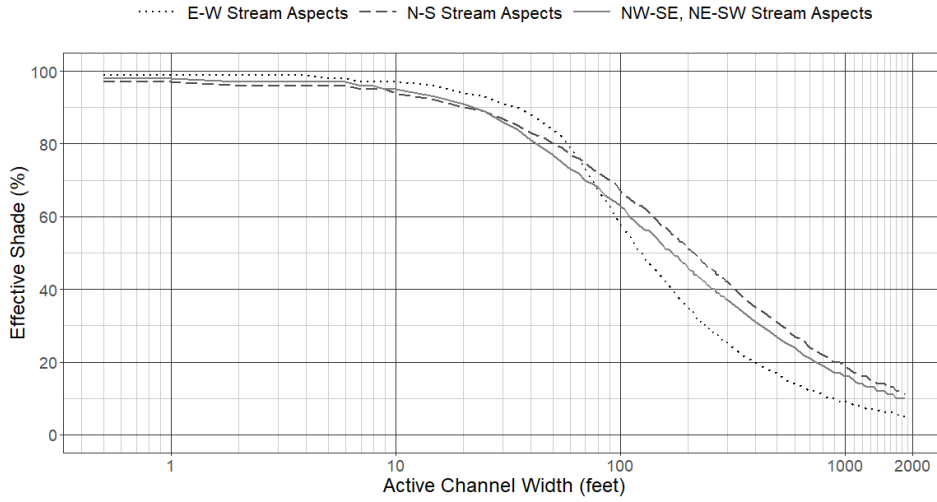
Figure 9-14: Effective shade targets for stream sites in the Qtg mapping unit.
