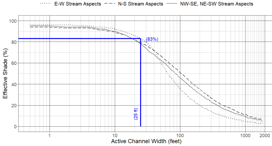
Figure 9-4: Example illustrating use of the shade curve for the Qalc mapping unit based on an east to west aspect and an active channel width of 25 ft.
