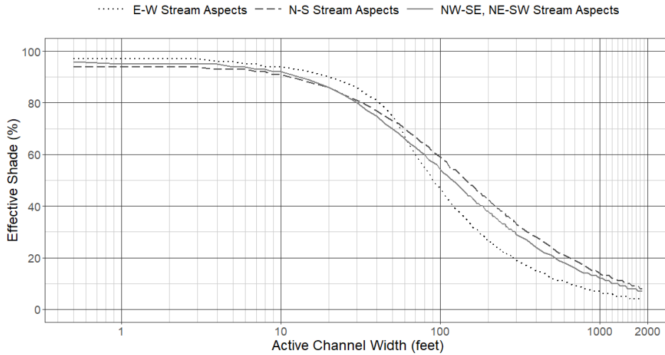
Figure 9-15: Effective shade targets for stream sites in the Tvw mapping unit.
