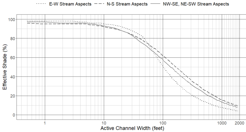
Figure 9-16: Effective shade targets for stream sites in the Tcr mapping unit.
