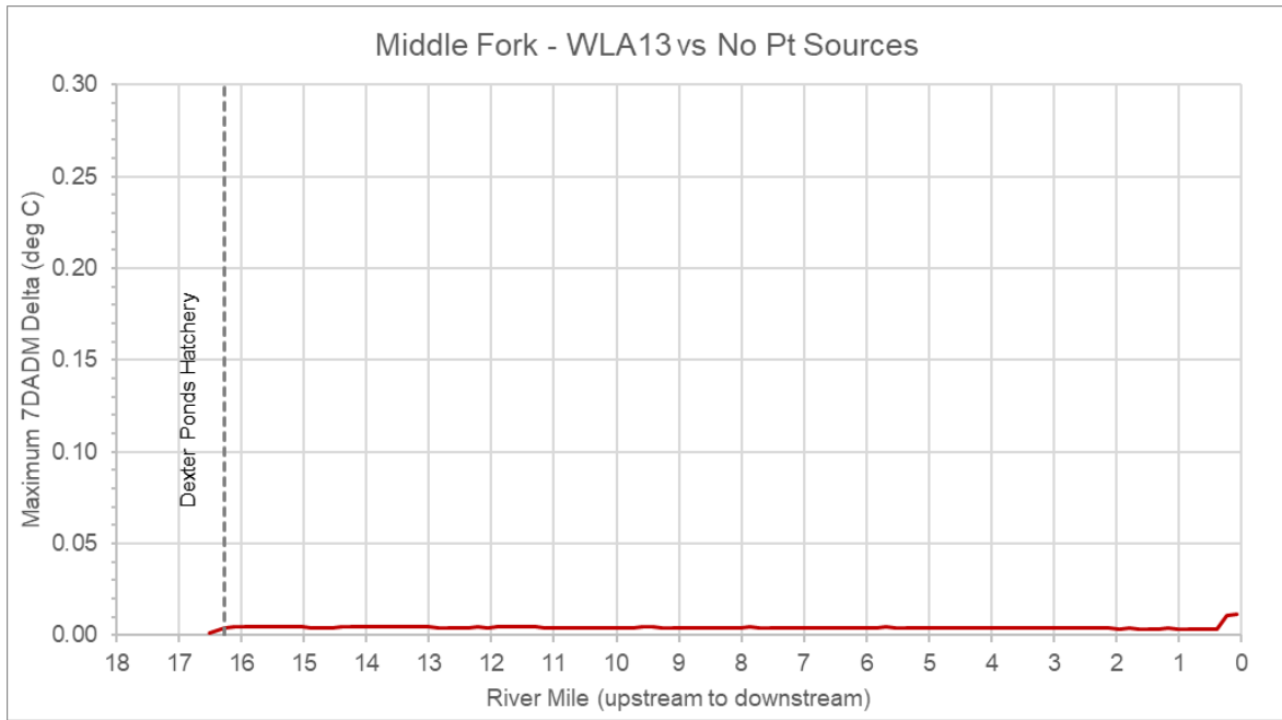
Figure 10-12 10-12 : Change in maximum 7DADM stream temperatures between the Wasteload Allocations and No Point Sources scenarios for the Middle Fork Willamette River over all time periods
