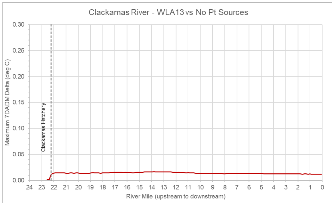
Figure 10-10-10: Change in maximum 7DADM stream temperatures between the Wasteload Allocations and No Point Sources scenarios for the Clackamas River over all time periods
