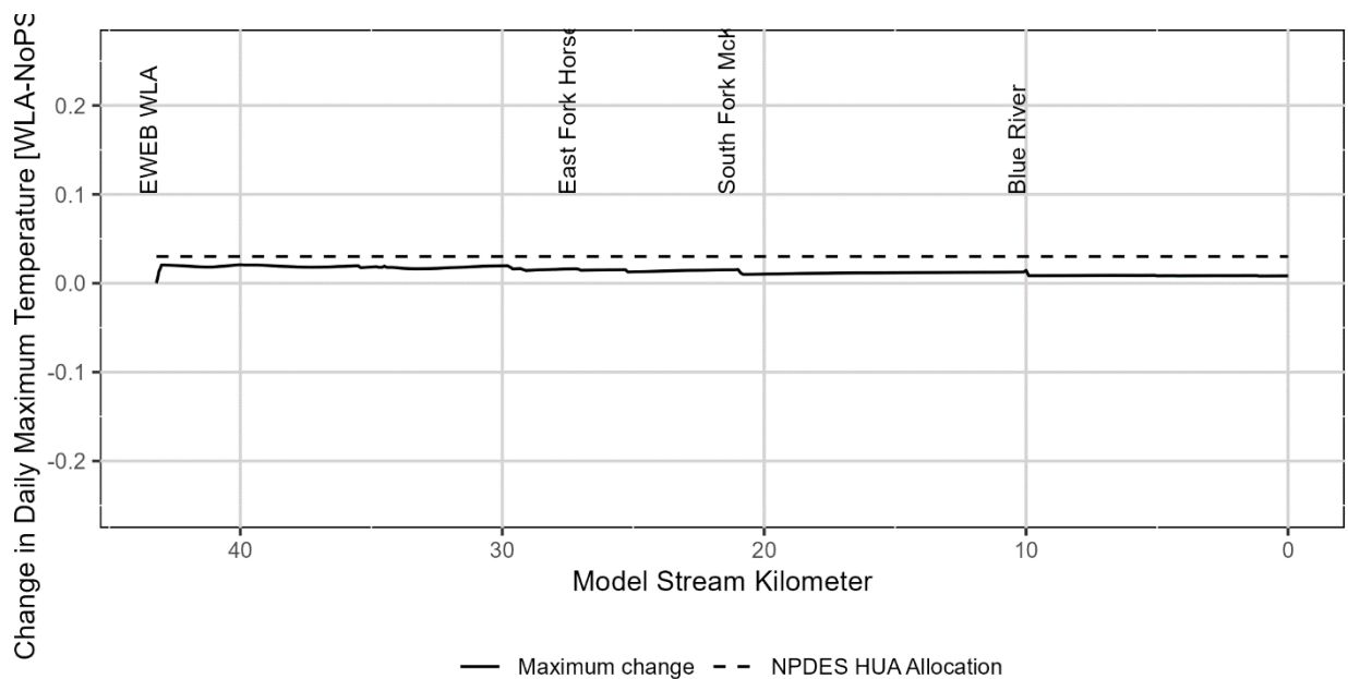
Figure 10-310-310-310-310-310-310-310-3: Change in daily maximum stream temperature between the Wasteload Allocations and No Point Sources model scenarios for the upper McKenzie River.
