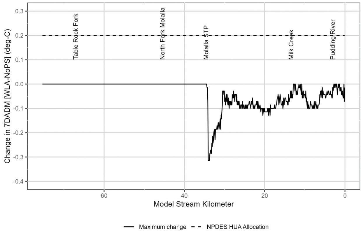
Figure 10-110-110-110-110-110-110-1: Change in maximum 7DADM stream temperatures between the Wasteload Allocations and No Point Sources scenarios for the Molalla River over the entire model period.
