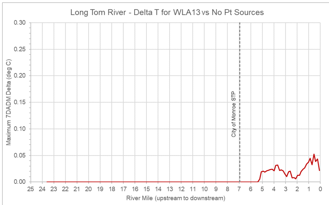
Figure 10-710-710-7: Change in maximum 7DADM stream temperatures between the Wasteload Allocations and No Point Sources scenarios for the Long Tom River over all time periods
