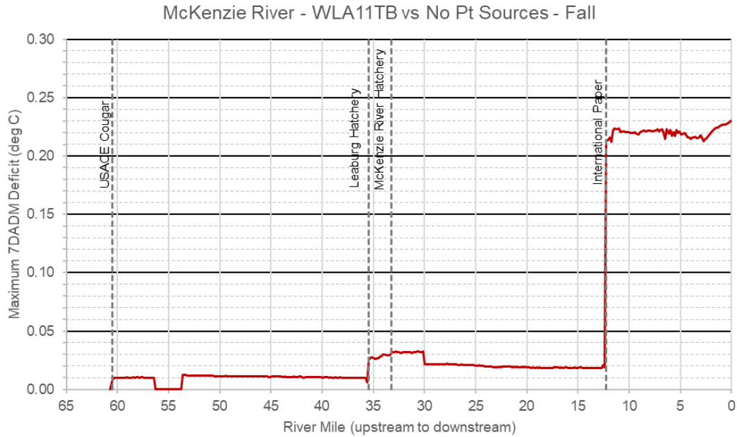
Figure 10-610-610-610-610-610-610-6: Change in maximum 7DADM stream temperatures between the Wasteload Allocations and No Point Sources scenarios for the McKenzie River over the fall spawning period.
