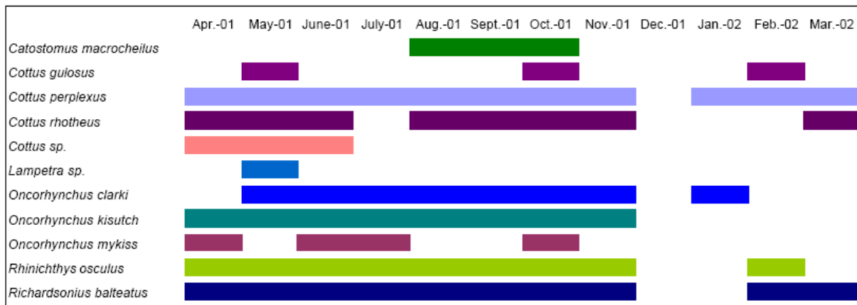
Figure 4- 144-144-144-144-144-144-134-124-11 : Temporal distribution of fish species encountered upstream of the lower reach for comparison, at approximately river mile 16 (Site #6) April 2001 – March 2002 (Chastain et al., 2002, Figure 3f).
