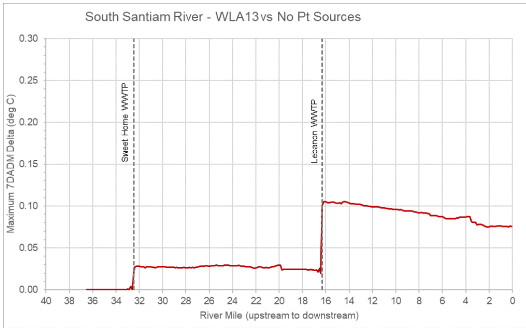
Figure 10-810-8: Change in maximum 7DADM stream temperatures between the Wasteload Allocations and No Point Sources scenarios for the South Santiam River over all time periods
