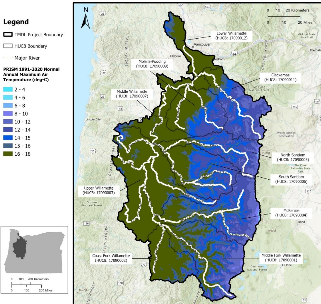
Figure 2-42-42-42-42-42-42-4: PRISM 1991-2020 Normal Annual Maximum Air Temperature in the Willamette Subbasins temperature TMDL project area (Data Source: PRISM Climate Group, 2022).
