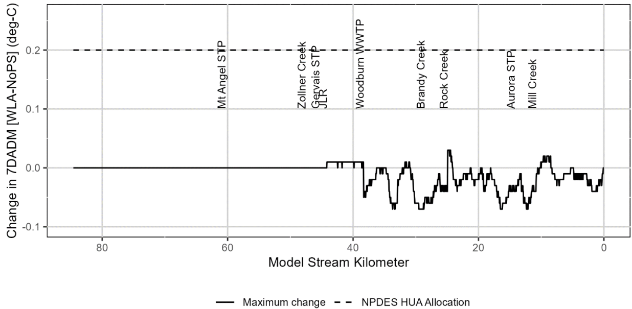
Figure 10-210-210-210-210-210-210-210-2: Change in maximum 7DADM stream temperatures between the Wasteload Allocations and No Point Sources scenarios for the Pudding River over the entire model period.
