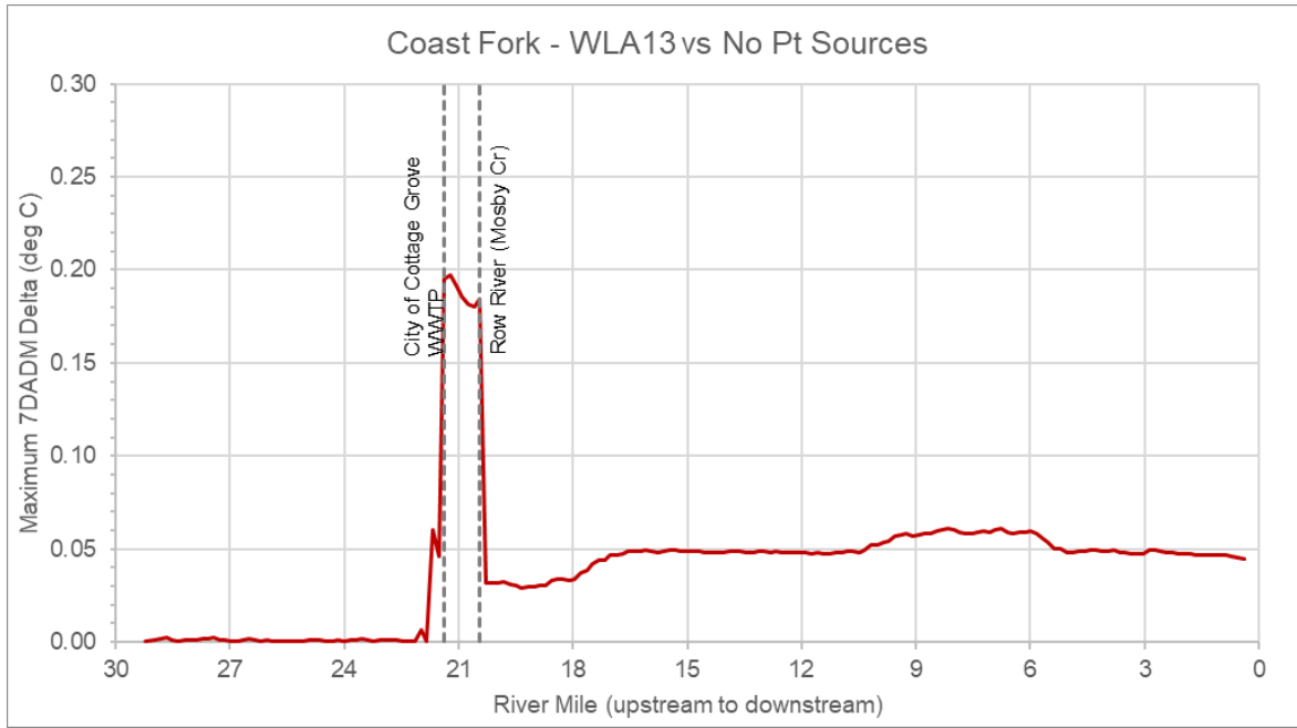
Figure 10-11 10-11 : Change in maximum 7DADM stream temperatures between the Wasteload Allocations and No Point Sources scenarios for the Coast Fork Willamette River over all time periods
