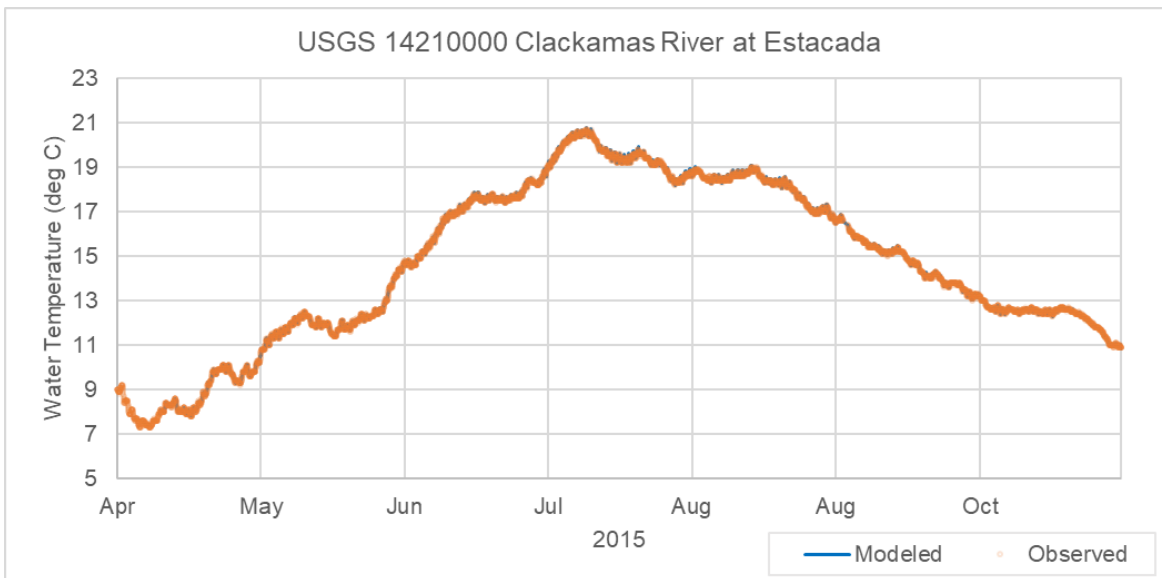
Figure 4-19. Clackamas River at Estacada water temperature comparison, 2015
