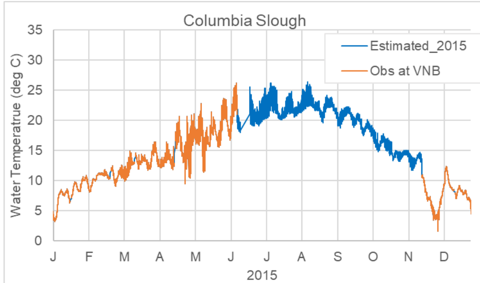
Figure 3-25. Temperature time series developed using observed data and calculated values for Columbia Slough
