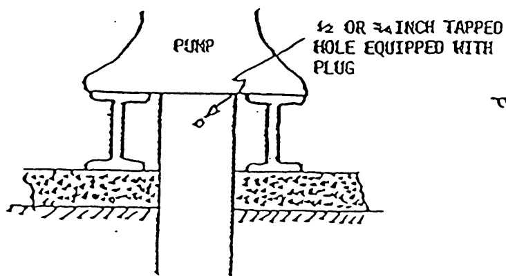
ACCESS PORT FOR MEASURING DEVICE
