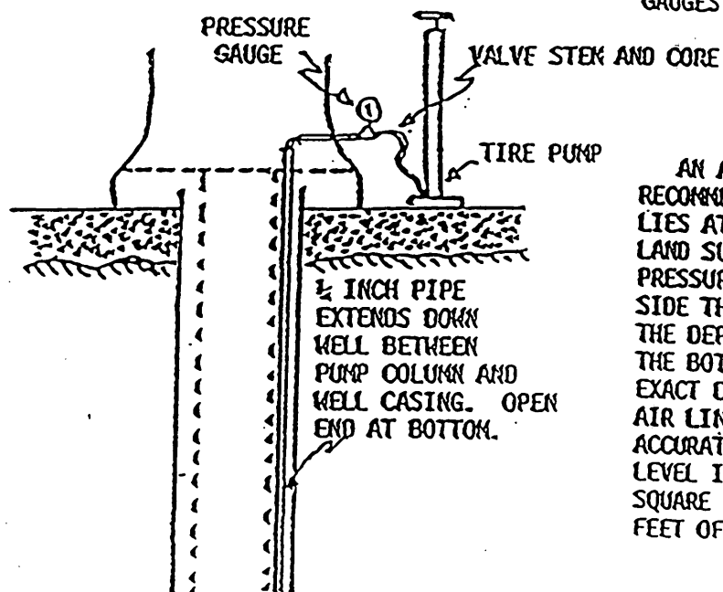
AIR LINE INSTALLATION
