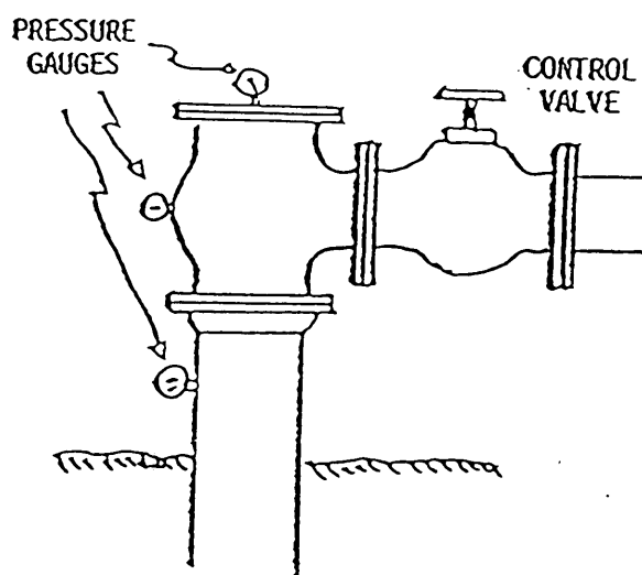
POSSIBLE LOCATION FOR PRESSURE GAUGES ON AN ARTESIAN WELL
