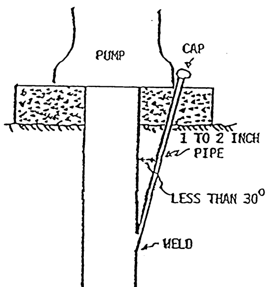
ACCESS PORT FOR MEASURING DEVICE
