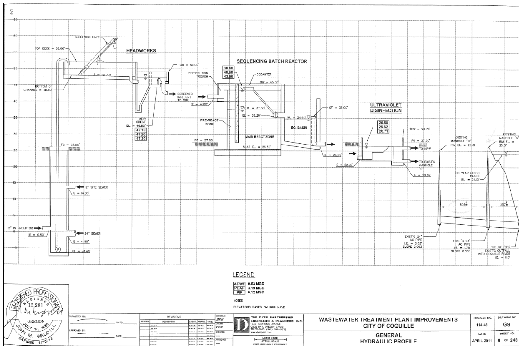
Figure 2-3: Hydraulic Profile
