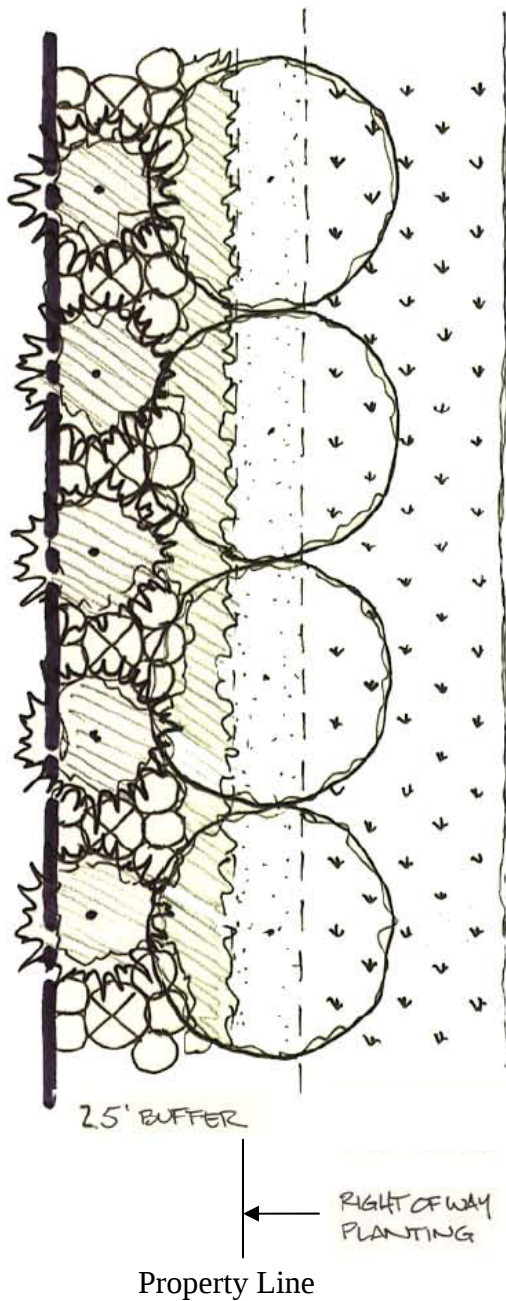
Figure 1: Highway 219 Landscaping Standards “Plan View”
